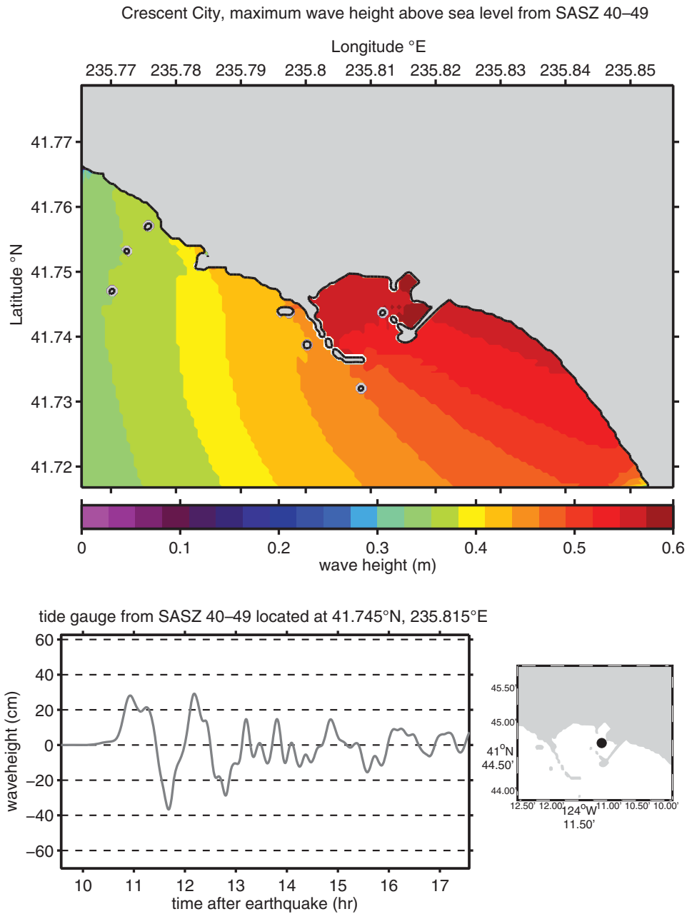
Figure 49: Maximum wave height plot and time series results for the forecast model using synthetic megatunami Event SASZ 40–49 for Crescent City, California.
