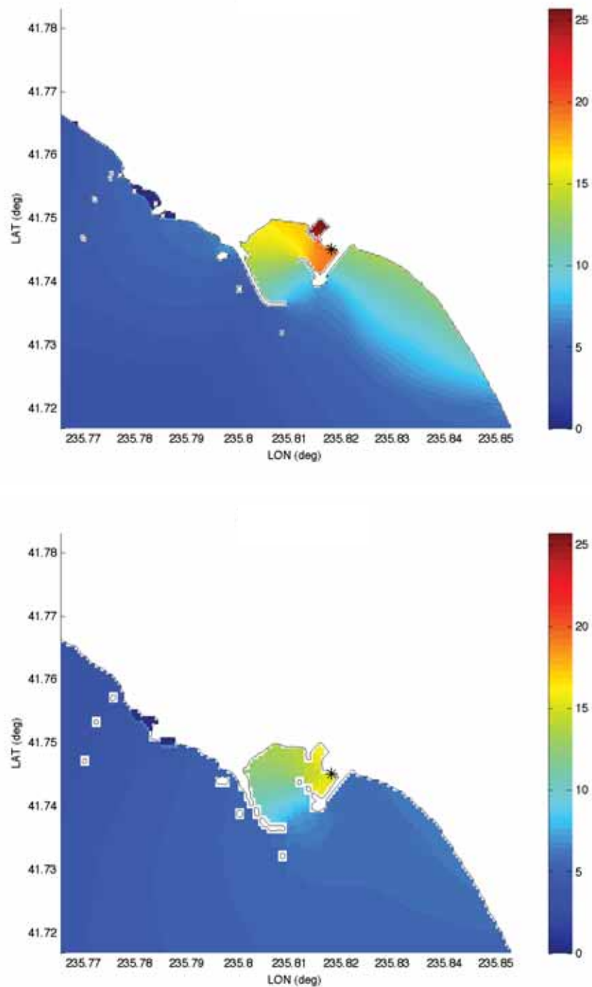
Figure 33: Maximum wave heights (cm) computed with forecast model grids. Asterisk indicates location of the tide gauge (reference model—upper, forecast model—lower) for the 1996 Andean event.
