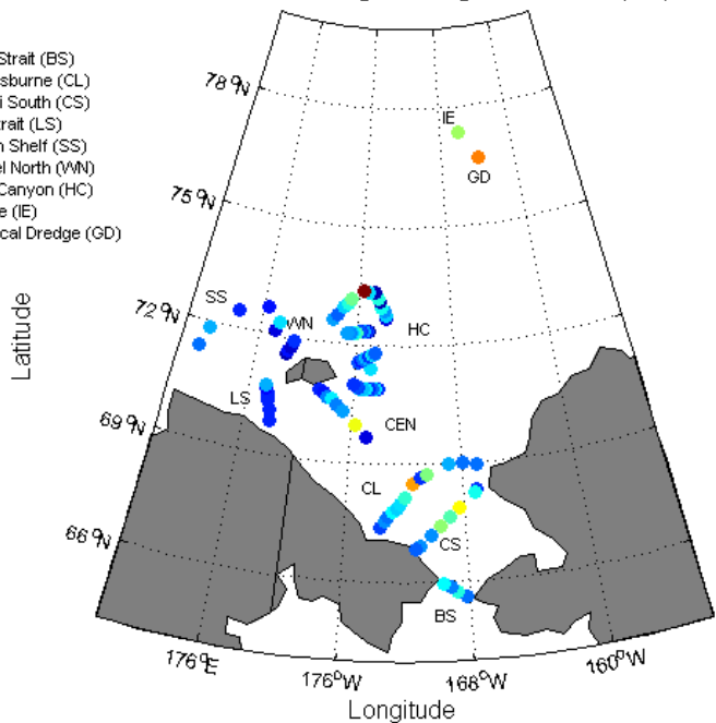
Rusalca 2009 Leg 2 Integrated PO 4 (μM)
