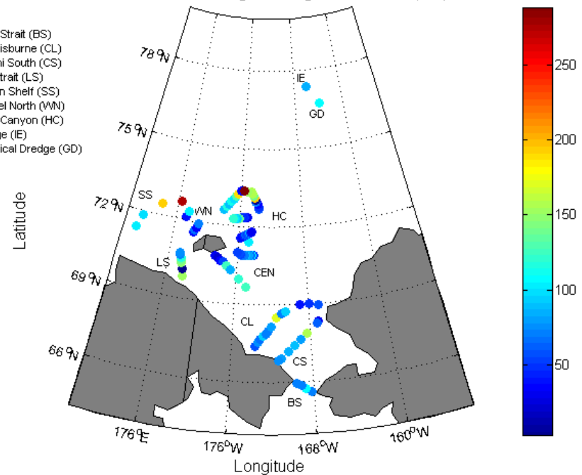
Rusalca 2009 Leg 2 Integrated SiO 4 (μM)
