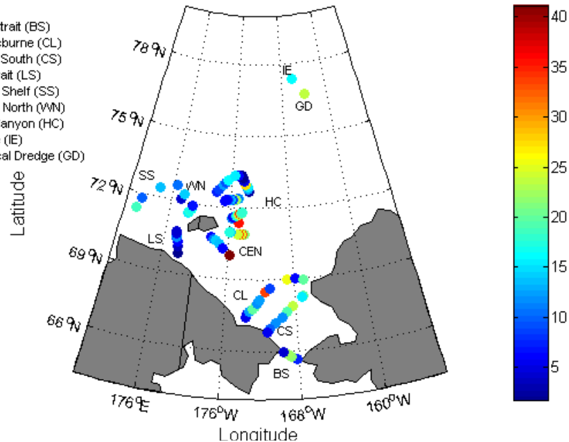
Rusalca 2009 Leg 2 Integrated SiO 4 (μM)
