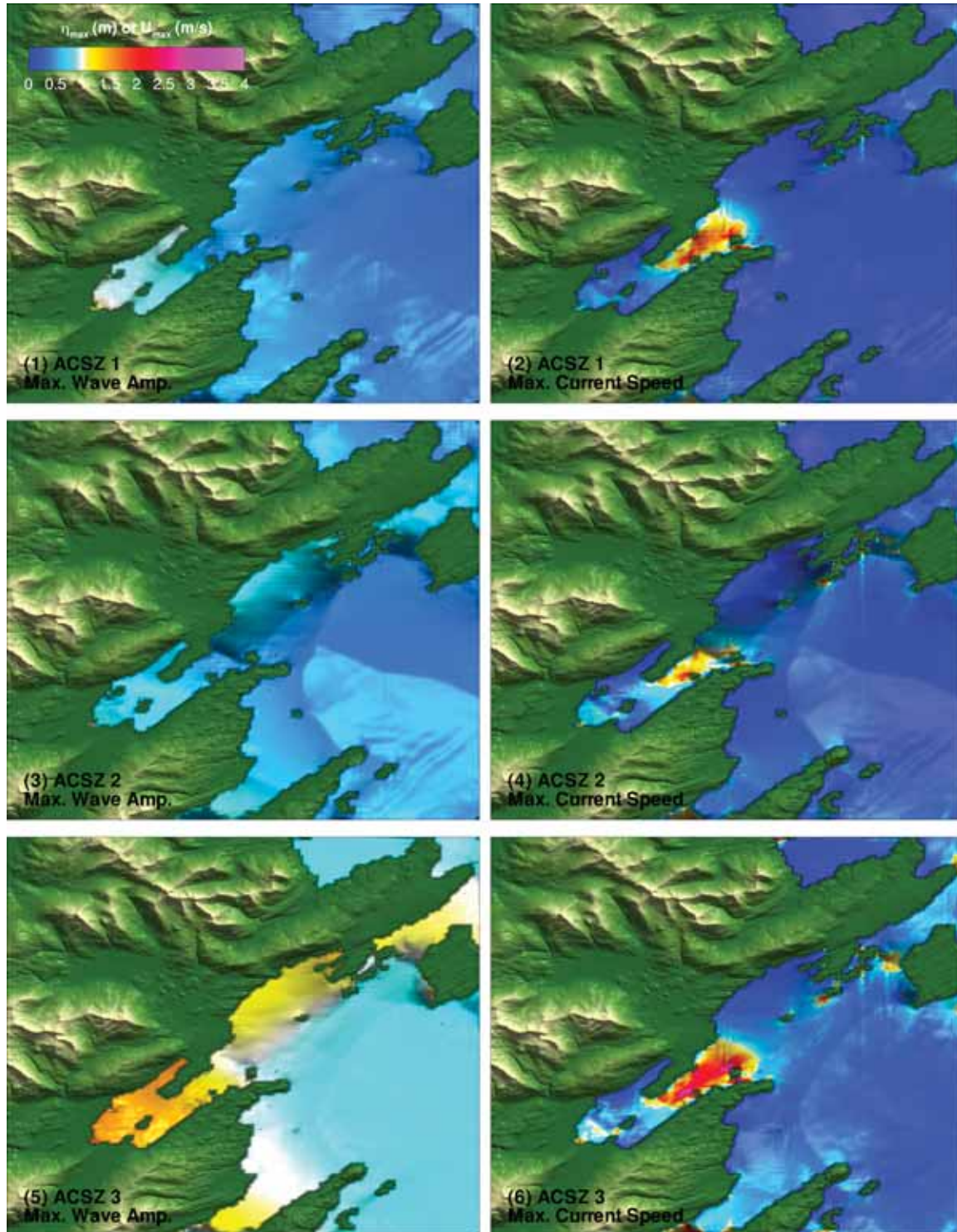
Figure 18: Computed tsunami wave amplitude and current speed in Kodiak, Alaska from 43 synthetic mega tsunami scenarios tested.
