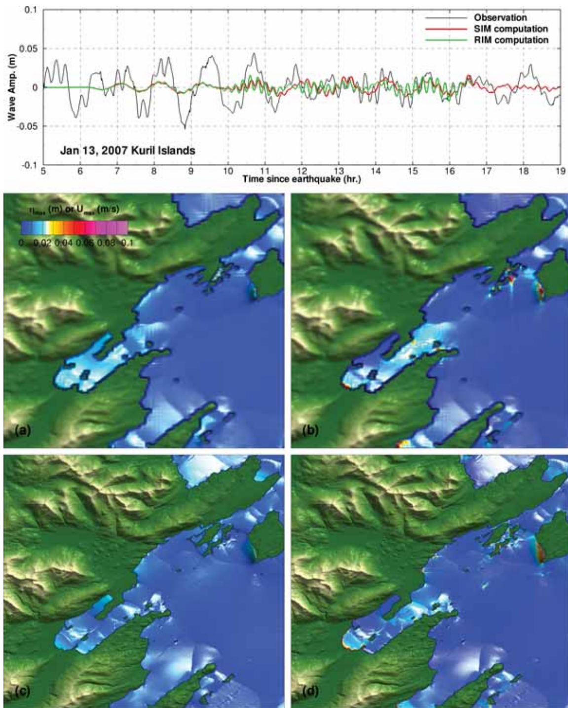
Figure 8: Model validation of forecast and reference model for 13 January 2007 Kuril Island tsunami. The upper panel shows the comparison of forecast (red) and reference (green) model against observations (black) at Kodiak tide station. The lower panel shows the computed maximum values of (a) forecast model wave amplitude (b) forecast model current speed (c) reference model wave amplitude; (d) reference model current speed.
