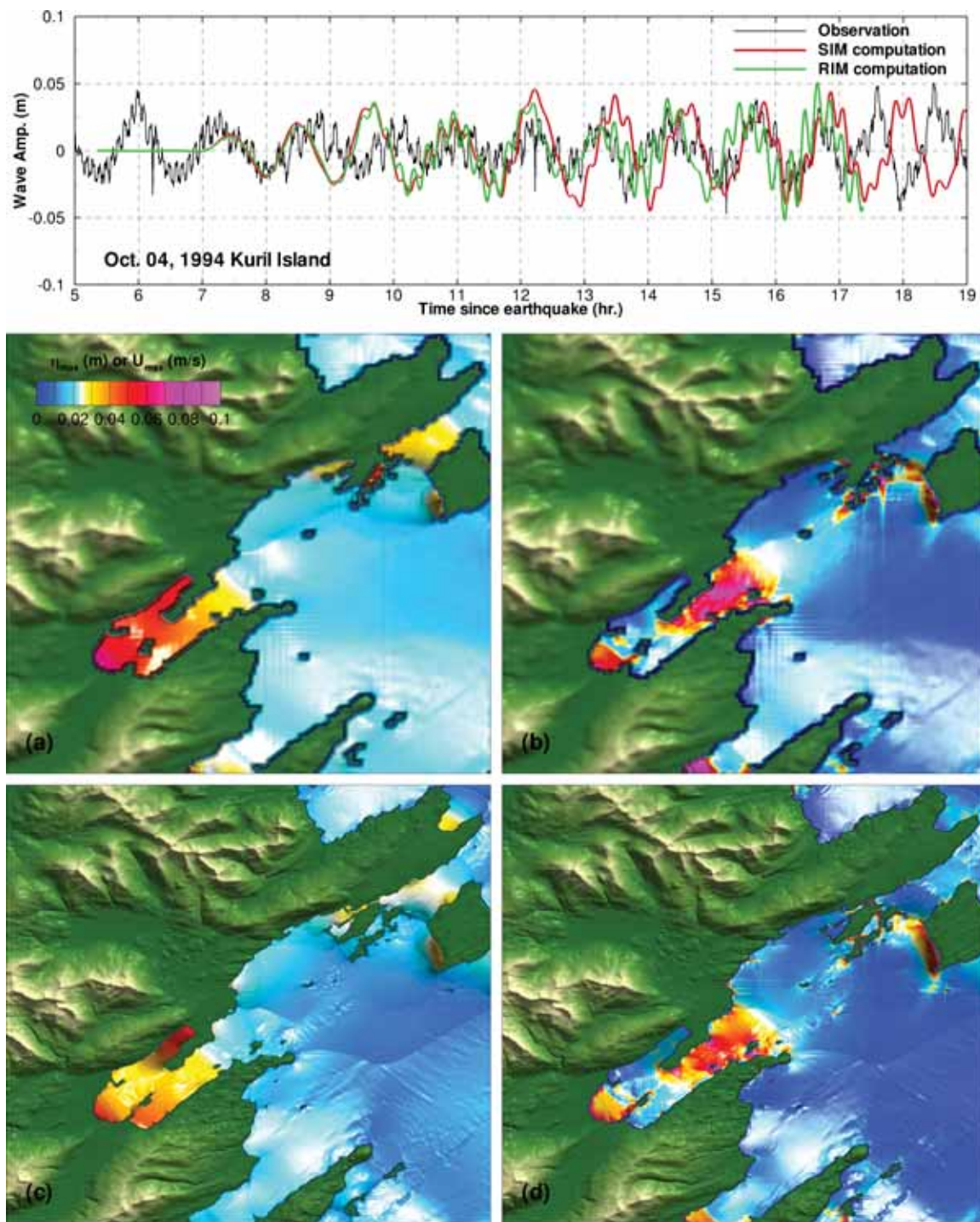
Figure 14: Model validation of forecast and reference model for 4 October 1994 Kuril Island tsunami. The upper panel shows the comparison of forecast (red) and reference (green) model against observations (black) at Kodiak tide station. The lower panel shows the computed maximum values of (a) forecast model wave amplitude (b) forecast model current speed (c) reference model wave amplitude; (d) reference model current speed.
