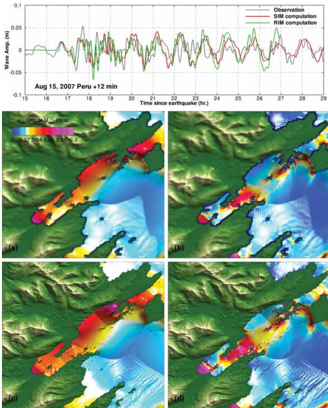
Figure 7: Model validation of forecast and reference model for 15 August 2007 Peru tsunami. The upper panel shows the comparison of forecast (red) and reference (green) model against observations (black) at Kodiak tide station. The lower panel shows the computed maximum values of (a) forecast model wave amplitude (b) forecast model current speed (c) reference model wave amplitude; (d) reference model current speed.
