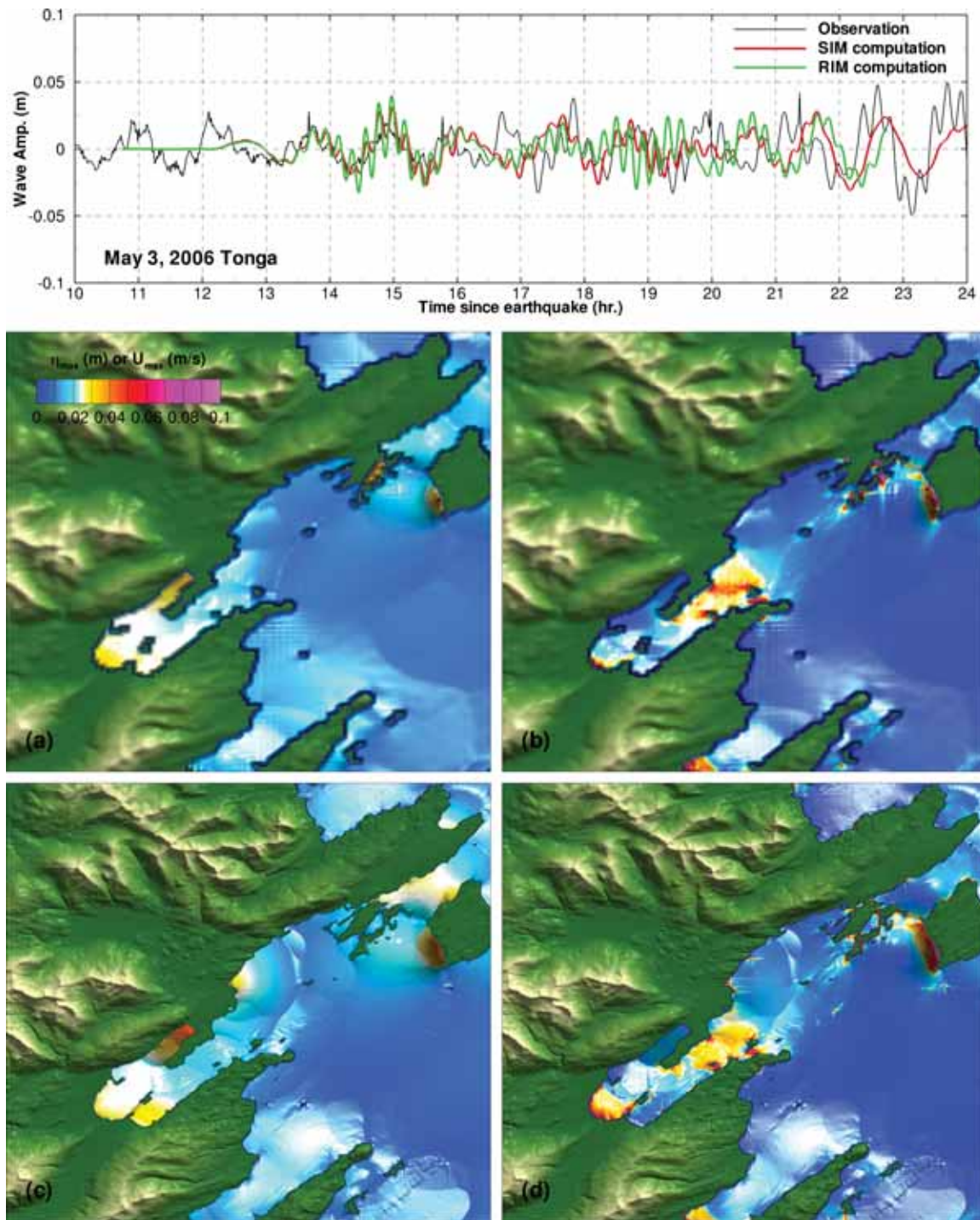
Figure 10: Model validation of forecast and reference model for 3 May 2006 Tonga tsunami. The upper panel shows the comparison of forecast (red) and reference (green) model against observations (black) at Kodiak tide station. The lower panel shows the computed maximum values of (a) forecast model wave amplitude (b) forecast model current speed (c) reference model wave amplitude; (d) reference model current speed.
