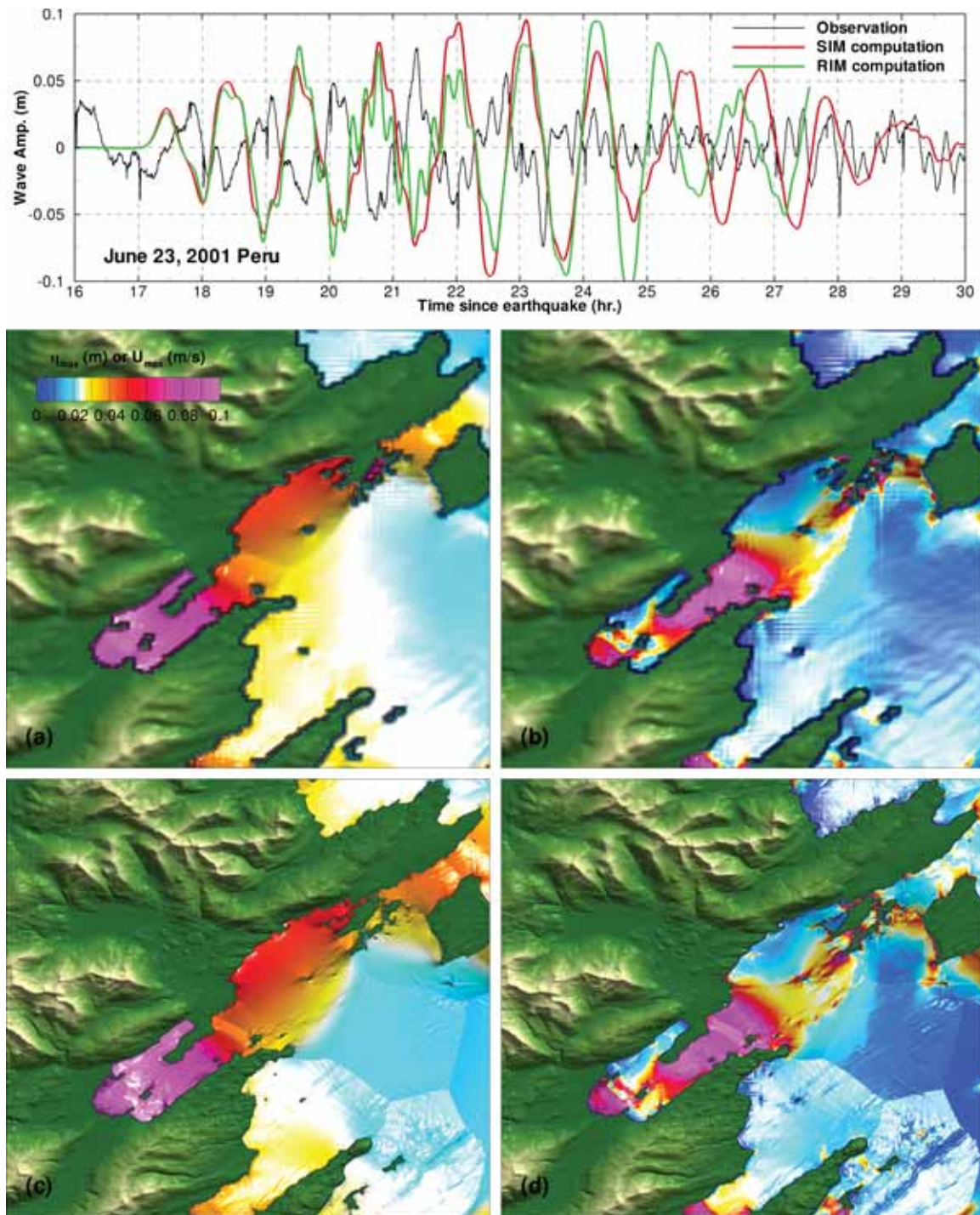
Figure 12: Model validation of forecast and reference model for 23 June 2001 Peru tsunami. The upper panel shows the comparison of forecast (red) and reference (green) model against observations (black) at Kodiak tide station. The lower panel shows the computed maximum values of (a) forecast model wave amplitude (b) forecast model current speed (c) reference model wave amplitude; (d) reference model current speed.
