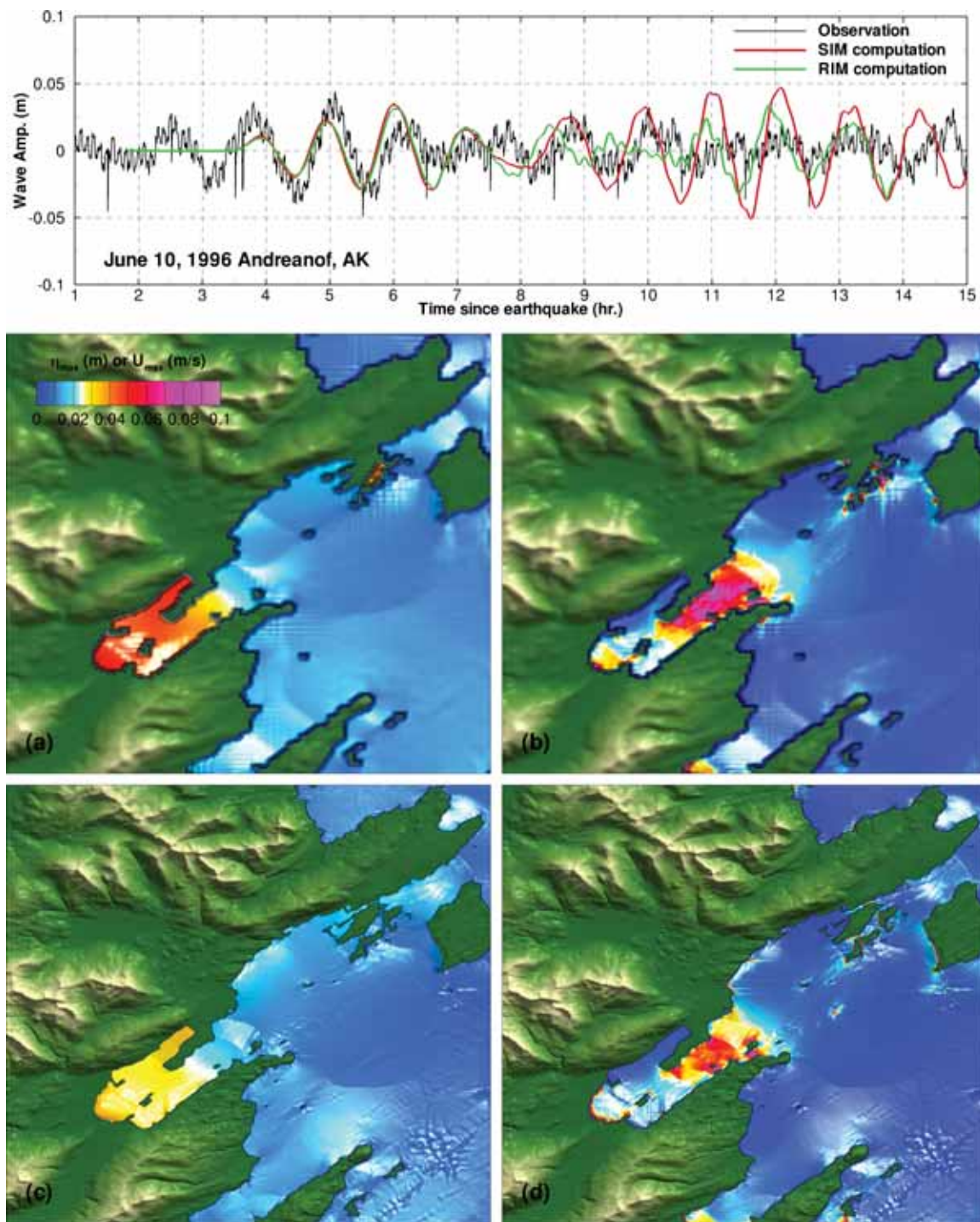
Figure 13: Model validation of forecast and reference model for 10 June 1996 Andreanof tsunami. The upper panel shows the comparison of forecast (red) and reference (green) model against observations (black) at Kodiak tide station. The lower panel shows the computed maximum values of (a) forecast model wave amplitude (b) forecast model current speed (c) reference model wave amplitude; (d) reference model current speed.
