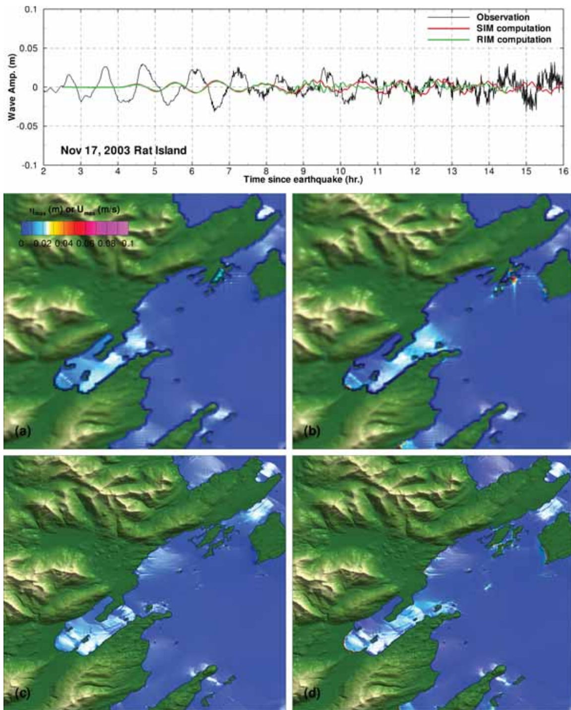
Figure 11: Model validation of forecast and reference model for 17 November 2003 Rat Island tsunami. The upper panel shows the comparison of forecast (red) and reference (green) model against observations (black) at Kodiak tide station. The lower panel shows the computed maximum values of (a) forecast model wave amplitude (b) forecast model current speed (c) reference model wave amplitude; (d) reference model current speed.
