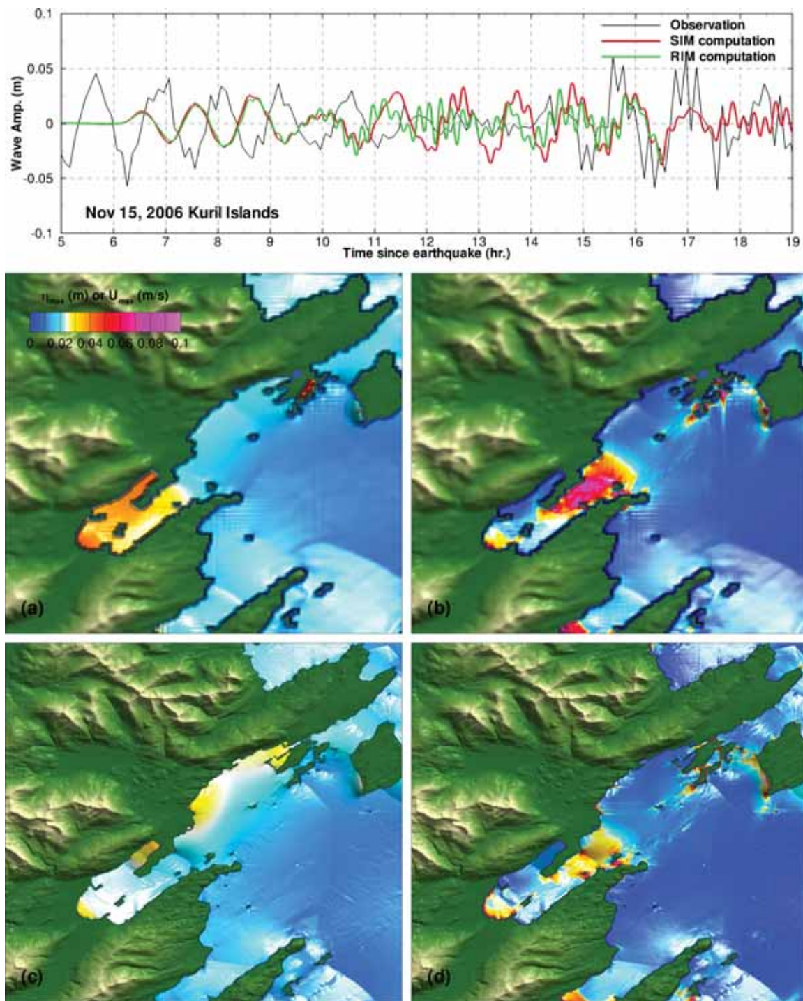
Figure 9: Model validation of forecast and reference model for 15 November 2006 Kuril Island tsunami. The upper panel shows the comparison of forecast (red) and reference (green) model against observations (black) at Kodiak tide station. The lower panel shows the computed maximum values of (a) forecast model wave amplitude (b) forecast model current speed (c) reference model wave amplitude; (d) reference model current speed.
