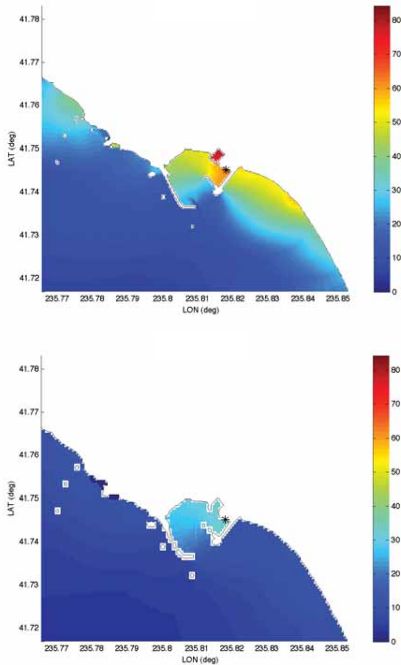
Figure 38: Maximum wave heights (cm) computed with forecast model grids. Asterisk indicates location of the tide gauge (reference model—upper, forecast model—lower) for the 2007 Kuril event.
