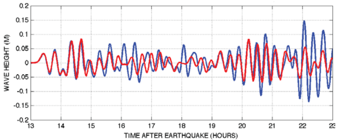
Figure 23: Time series comparison of reference vs. forecast model for the 2001 Peru event, blue—reference model, red—optimized forecast model.
