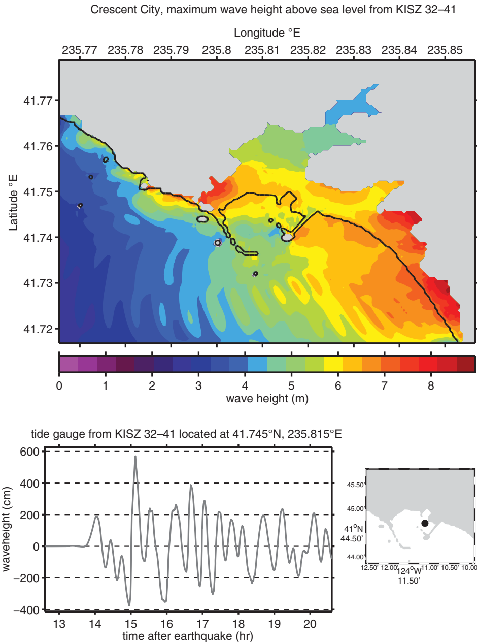
Figure 57: Maximum wave height plot and time series results for the forecast model using synthetic megatunami Event KISZ 32–41 for Crescent City, California.
