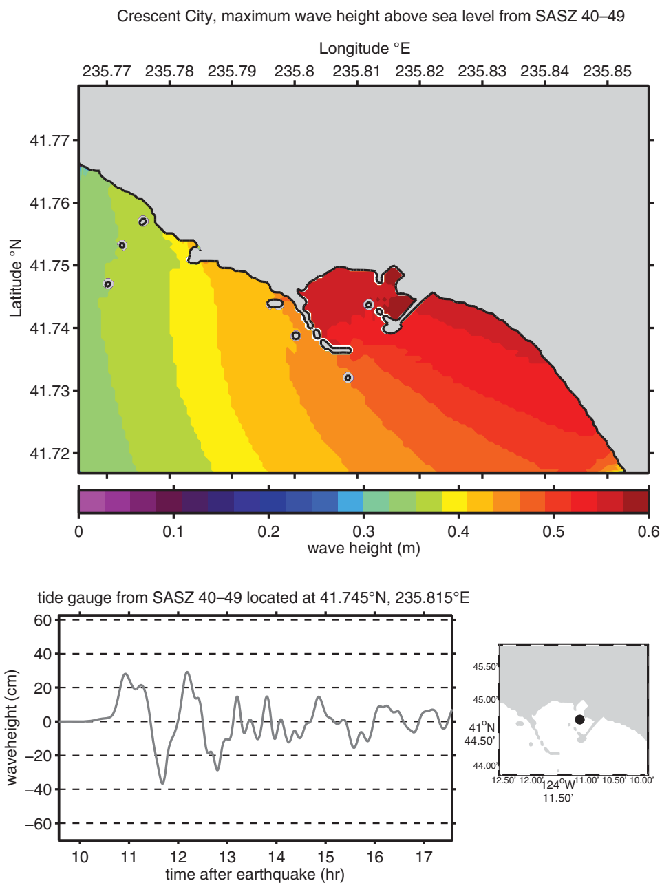
Figure 49: Maximum wave height plot and time series results for the forecast model using synthetic megatsunami Event SASZ 40–49 for Crescent City, California.
