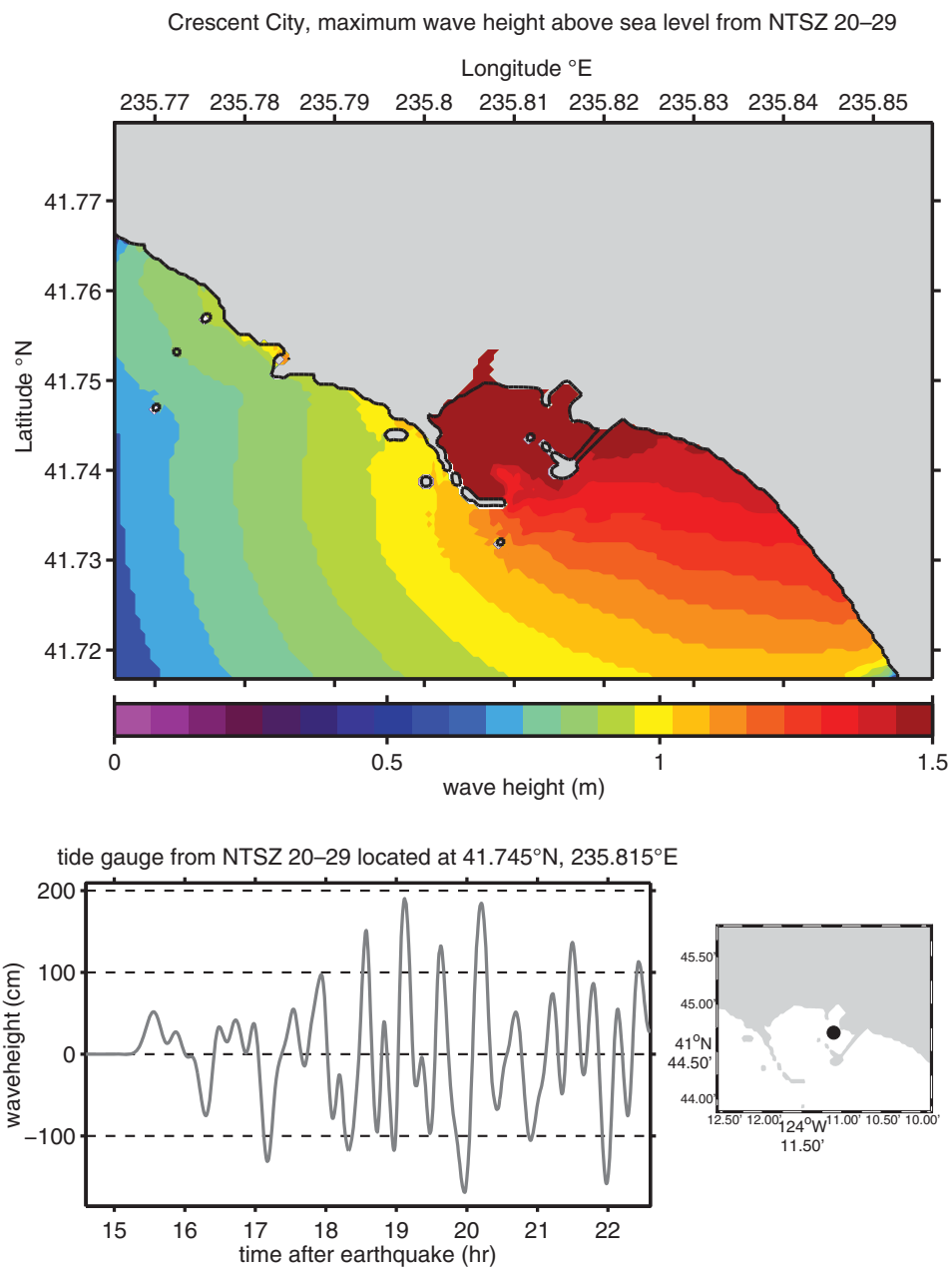
Figure 50: Maximum wave height plot and time series results for the forecast model using synthetic megatunami Event NTSZ 20–29 for Crescent City, California.
