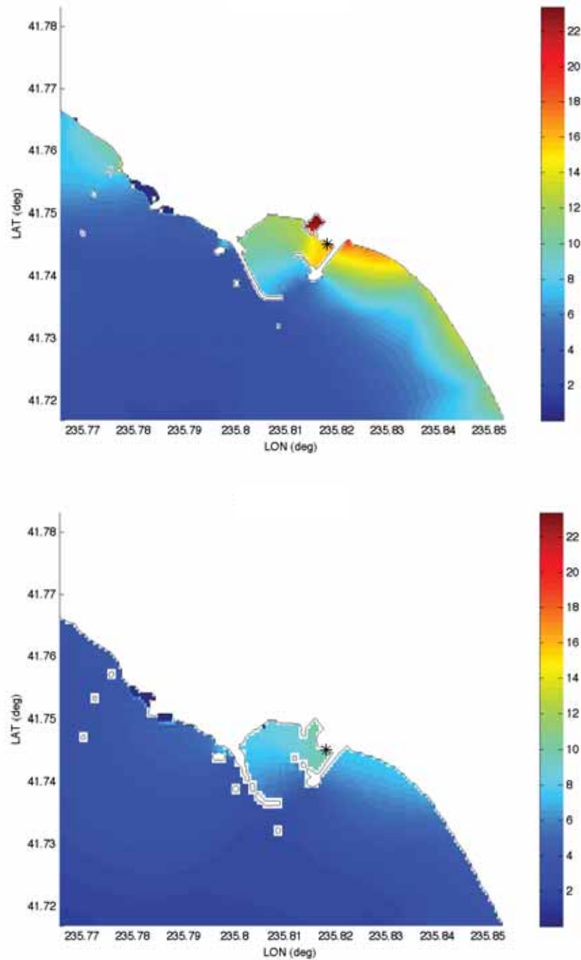
Figure 35: Maximum wave heights (cm) computed with forecast model grids. Asterisk indicates location of the tide gauge (reference model—upper, forecast model—lower) for the 2003 Rat Island event.
