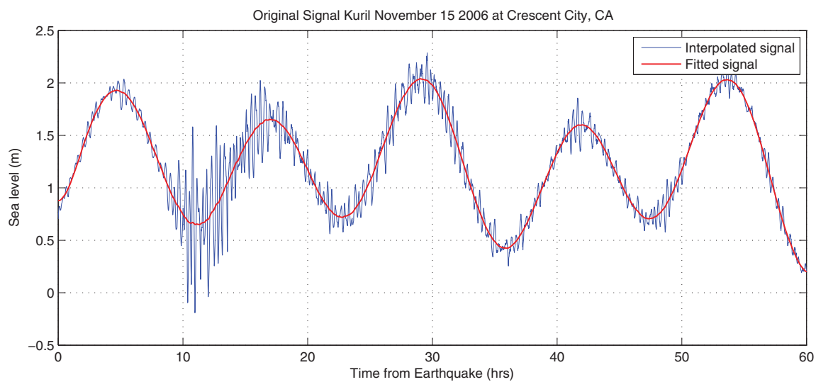
Figure 17: Original observed time series, spline fit, and tsunami signal, Kuril 2006.
