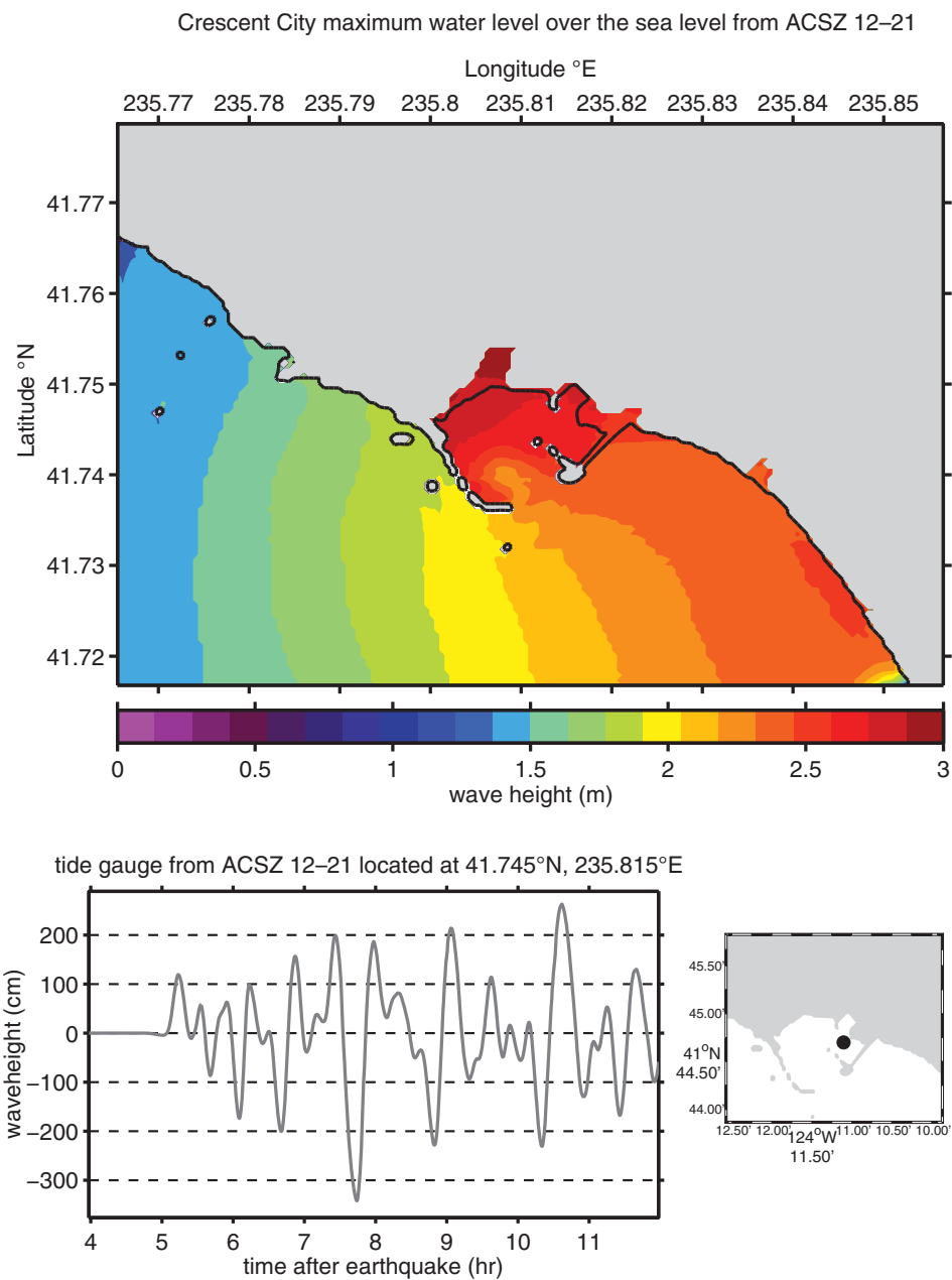
Figure 44: Maximum wave height plot and time series results for the forecast model using synthetic megatunami Event ACSZ 12–21 for Crescent City, California.
