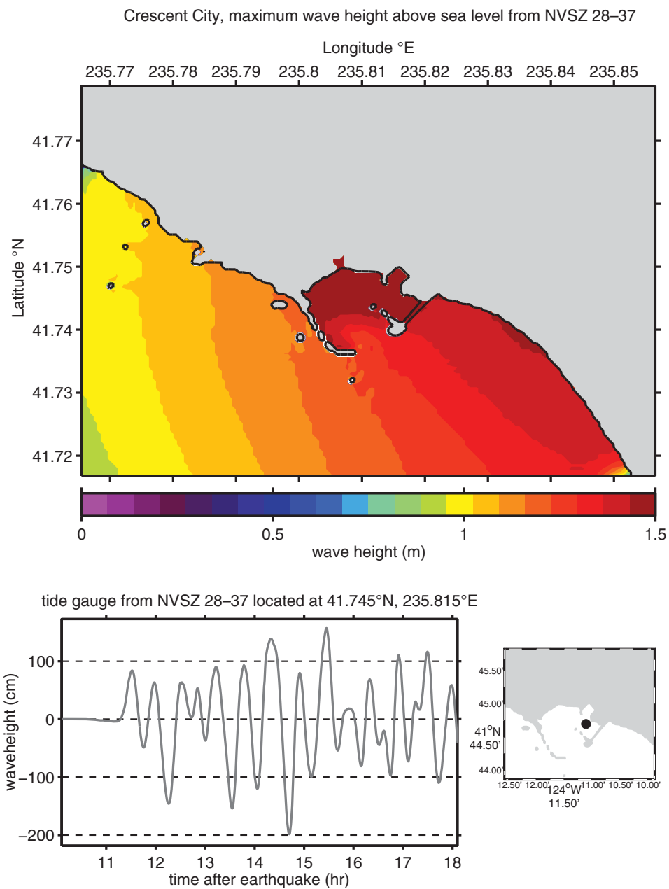
Figure 52: Maximum wave height plot and time series results for the forecast model using synthetic megatunami Event NVSZ 28–37 for Crescent City, California.
