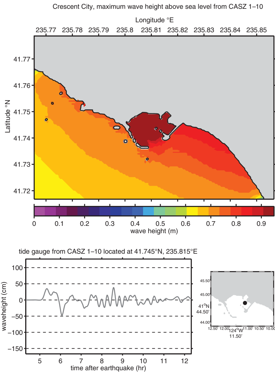
Figure 48: Maximum wave height plot and time series results for the forecast model using synthetic megatunami Event CASZ 1–10 for Crescent City, California.
