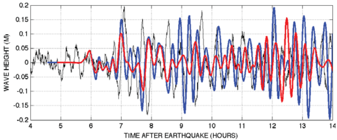
Figure 22: Time series comparison of tide gauge, reference model, and forecast model for the 1996 Andreanov event, black—tide gauge data, blue—reference model, red—optimized forecast model.
