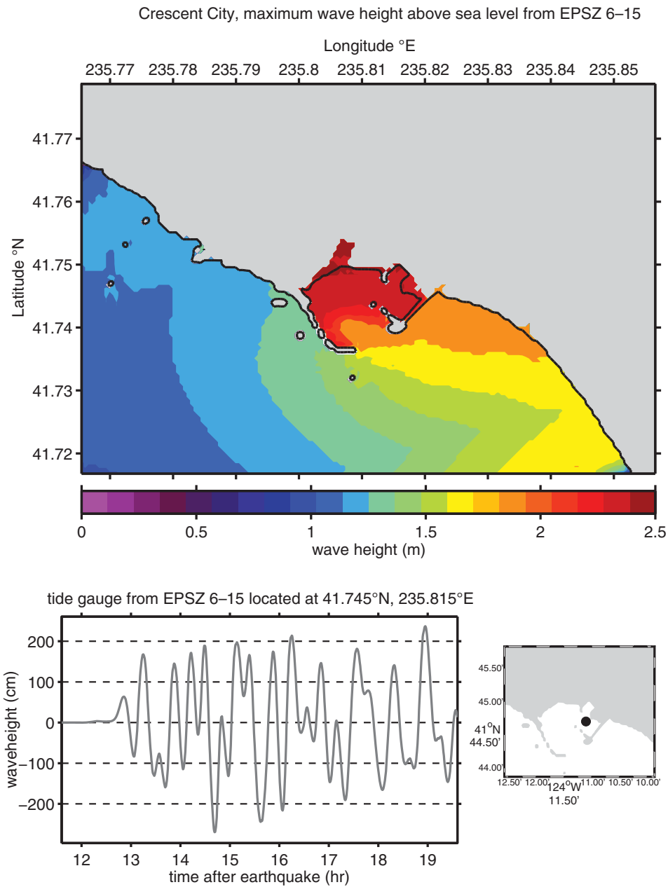
Figure 55: Maximum wave height plot and time series results for the forecast model using synthetic megatunami Event EPSZ 6–15 for Crescent City, California.
