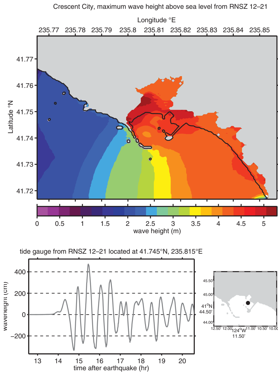
Figure 56: Maximum wave height plot and time series results for the forecast model using synthetic megatunami Event RNSZ 12–21 for Crescent City, California.
