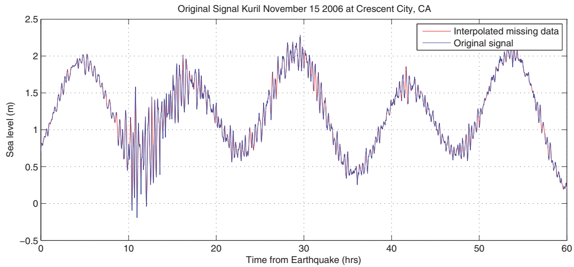
Figure 15: Original observed time series for 2006 Kuril event.
