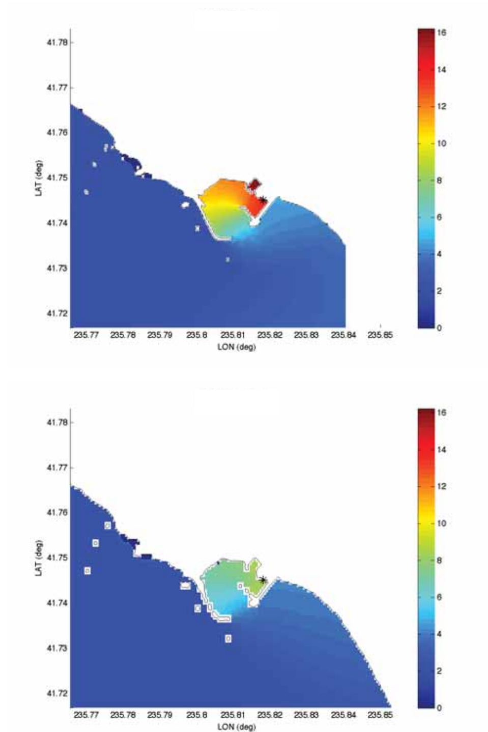
Figure 34: Maximum wave heights (cm) computed with forecast model grids. Asterisk indicates location of the tide gauge (reference model—upper, forecast model—lower) for the 2001 Peru event.
