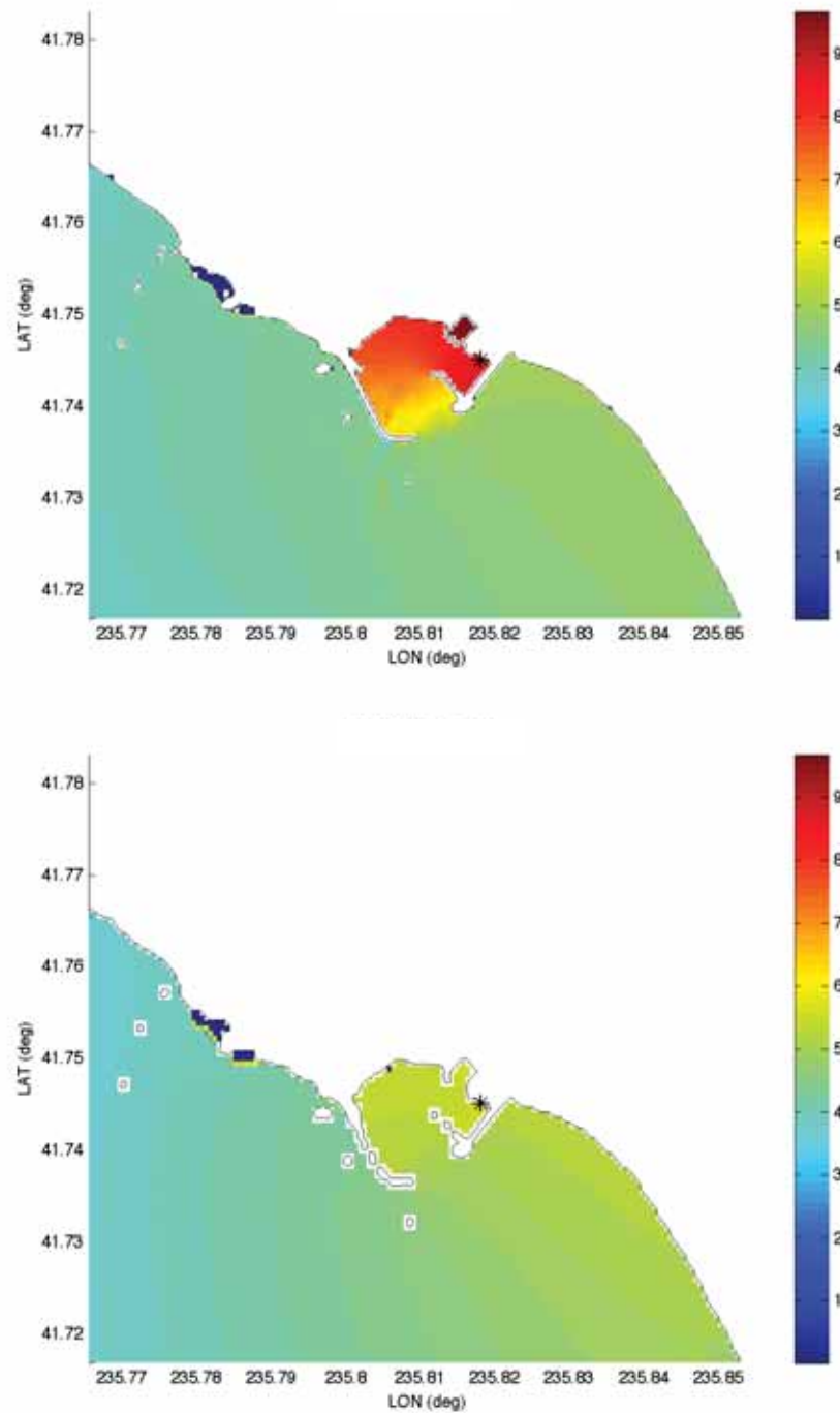
Figure 39: Maximum wave heights (cm) computed with forecast model grids. Asterisk indicates location of the tide gauge (reference model—upper, forecast model—lower) for the 2007 Solomon event.
