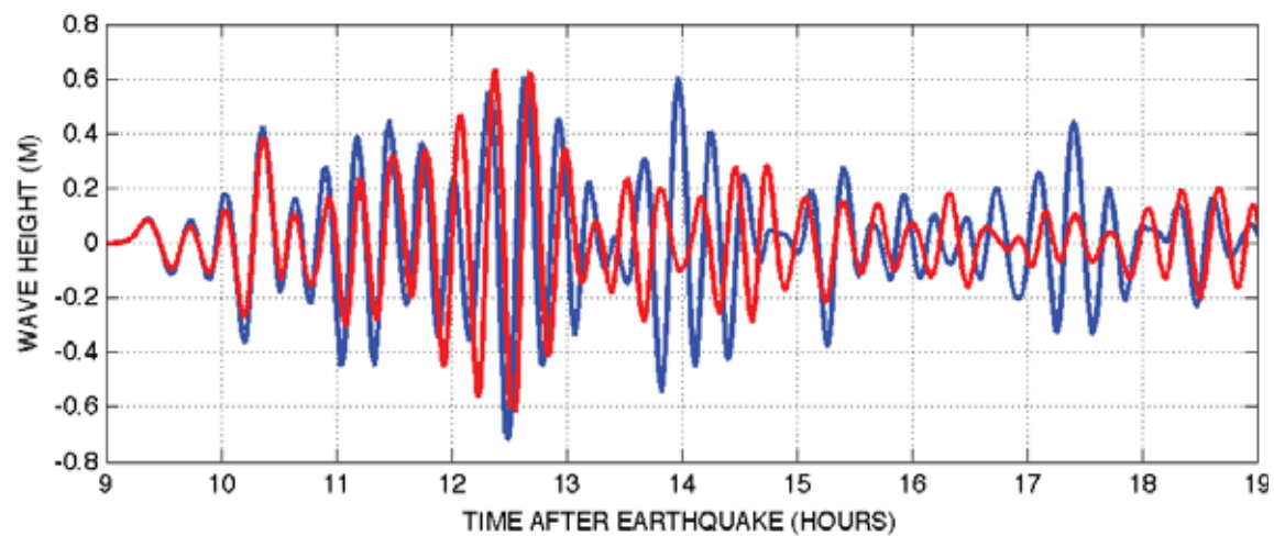
Figure 21: Time series comparison of reference vs. forecast model for the 1994 Kuril event, blue—reference model, red—optimized forecast model.
