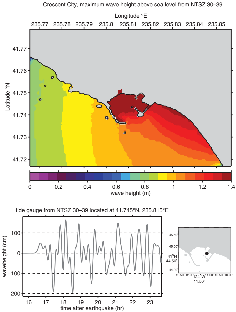
Figure 51: Maximum wave height plot and time series results for the forecast model using synthetic megatunami Event NTSZ 30–39 for Crescent City, California.
