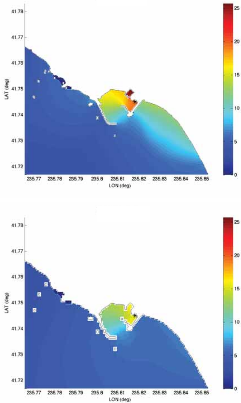
Figure 33: Maximum wave heights (cm) computed with forecast model grids. Asterisk indicates location of the tide gauge (reference model—upper, forecast model—lower) for the 1996 Andreanov event.
