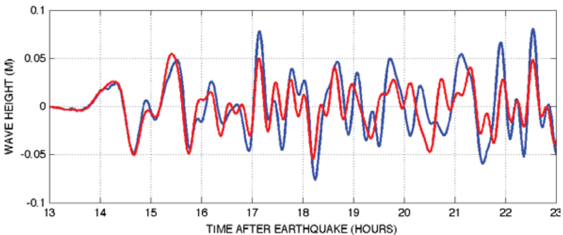
Figure 28: Time series comparison of reference vs. forecast model for the 2007 Solomon event, blue—reference model, red—optimized forecast model.
