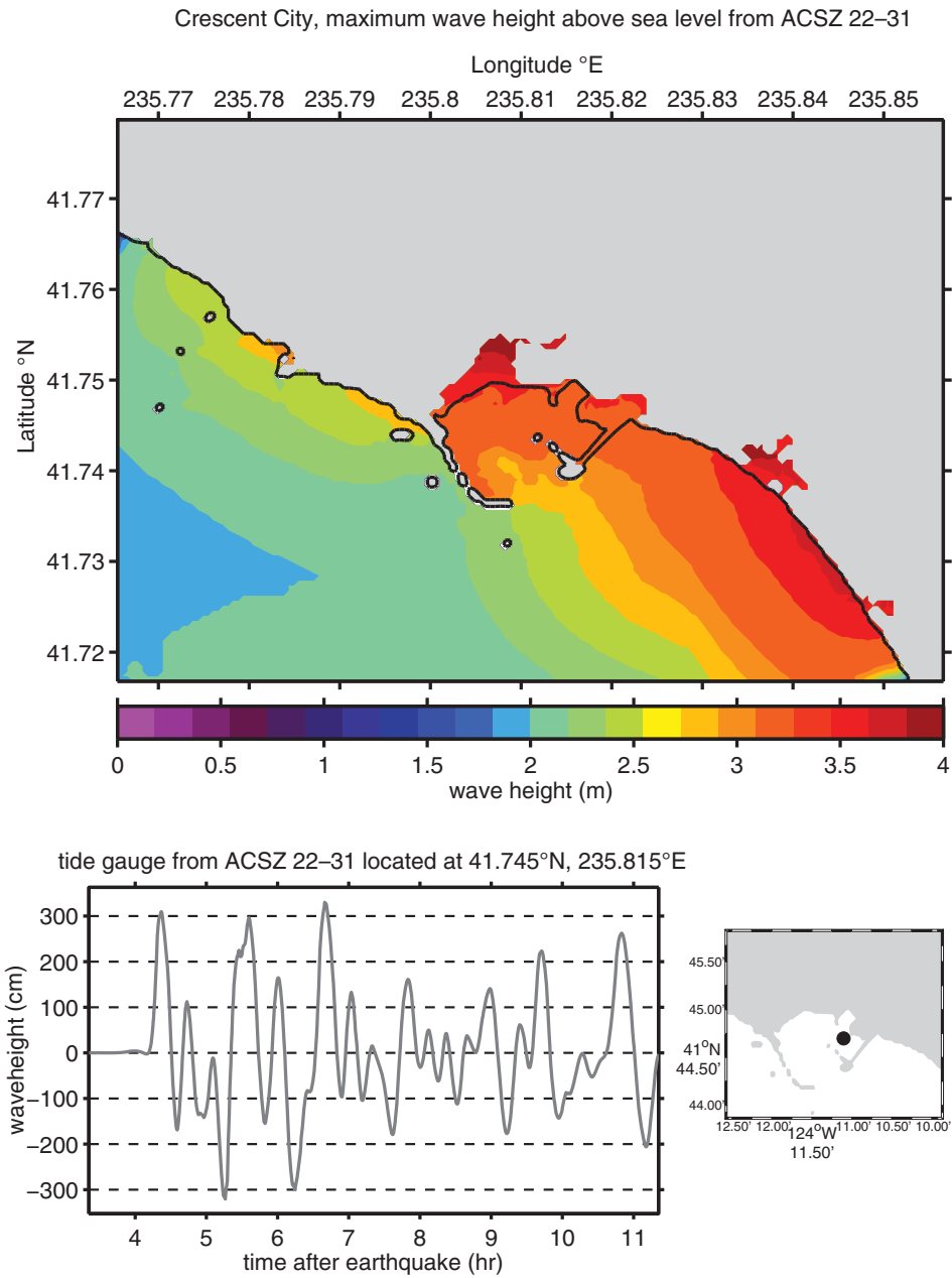
Figure 45: Maximum wave height plot and time series results for the forecast model using synthetic megatunami Event ACSZ 22–31 for Crescent City, California.
