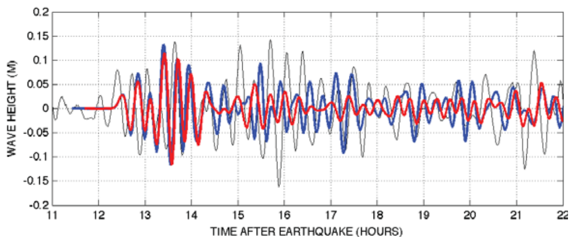
Figure 29: Time series comparison of reference vs. forecast model for the 2007 Peru event, blue—reference model, red—optimized forecast model.
