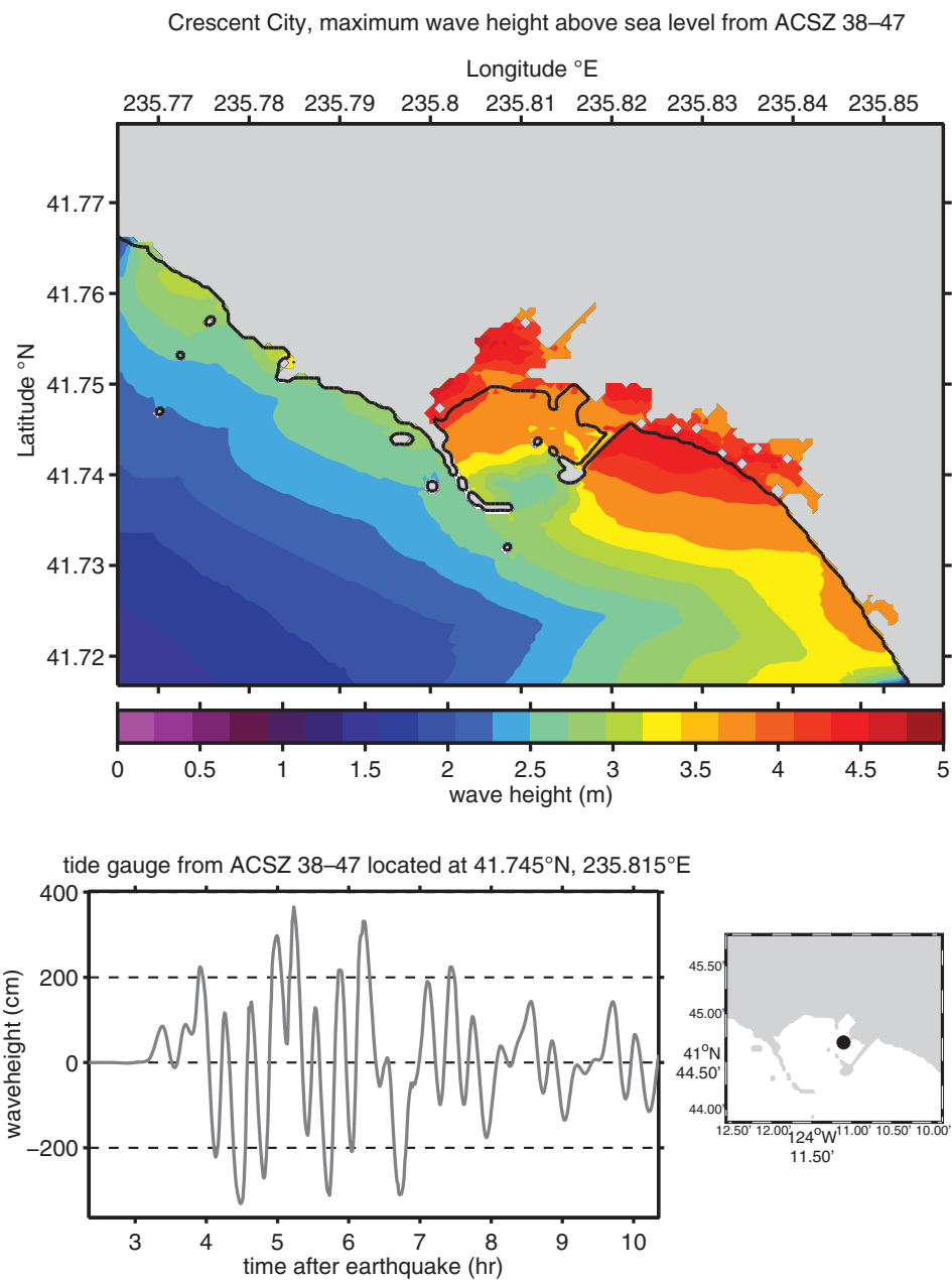
Figure 46: Maximum wave height plot and time series results for the forecast model using synthetic megatunami Event ACSZ 38–47 for Crescent City, California.
