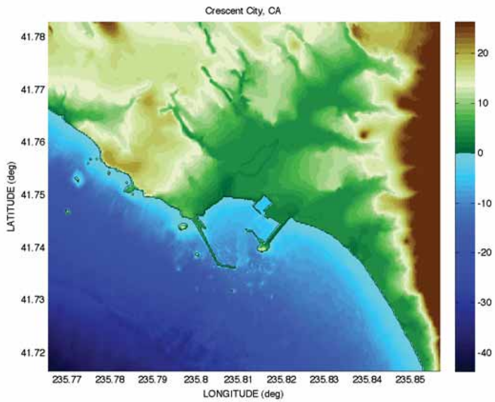
Figure 7: Color-filled surface plot of initial digital elevation model for grid C of the Crescent City, California, forecast model. Color bar units are in meters.
