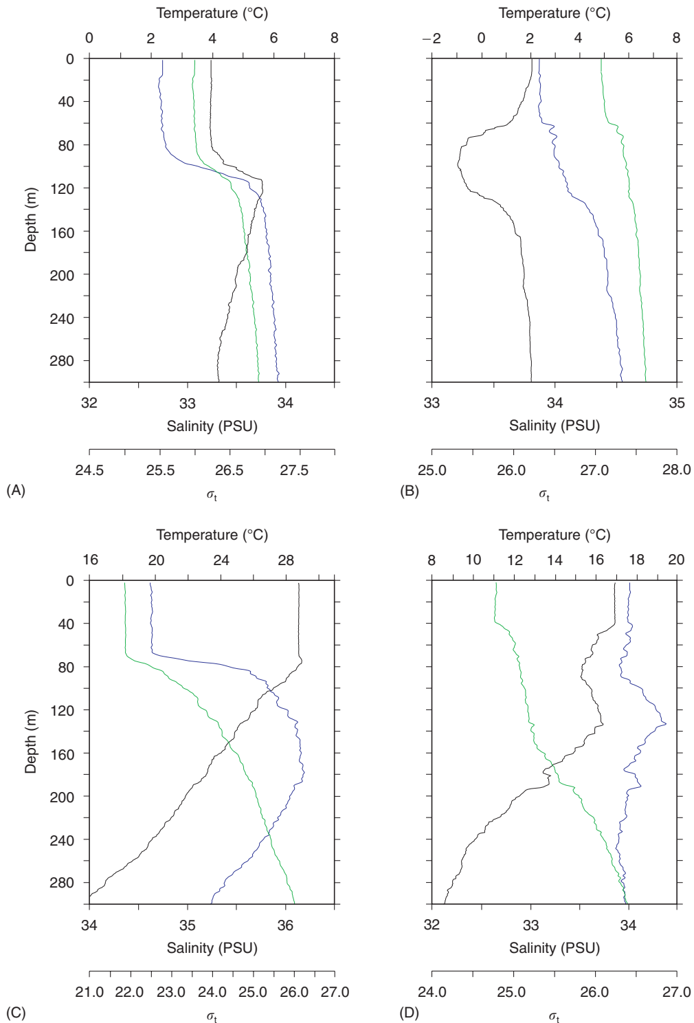
a0149fig0004 Figure 4 Temperature (black line), salinity (blue line) and density ( \sigma_t , green line) from expendable conductivity–temperature–density casts at (A) 58.2°N, 147.3°W in March 1996, (B) 61°S, 63.9°W in January 1997, (C) 11.9°S, 176.1°W in August 1998, and (D) 33.5°N, 134.6°W in May 1995. Note the presence of temperature inversions at the base of the mixed layer in all casts.
