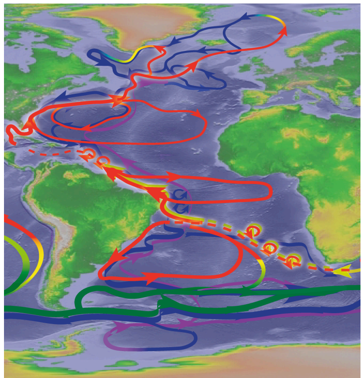
Figure 1 Pathways of the overturning circulation in the Atlantic Ocean that represents the large-scale conversion of surface waters (red arrows) to deep waters (blue arrows in the Southern Ocean; dashed blue line arrows North Atlantic Deep Water) that have global impacts. The Atlantic overturning circulation has many complex and interacting parts (e.g. rings, inter-basin and inter-ocean exchanges) but the most important aspect is the large heat it carries and its apparent sensitivity to the hydrological cycle and climate change (adapted from "Charting the course of the Ocean Science in the United States for the next decade", 2007, to include Antarctic Bottom Water). Graphics: S. Speich adapted from R. Lumpkin NOAA/AOML
