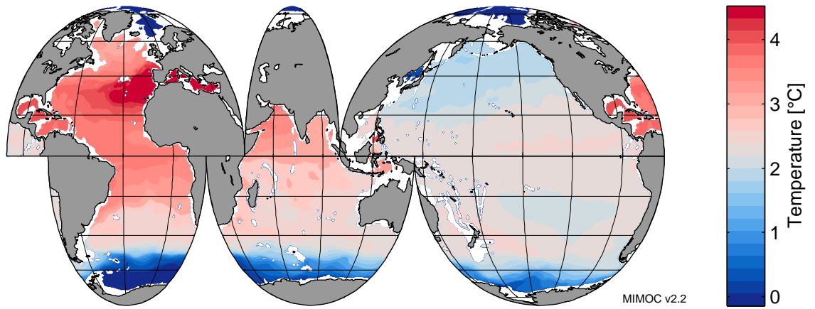
Potential Temperature at 1800 dbar in August
