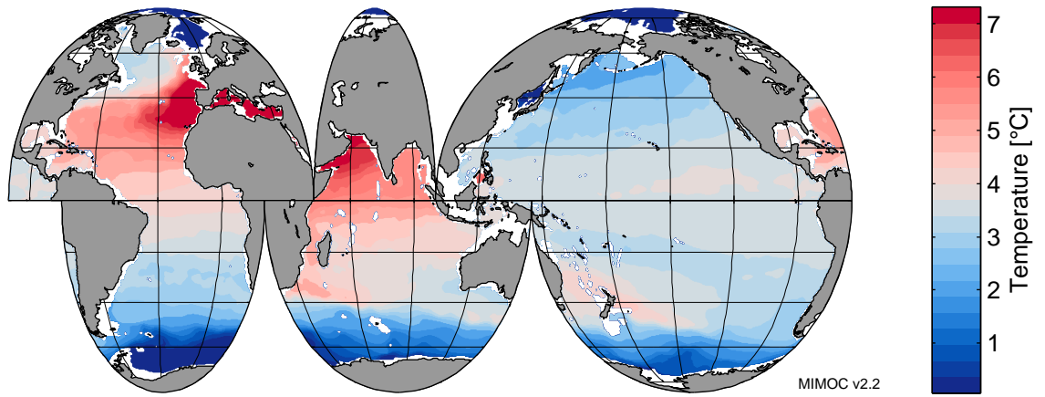
Potential Temperature at 1200 dbar in August
