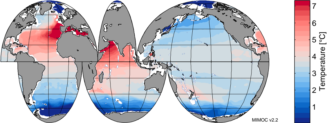
Potential Temperature at 1200 dbar in February
