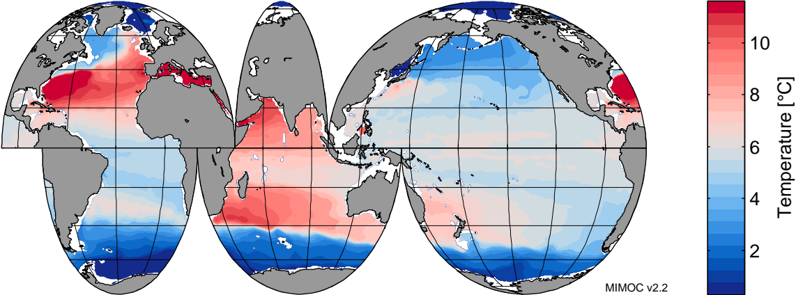
Potential Temperature at 700 dbar in November
