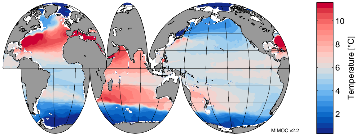
Potential Temperature at 700 dbar in August
