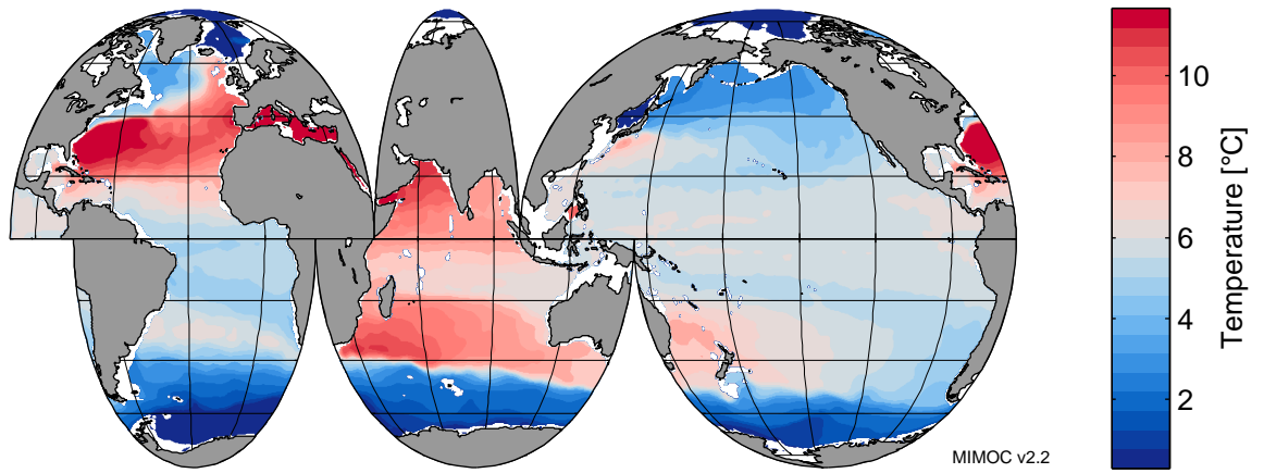
Potential Temperature at 700 dbar in February
