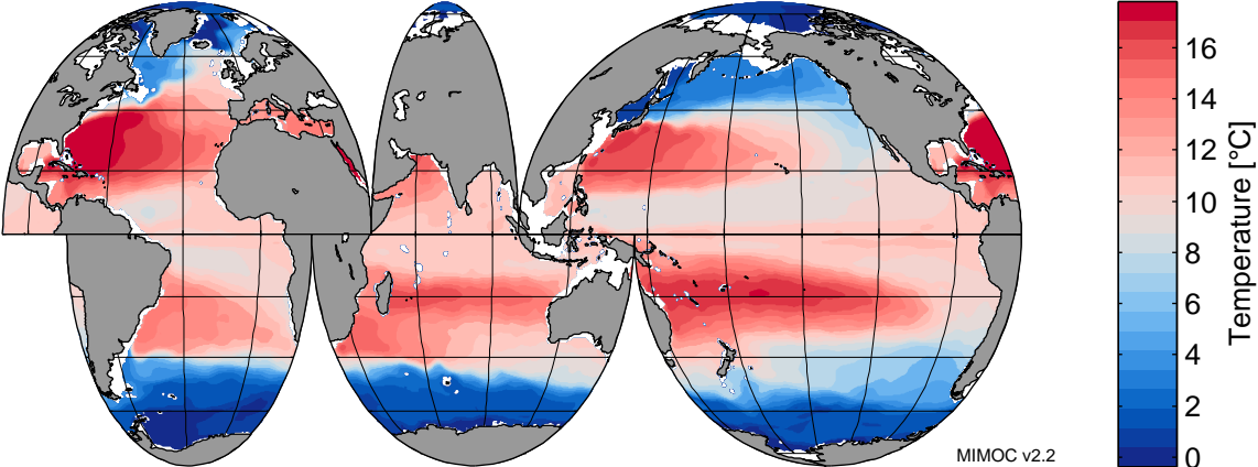
Potential Temperature at 300 dbar in November
