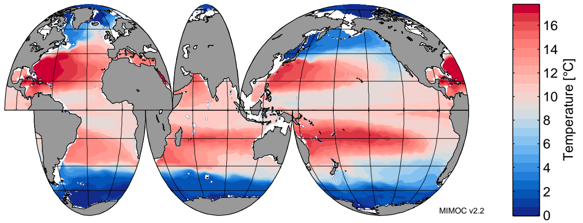
Potential Temperature at 300 dbar in August
