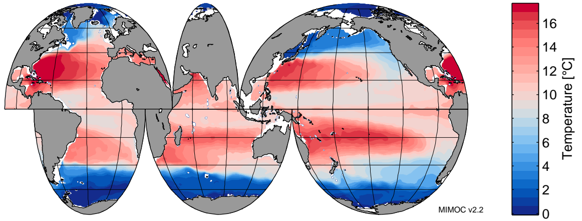
Potential Temperature at 300 dbar in May
