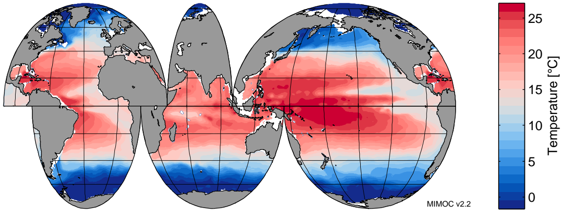
Potential Temperature at 100 dbar in November
