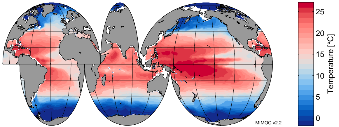
Potential Temperature at 100 dbar in August
