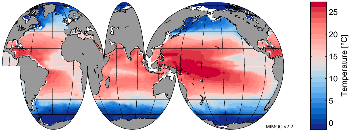
Potential Temperature at 100 dbar in May
