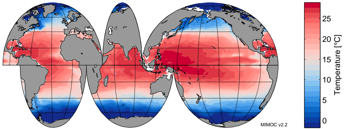
Potential Temperature at 50 dbar in November
