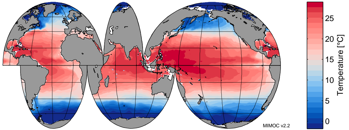
Potential Temperature at 50 dbar in August
