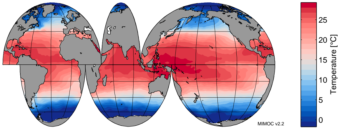
Potential Temperature at 0 dbar in November
