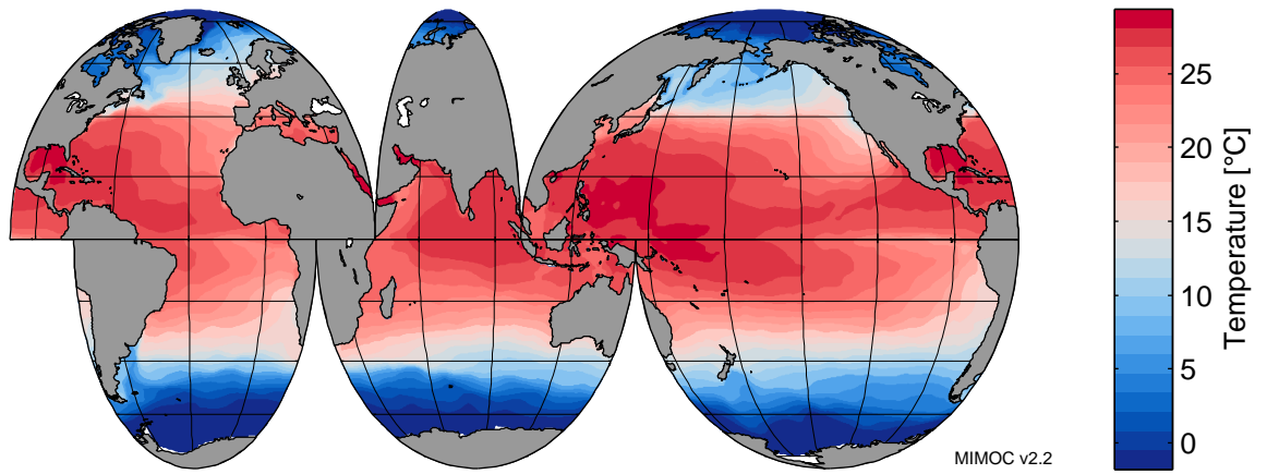
Potential Temperature at 0 dbar in August
