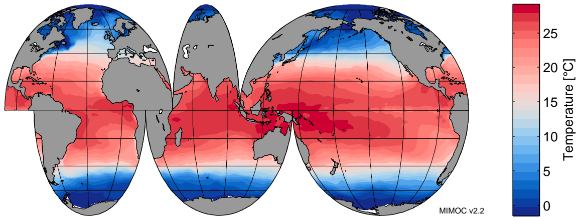
Potential Temperature at 0 dbar in February
