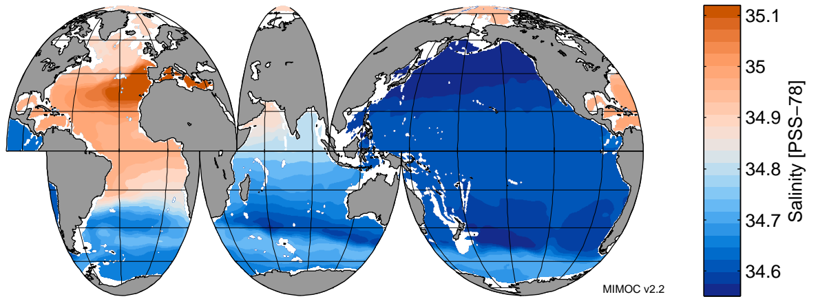
Salinity at 1800 dbar in February
