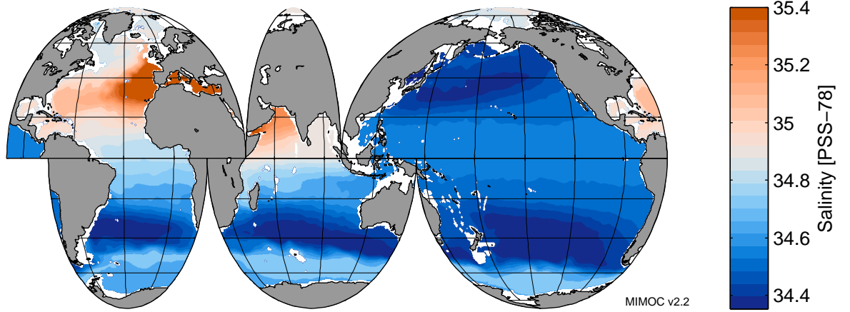
Salinity at 1200 dbar in November
