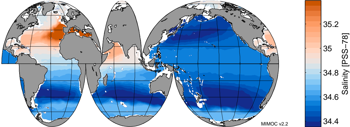
Salinity at 1200 dbar in May
