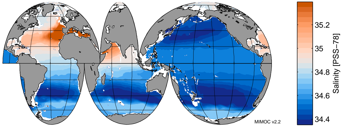
Salinity at 1200 dbar in February
