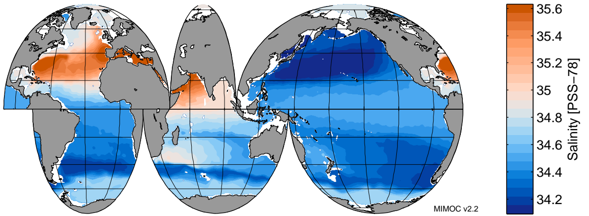
Salinity at 700 dbar in May
