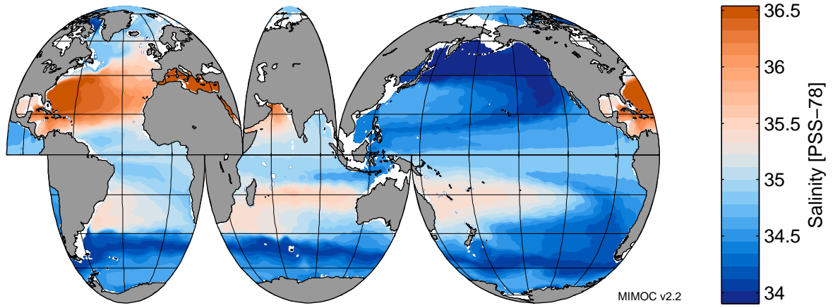
Salinity at 300 dbar in November
