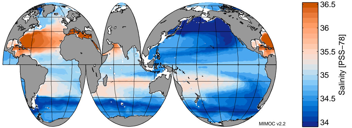
Salinity at 300 dbar in August
