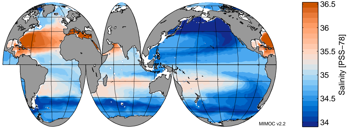
Salinity at 300 dbar in February
