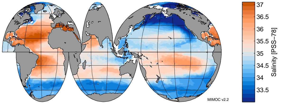
Salinity at 100 dbar in May
