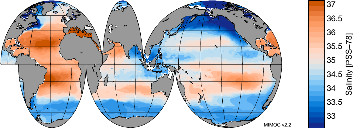
Salinity at 50 dbar in May
