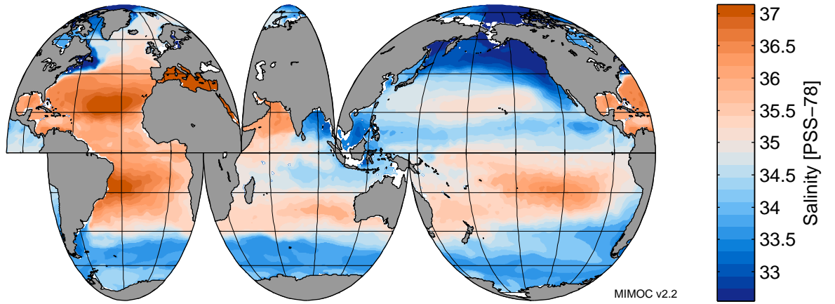
Salinity at 50 dbar in February
