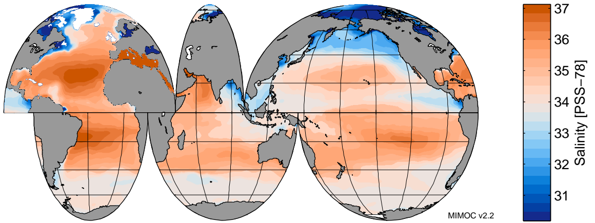
Salinity at 0 dbar in August
