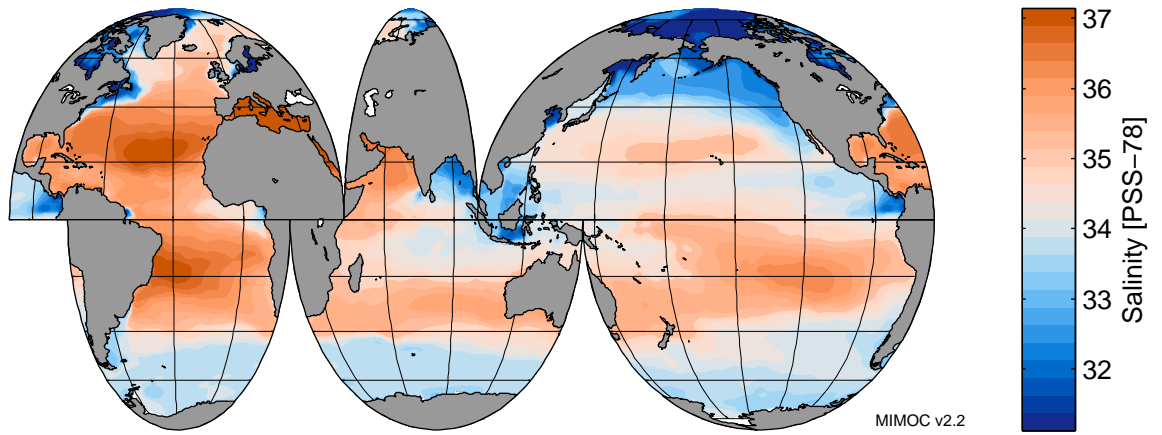
Salinity at 0 dbar in February
