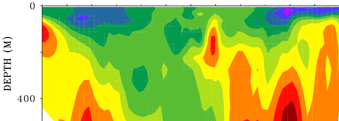
(c) Model - Levitus
