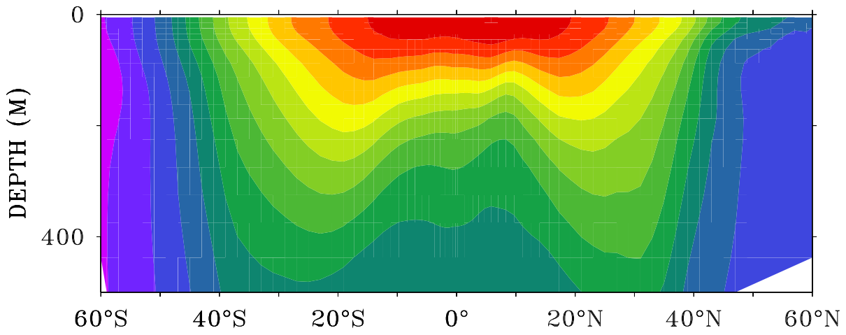
(b) Temp, Model
