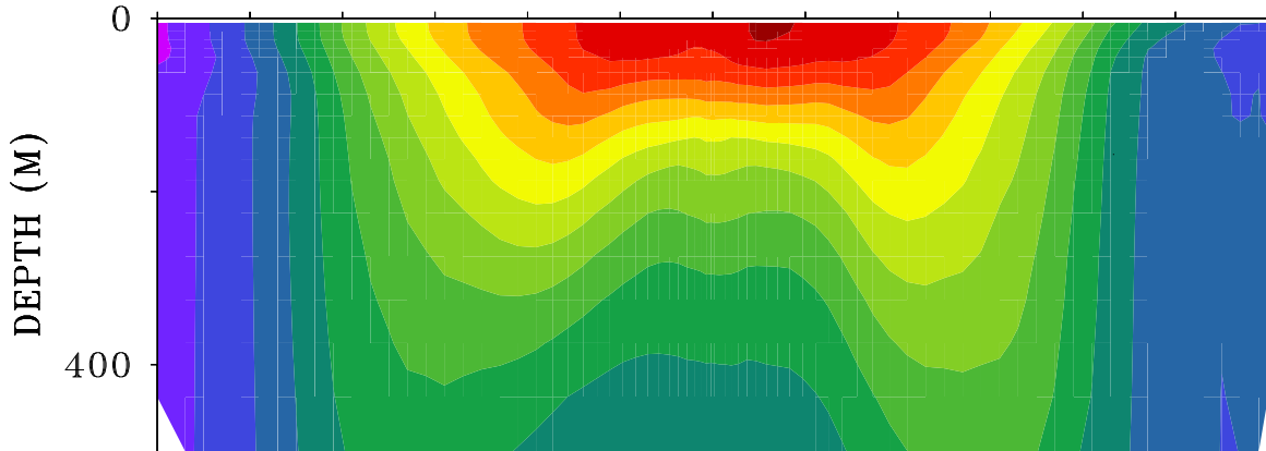
(b) Temp, Model
