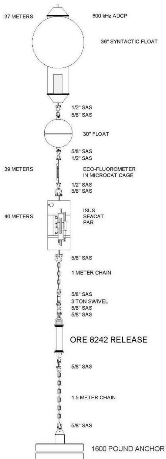
Figure A 4.2. Mooring design for 16CKP moorings. In addition to the 600 kHz ADCP (currents), this mooring contains instruments to measure nitrate (ISUS), temperature and salinity (Seacat), fluorescence (EcoFluorometer) and Photosynthetically Active Radiation (PAR).
