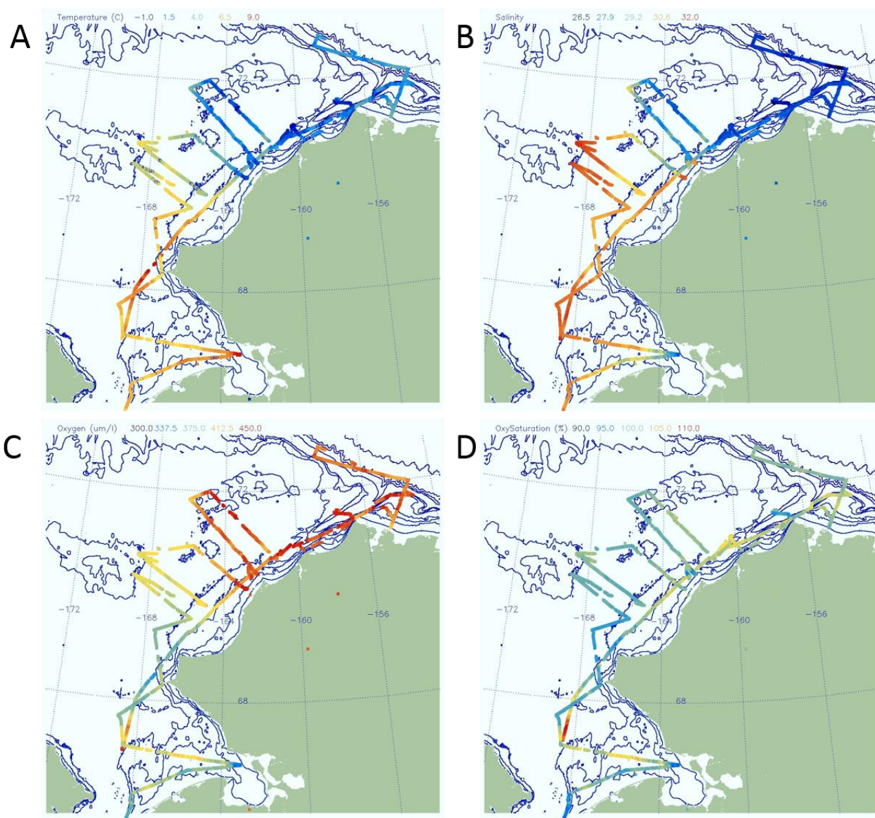
Figure 20. Data obtained from the underway sampling system. A) Temperature (°C); B) Salinity (psu); C) Oxygen (µm/l); D) Oxygen saturation (%). Plots made from raw data.
