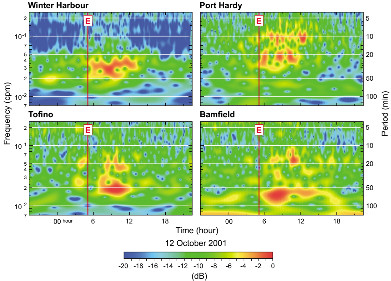
Fig. 3 Frequency-time ( f-t ) diagrams for the 12 October 2001 QCI tsunami for the Winter Harbour, Port Hardy, Tofino and Bamfield tide gauge records. The vertical line (E) indicates the time of the main earthquake shock.
