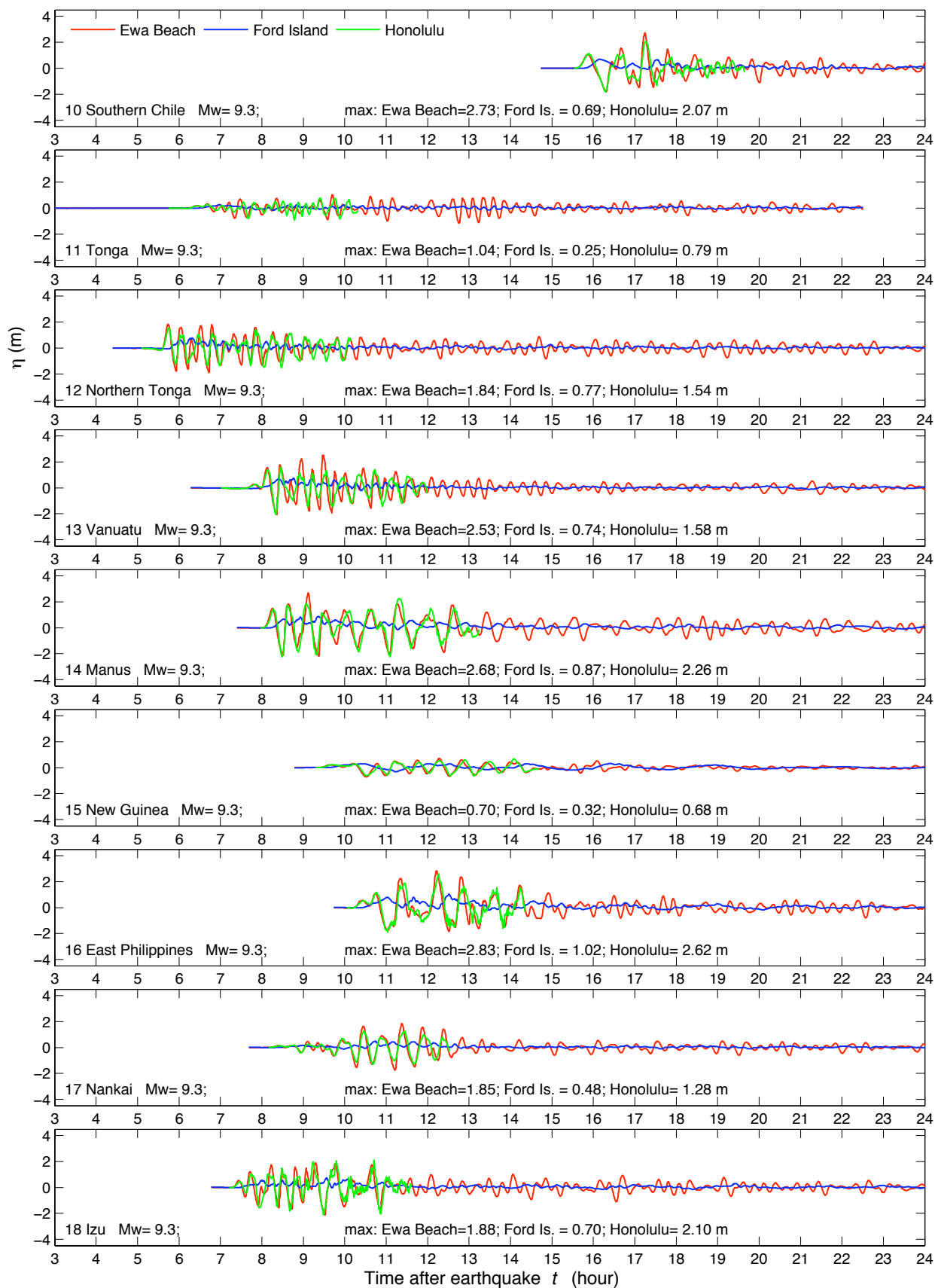
Figure 19 Modeled time series of sea surface elevation \eta at Ewa Beach and Ford Island warning points, and Honolulu tide gage for the eighteen simulated magnitude 9.3 tsunamis.
