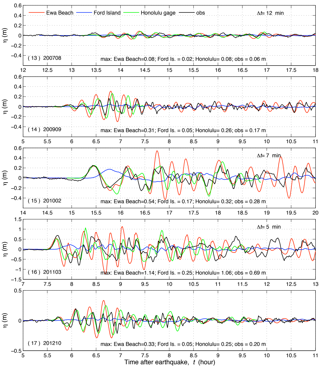
Figure 18 Modeled time series of sea surface elevation \eta at Ewa Beach and Ford Island warning points, and Honolulu tide gage for the past tsunamis.
