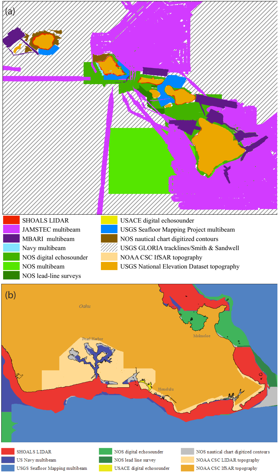
Figure 7 Bathymetric and topographic data source overview. (a) 6'' sec (~180m) Hawaii DEM and (b) 1/3'' (~10m) South Oahu DEM developed at PMEL/NCTR.
