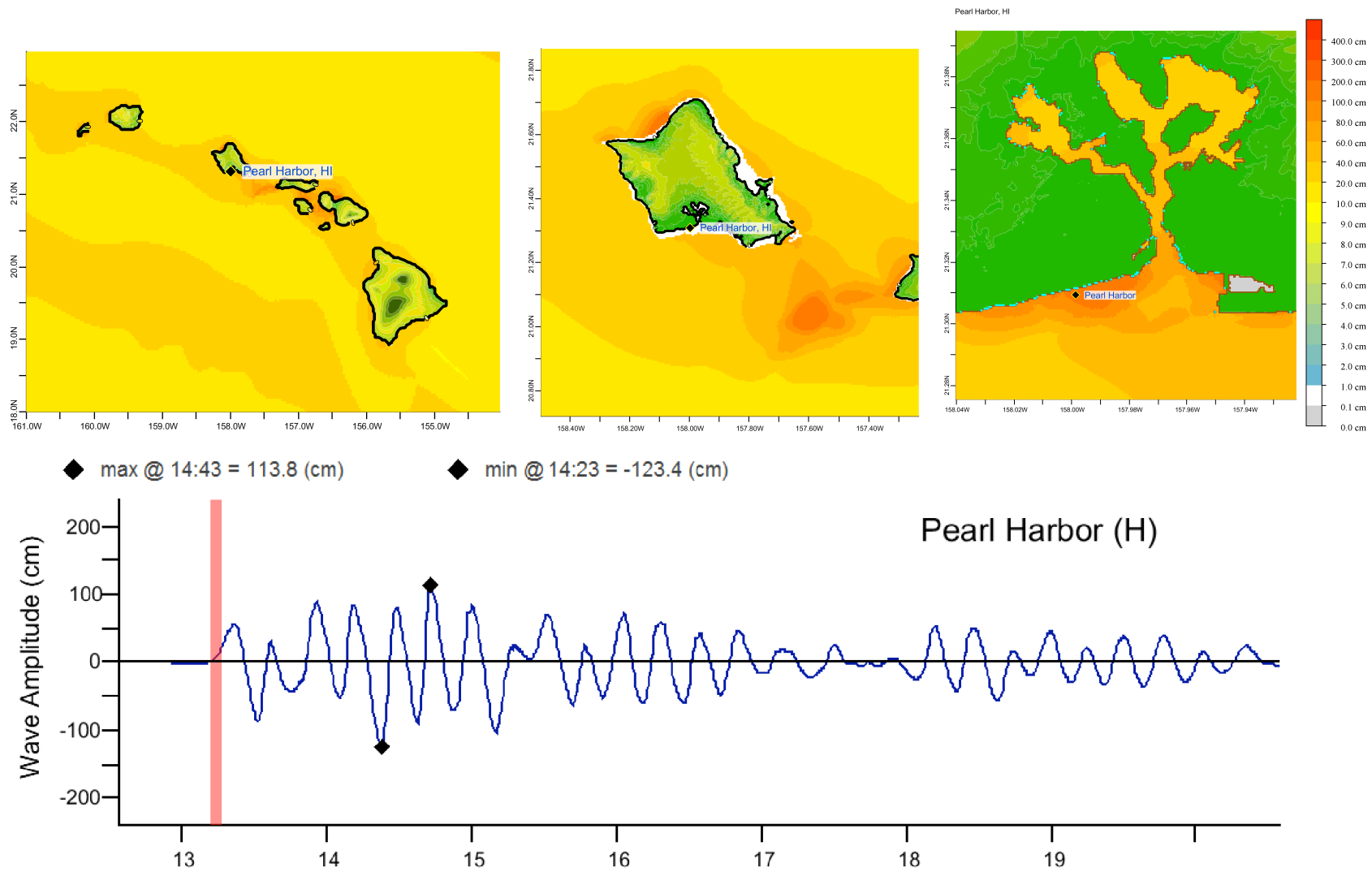
Figure C5 Response of the Pearl Harbor forecast model to the 2011 Tohoku tsunami. Maximum sea surface elevation for (a) A-grid, b) B-grid, c) C-grid. Sea surface elevation time series at the C-grid warning point (d).
