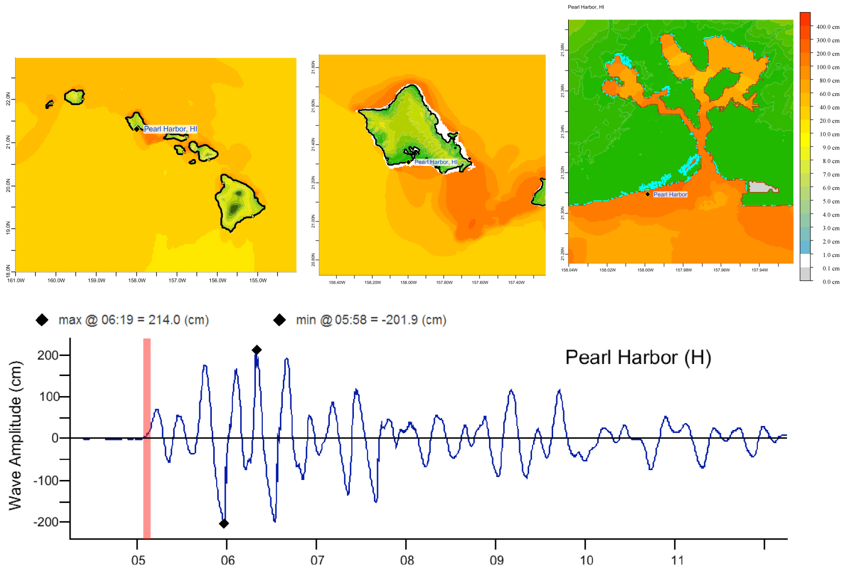
Figure C2 Response of the Pearl Harbor forecast model to synthetic scenario ACSZ 56-65 ( \alpha=29 ). Maximum sea surface elevation for (a) A-grid, b) B-grid, c) C-grid. Sea surface elevation time series at the C-grid warning point (d). ).
