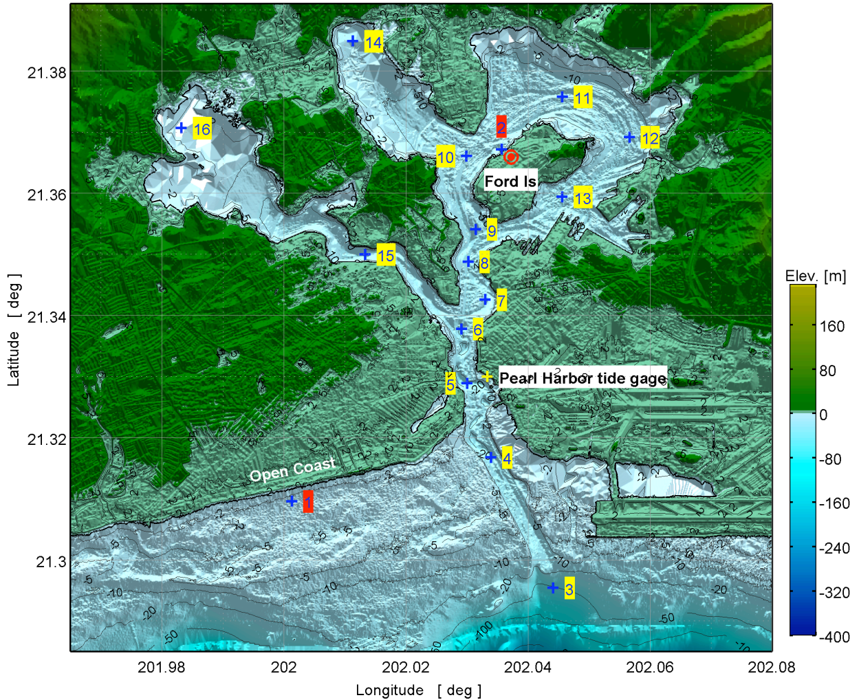
Figure 10 Location of Ewa Beach and Ford Island warnig points, Pearl Harbor tide gage and virtual gages in Pearl Harbor (Tang et al., 2006).
