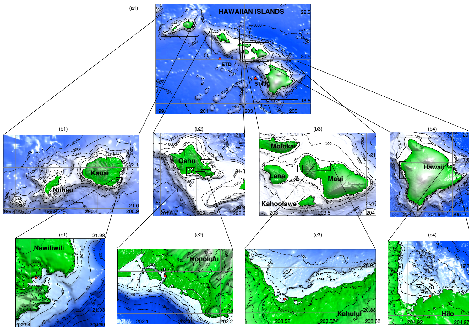
Figure 2 Forecast model setups for 13 forecast sites in Hawaii: (a) 2-arc-min ( \sim 3600\text{m} ) regional, (b) 12-18-arc-sec ( \sim 360\text{-}540\text{m} ) intermediate and (c) 2-arc-sec ( \sim 60\text{m} ) nearshore grids for Nawiliwili, Honolulu, Kahului and Hilo. Red dots, coastal tide stations.
