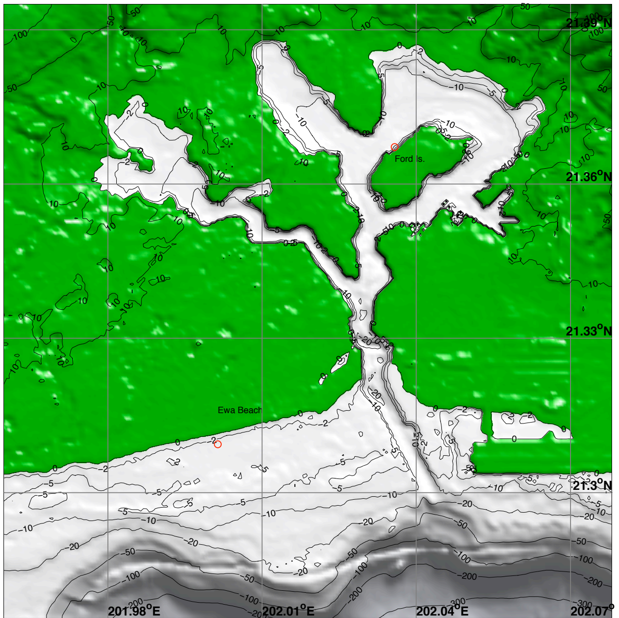
Figure 9 Grid setup of the Pearl Harbor forecast model with resolutions of (a) 120" (3600m), (b) 18" (540m) and (c) 2" (60m). \square , nested grid boundary; \circ , warning points near Ewa Beach and Ford Island.
