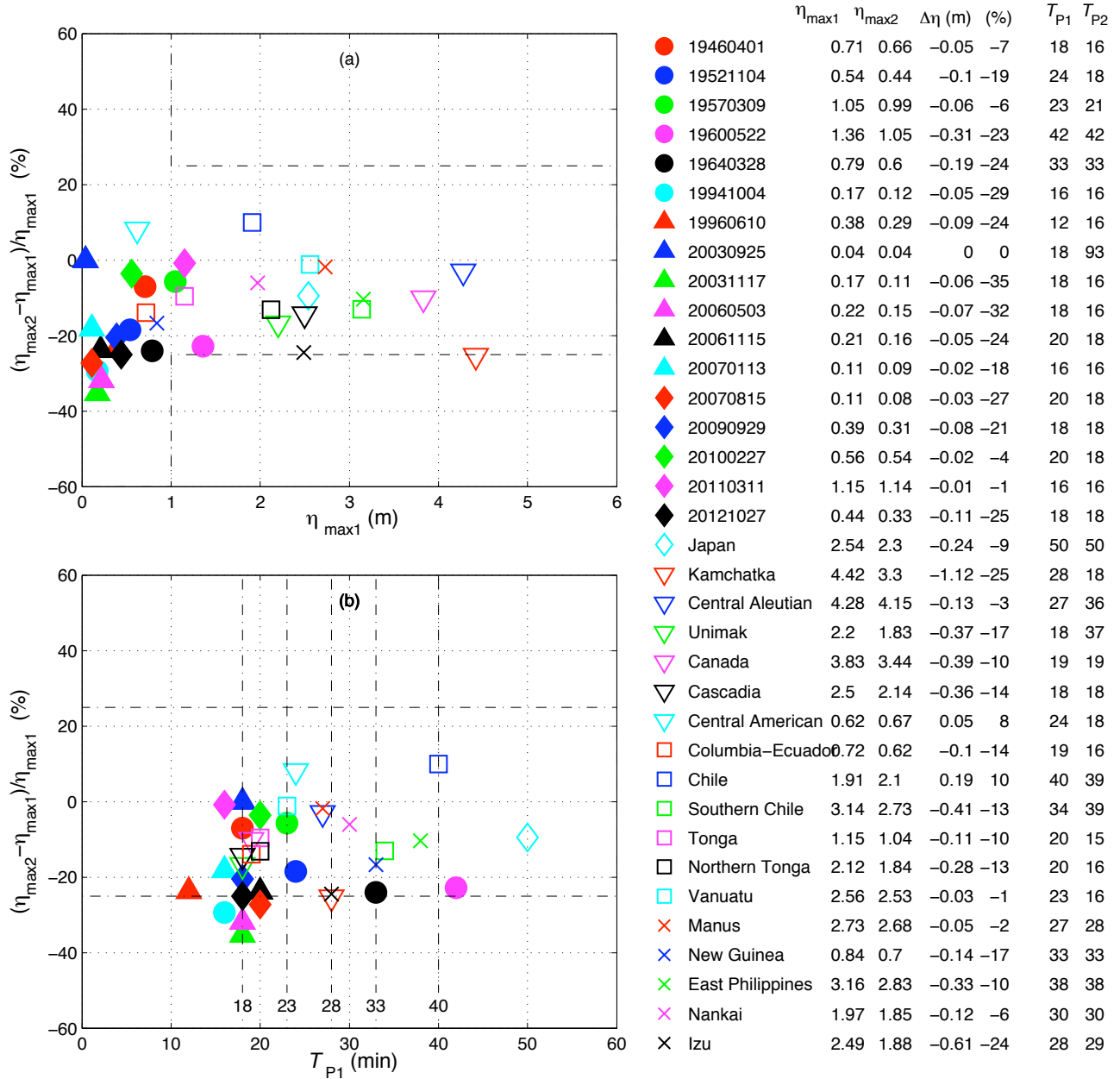
Figure 17 (a) Uncertainty in the computed \eta_{\max} at Ewa Beach warning point. When \eta_{\max 1} > 1.0\text{m} , the uncertainty is within 25%. (b) Uncertainty v.s. peak period. Filled markers, 17 past tsunamis; open markers, 18 simulated M_w = 9.3 tsunamis. \eta_{\max 1} and \eta_{\max 2} are the maximum water elevation at the Ewa Beach warning point computed by reference and forecast model respectively.
