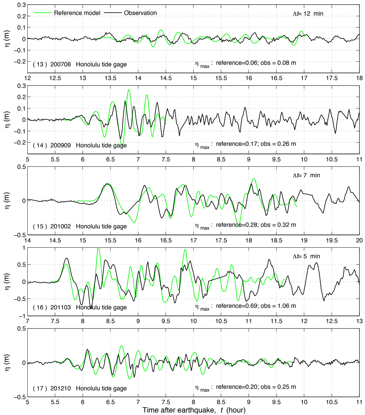
Figure 12 Modeled and measured time series of sea surface elevation \eta at Honolulu tide gage for past tsunamis. Model results were computed from the Pearl Harbor reference model. Modeled time series was shifted \Delta t min behind.
