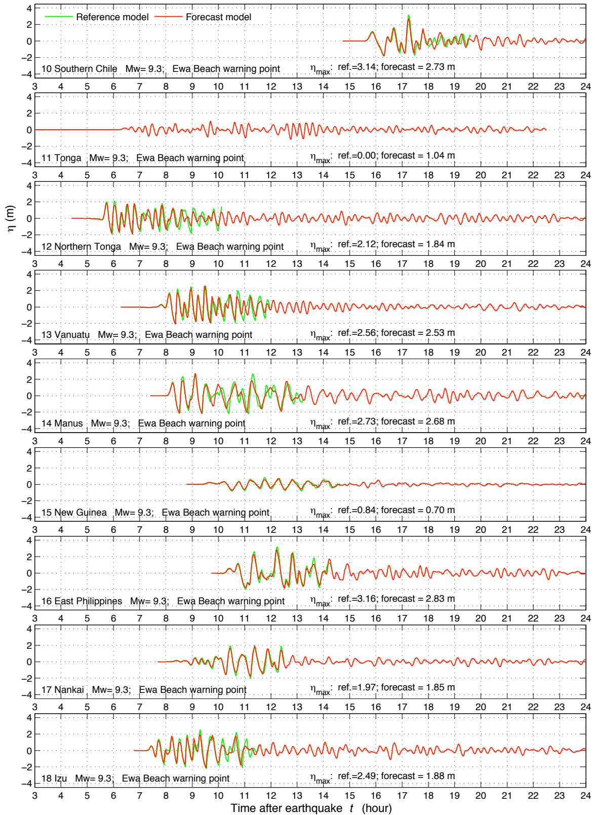
Figure 14 Modeled time series of sea surface elevation \eta at Ewa Beach warning point for the eighteen simulated magnitude 9.3 tsunamis.
