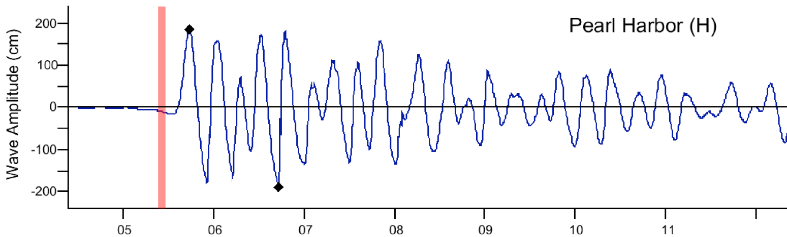
Figure C4 Response of the Pearl Harbor forecast model to synthetic scenario NTSZ 30-39 ( \alpha=29 ). Maximum sea surface elevation for (a) A-grid, b) B-grid, c) C-grid. Sea surface elevation time series at the C-grid warning point (d).
