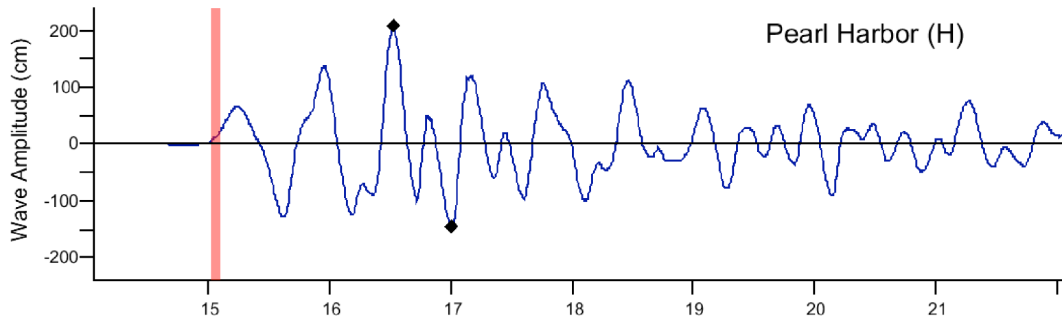
Figure C3 Response of the Pearl Harbor forecast model to synthetic scenario CSSZ 86-95 ( \alpha=29 ). Maximum sea surface elevation for (a) A-grid, b) B-grid, c) C-grid. Sea surface elevation time series at the C-grid warning point (d).
