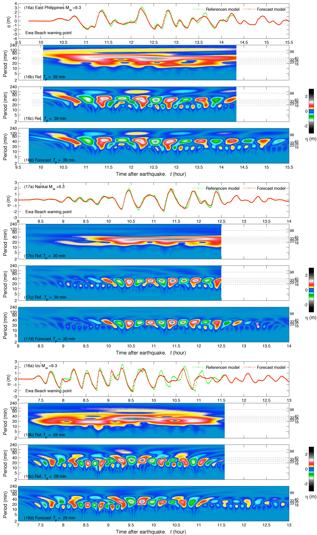
Figure 16 (a) Modeled \eta time series at Ewa Beach warning point for the 18 simulated M_w=9.3 tsunamis.
