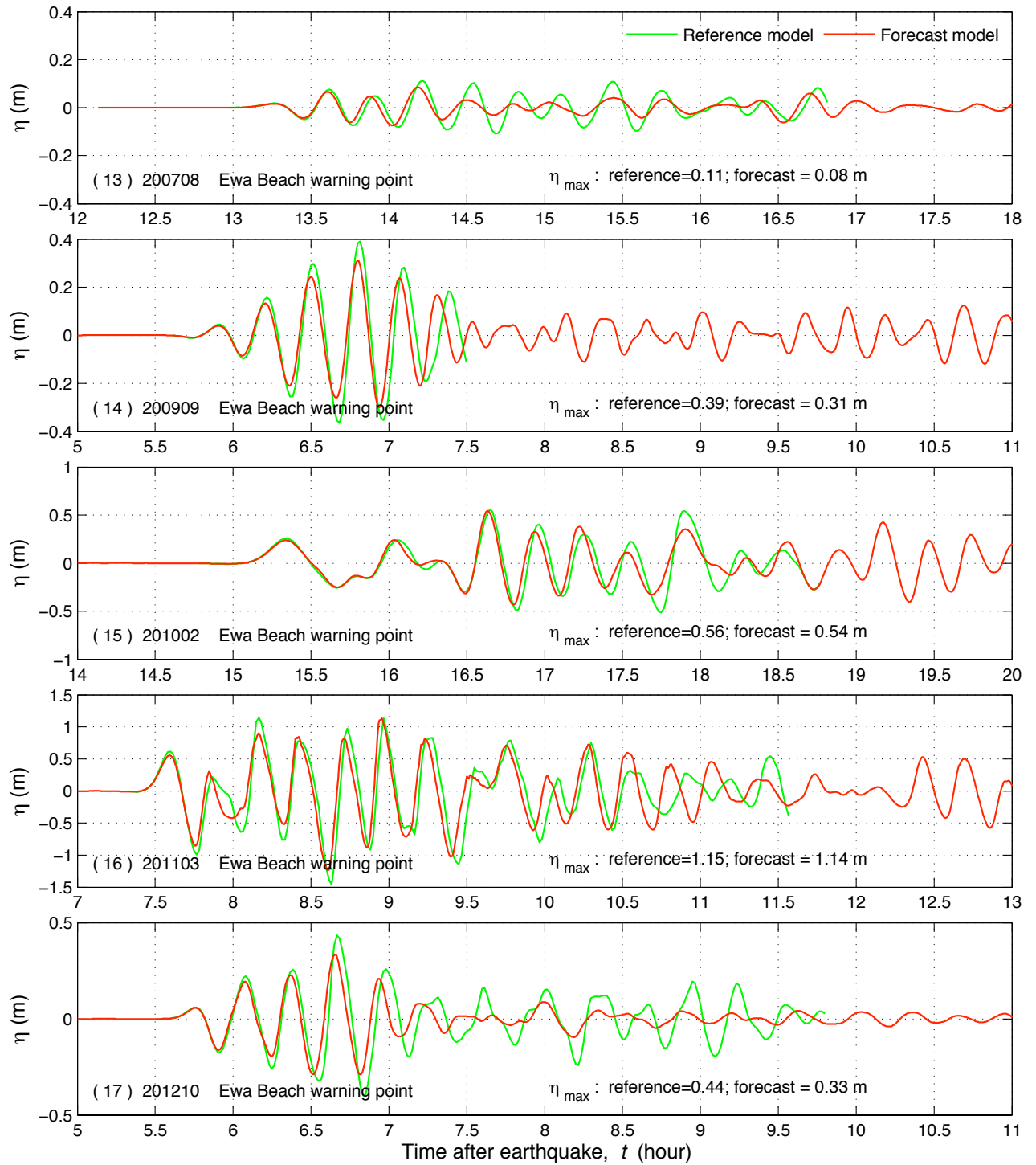
Figure 13 Modeled time series of sea surface elevation \eta at Ewa Beach warning point for the past tsunamis.
