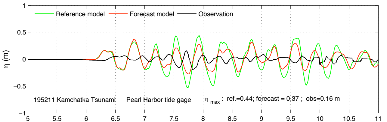
Figure 11 Modeled and measured time series of sea surface elevation \eta at Pearl Harbor tide gage for the 1952 Kamchatka tsunami.
