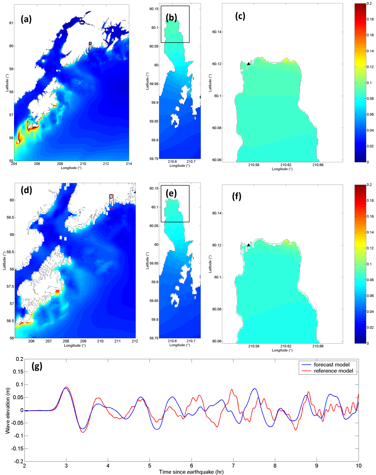
Figure 5: Model results for the 1946 Unimak event: maximum water surface elevations (m) in reference model A- (a), B- (b), and C-grids (c), in forecast model A- (d), B- (e), and C-grids (f), and time-series of water surface elevations at the tide gage (indicated as black triangles in C-grids).
