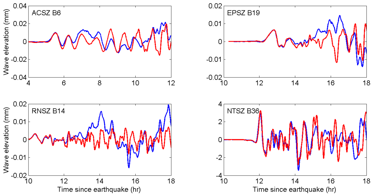
Figure 22: Time-series of water surface elevations at the tide gage in micro-tsunami and Mw 7.5 scenarios computed with reference model (red) and forecast model (blue), respectively.
