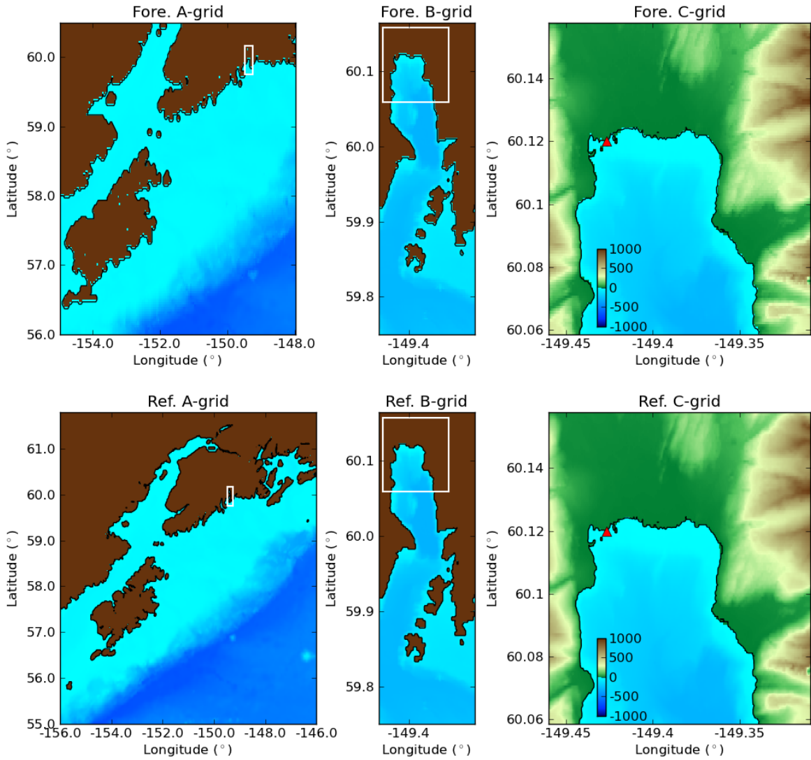
Figure 2: Computational grids in the Seward forecast and reference models. Topography in A- and B-grids is not presented. Location of the tide gauge is indicated as a red triangle in C-grids.
