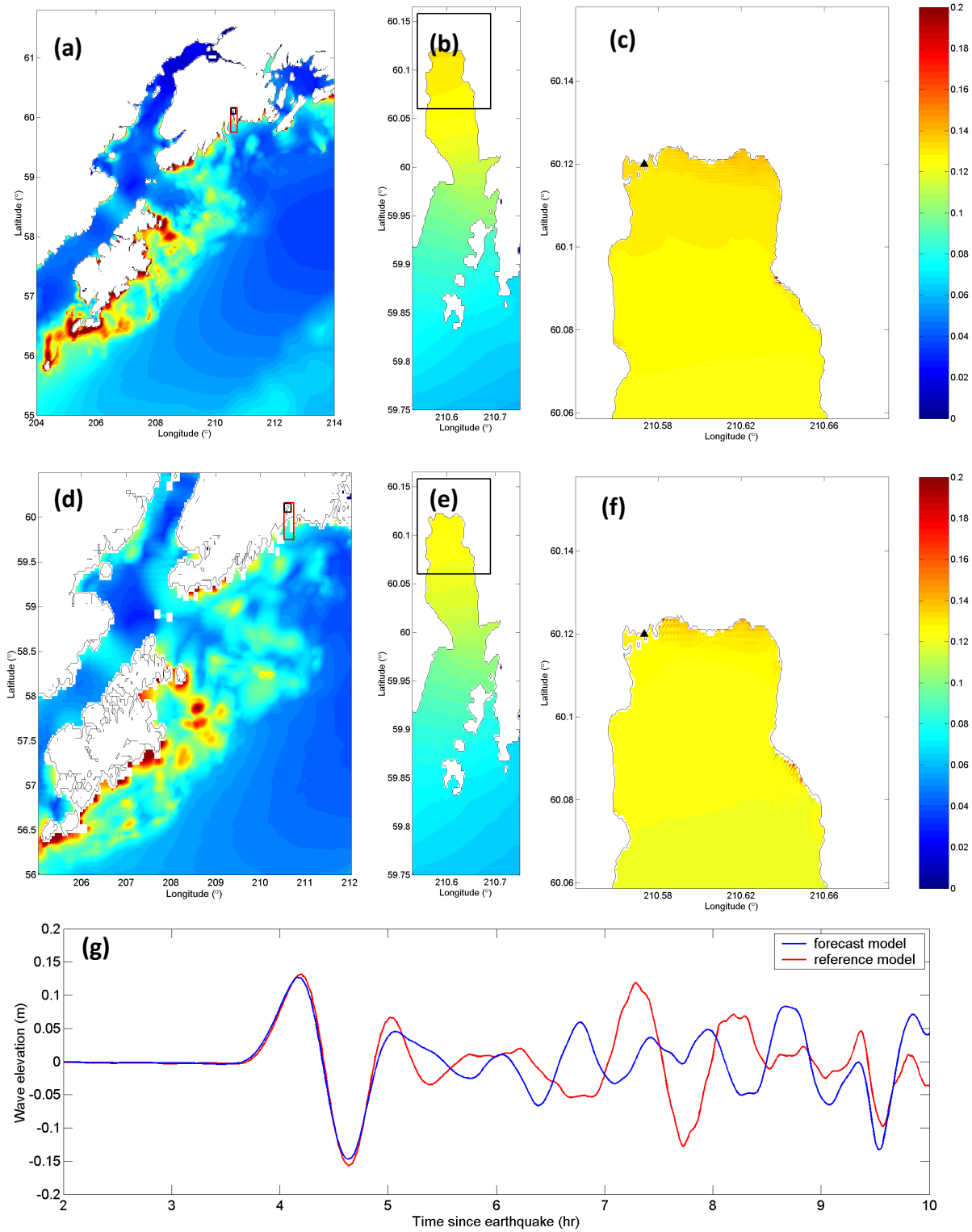
Figure 6: Model results for the 1957 Andreanov event: maximum water surface elevations (m) in reference model A- (a), B- (b), and C-grids (c), in forecast model A- (d), B- (e), and C-grids (f), and time-series of water surface elevations at the tide gage (indicated as black triangles in C-grids).
