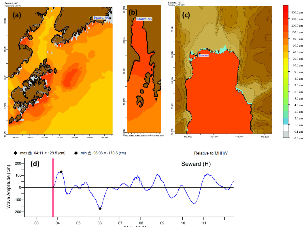
Figure C2: Response of the Seward forecast model to synthetic scenario ACSZ 56-65 ( \alpha=30 ). Maximum sea surface elevation for (a) A-grid, (b) B-grid, (c) C-grid. Sea surface elevation time series at the C-grid warning point (d).
