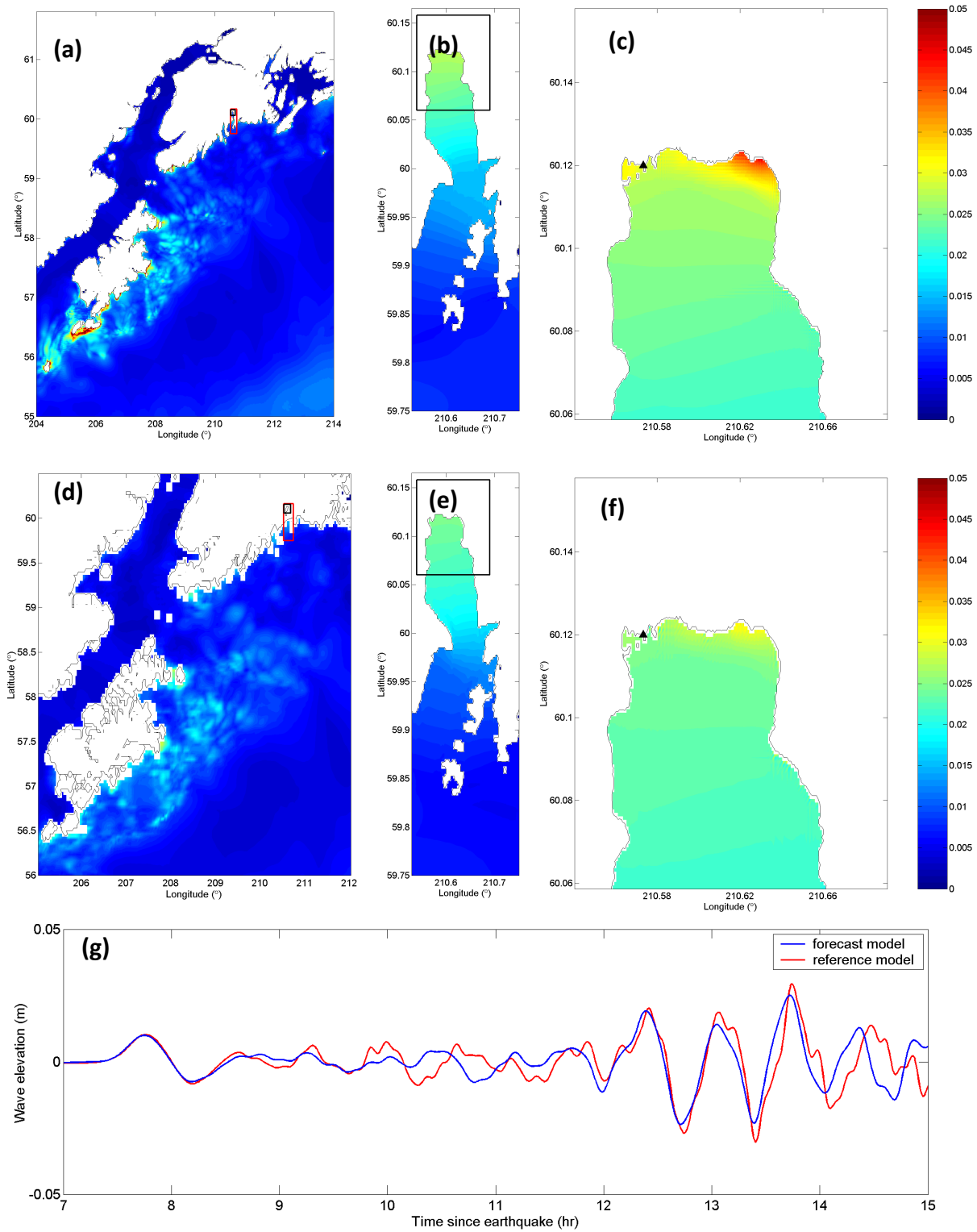
Figure 7: Model results for the 1994 Kuril Islands event: maximum water surface elevations (m) in reference model A- (a), B- (b), and C-grids (c), in forecast model A- (d), B- (e), and C-grids (f), and time-series of water surface elevations at the tide gage (indicated as black triangles in C-grids).
