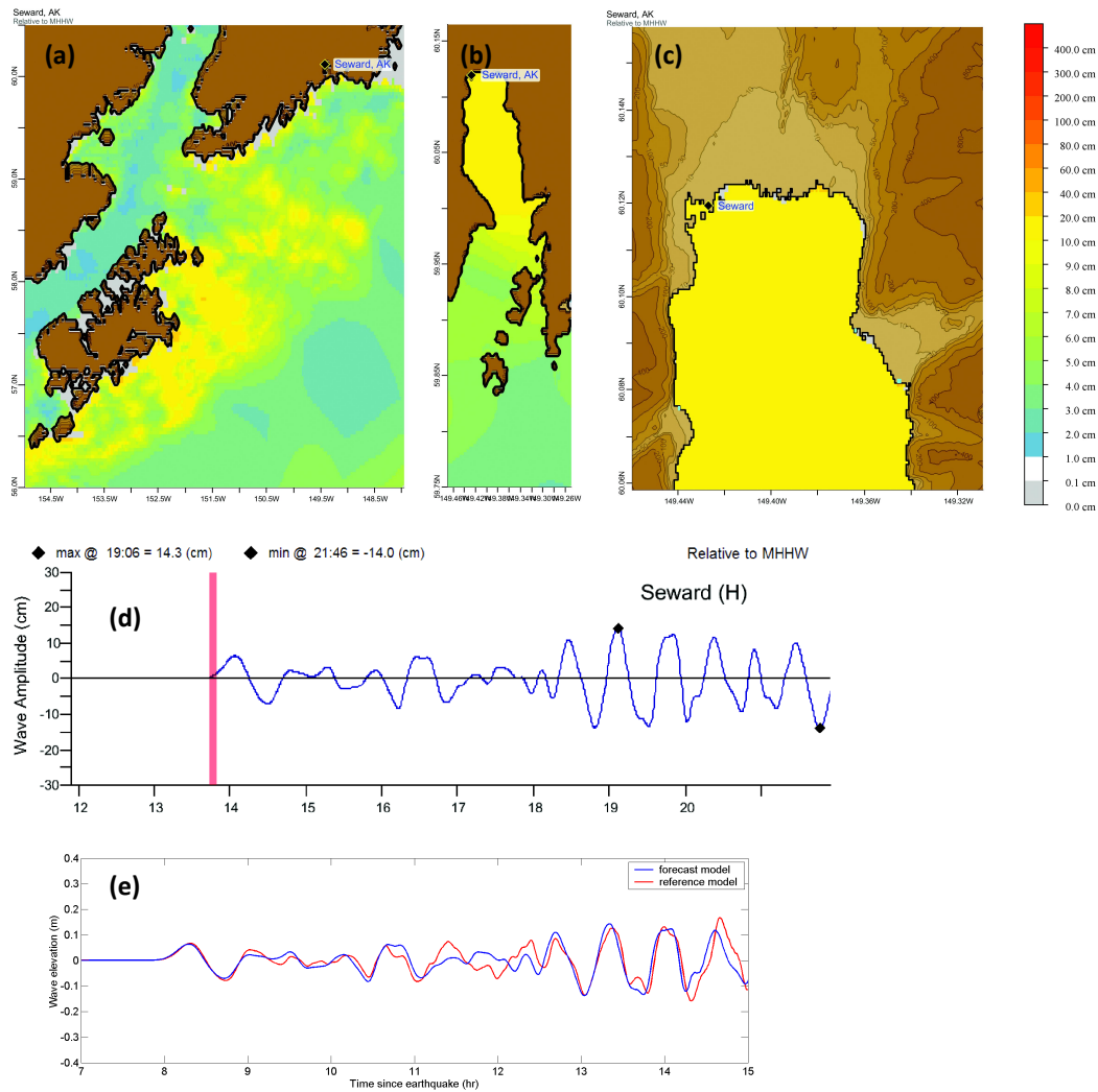
Figure C5: Response of the Seward forecast model to the 2006 Tonga tsunami. Maximum sea surface elevation for (a) A-grid, (b) B-grid, (c) C-grid. Sea surface elevation time series at the C-grid warning point (d). The lower time series plot (e) is the result obtained during model development and is shown for comparison with test results.
