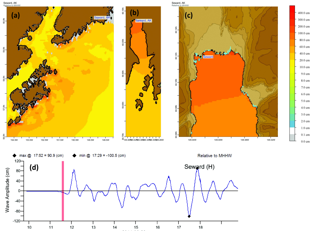
Figure C4: Response of the Seward forecast model to synthetic scenario NTSZ 30-39 ( \alpha=30 ). Maximum sea surface elevation for (a) A-grid, (b) B-grid, (c) C-grid. Sea surface elevation time series at the C-grid warning point (d).
