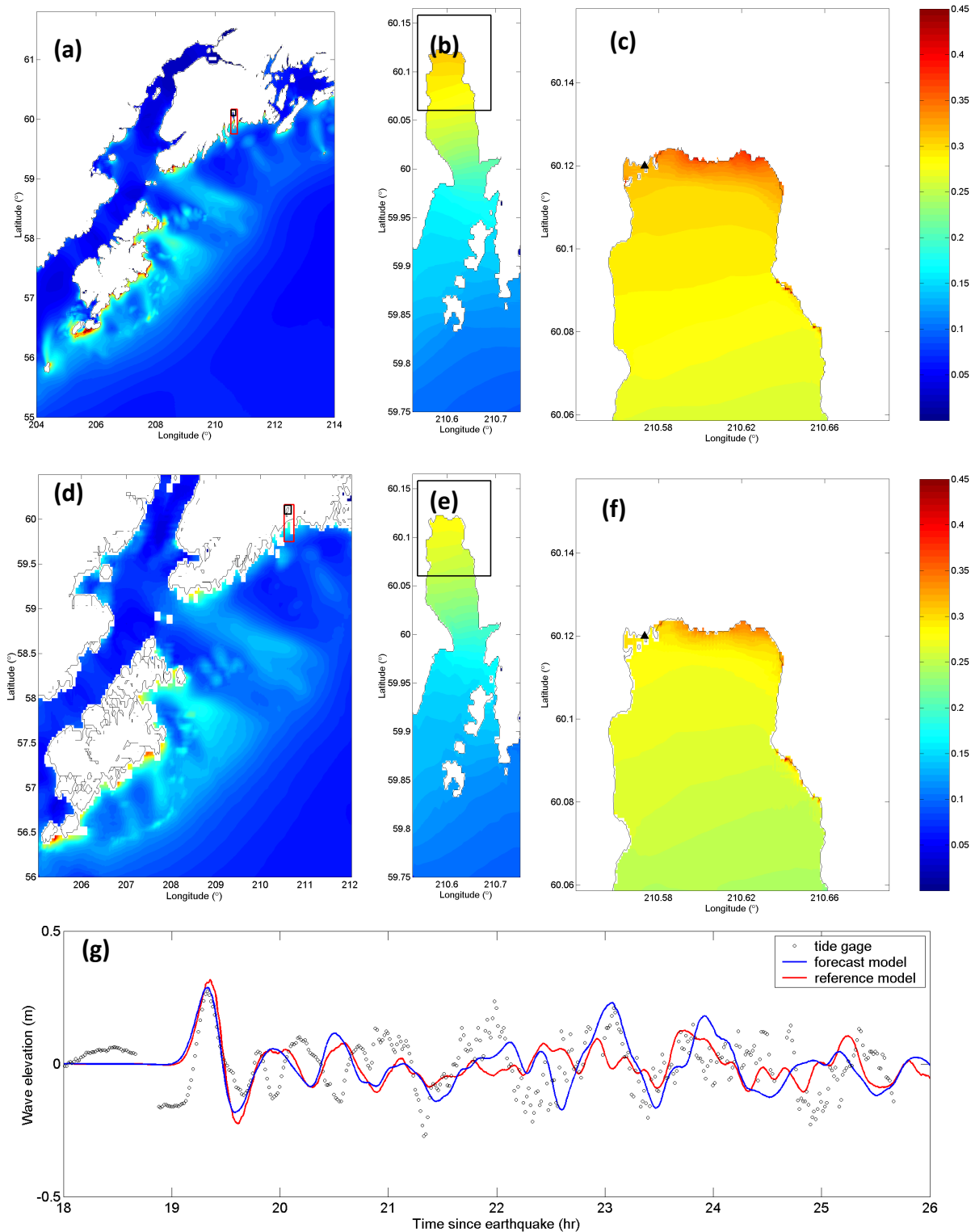
Figure 13: Model results for the 2010 Chile event: maximum water surface elevations (m) in reference model A- (a), B- (b), and C-grids (c), in forecast model A- (d), B- (e), and C-grids (f), and time-series of water surface elevations at the tide gage (indicated as black triangles in C-grids). Computed time-series are shifted +8 minutes for better agreement in (g).
