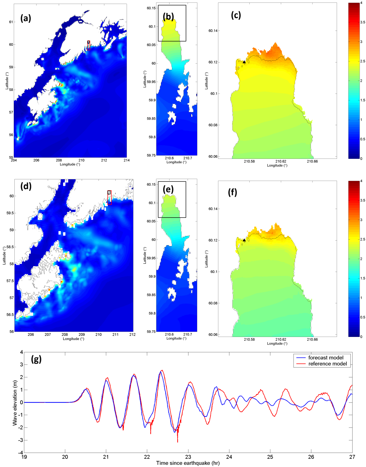
Figure 18: Model results for synthetic scenario of CSSZ 102-111: maximum water surface elevations (m) in reference model A- (a), B- (b), and C-grids (c), in forecast model A- (d), B- (e), and C-grids (f), and time-series of water surface elevations at the tide gage (indicated as black triangles in C-grids).
