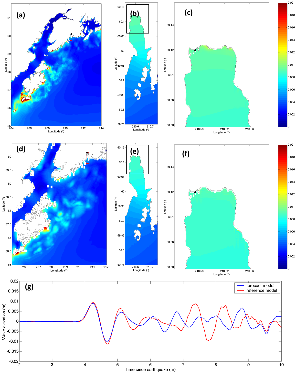
Figure 8: Model results for the 1996 Andreanov event: maximum water surface elevations (m) in reference model A- (a), B- (b), and C-grids (c), in forecast model A- (d), B- (e), and C-grids (f), and time-series of water surface elevations at the tide gage (indicated as black triangles in C-grids).
