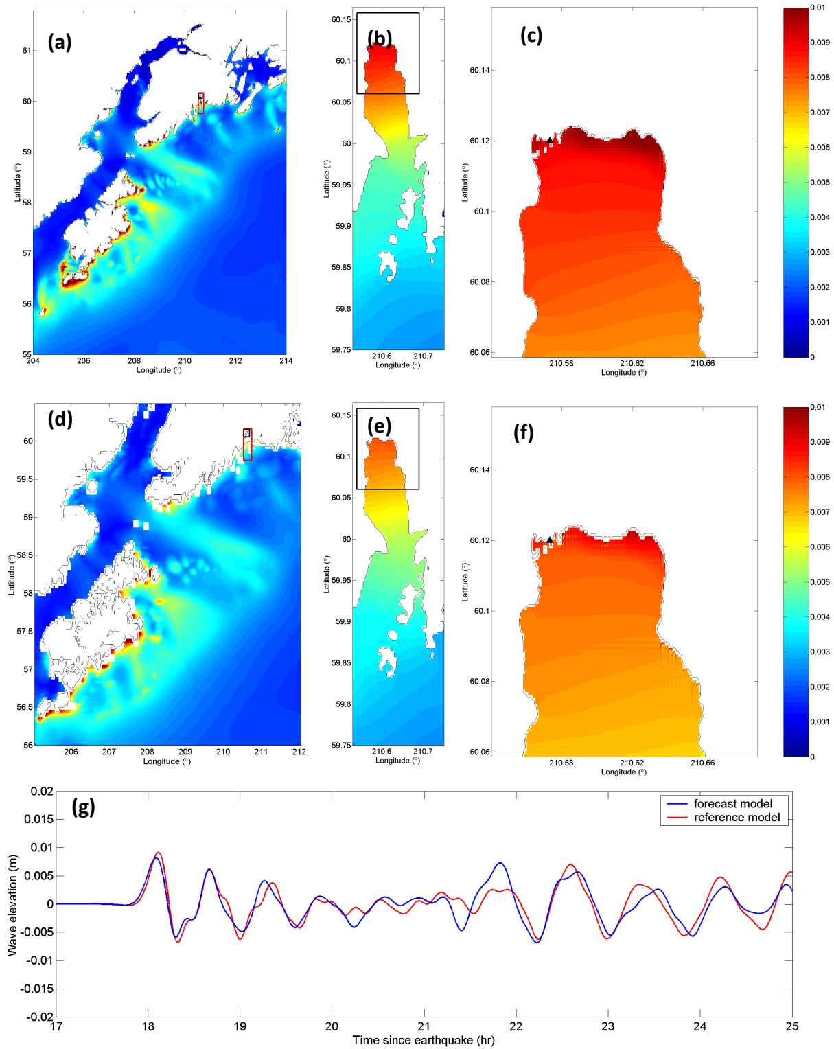
Figure 11: Model results for the 2007 Chile event: maximum water surface elevations (m) in reference model A- (a), B- (b), and C-grids (c), in forecast model A- (d), B- (e), and C-grids (f), and time-series of water surface elevations at the tide gage (indicated as black triangles in C-grids).
