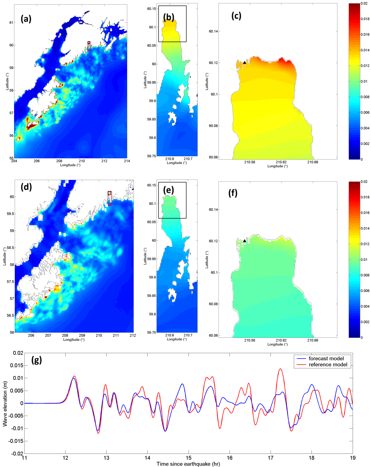
Figure 12: Model results for the 2009 Samoa event: maximum water surface elevations (m) in reference model A- (a), B- (b), and C-grids (c), in forecast model A- (d), B- (e), and C-grids (f), and time-series of water surface elevations at the tide gage (indicated as black triangles in C-grids).
