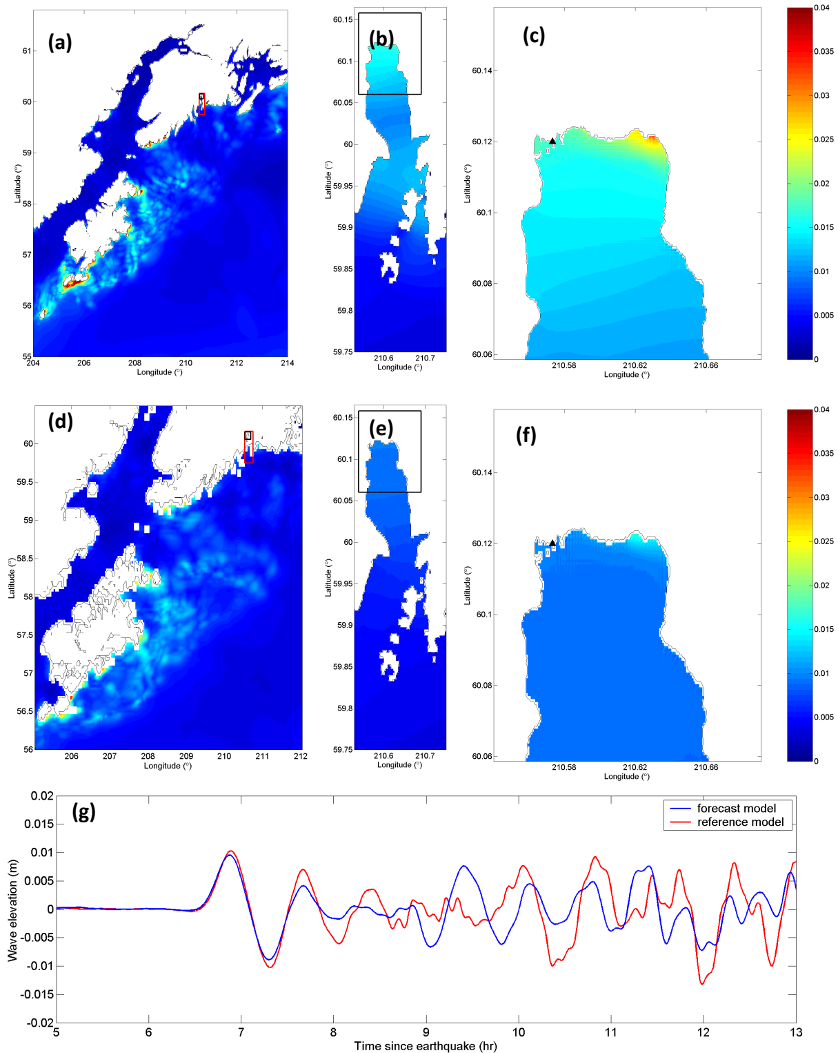
Figure 9: Model results for the 2006 Kuril Islands event: maximum water surface elevations (m) in reference model A- (a), B- (b), and C-grids (c), in forecast model A- (d), B- (e), and C-grids (f), and time-series of water surface elevations at the tide gage (indicated as black triangles in C-grids).
