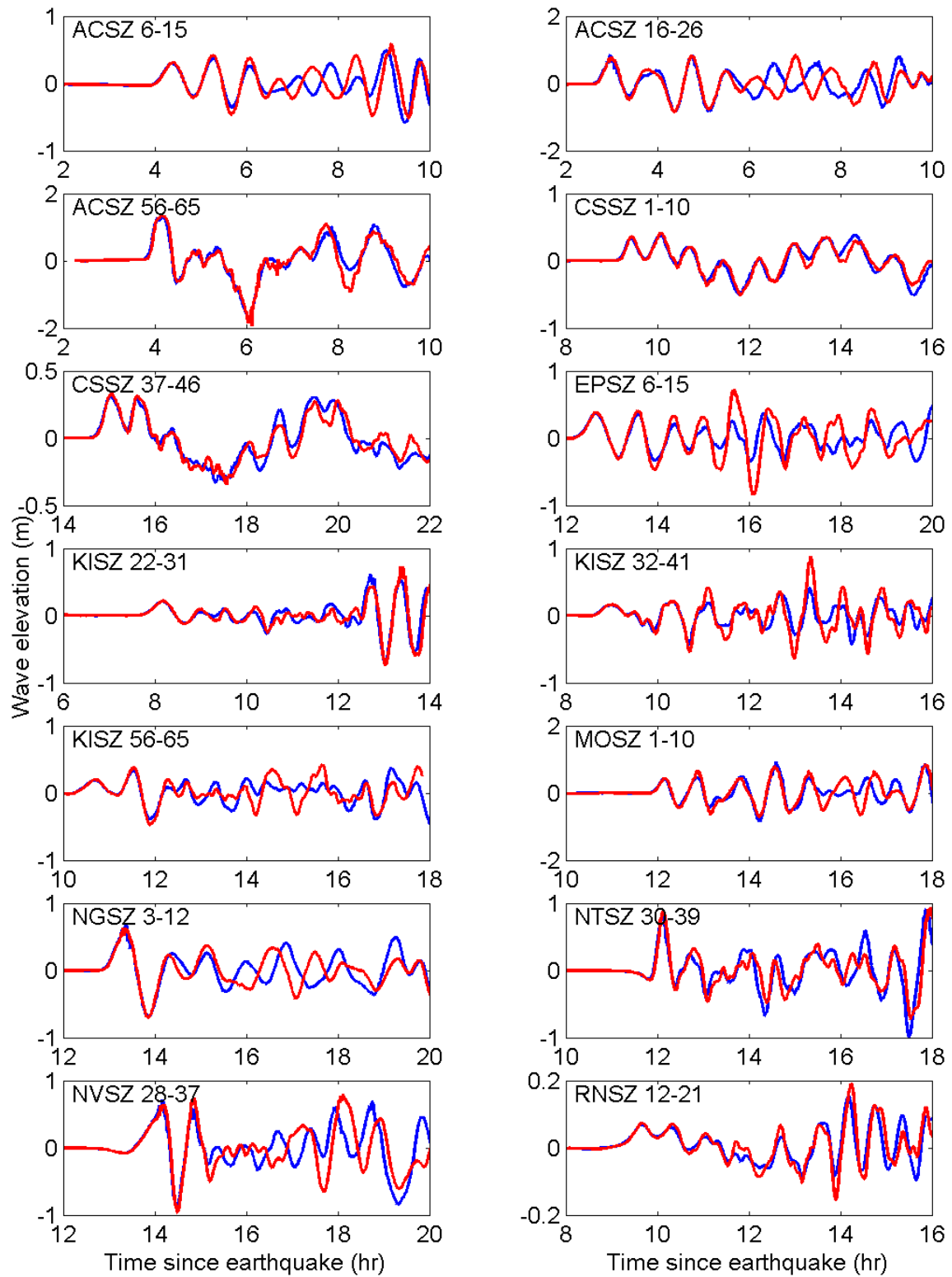
Figure 21: Time-series of water surface elevations at the tide gage in mega tsunami scenarios computed with reference model (red) and forecast model (blue), respectively.
