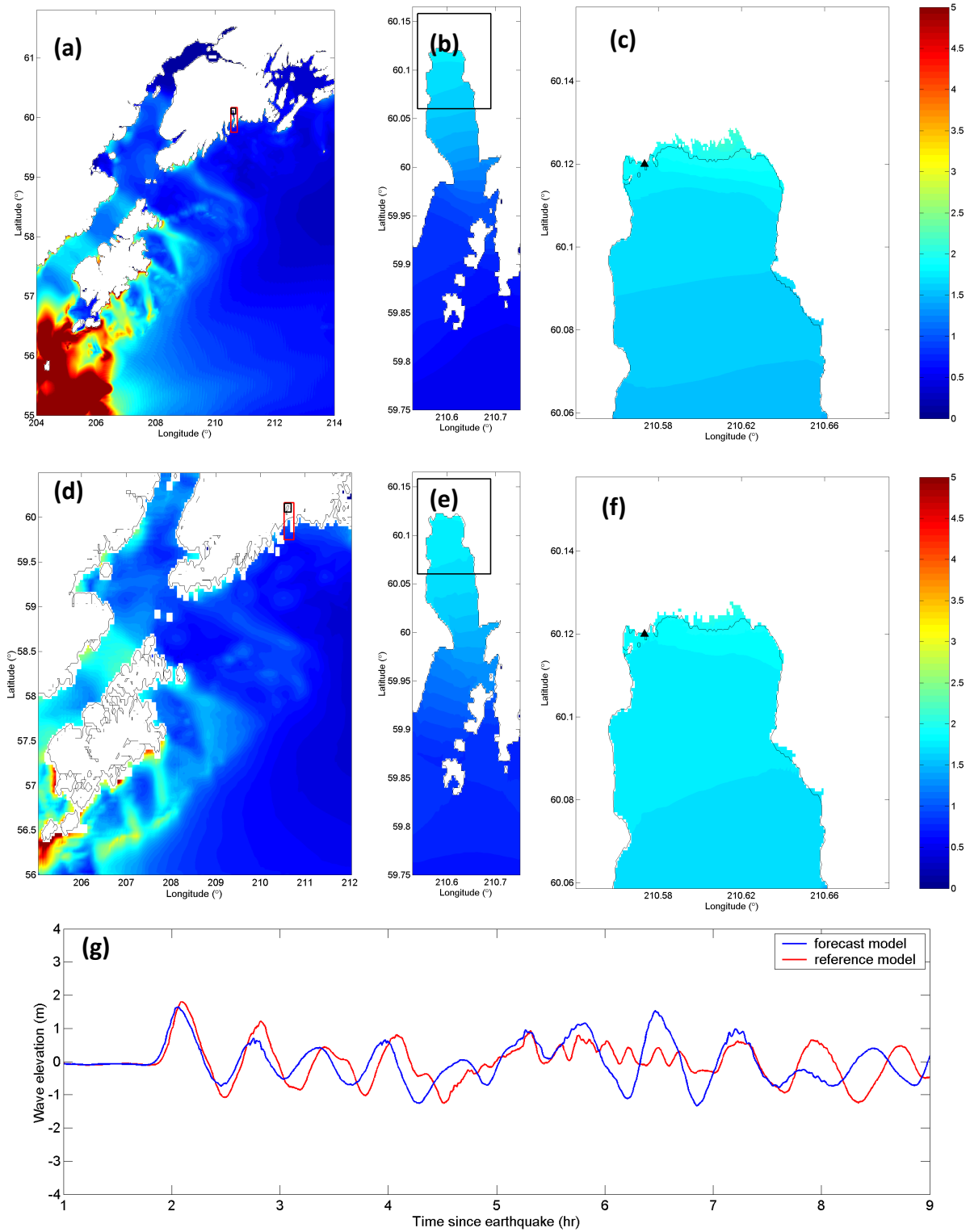
Figure 16: Model results for synthetic scenario of ACSZ 22–31: maximum water surface elevations (m) in reference model A- (a), B- (b), and C-grids (c), in forecast model A- (d), B- (e), and C-grids (f), and time-series of water surface elevations at the tide gage (indicated as black triangles in C-grids).
