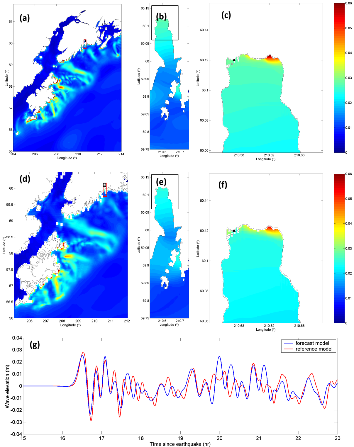
Figure 10: Model results for the 2007 Peru event: maximum water surface elevations (m) in reference model A- (a), B- (b), and C-grids (c), in forecast model A- (d), B- (e), and C-grids (f), and time-series of water surface elevations at the tide gage (indicated as black triangles in C-grids).
