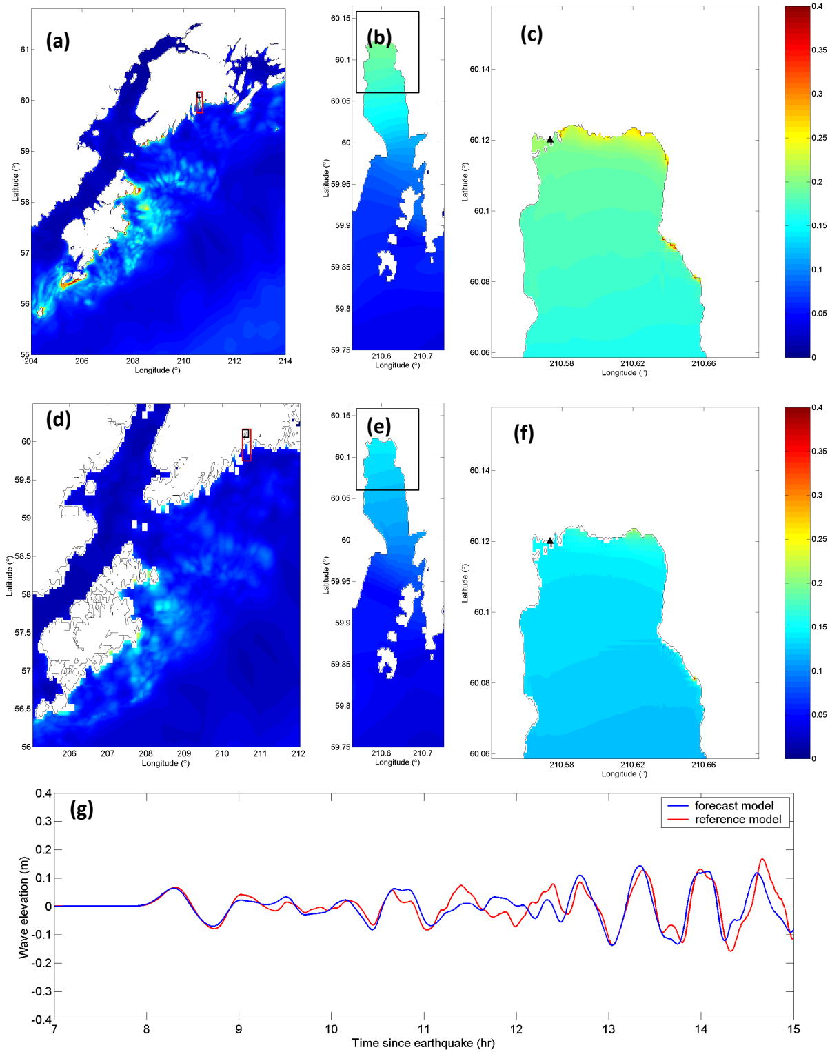
Figure 14: Model results for the 2011 Tohoku event: maximum water surface elevations (m) in reference model A- (a), B- (b), and C-grids (c), in forecast model A- (d), B- (e), and C-grids (f), and time-series of water surface elevations at the tide gage (indicated as black triangles in C-grids).
