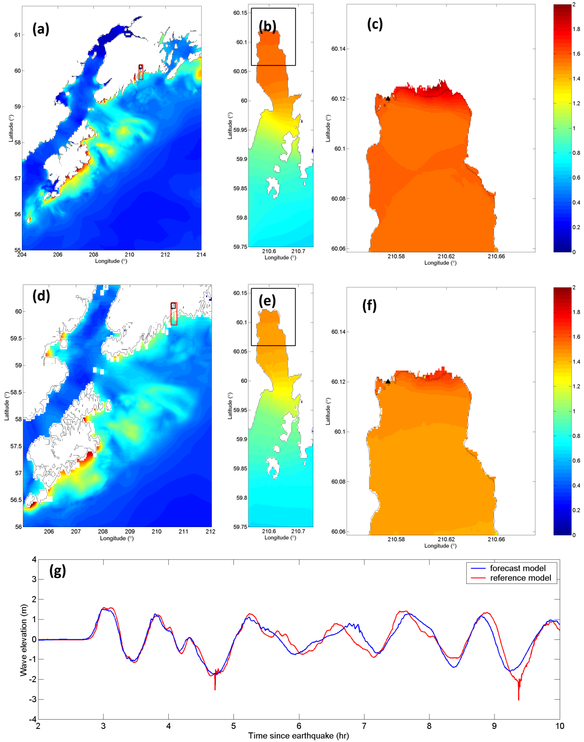
Figure 17: Model results for synthetic scenario of ACSZ 50–59: maximum water surface elevations (m) in reference model A- (a), B- (b), and C-grids (c), in forecast model A- (d), B- (e), and C-grids (f), and time-series of water surface elevations at the tide gage (indicated as black triangles in C-grids).
