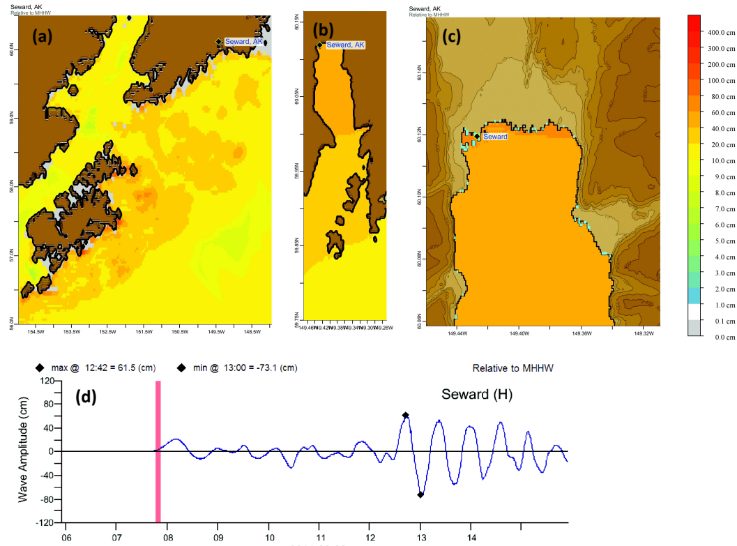
Figure C1: Response of the Seward forecast model to synthetic scenario KISZ 22-31 ( \alpha=30 ). Maximum sea surface elevation for (a) A-grid, (b) B-grid, (c) C-grid. Sea surface elevation time series at the C-grid warning point (d).
