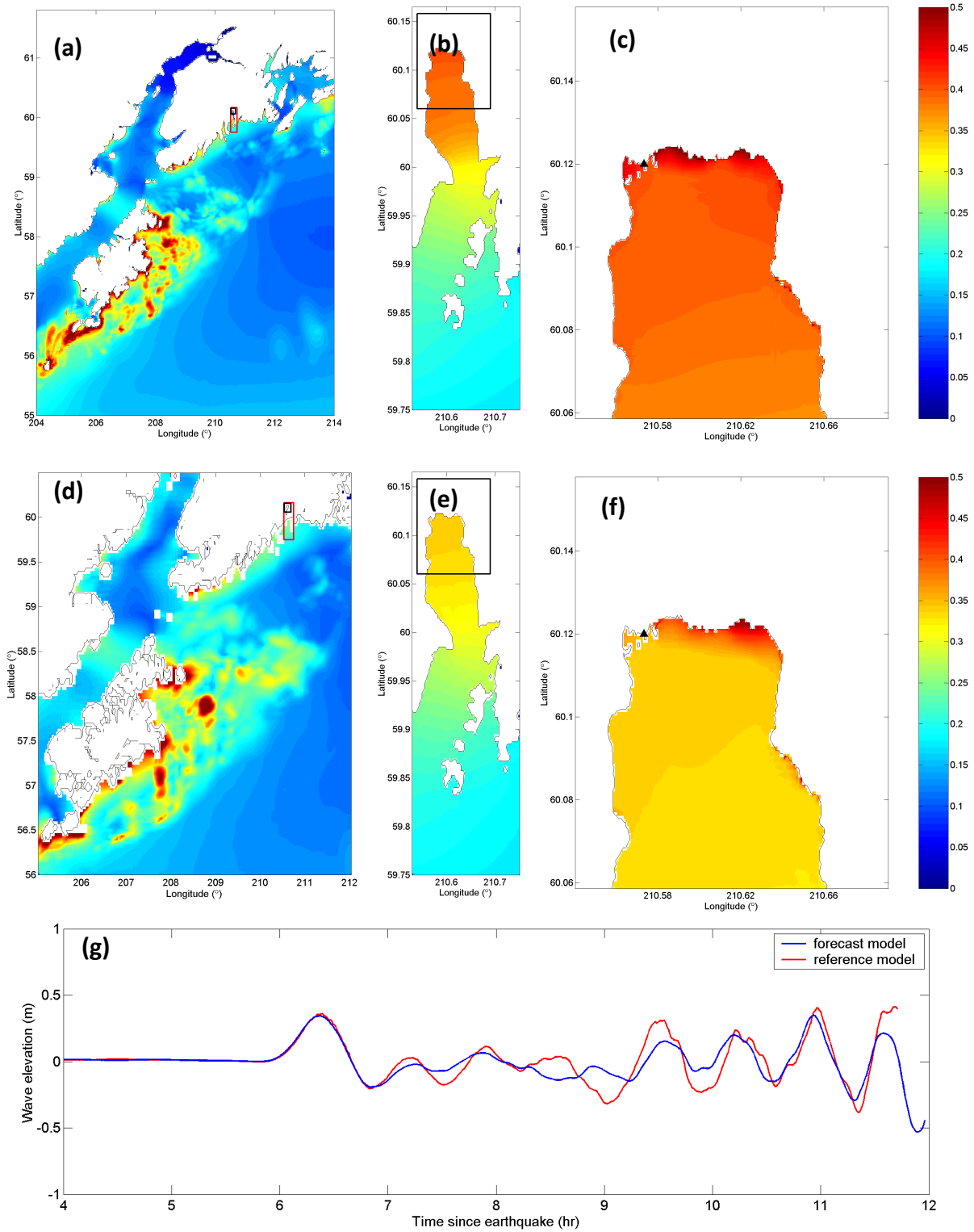
Figure 19: Model results for synthetic scenario of KISZ 1–10: maximum water surface elevations (m) in reference model A- (a), B- (b), and C-grids (c), in forecast model A- (d), B- (e), and C-grids (f), and time-series of water surface elevations at the tide gage (indicated as black triangles in C-grids).
