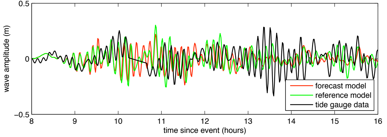
Figure 20 Model results for the 2011 Tohoku Mw 9.0 event. The upper two panels show, respectively, the forecast and reference model maximum wave height predictions. The lower panel shows the forecast model (red), reference model (green) and observed (black) wave amplitudes at the Port Alexander tide gauge location.
