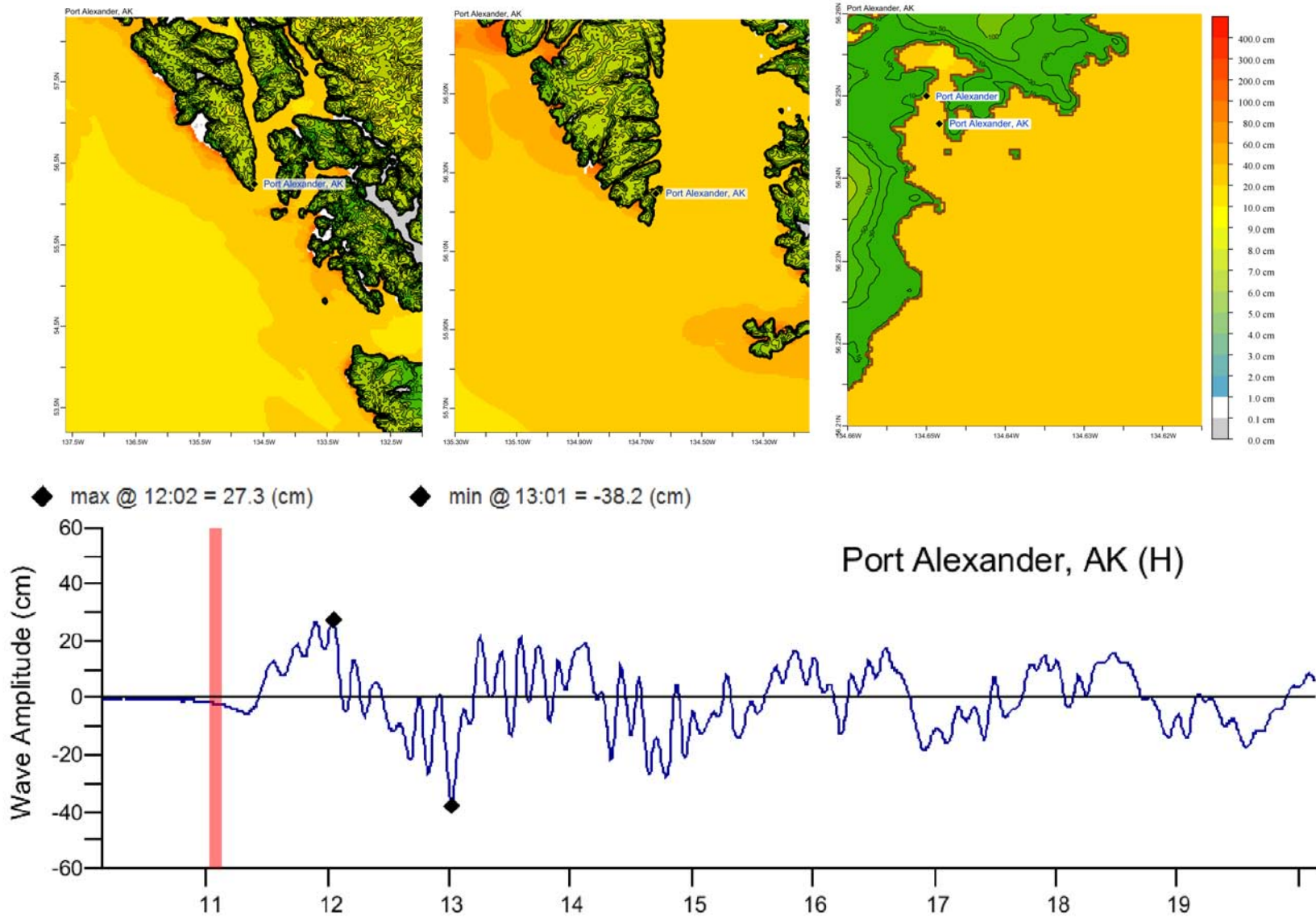
Figure 4: Response of the Port Alexander forecast model to synthetic scenario NTSZ 30-39 ( \alpha=25 ). Maximum sea surface elevation for (a) A-grid, b) B-grid, c) C-grid. Sea surface elevation time series at the C-grid warning point .
