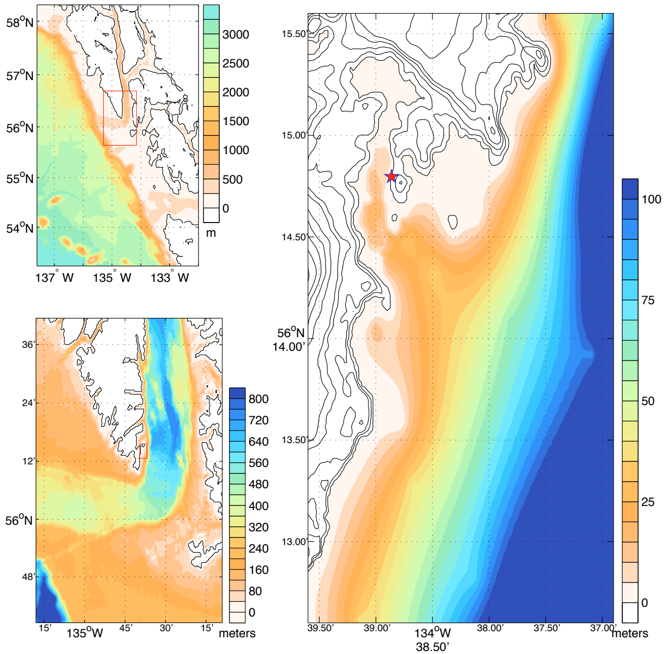
Figure 8 Bathymetry (meters) for the forecast inundation model grids. The A grid is shown in the top left panel, the B grid in the bottom left panel, and the C grid in the right panel. The topography of the C grid is shown using contours with 10 meter intervals from 0 to 40 and then 40 meters intervals for higher values. The red boxes in the A and B plots show the position of the nested B and C grids, respectively. The red star shows the location of the Port Alexander tide gauge.
