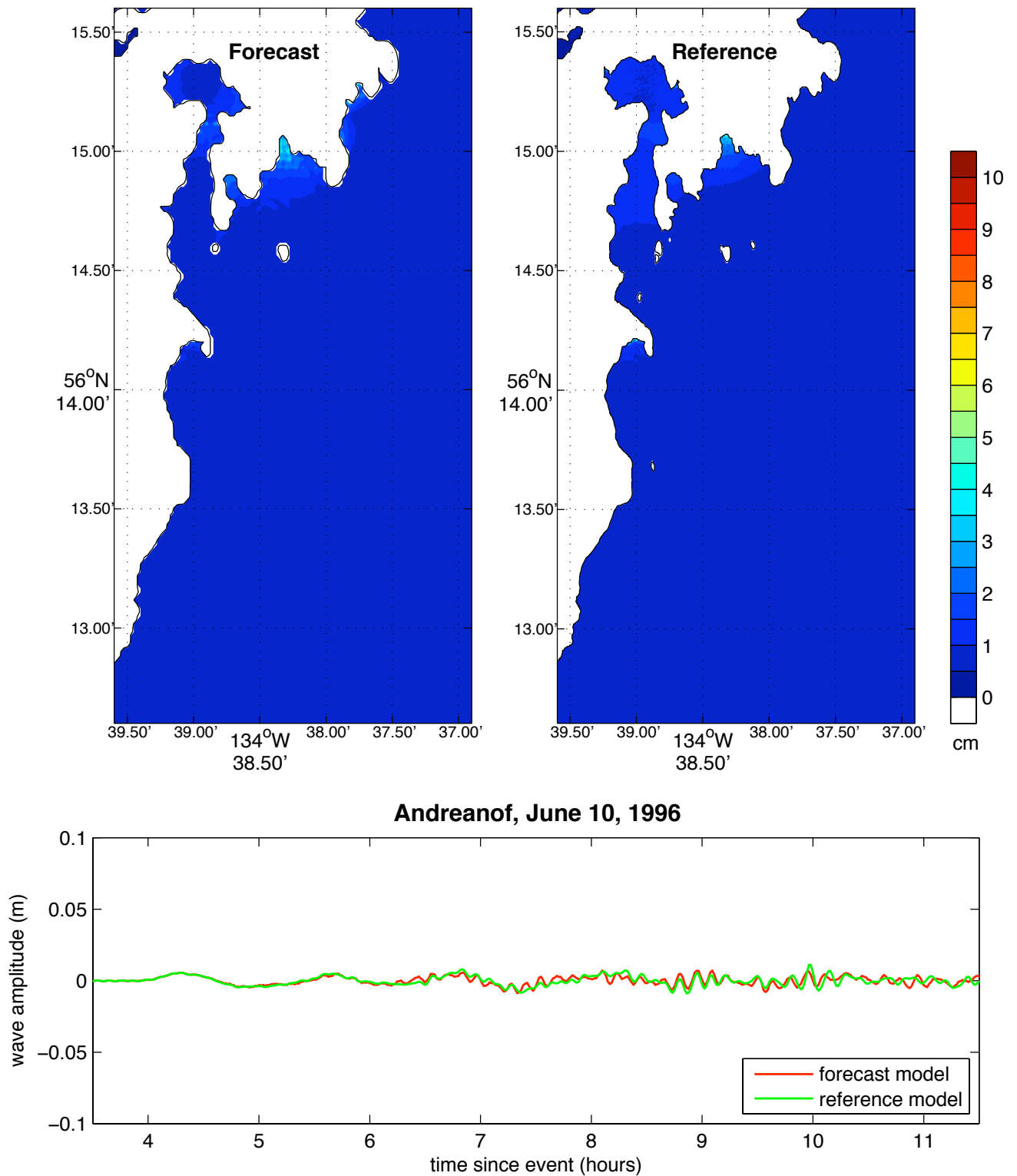
Figure 14 Model results for the 1996 Andreanof Mw 7.9 event. The upper two panels show, respectively, the forecast and reference model maximum wave height predictions. The lower panel shows the forecast model (red) and reference model (green) wave amplitudes at the Port Alexander tide gauge location.
