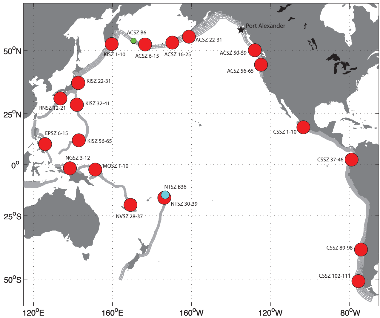
Figure 21 Map of the Pacific Ocean Basin showing the locations of the 19 simulated Mw 9.3 events (red circles) and the medium and micro events used to test and validate the Port Alexander model. The solid star denotes the location of Port Alexander.
