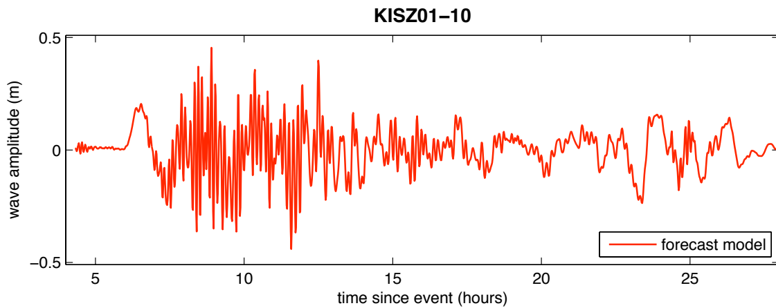
Figure 22 Results from the forecast model for the KISZ 1-10 synthetic event. The upper panel shows the map of predicted maximum wave height in the Port Alexander C-grid and the lower panel shows the time series of wave amplitude at the tide gauge location.
