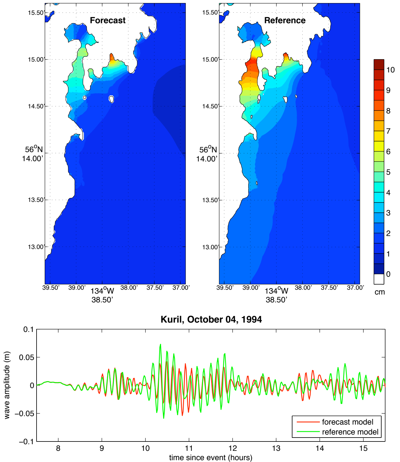
Figure 13 Model results for the 1994 Kuril Mw 8.3 event. The upper two panels show, respectively, the forecast and reference model maximum wave height predictions. The lower panel shows the forecast model (red) and reference model (green) wave amplitudes at the Port Alexander tide gauge location.
