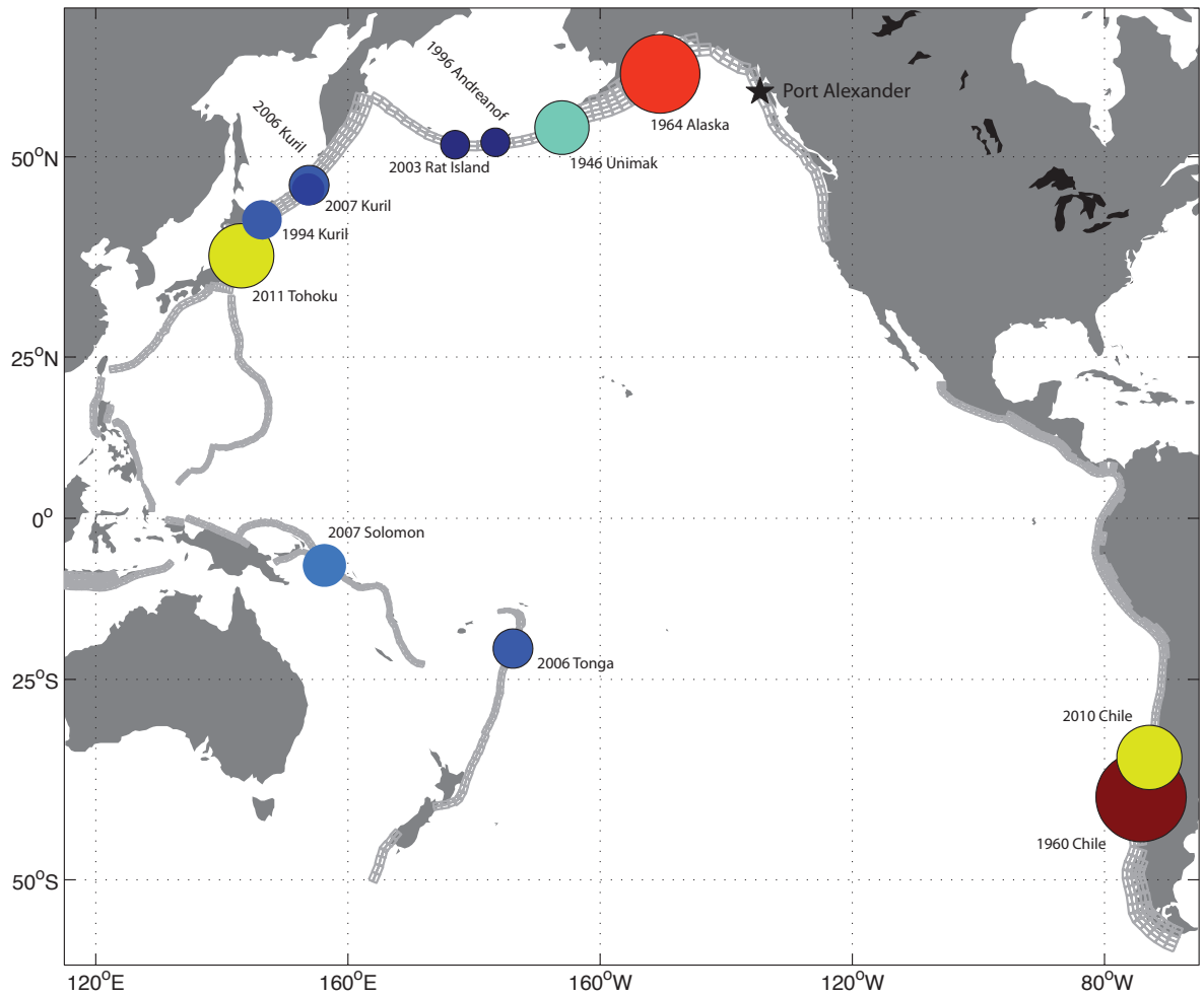
Figure 9 Map of the Pacific Ocean Basin showing the locations and magnitudes of the 12 historical events used to test and validate the Port Alexander model. Relative earthquake magnitude is shown by the varying sizes and colors of the filled circles. The largest magnitude earthquake used in model validation was the 1960 Chile Mw 9.5 earthquake. The star denotes Port Alexander's location.
