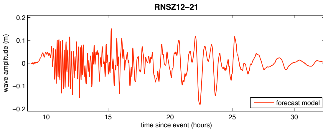
Figure 40 Results from the forecast model for the RNSZ 12-21 synthetic event. The upper panel shows the map of predicted maximum wave height in the Port Alexander C-grid and the lower panel shows the time series of wave amplitude at the tide gauge location.
