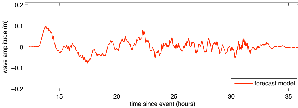
Figure 32 Results from the forecast model for the CSSZ 37-46 synthetic event. The upper panel shows the map of predicted maximum wave height in the Port Alexander C-grid and the lower panel shows the time series of wave amplitude at the tide gauge location.
