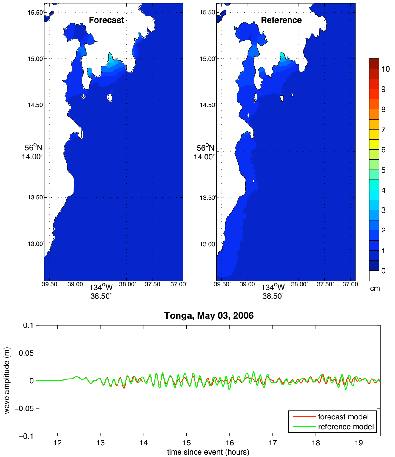
Figure 16 Model results for the 2006 Tonga Mw 8.0 event. The upper two panels show, respectively, the forecast and reference model maximum wave height predictions. The lower panel shows the forecast model (red) and reference model (green) wave amplitudes at the Port Alexander tide gauge location.
