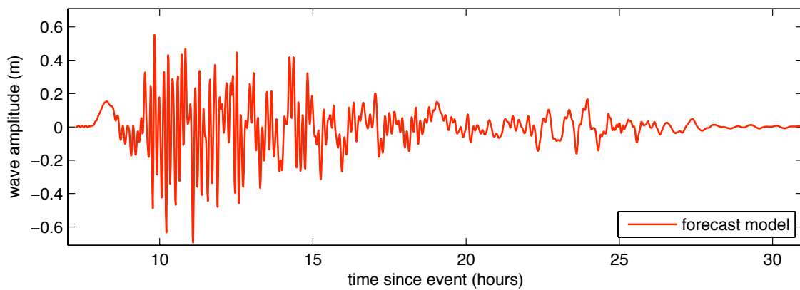
Figure 23 Results from the forecast model for the KISZ 22-31 synthetic event. The upper panel shows the map of predicted maximum wave height in the Port Alexander C-grid and the lower panel shows the time series of wave amplitude at the tide gauge location.
