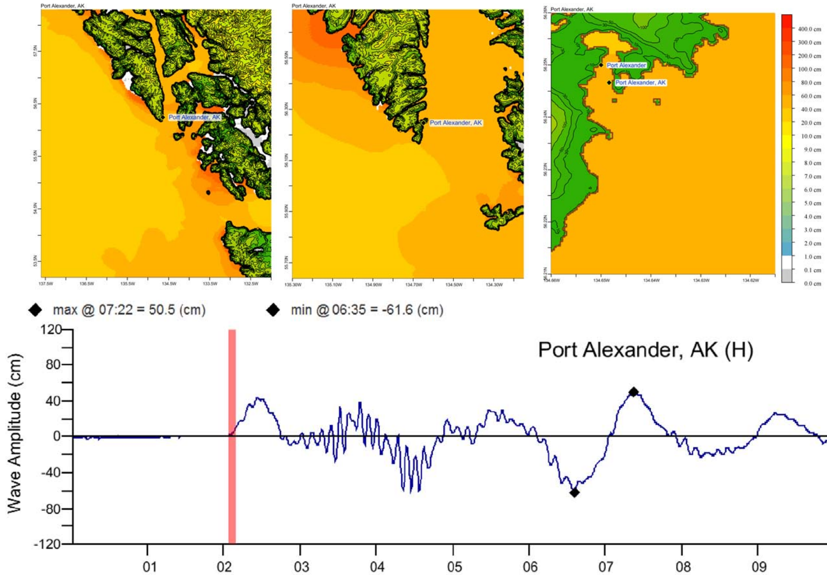
Figure 2: Response of the Port Alexander forecast model to synthetic scenario ACSZ 56-65 ( \alpha=25 ). Maximum sea surface elevation for (a) A-grid, b) B-grid, c) C-grid. Sea surface elevation time series at the C-grid warning point
