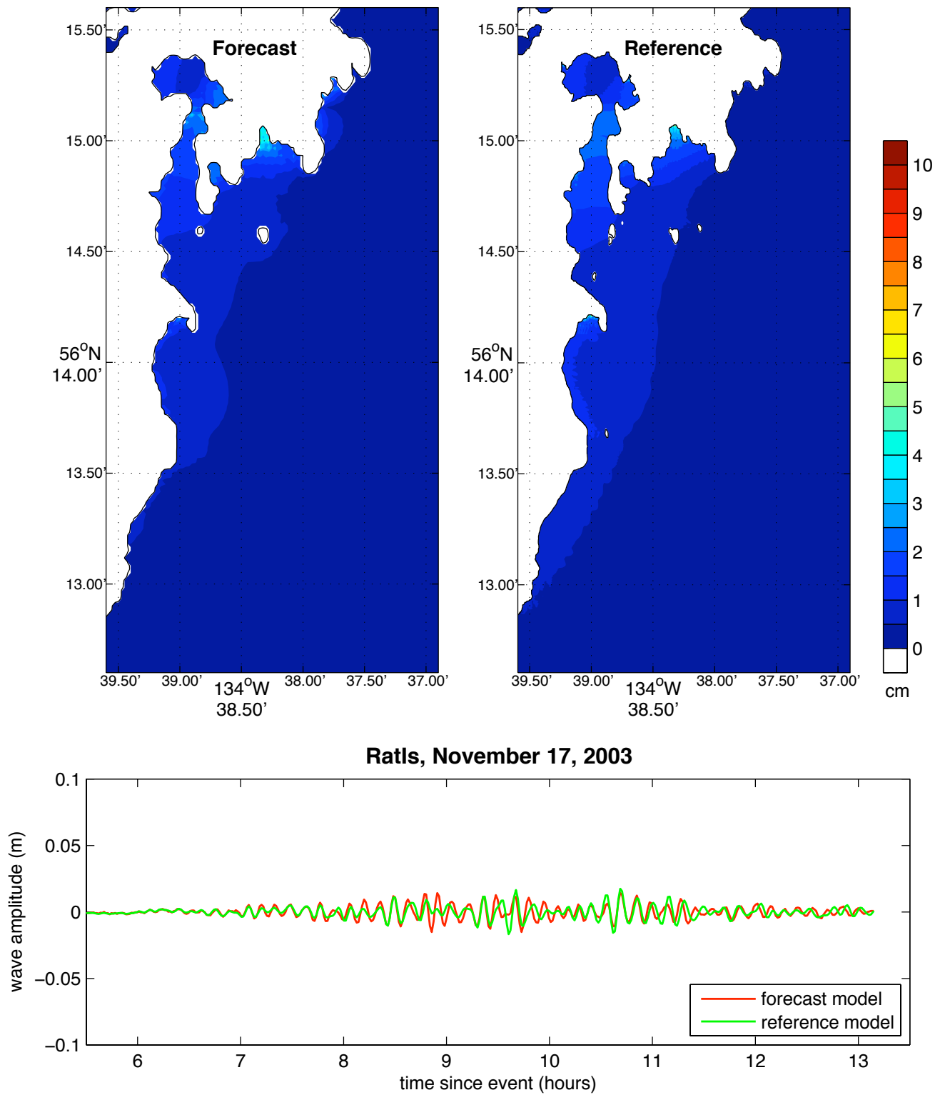
Figure 15 Model results for the 2003 Rat Island Mw 7.7 event. The upper two panels show, respectively, the forecast and reference model maximum wave height predictions. The lower panel shows the forecast model (red) and reference model (green) wave amplitudes at the Port Alexander tide gauge location.
