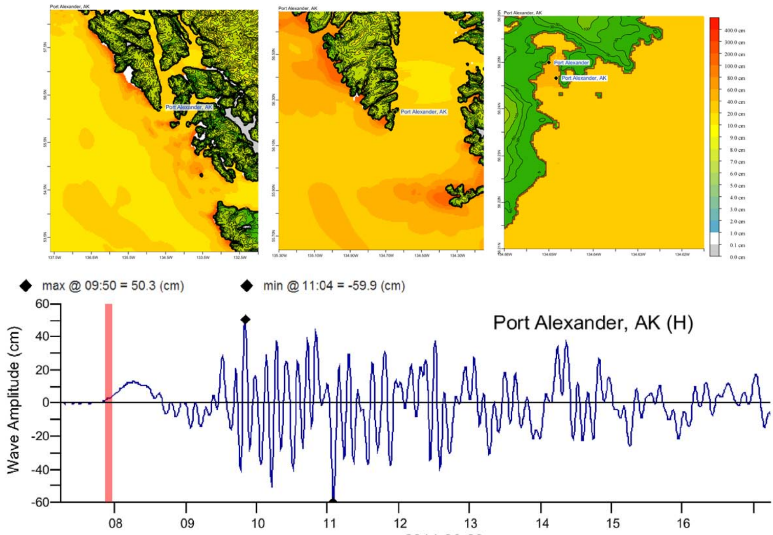
Figure 1: Response of the Port Alexander forecast model to synthetic scenario KISZ 22-31 ( \alpha=25 ). Maximum sea surface elevation for (a) A-grid, b) B-grid, c) C-grid. Sea surface elevation time series at the C-grid warning point
