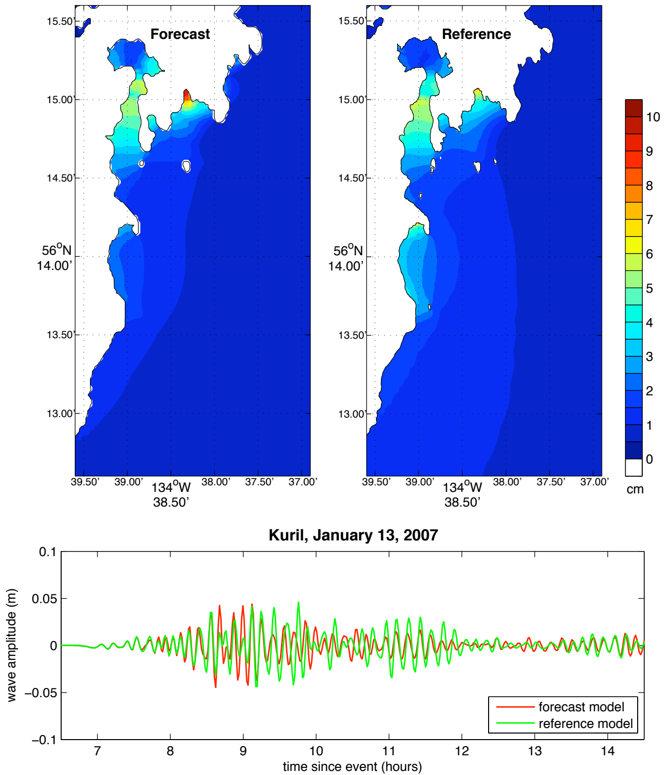
Figure 18 Model results for the 2007 Kuril Mw 8.1 event. The upper two panels show, respectively, the forecast and reference model maximum wave height predictions. The lower panel shows the forecast model (red) and reference model (green) wave amplitudes at the Port Alexander tide gauge location.
