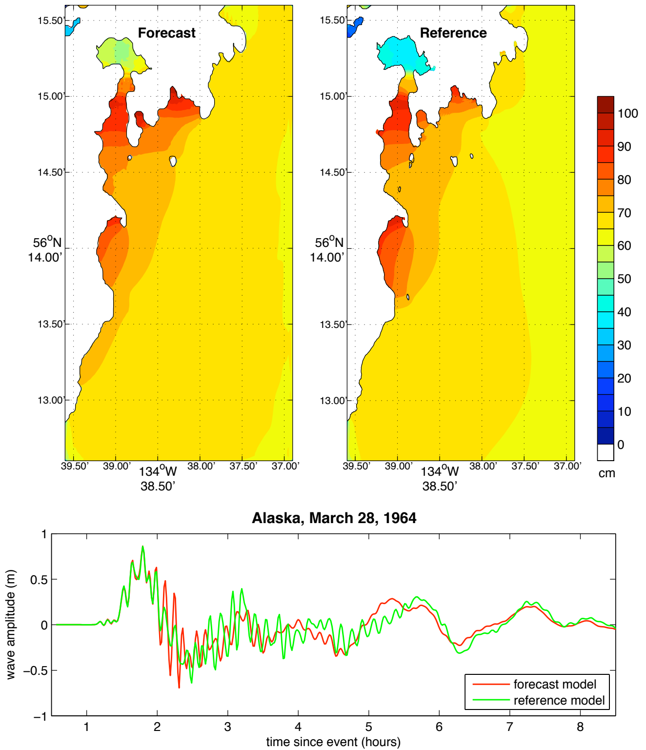
Figure 12 Model results for the 1964 Alaska Mw 9.2 event. The upper two panels show, respectively, the forecast and reference model maximum wave height predictions. The lower panel shows the forecast model (red) and reference model (green) wave amplitudes at the Port Alexander tide gauge location
