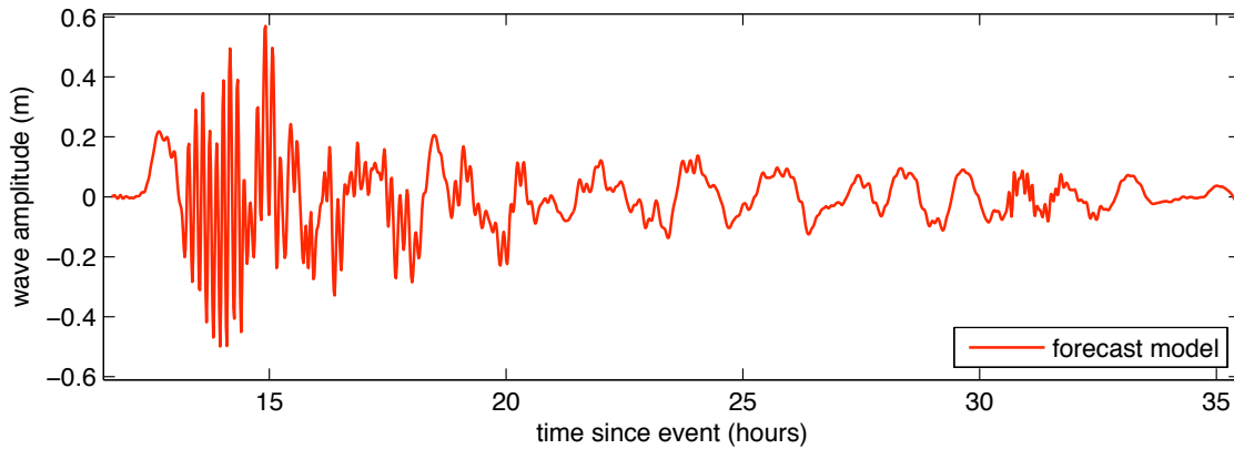
Figure 39 Results from the forecast model for the EPSZ 6-15 synthetic event. The upper panel shows the map of predicted maximum wave height in the Port Alexander C-grid and the lower panel shows the time series of wave amplitude at the tide gauge location.
