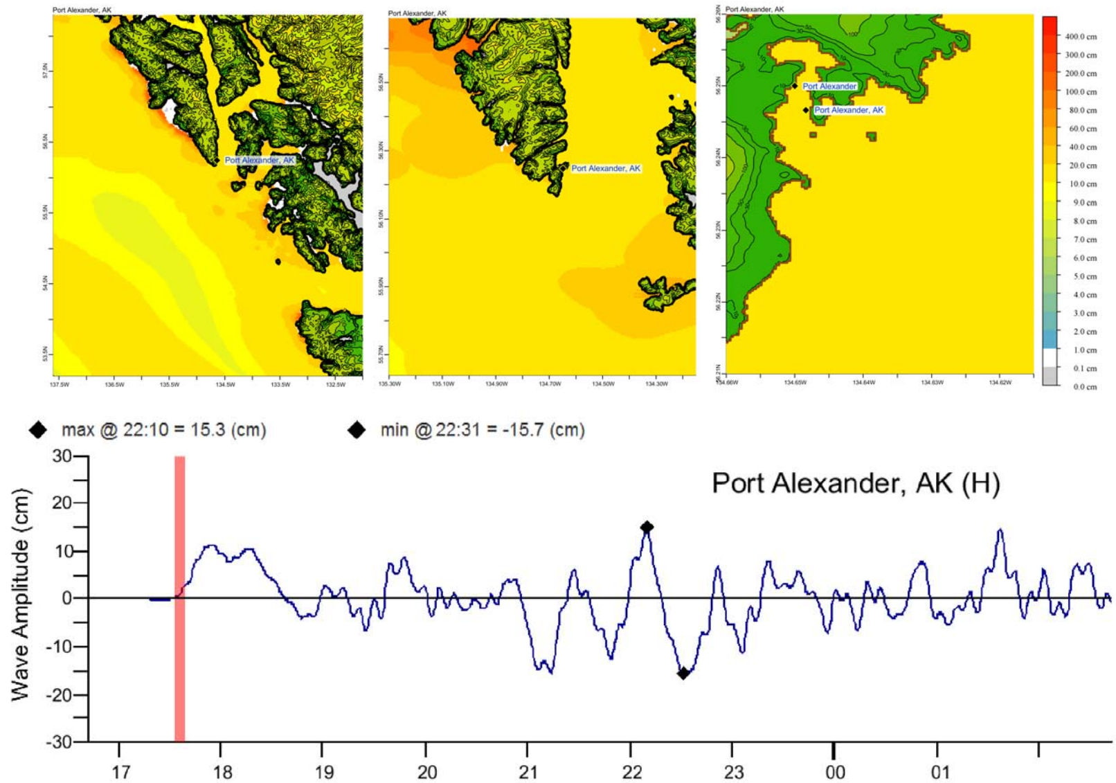
Figure 3: Response of the Port Alexander forecast model to synthetic scenario CSSZ 89-98 (alpha=25). Maximum sea surface elevation for (a) A-grid, b) B-grid, c) C-grid. Sea surface elevation time series at the C-grid warning point
