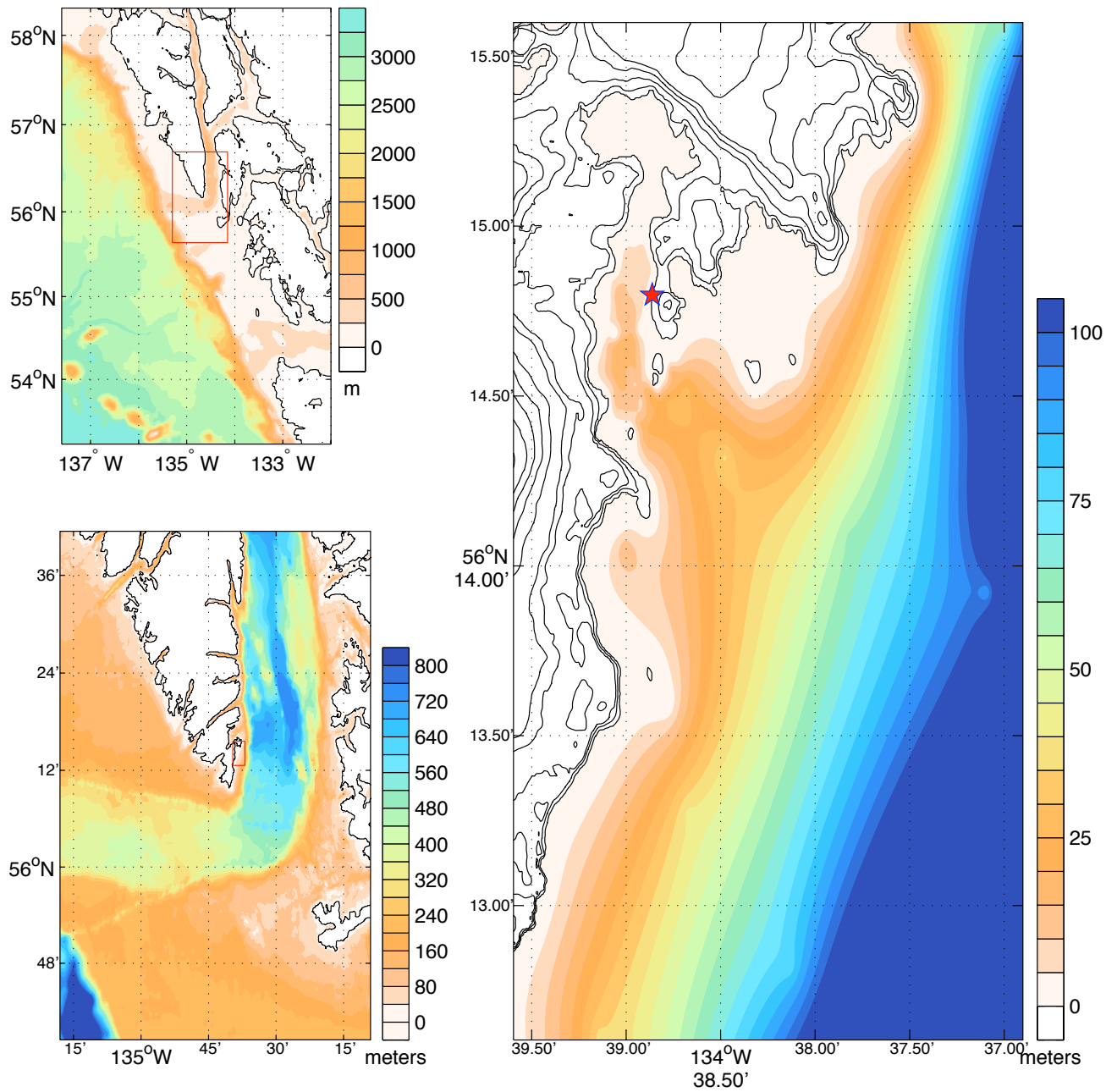
Figure 7 Bathymetry (meters) for the reference inundation model grids. The A grid is shown in the top left panel, the B grid in the bottom left panel, and the C grid in the right panel. The topography of the C grid is shown using contours with 10 meter intervals from 0 to 40 and then 40 meters intervals for higher values. The red boxes in the A and B plots show the position of the nested B and C grids, respectively. The red star shows the location of the Port Alexander tide gauge.
