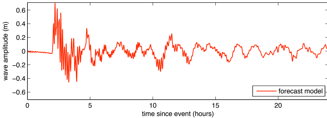
Figure 28 Results from the forecast model for the ACSZ 22-31 synthetic event. The upper panel shows the map of predicted maximum wave height in the Port Alexander C-grid and the lower panel shows the time series of wave amplitude at the tide gauge location.
