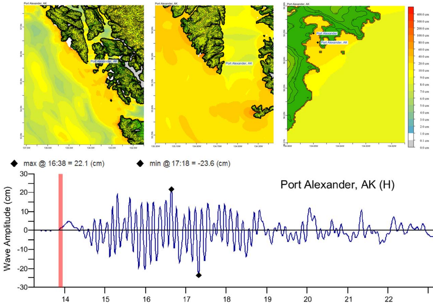
Figure 5: Response of the Port Alexander forecast model to the 2011 Tohoku, Japan tsunami. Maximum sea surface elevation for (a) A-grid, b) B-grid, c) C-grid. Sea surface elevation time series at the C-grid warning point (d).
