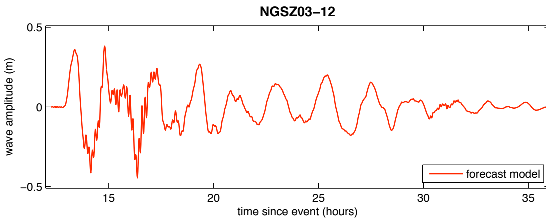
Figure 38 Results from the forecast model for the NGSZ 3-12 synthetic event. The upper panel shows the map of predicted maximum wave height in the Port Alexander C-grid and the lower panel shows the time series of wave amplitude at the tide gauge location.
