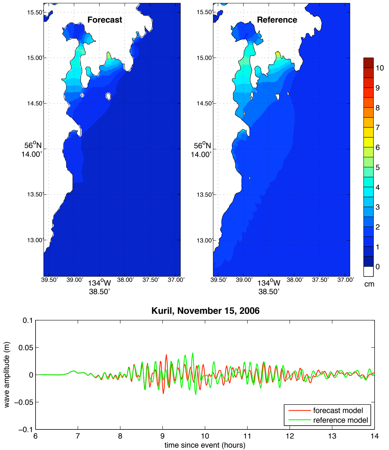
Figure 17 Model results for the 2006 Kuril Mw 8.3 event. The upper two panels show, respectively, the forecast and reference model maximum wave height predictions. The lower panel shows the forecast model (red) and reference model (green) wave amplitudes at the Port Alexander tide gauge location.
