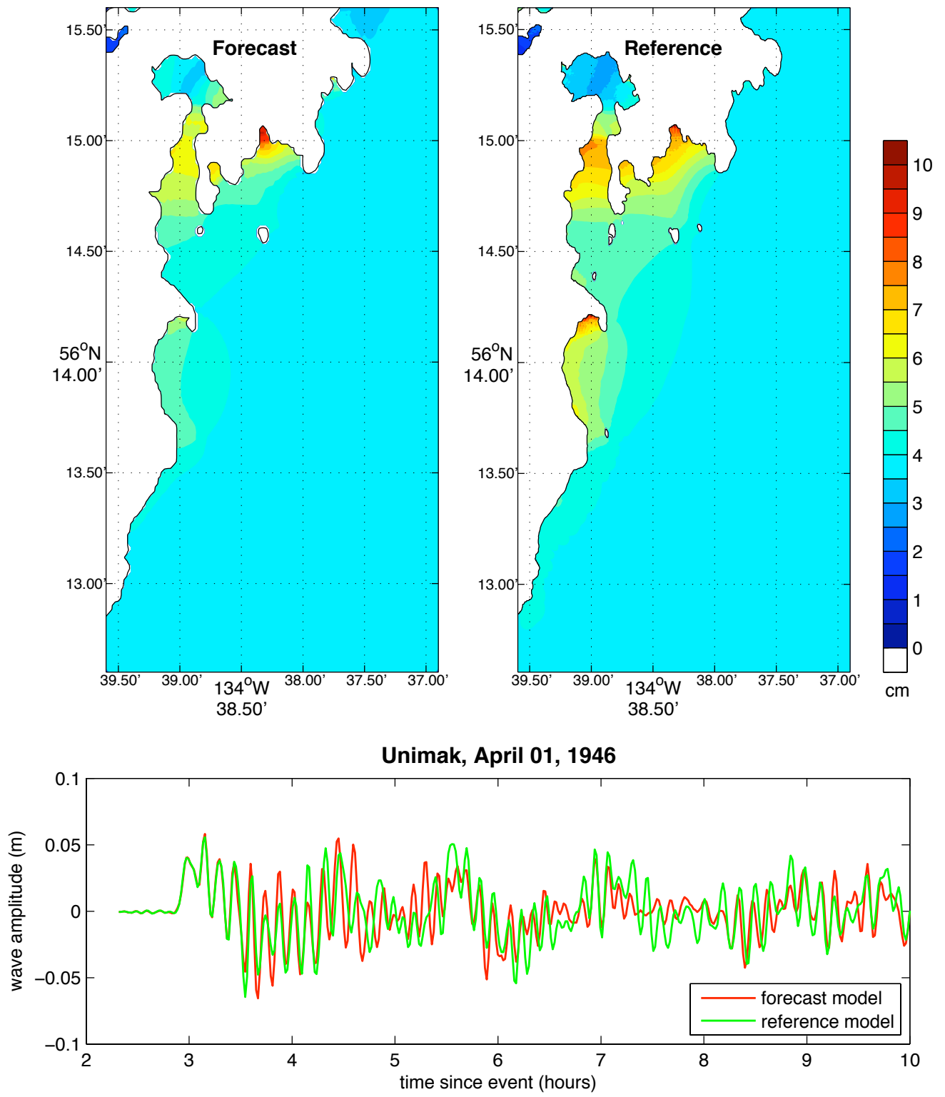
Figure 10 Model results for the 1946 Unimak Mw 8.5 event. The upper two panels show, respectively, the forecast and reference model maximum wave height predictions. The lower panel shows the forecast model (red) and reference model (green) wave amplitudes at the Port Alexander tide gauge location.
