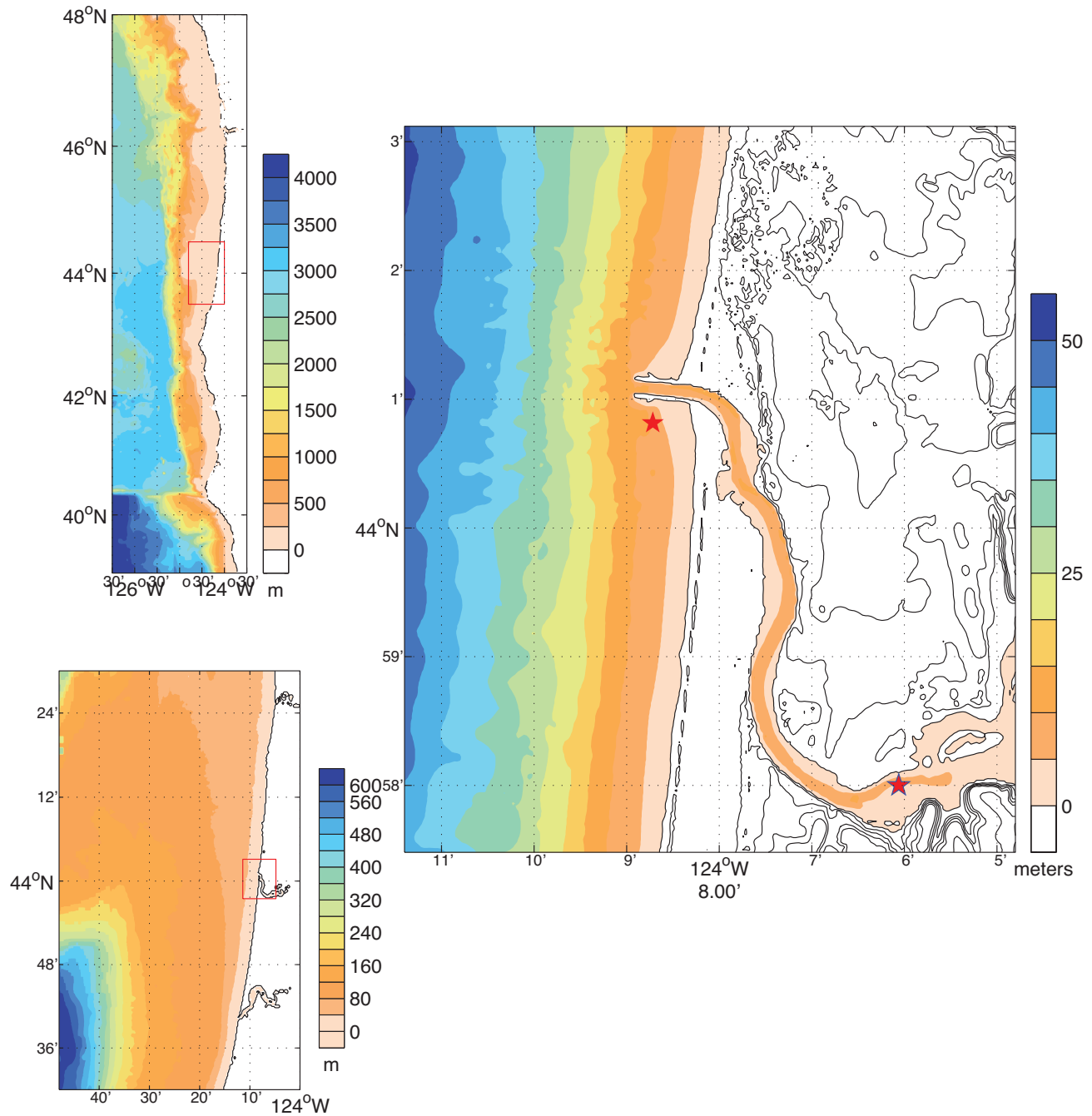
Figure 7 Bathymetry (meters) for the forecast inundation model grids. The A grid is shown in the top left panel, the B grid in the bottom left panel, and the C grid in the right panel. The topography of the C grid is shown using contours with 10 meter intervals from 0 to 40 and then 40 meters intervals for higher values. The red boxes in the A and B plots show the position of the nested B and C grids, respectively. The red stars show the location of the Florence ocean and dock time-series points used in later figures.
