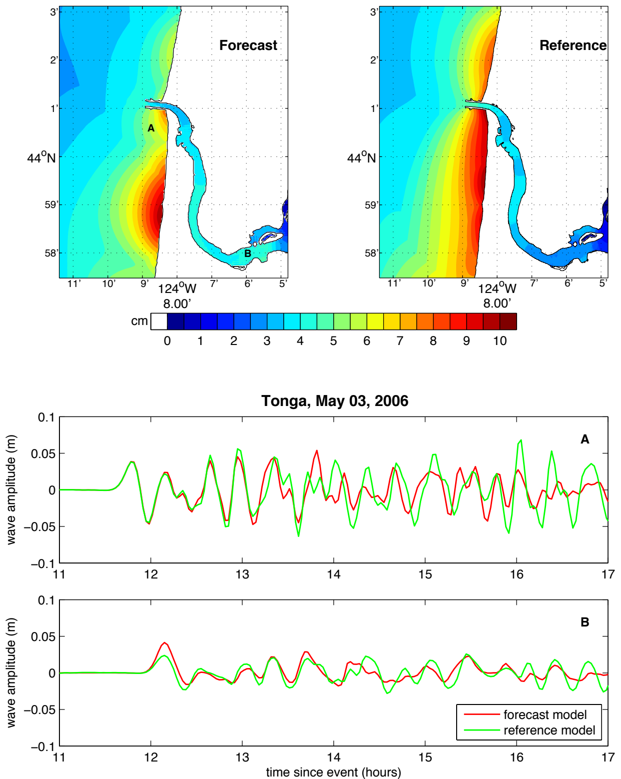
Figure 13 Model results for the 2006 Tonga Mw 8.0 event. The upper two panels show the forecast (left) and reference (right) model maximum wave height predictions. The lower panels show the forecast model (red) and reference model (green) wave amplitudes at the points labeled A and B in the forecast model wave height map.
