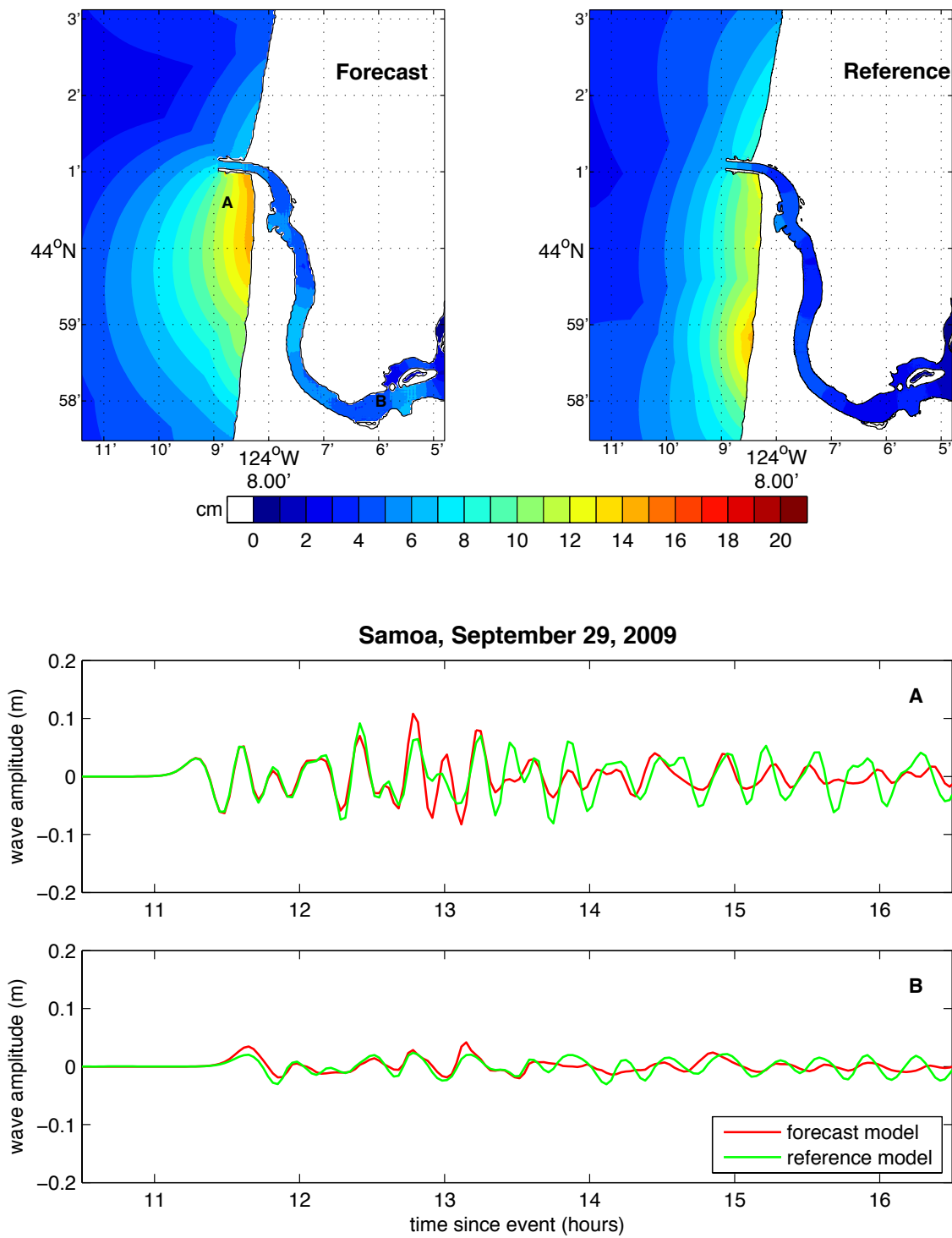
Figure 16 Model results for the 2009 Samoa Mw 8.1 event. The upper two panels show, respectively, the forecast and reference model maximum wave height predictions. The upper two panels show the forecast (left) and reference (right) model maximum wave height predictions. The lower panels show the forecast model (red) and reference model (green) wave amplitudes at the points labeled A and B in the forecast model wave height map.
