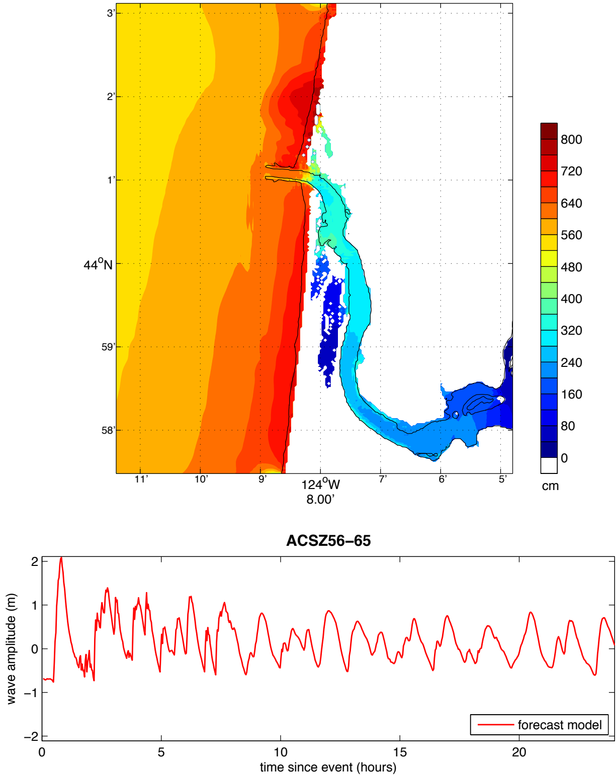
Figure 28 Results from the forecast model for the ACSZ 56-65 synthetic event. The upper panel shows the map of predicted maximum wave height in the Florence C-grid and the lower panel shows the time series of wave amplitude at the warning point location.
