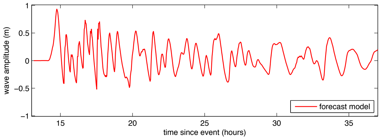
Figure 36 Results from the forecast model for the NGSZ 3-12 synthetic event. The upper panel shows the map of predicted maximum wave height in the Florence C-grid and the lower panel shows the time series of wave amplitude at the warning point location.
