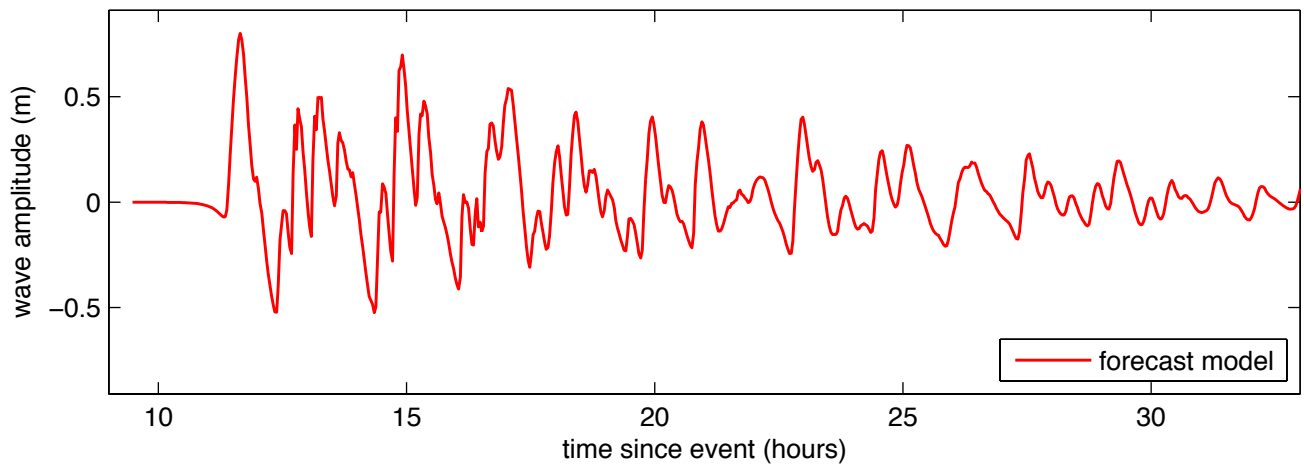
Figure 33 Results from the forecast model for the NTSZ 30-39 synthetic event. The upper panel shows the map of predicted maximum wave height in the Florence C-grid and the lower panel shows the time series of wave amplitude at the warning point location.
