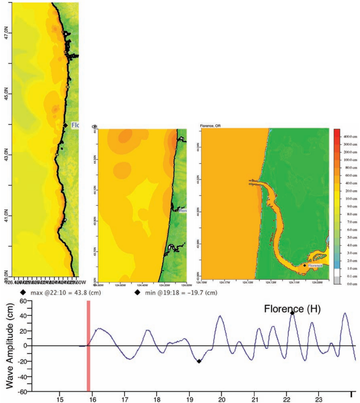
Figure 3: Response of the Florence forecast model to synthetic scenario CSSZ 89-98 (alpha=25). Maximum sea surface elevation for (a) A-grid, b) B-grid, c) C-grid. Sea surface elevation time series at the C-grid warning point
