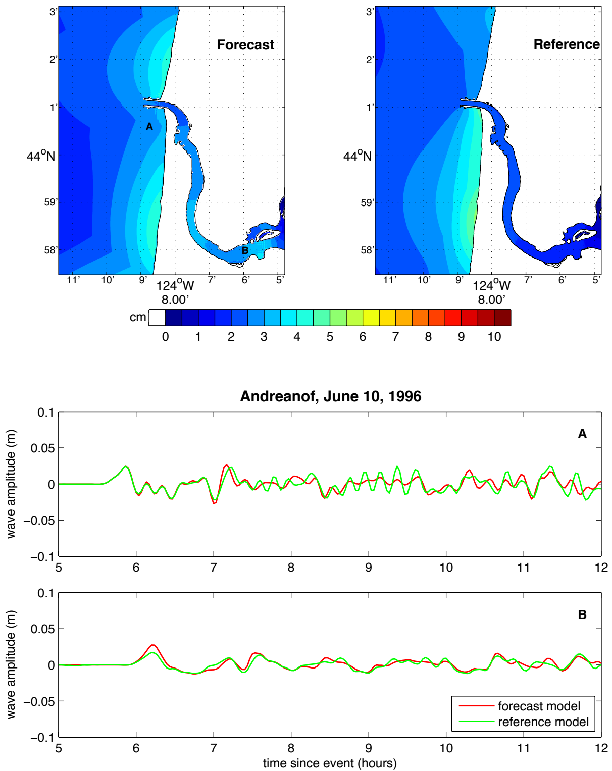
Figure 12 Model results for the 1996 Andreanof Mw 7.9 event. The upper two panels show the forecast (left) and reference (right) model maximum wave height predictions. The lower panels show the forecast model (red) and reference model (green) wave amplitudes at the points labeled A and B in the forecast model wave height map.
