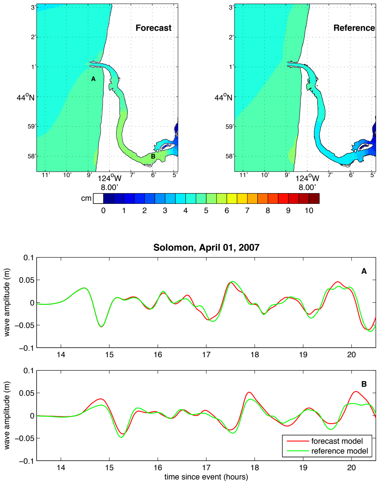
Figure 15 Model results for the 2007 Solomon Mw 8.1 event. The upper two panels show the forecast (left) and reference (right) model maximum wave height predictions. The lower panels show the forecast model (red) and reference model (green) wave amplitudes at the points labeled A and B in the forecast model wave height map.
