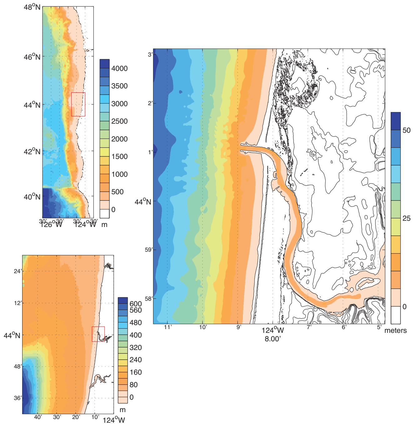
Figure 6 Bathymetry (meters) for the reference inundation model grids. The A grid is shown in the top left panel, the B grid in the bottom left panel, and the C grid in the right panel. The topography of the C grid is shown using contours with 10 meter intervals from 0 to 40 and then 40 meters intervals for higher values. The red boxes in the A and B plots show the position of the nested B and C grids, respectively.
