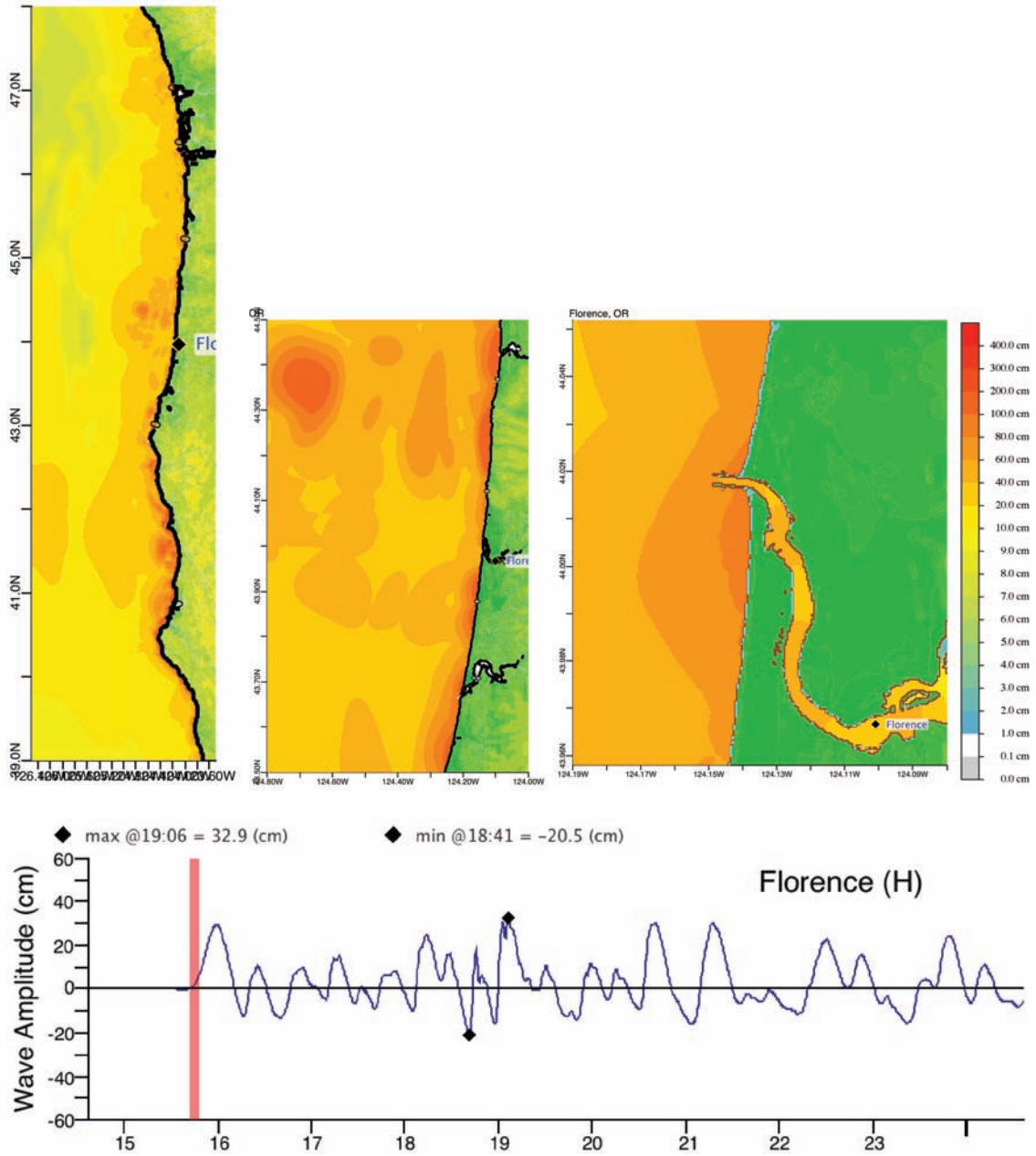
Figure 5: Response of the Florence forecast model to the 2011 Tohoku, Japan tsunami. Maximum sea surface elevation for (a) A-grid, b) B-grid, c) C-grid. Sea surface elevation time series at the C-grid warning point (d).
