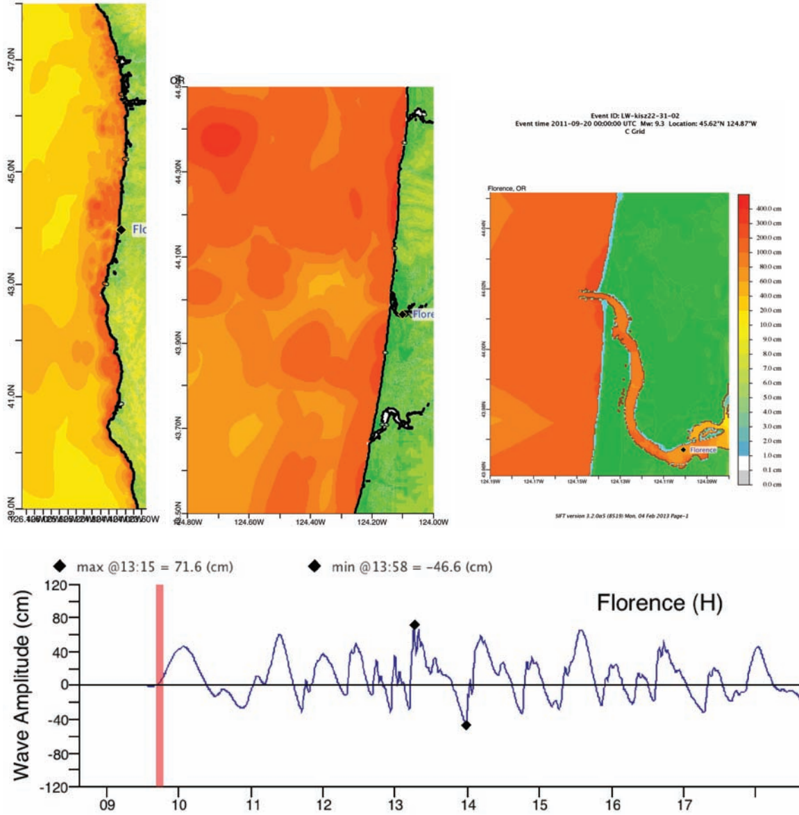
Figure 1: Response of the Florence forecast model to synthetic scenario KISZ 22-31 ( \alpha=25 ). Maximum sea surface elevation for (a) A-grid, b) B-grid, c) C-grid. Sea surface elevation time series at the C-grid warning point
