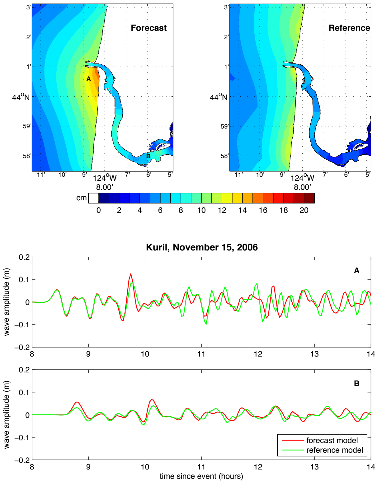
Figure 14 Model results for the 2006 Kuril Mw 8.3 event. The upper two panels show the forecast (left) and reference (right) model maximum wave height predictions. The lower panels show the forecast model (red) and reference model (green) wave amplitudes at the points labeled A and B in the forecast model wave height map.
