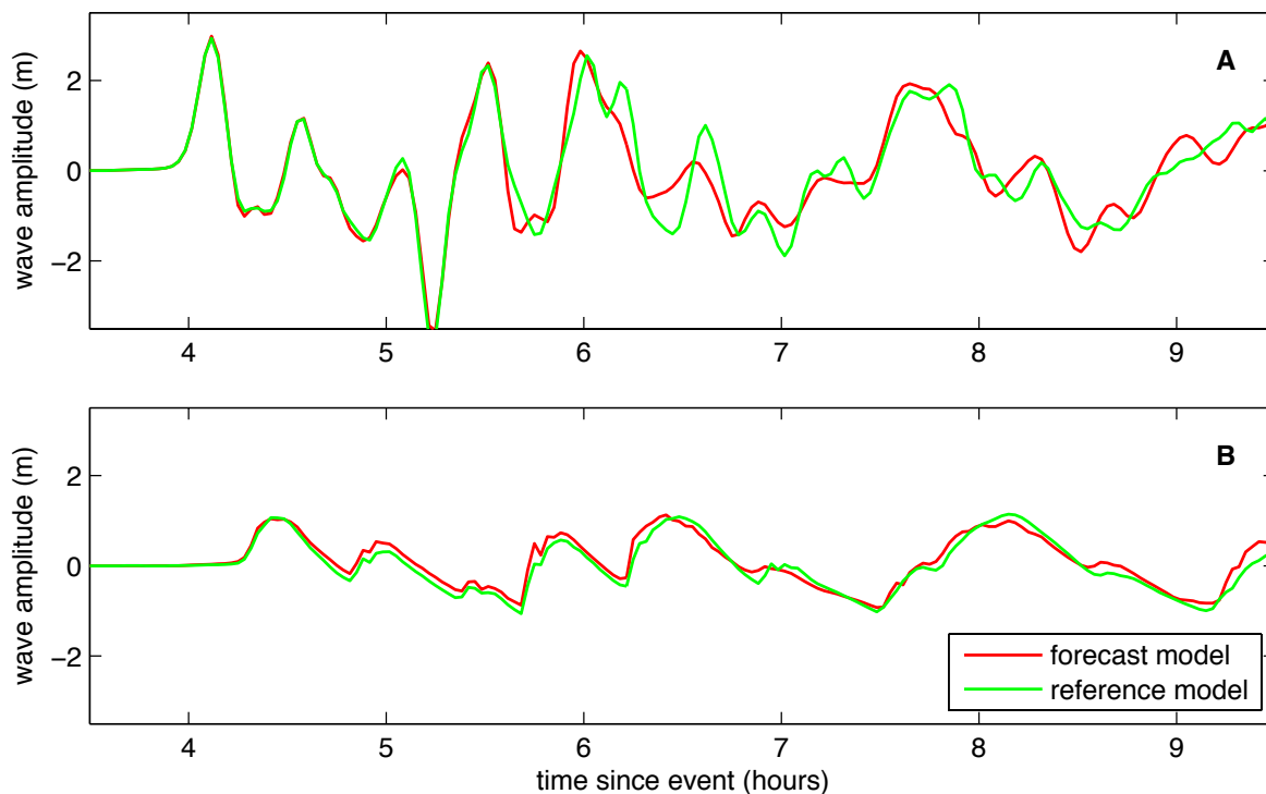
Figure 10 Model results for the 1964 Alaska Mw 9.2 event. The upper two panels show the forecast (left) and reference (right) model maximum wave height predictions. The lower panels show the forecast model (red) and reference model (green) wave amplitudes at the points labeled A and B in the forecast model wave height map.
