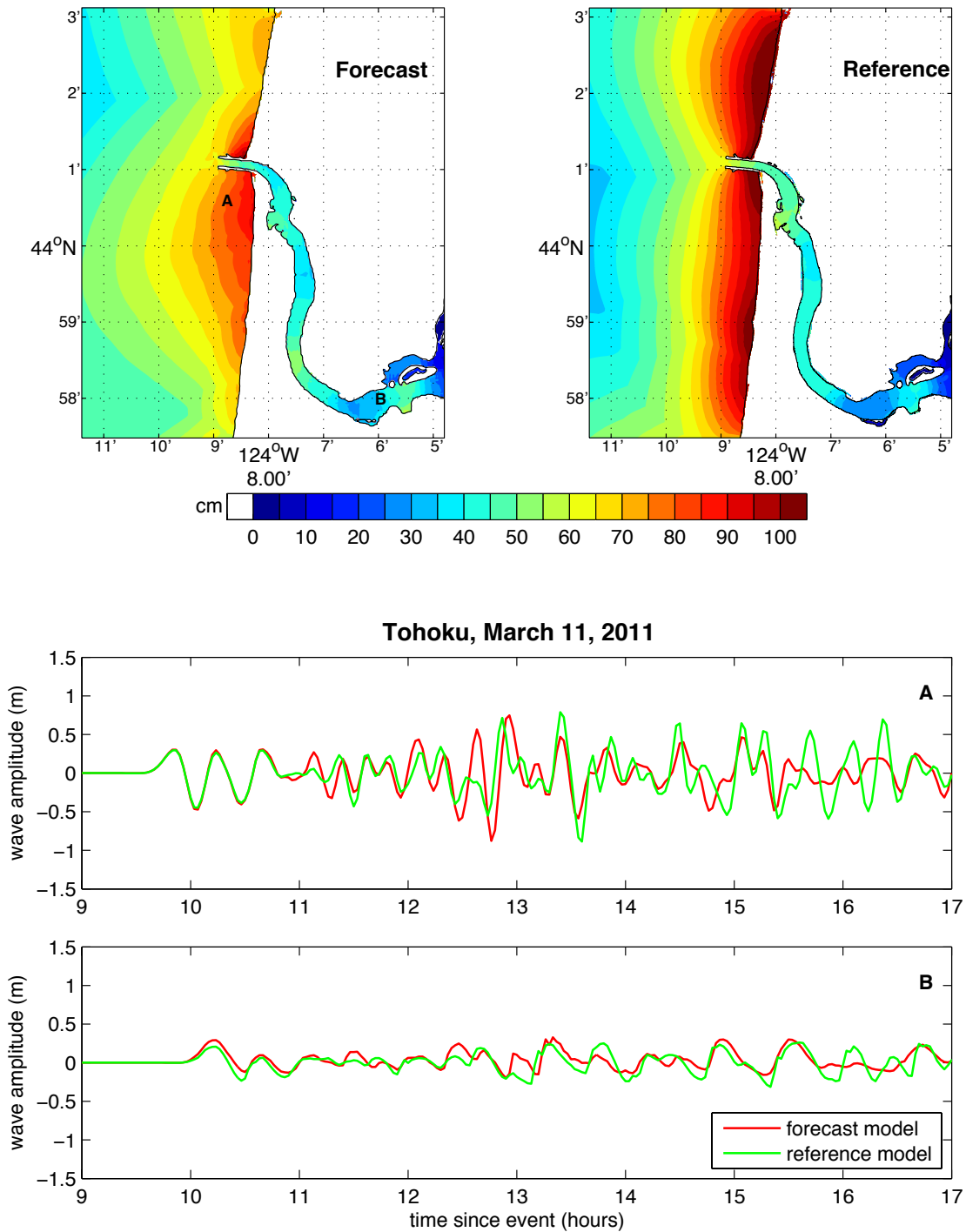
Figure 18 Model results for the 2011 Tohoku Mw 9.0 event. The upper two panels show, respectively, the forecast and reference model maximum wave height predictions. The upper two panels show the forecast (left) and reference (right) model maximum wave height predictions. The lower panels show the forecast model (red) and reference model (green) wave amplitudes at the points labeled A and B in the forecast model wave height map.
