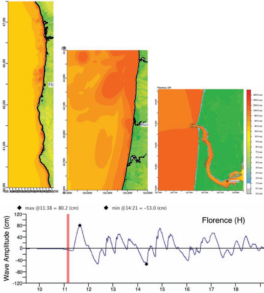
Figure 4: Response of the Florence forecast model to synthetic scenario NTSZ 30-39 ( \alpha=25 ). Maximum sea surface elevation for (a) A-grid, b) B-grid, c) C-grid. Sea surface elevation time series at the C-grid warning point .
