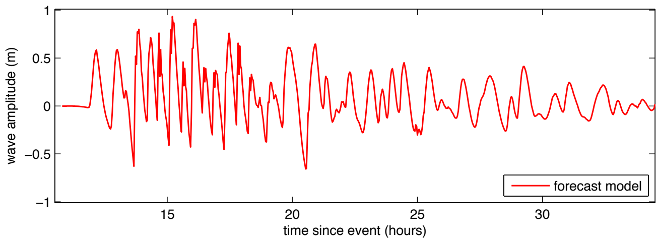
Figure 23 Results from the forecast model for the KISZ 56-65 synthetic event. The upper panel shows the map of predicted maximum wave height in the Florence C-grid and the lower panel shows the time series of wave amplitude at the warning point location.
