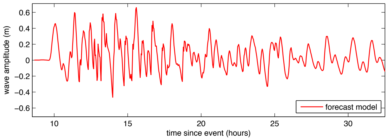
Figure 21 Results from the forecast model for the KISZ 22-31 synthetic event. The upper panel shows the map of predicted maximum wave height in the Florence C-grid and the lower panel shows the time series of wave amplitude at the warning point location.
