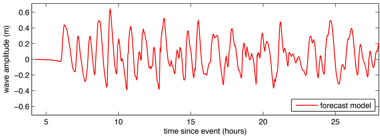
Figure 24 Results from the forecast model for the ACSZ 6-15 synthetic event. The upper panel shows the map of predicted maximum wave height in the Florence C-grid and the lower panel shows the time series of wave amplitude at the warning point location.
