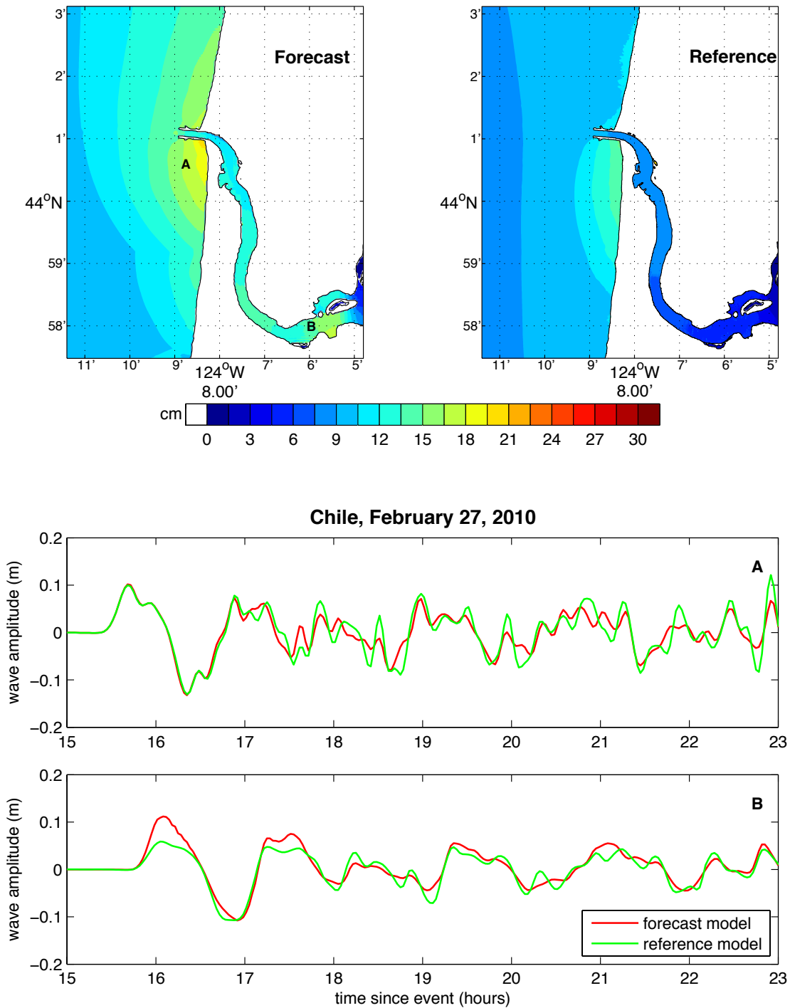
Figure 17 Model results for the 2010 Chile Mw 8.8 event. The upper two panels show, respectively, the forecast and reference model maximum wave height predictions. The upper two panels show the forecast (left) and reference (right) model maximum wave height predictions. The lower panels show the forecast model (red) and reference model (green) wave amplitudes at the points labeled A and B in the forecast model wave height map.
