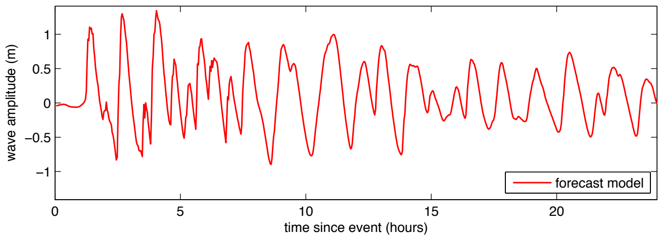
Figure 27 Results from the forecast model for the ACSZ 50-59 synthetic event. The upper panel shows the map of predicted maximum wave height in the Florence C-grid and the lower panel shows the time series of wave amplitude at the warning point location.
