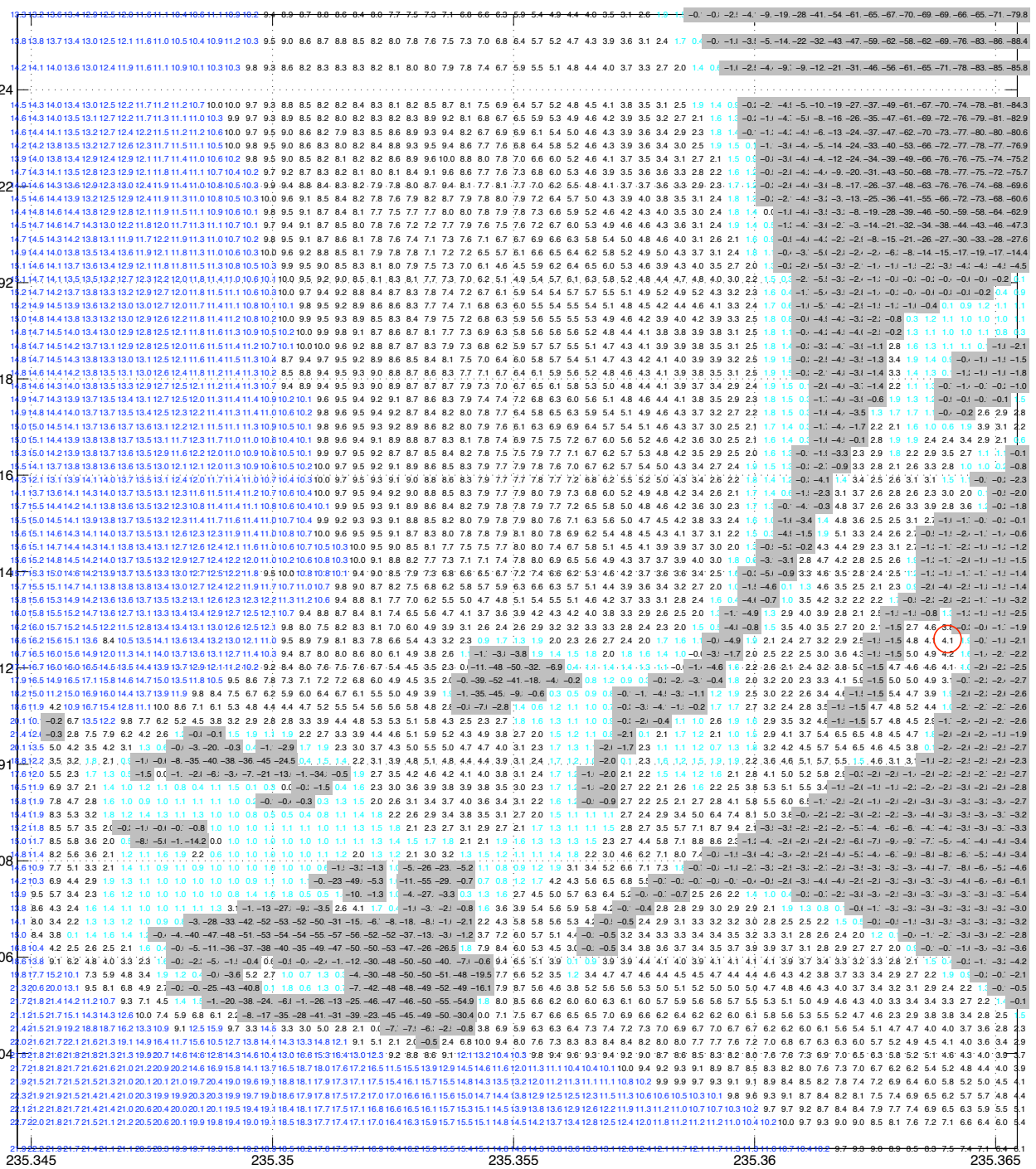
Figure 10 Water depth at each node at the La Push Harbor in the forecast C-grid. A 1'' resolution was applied to outside areas. The Harbor and river entrance were manually reconstructed based on the height of the 1/3'' DEM and adjusted to two-node wide. o, La Push tide gauge. Cyan, water depth less than 2m; blue, water depth > 10m.
