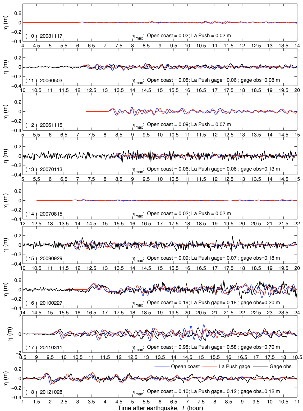
Figure 16 Time series of sea surface elevation \eta at open coast and La Push gage for the past tsunamis. Blue and red, forecast model; black, observations.
