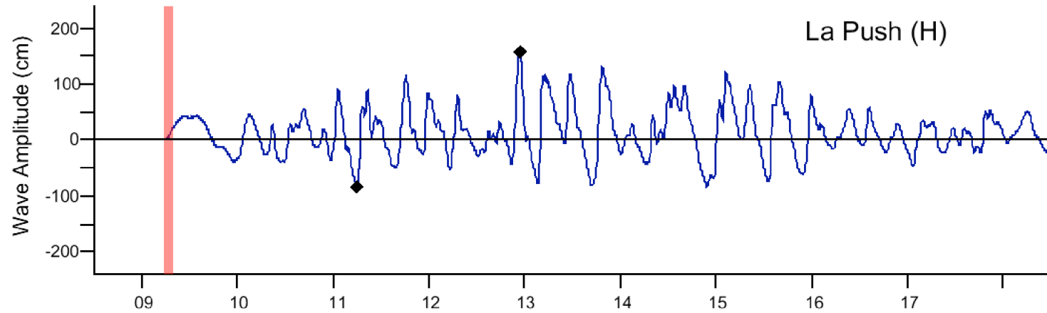
Figure C1: Response of the La Push forecast model to synthetic scenario KISZ 22-31 (alpha=29). Maximum sea surface elevation for (a) A-grid, b) B-grid, c) C-grid. Sea surface elevation time series at the C-grid warning point (d).
