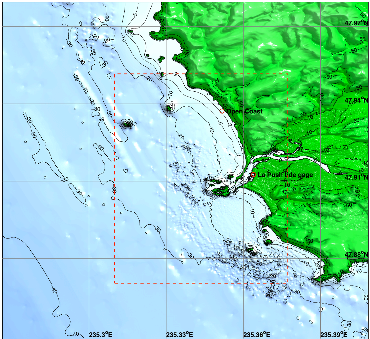
Figure 7 Grid setup for the La Push reference model. Grid resolutions are (a) 30", (b) 6" and (c) 1/3". O , Warning points at La Push tide station and the open coast; black rectangles, boundaries of nested reference grids; red dashed rectangles, boundaries of the forecast grids.
