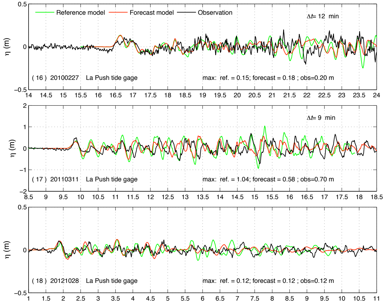
Figure 11 Tsunami amplitude time-series at La Push tide gage for past tsunamis. The green and red lines are model results from the La Push reference and forecast models respectively. The black lines are the observations. The model time series were shifted \Delta t min behind.
