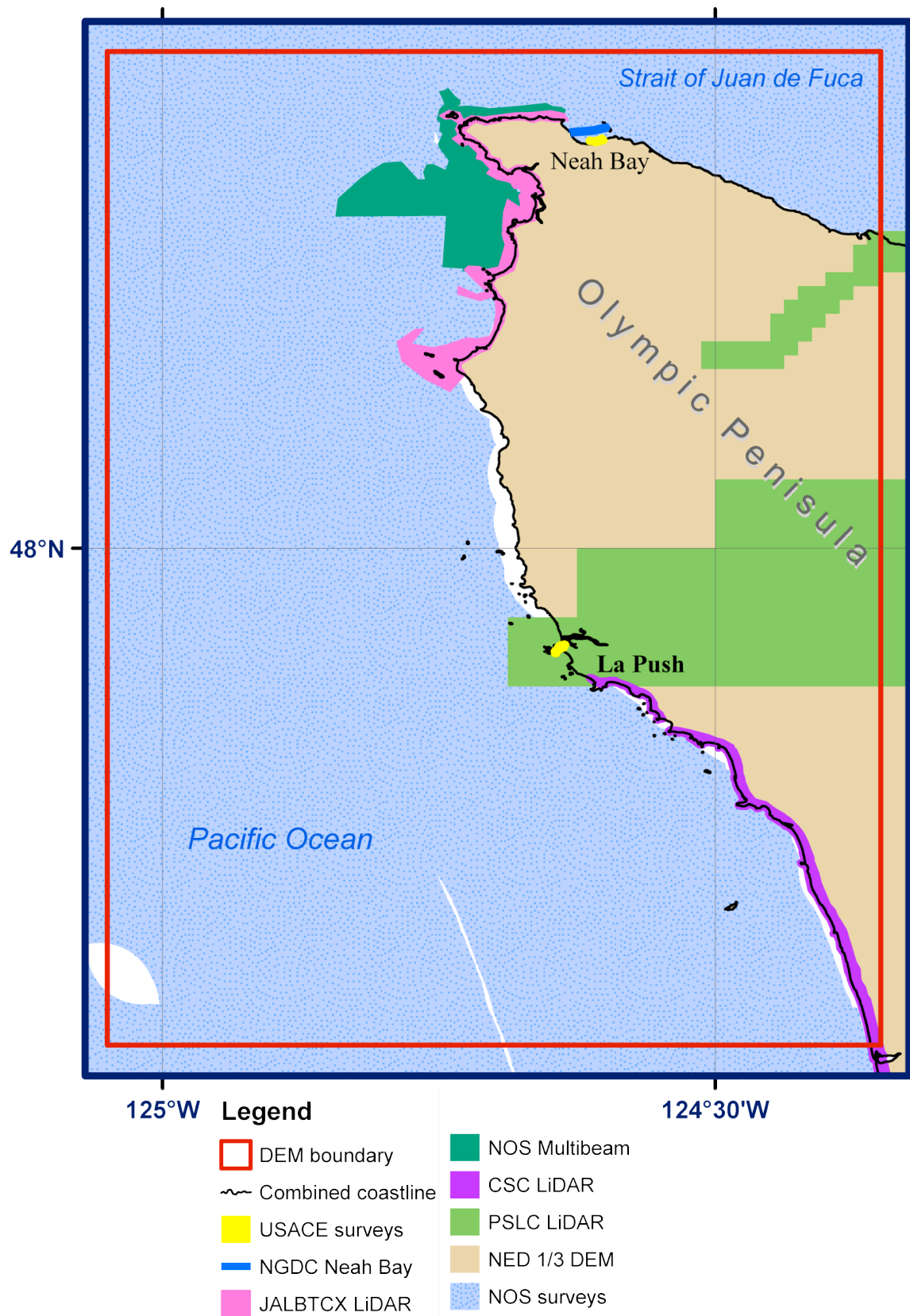
Figure 6 Bathymetric and topographic data source overview for the 1/3'' La Push DEM. The DEM was developed at NGDC (image courtesy of Tyler et al. (2009)).
