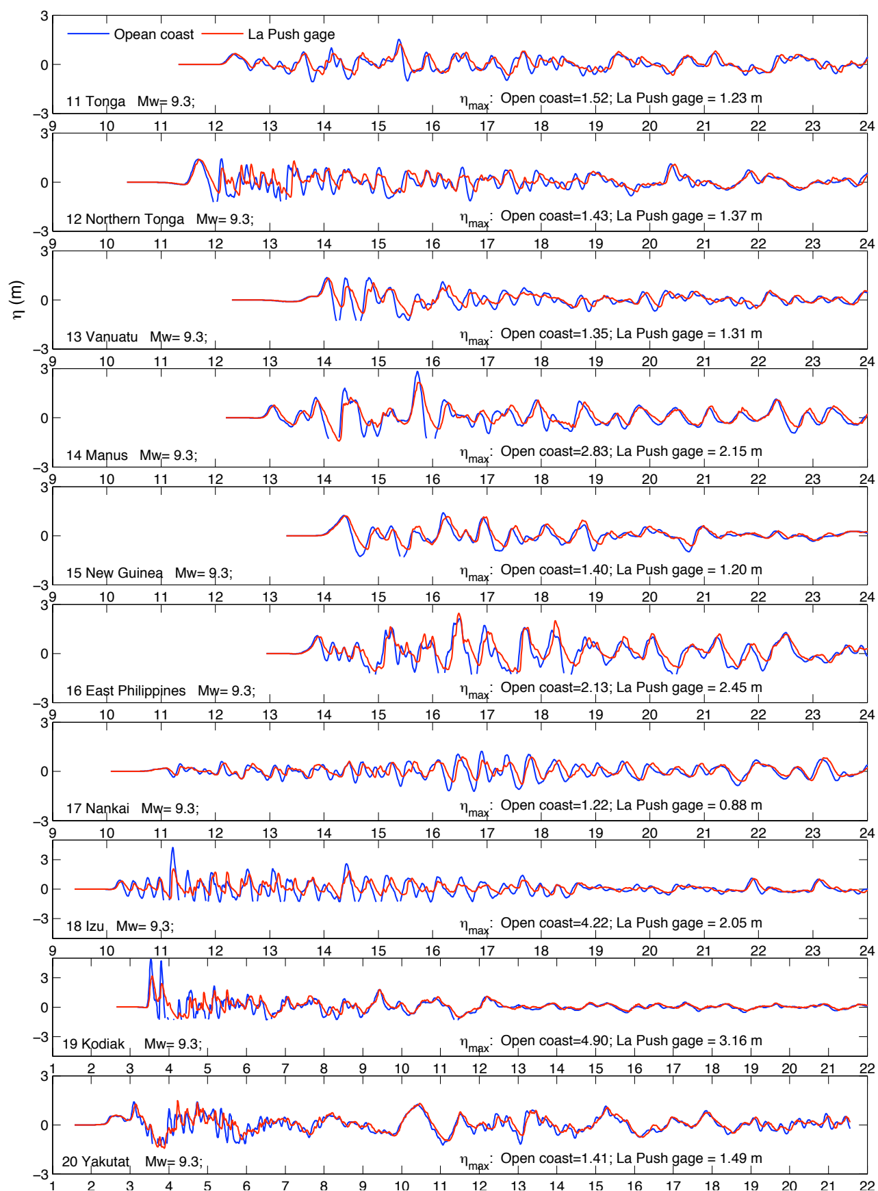
Figure 17 Time series of sea surface elevation \eta at open coast and La Push tide gage computed by the forecast model for the 20 simulated magnitude- 9.3 tsunamis.
