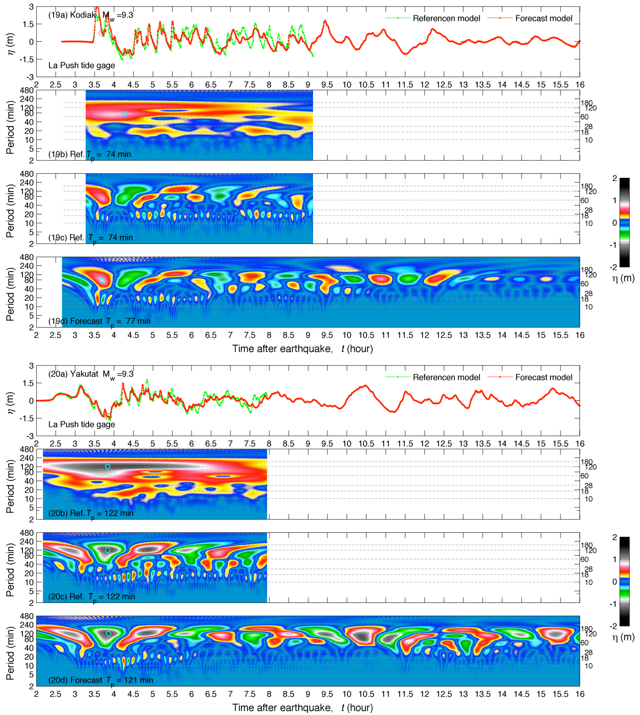
Figure 14 (a) Modeled \eta time series at La Push tide station for the 20 simulated magnitude-9.3 tsunamis. (b) Wavelet-derived amplitude spectrogram for the reference model. (c and d) Real part of the spectrograms computed by the reference and forecast models.
