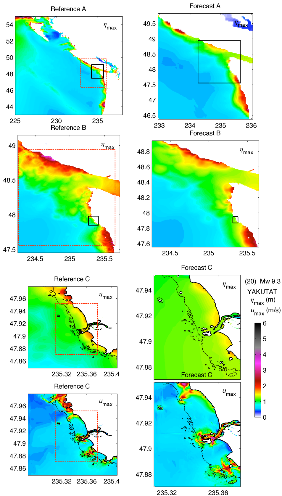
Figure 19 Maximum water elevation and current computed by the La Push reference and forecast models for the simulated magnitude-9.3 tsunamis.
