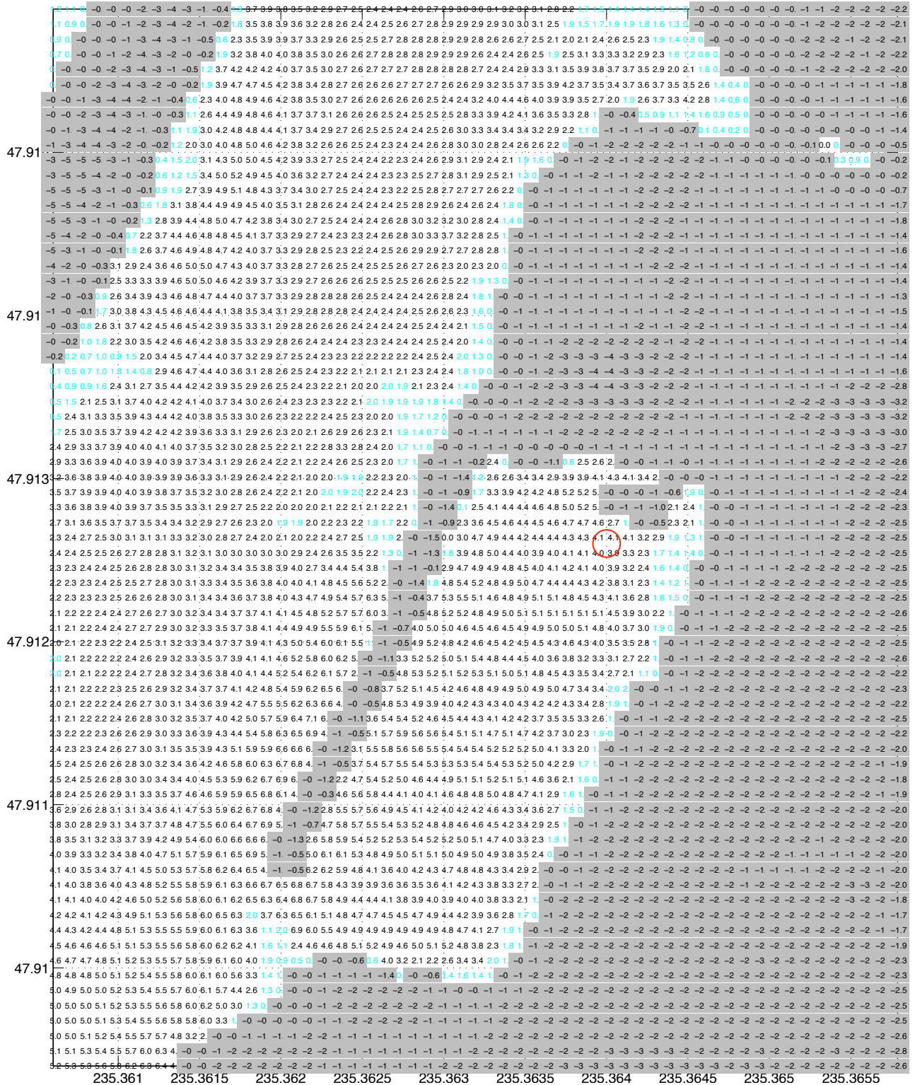
Figure 9 Water depth at each node at La Push Harbor in the reference C-grid (1/3" resolution). o, La Push tide gage. Cyan, water depth less than 2m; blue, water depth > 10m.
