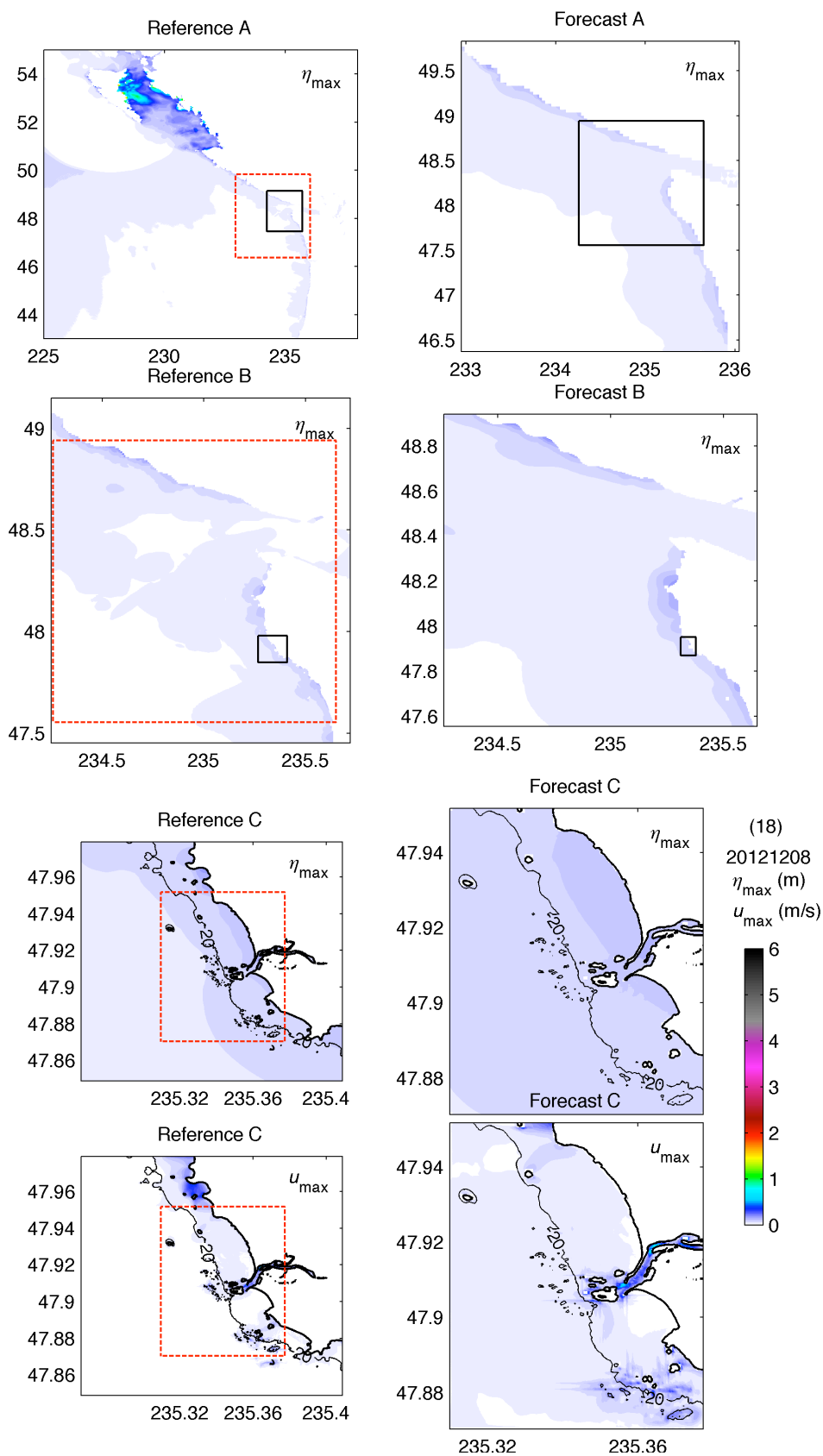
Figure 18 Maximum water elevation and current computed by the La Push reference and forecast models for past tsunamis.
