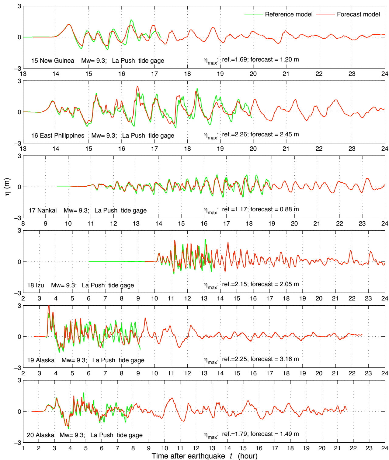
Figure 12 Tsunami amplitude time-series for the 20 simulated magnitude-9.3 tsunamis. The green and red lines are model results from the La Push reference and forecast models respectively.
