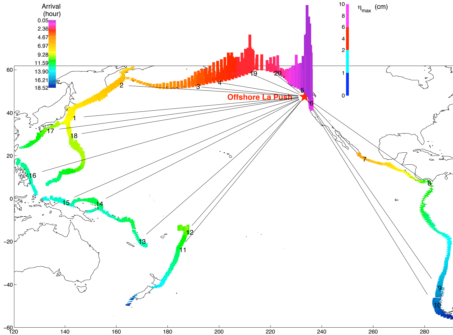
Figure 2 Maximum sea surface elevation ( \eta_{\max} ) offshore La push from 1129 magnitude-7.5 earthquakes. Data were taken from NCTR's pre-computed propagation database. Heights and colors of the bars represent \eta_{\max} and the first arrival at the offshore point (233.35°E, 47.501°N; water depth = 2324 m) respectively. 1-20, twenty simulated magnitude-9.3 tsunamis tested in this study.
