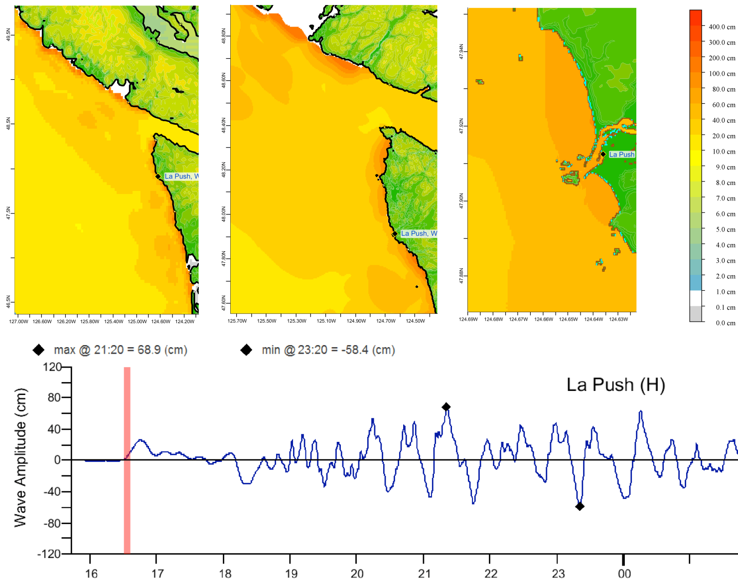
Figure C3: Response of the La Push forecast model to synthetic scenario CSSZ 92-101 ( \alpha=29 ). Maximum sea surface elevation for (a) A-grid, b) B-grid, c) C-grid. Sea surface elevation time series at the C-grid warning point (d).
