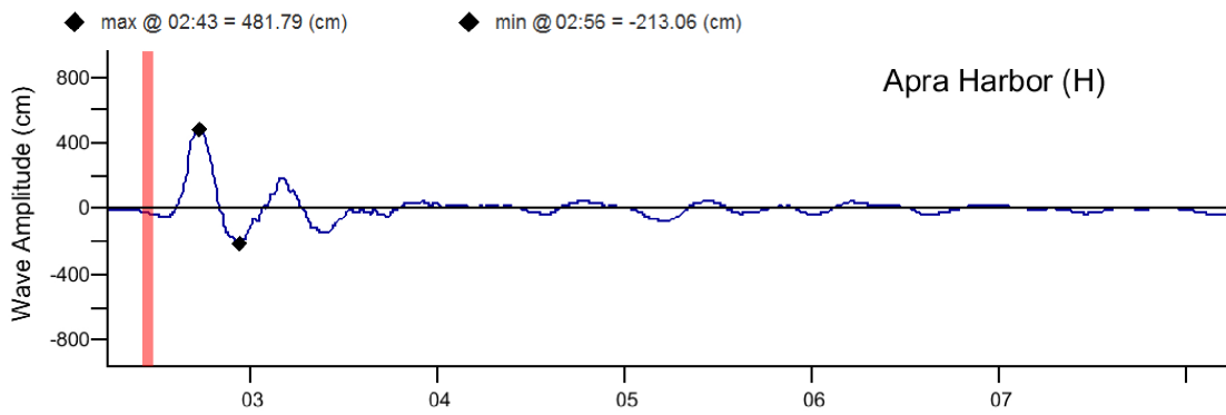
EPSZ6-15 scenario at Apra Harbor forecast model.
