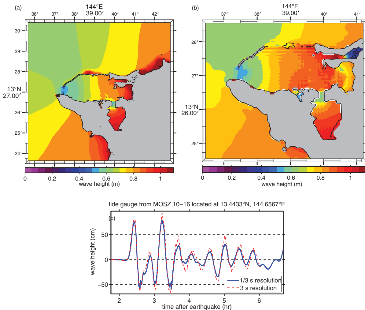
Figure 18: Magnitude 9.0 MOSZ source segment 10–16 synthetic scenario model results. (a) Maximum computed wave heights computed with reference model grids. (b) Maximum computed wave heights computed with forecast model grids. (c) Comparison of time series computed with reference model and forecast model grids at the Apra Harbor tide gauge.
