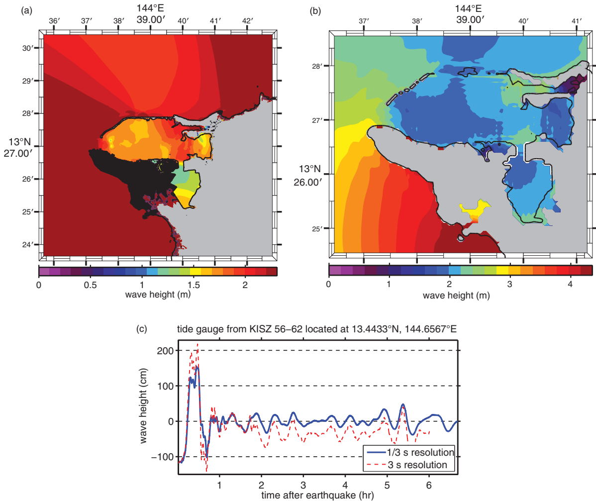
Figure 17: Magnitude 9.0 KISZ source segment 56–62 synthetic scenario model results. (a) Maximum computed wave heights computed with reference model grids. (b) Maximum computed wave heights computed with forecast model grids. (c) Comparison of time series computed with reference model and forecast model grids at the Apra Harbor tide gauge.
