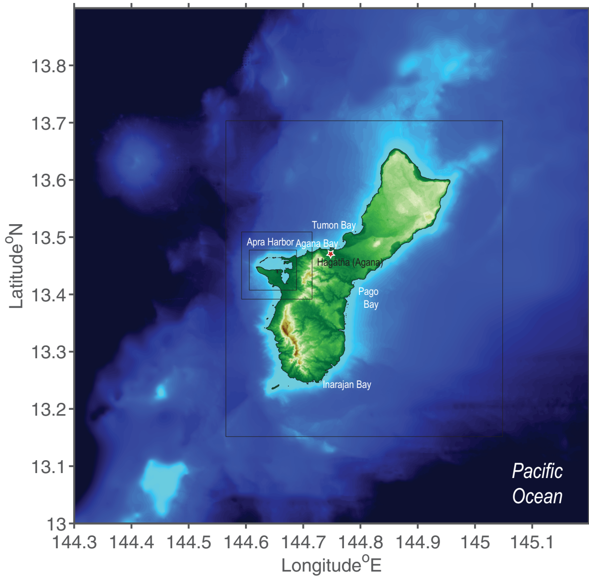
Figure 7: The three nested grids developed for the Apra Harbor tsunami forecast model. The largest rectangle denotes the extent of the outermost A-grid and the smallest rectangle denotes the extent of the innermost C-grid. Extent of the B-grid is denoted by the intermediate rectangle.
