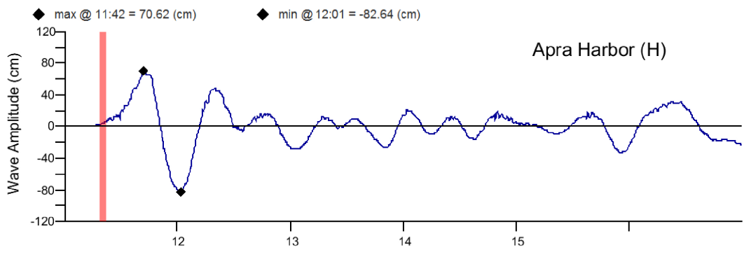
ACSZ56-65 scenario at Apra Harbor forecast model.
