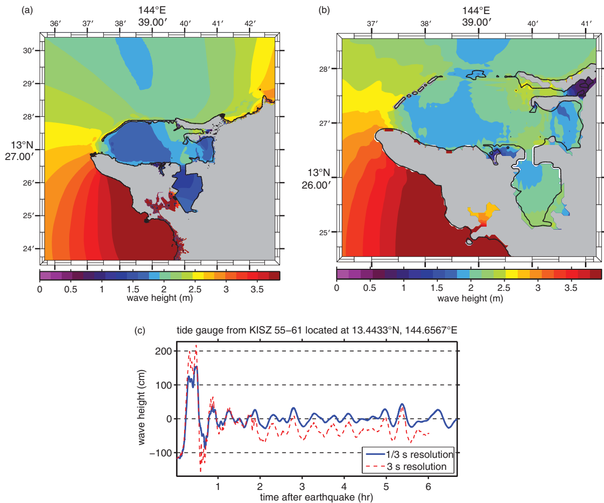
Figure 16: Magnitude 9.0 KISZ source segment 55–61 synthetic scenario model results. (a) Maximum computed wave heights computed with reference model grids. (b) Maximum computed wave heights computed with forecast model grids. (c) Comparison of time series computed with reference model and forecast model grids at the Apra Harbor tide gauge.
