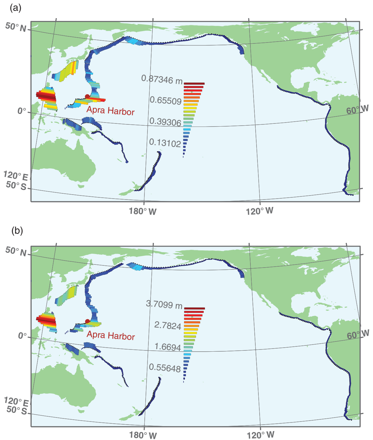
Figure 30: (a) Summary plot of the tsunami wave height response of Apra Harbor at the tide gauge from the 376 Mw 8.5 scenarios modeled to evaluate the sensitivity of the harbor to tsunamis generated by moderate earthquakes around the Pacific Ocean Basin. (b) Summary plot of the tsunami wave height response of Apra Harbor at the tide gauge from the 349 Mw 9.0 scenarios modeled to evaluate the sensitivity of the harbor to tsunamis generated by mega earthquakes around the Pacific Ocean Basin.
