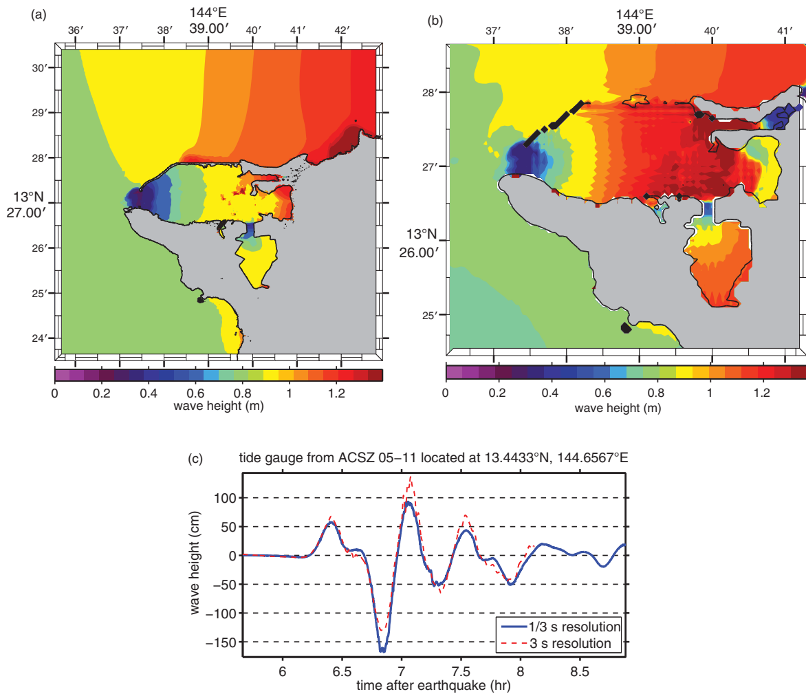
Figure 12: Magnitude 9.0 ACSZ source segment 05–11 synthetic scenario model results. (a) Maximum computed wave heights computed with reference model grids. (b) Maximum computed wave heights computed with forecast model grids. (c) Comparison of time series computed with reference model and forecast model grids at the Apra Harbor tide gauge.
