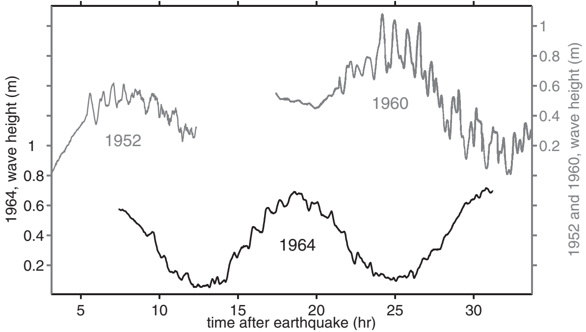
(b) 1952, 1960 and 1964 events at Apra Harbor, Guam (144.6567°E 13.4433°N).
