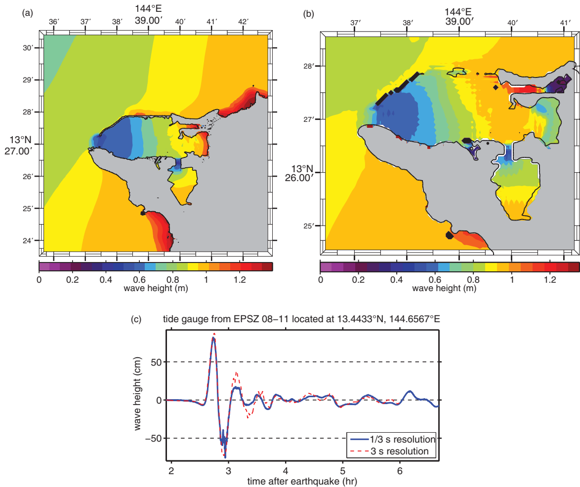
Figure 23: Magnitude 8.5 EPSZ source segment 08-11 synthetic scenario model results. (a) Maximum computed wave heights computed with reference model grids. (b) Maximum computed wave heights computed with forecast model grids. (c) Comparison of time series computed with reference model and forecast model grids at the Apra Harbor tide gauge.
