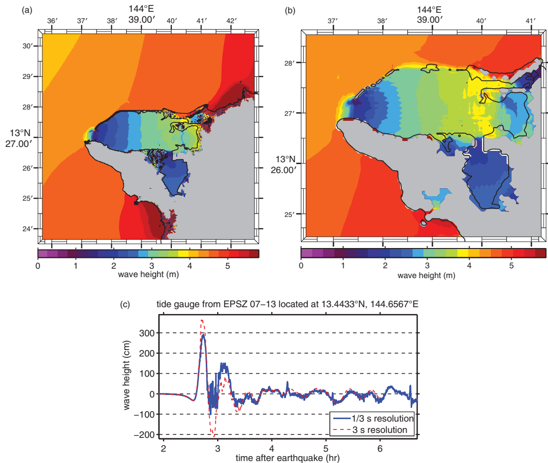
Figure 14: Magnitude 9.0 EPSZ source segment 07–13 synthetic scenario model results. (a) Maximum computed wave heights computed with reference model grids. (b) Maximum computed wave heights computed with forecast model grids. (c) Comparison of time series computed with reference model and forecast model grids at the Apra Harbor tide gauge.
