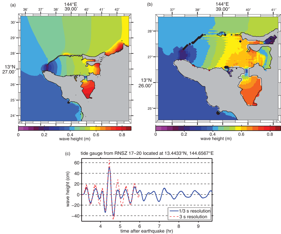
Figure 29: Magnitude 8.5 RNSZ source segment 17–20 synthetic scenario model results. (a) Maximum computed wave heights computed with reference model grids. (b) Maximum computed wave heights computed with forecast model grids. (c) Comparison of time series computed with reference model and forecast model grids at the Apra Harbor tide gauge.
