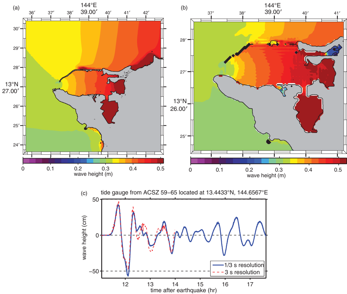
Figure 13: Magnitude 9.0 ACSZ source segment 59–65 synthetic scenario model results. (a) Maximum computed wave heights computed with reference model grids. (b) Maximum computed wave heights computed with forecast model grids. (c) Comparison of time series computed with reference model and forecast model grids at the Apra Harbor tide gauge.
