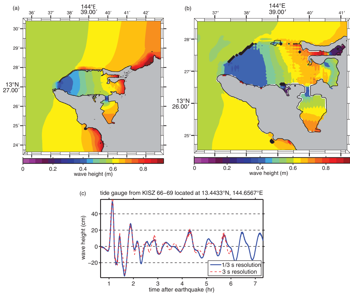
Figure 26: Magnitude 8.5 KISZ source segment 66–69 synthetic scenario model results. (a) Maximum computed wave heights computed with reference model grids. (b) Maximum computed wave heights computed with forecast model grids. (c) Comparison of time series computed with reference model and forecast model grids at the Apra Harbor tide gauge.
