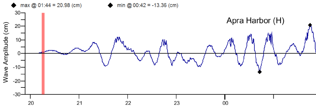
CSSZ89-98 scenario at Apra Harbor forecast model.
