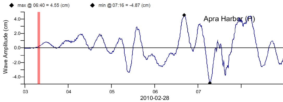
2010 Chile scenario at Apra Harbor forecast model.
