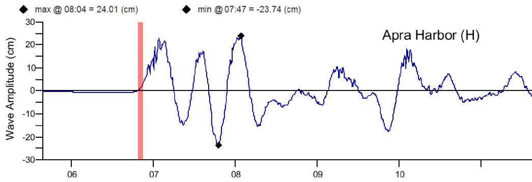
ACSZ16-325 scenario at Apra Harbor forecast model.
