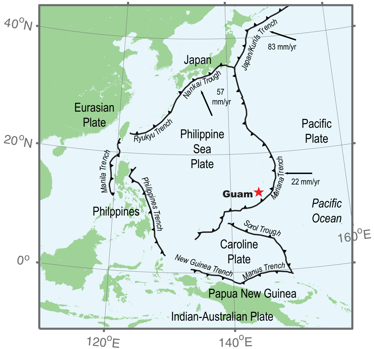
Figure 5: Regional setting showing the Island of Guam in relation to the Mariana Trench and surrounding tectonic plates and major specific subduction zones (Stein and Okal, 2007; Hall, 2002; 1997)
