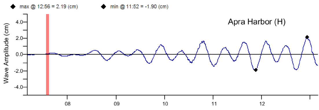
NTSZ B36 scenario at Apra Harbor forecast model.
