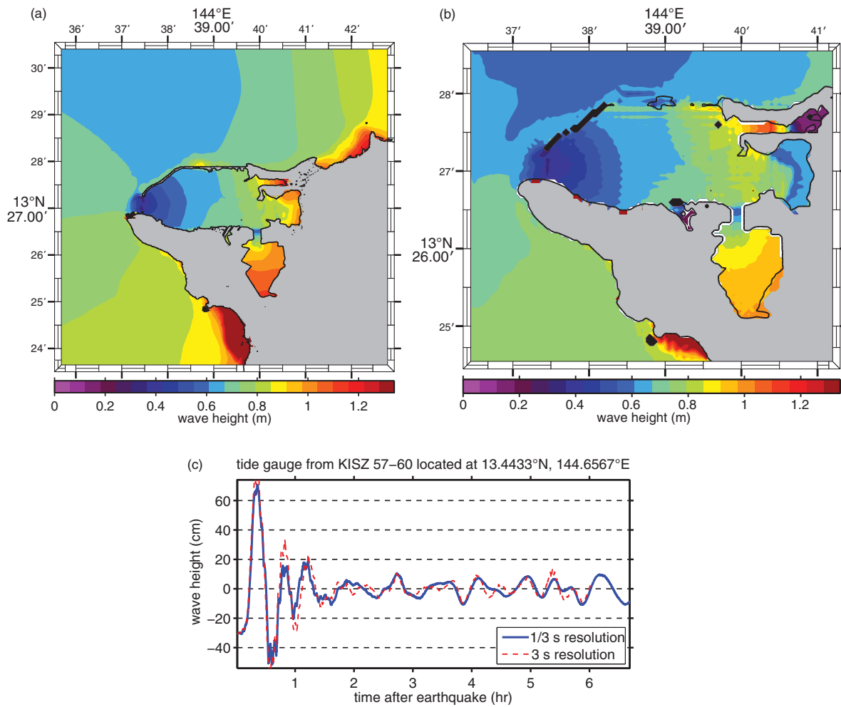
Figure 25: Magnitude 8.5 KISZ source segment 57–60 synthetic scenario model results. (a) Maximum computed wave heights computed with reference model grids. (b) Maximum computed wave heights computed with forecast model grids. (c) Comparison of time series computed with reference model and forecast model grids at the Apra Harbor tide gauge.
