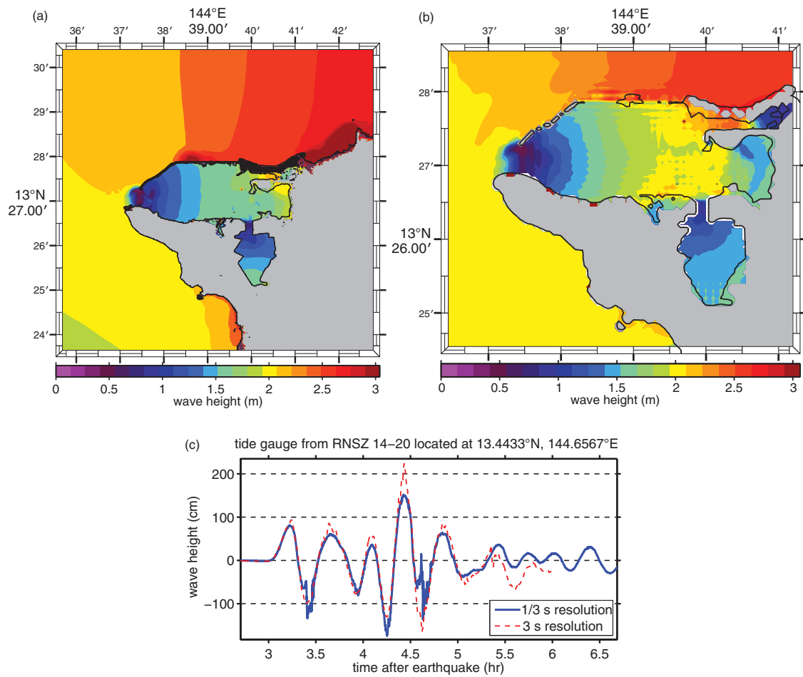
Figure 20: Magnitude 9.0 RNSZ source segment 14–20 synthetic scenario model results. (a) Maximum computed wave heights computed with reference model grids. (b) Maximum computed wave heights computed with forecast model grids. (c) Comparison of time series computed with reference model and forecast model grids at the Apra Harbor tide gauge.
