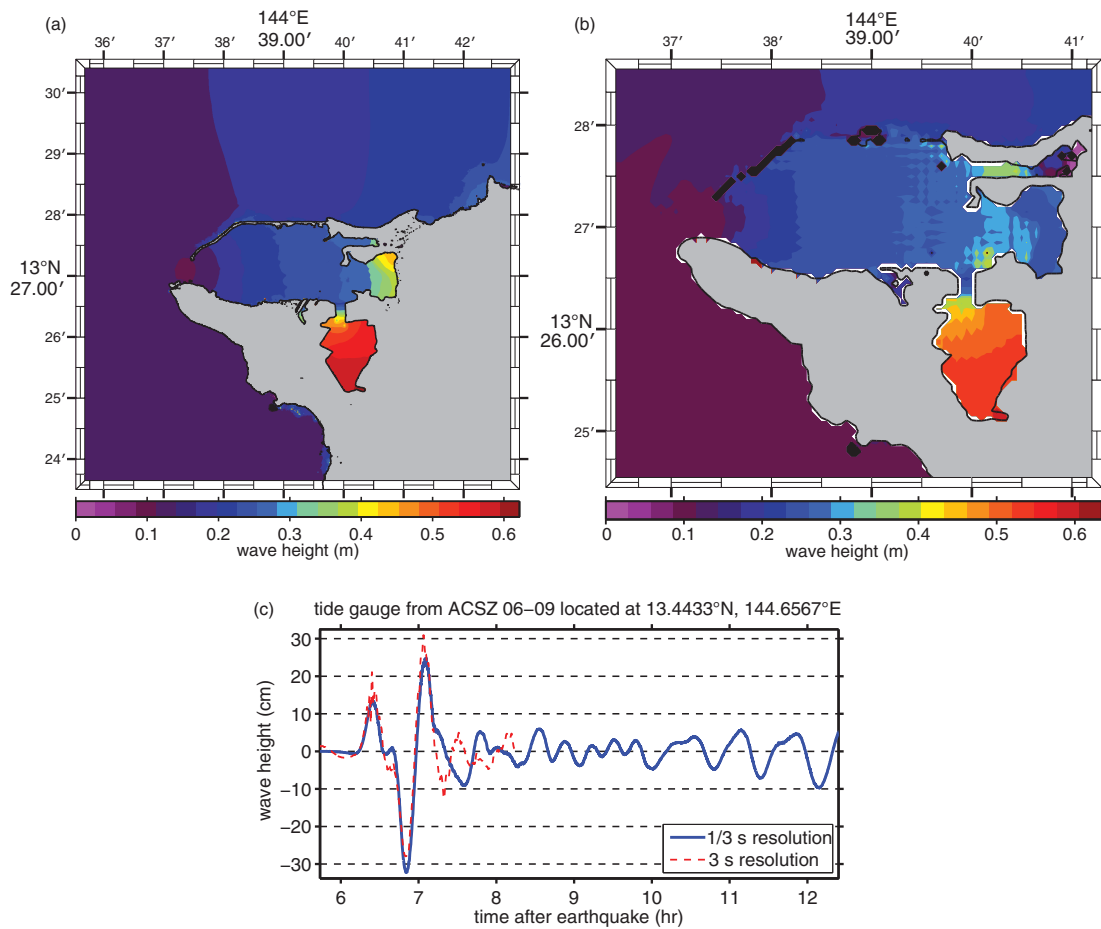
Figure 21: Magnitude 8.5 ACSZ source segment 06–09 synthetic scenario model results. (a) Maximum computed wave heights computed with reference model grids. (b) Maximum computed wave heights computed with forecast model grids. (c) Comparison of time series computed with reference model and forecast model grids at the Apra Harbor tide gauge.
