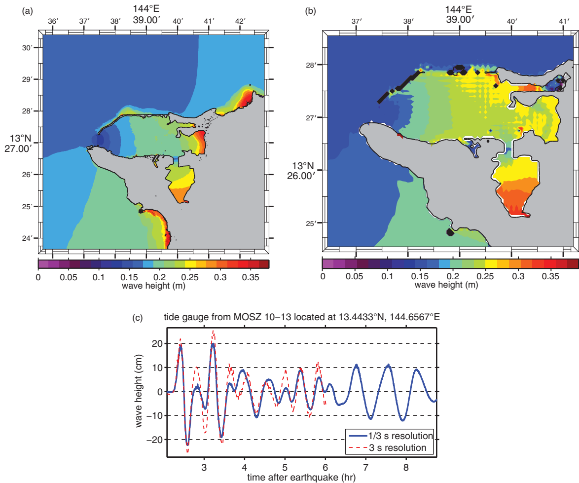
Figure 27: Magnitude 8.5 MOSZ source segment 10–13 synthetic scenario model results. (a) Maximum computed wave heights computed with reference model grids. (b) Maximum computed wave heights computed with forecast model grids. (c) Comparison of time series computed with reference model and forecast model grids at the Apra Harbor tide gauge.
