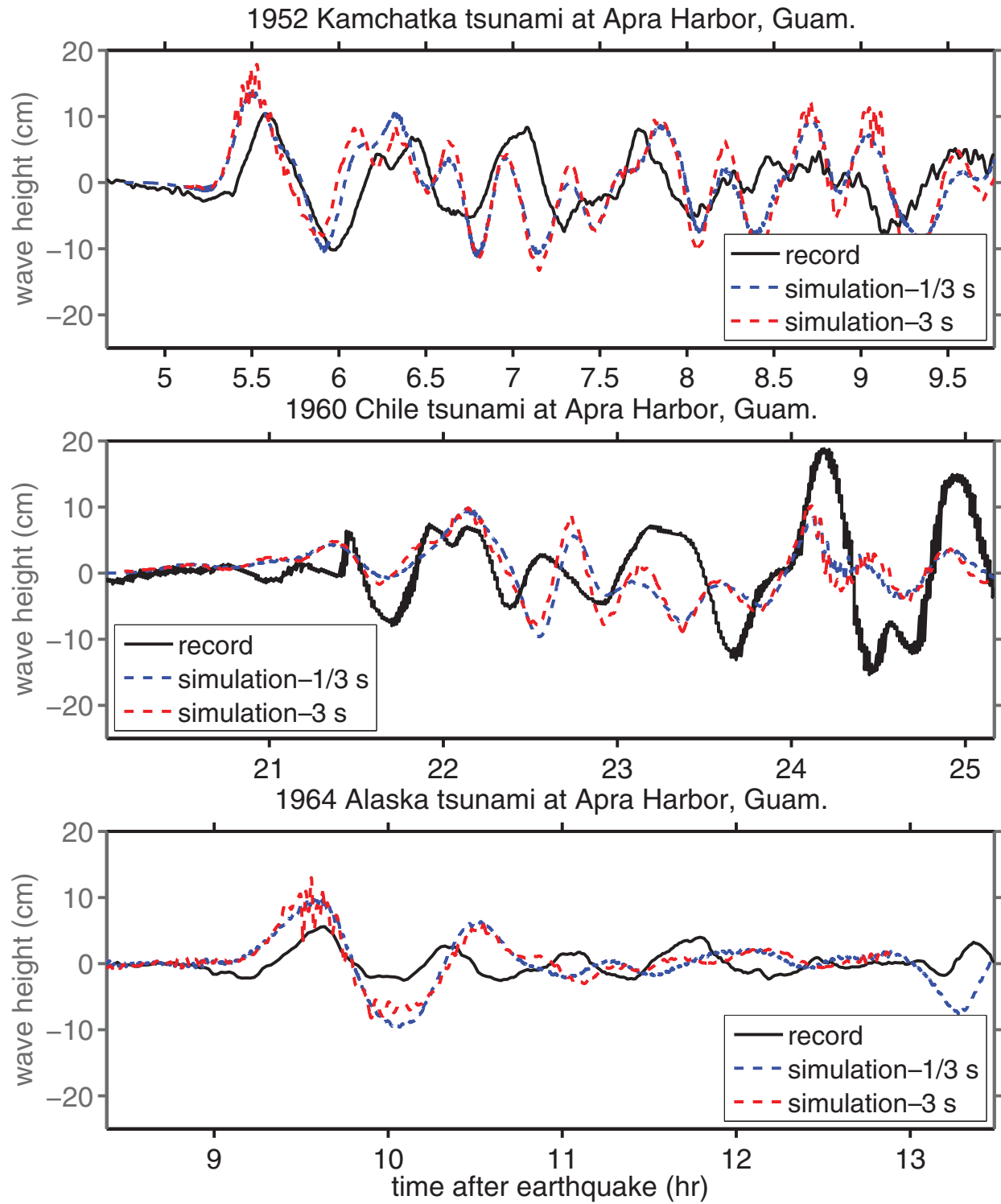
Figure 10: Comparison of computed time series with Apra Harbor tide gauge observations during the 1952 Kamchatka, 1960 Chile, and 1964 Alaska tsunamis.
