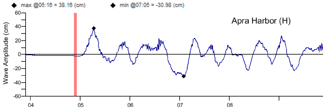
KISZ01-10 scenario at Apra Harbor forecast model.
