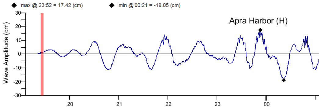
CSSZ102-111 scenario at Apra Harbor forecast model.
