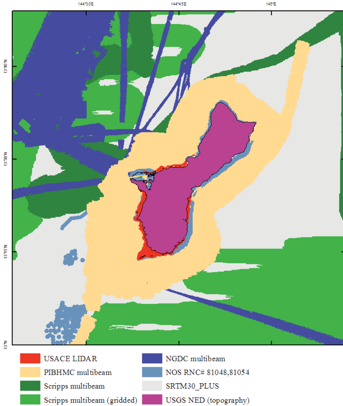
Figure 3: Data sources used for development of the Guam digital elevation model.
