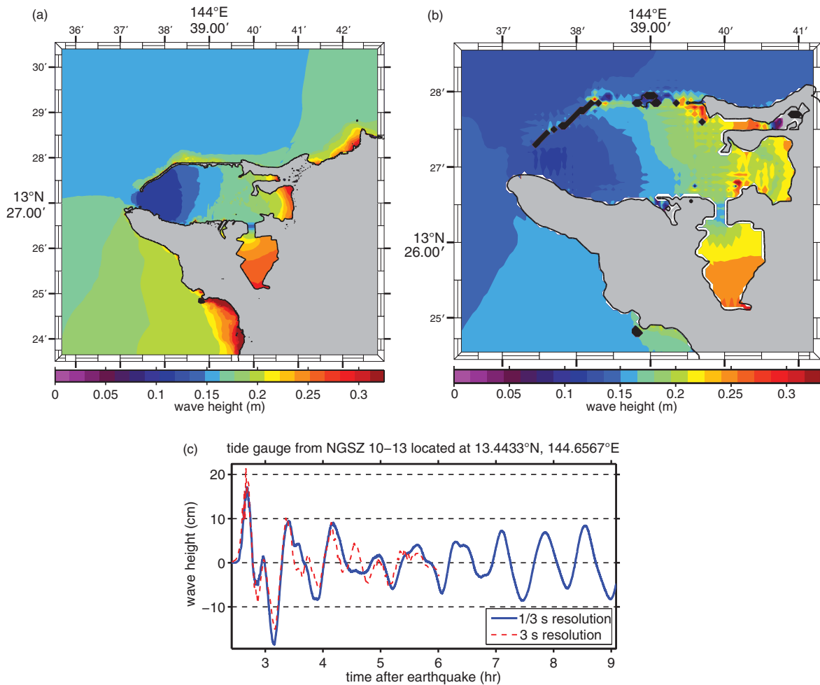
Figure 28: Magnitude 8.5 NGSZ source segment 10–13 synthetic scenario model results. (a) Maximum computed wave heights computed with reference model grids. (b) Maximum computed wave heights computed with forecast model grids. (c) Comparison of time series computed with reference model and forecast model grids at the Apra Harbor tide gauge.
