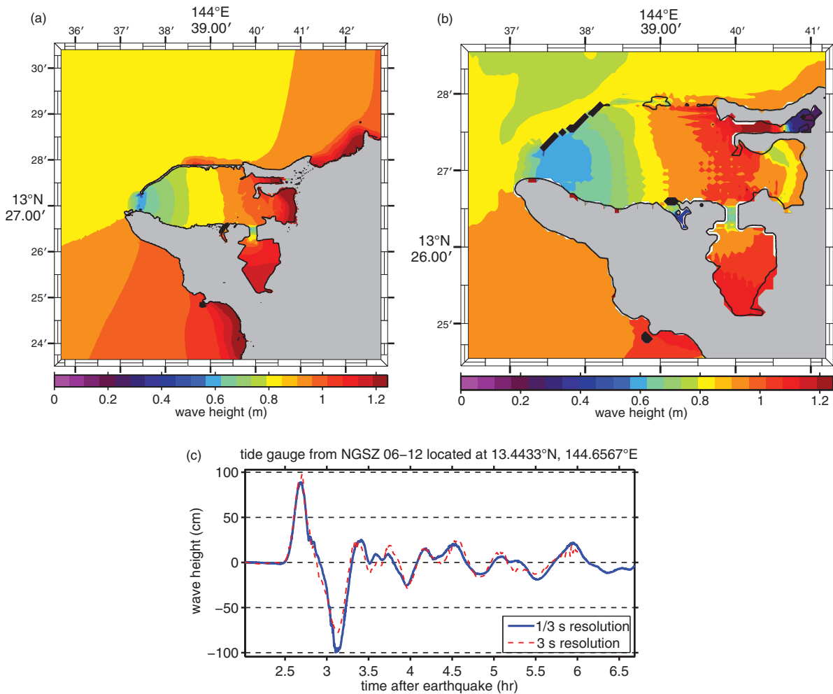
Figure 19: Magnitude 9.0 NGSZ source segment 06–12 synthetic scenario model results. (a) Maximum computed wave heights computed with reference model grids. (b) Maximum computed wave heights computed with forecast model grids. (c) Comparison of time series computed with reference model and forecast model grids at the Apra Harbor tide gauge.
