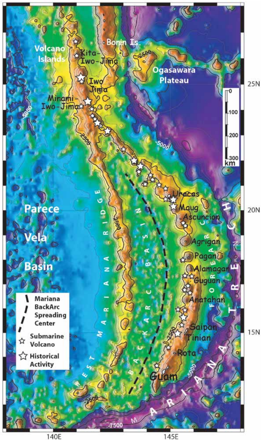
Figure 4: Satellite-derived bathymetry, from Smith and Sandwell (1997), of the Mariana Arc region. The southernmost island of Guam as well as other islands in the archipelago are labeled in black. Small white stars denote the location of submarine volcanoes. Bathymetric contour interval is 500 m. (National Oceanic and Atmospheric Administration/U.S. Department of Commerce, http://oceanexplorer.noaa.gov/explorations/03fire/logs/feb26/feb26.html )
