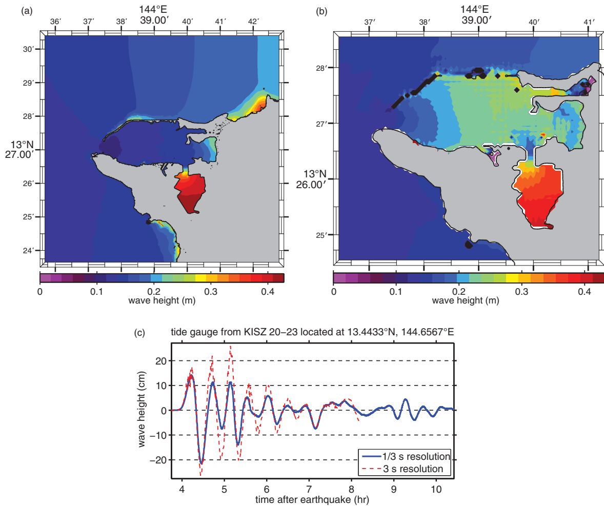
Figure 24: Magnitude 8.5 KISZ source segment 20–23 synthetic scenario model results. (a) Maximum computed wave heights computed with reference model grids. (b) Maximum computed wave heights computed with forecast model grids. (c) Comparison of time series computed with reference model and forecast model grids at the Apra Harbor tide gauge.
