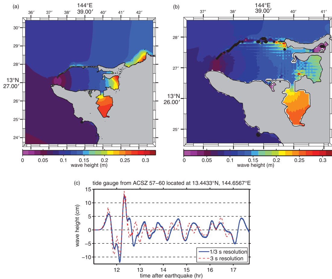
Figure 22: Magnitude 8.5 ACSZ source segment 57–60 synthetic scenario model results. (a) Maximum computed wave heights computed with reference model grids. (b) Maximum computed wave heights computed with forecast model grids. (c) Comparison of time series computed with reference model and forecast model grids at the Apra Harbor tide gauge.
