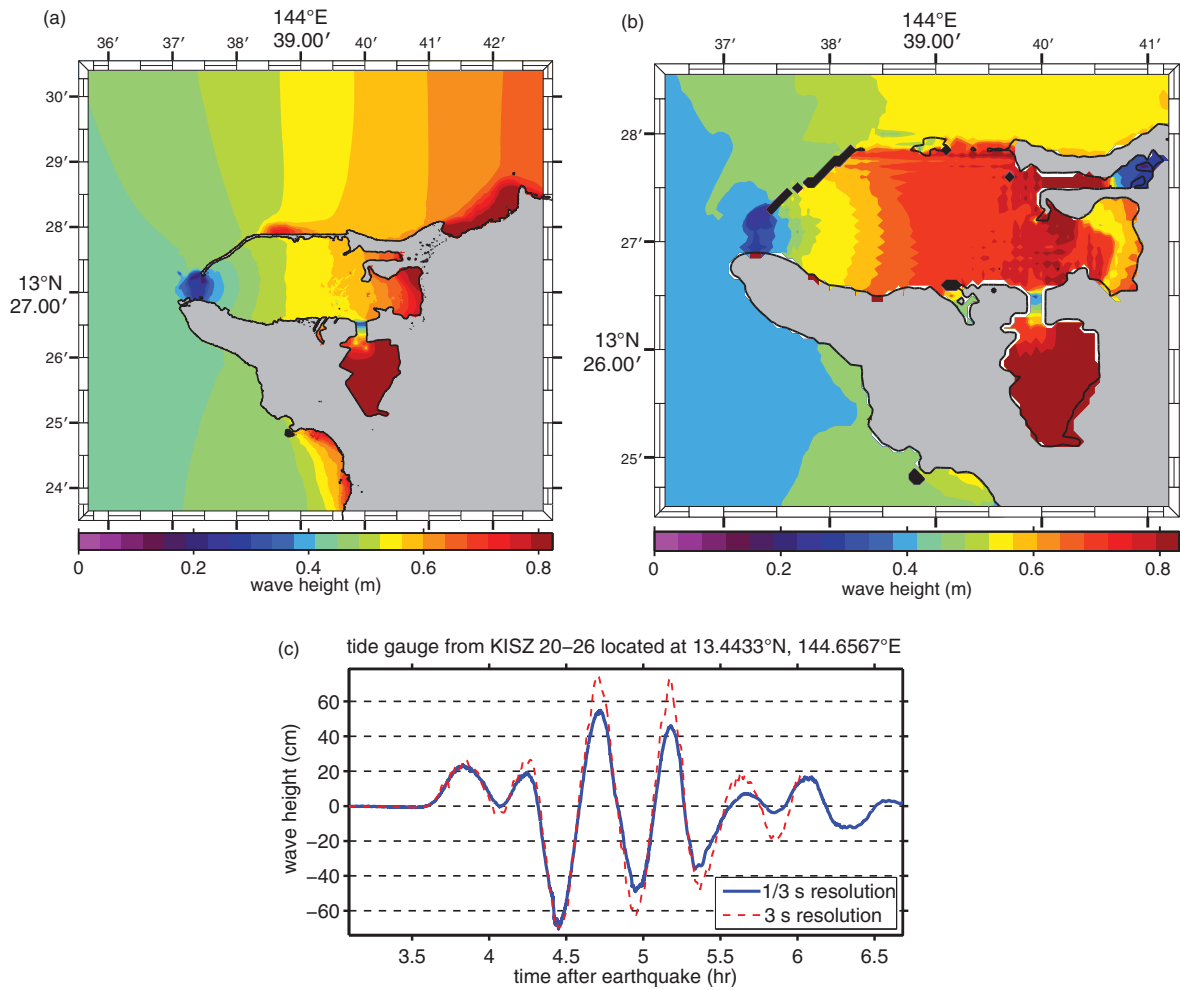
Figure 15: Magnitude 9.0 KISZ source segment 20–26 synthetic scenario model results. (a) Maximum computed wave heights computed with reference model grids. (b) Maximum computed wave heights computed with forecast model grids. (c) Comparison of time series computed with reference model and forecast model grids at the Apra Harbor tide gauge.
