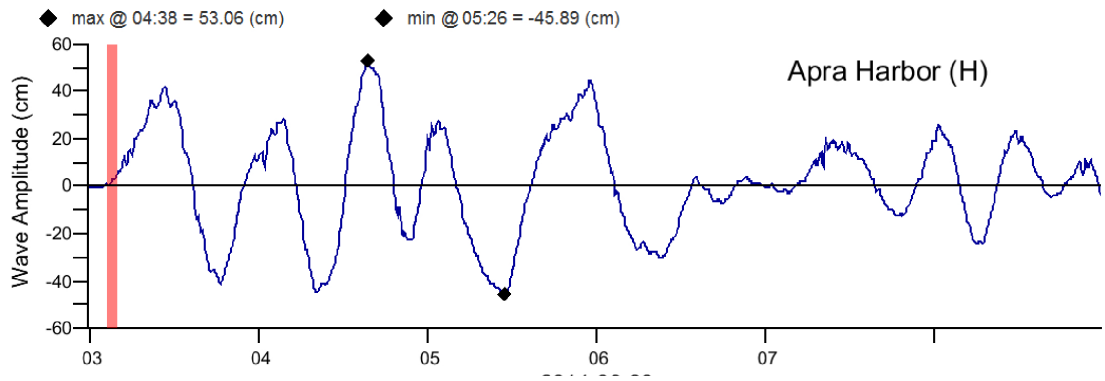
KISZ22-31 scenario at Apra Harbor forecast model.
