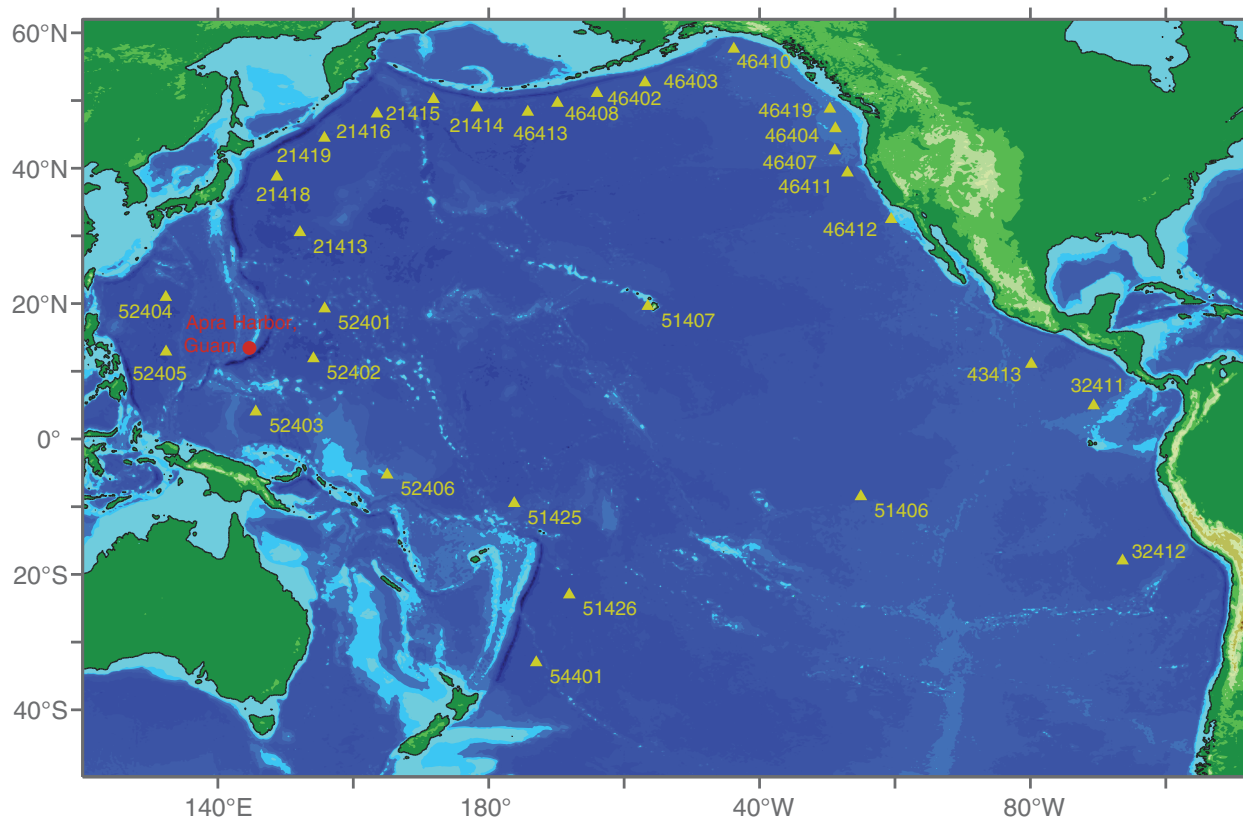
Figure 1: Pacific Ocean network of tsunameters.
