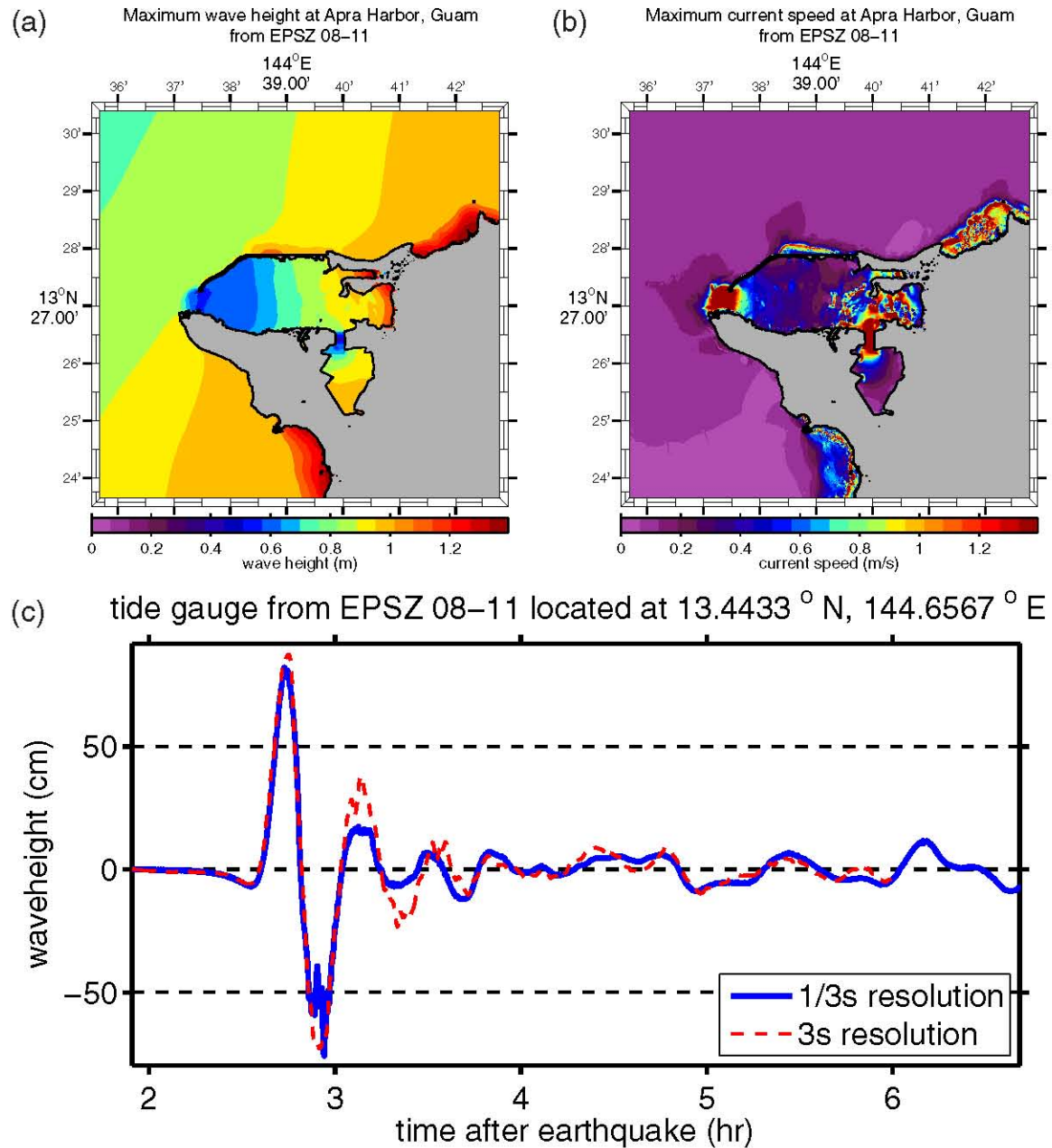
Figure D.4: (a) Maximum computed wave heights, (b) maximum computed currents, and (c) tsunami time history at the numerical tide gauge at Apra Harbor from a tsunami triggered by a M_w = 8.5 earthquake on EPSZ segments 08–11 by a 6-m slip.
