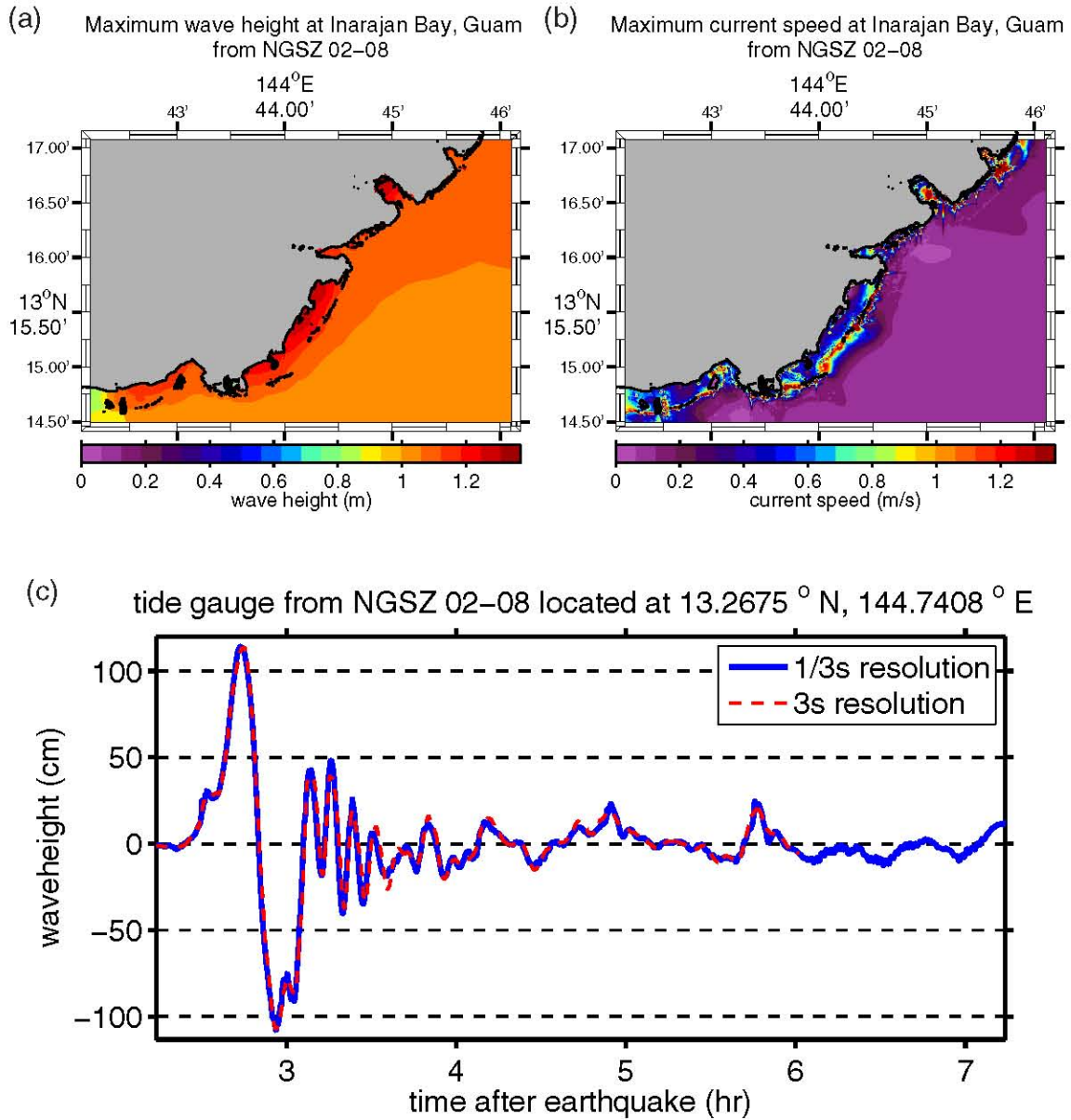
Figure G.17: (a) Maximum computed wave heights, (b) maximum computed currents, and (c) tsunami time history at the numerical tide gauge at Inarajan Bay from a tsunami triggered by a Mw = 9.0 earthquake on NGSZ segments 02–08 by a 20-m slip.
