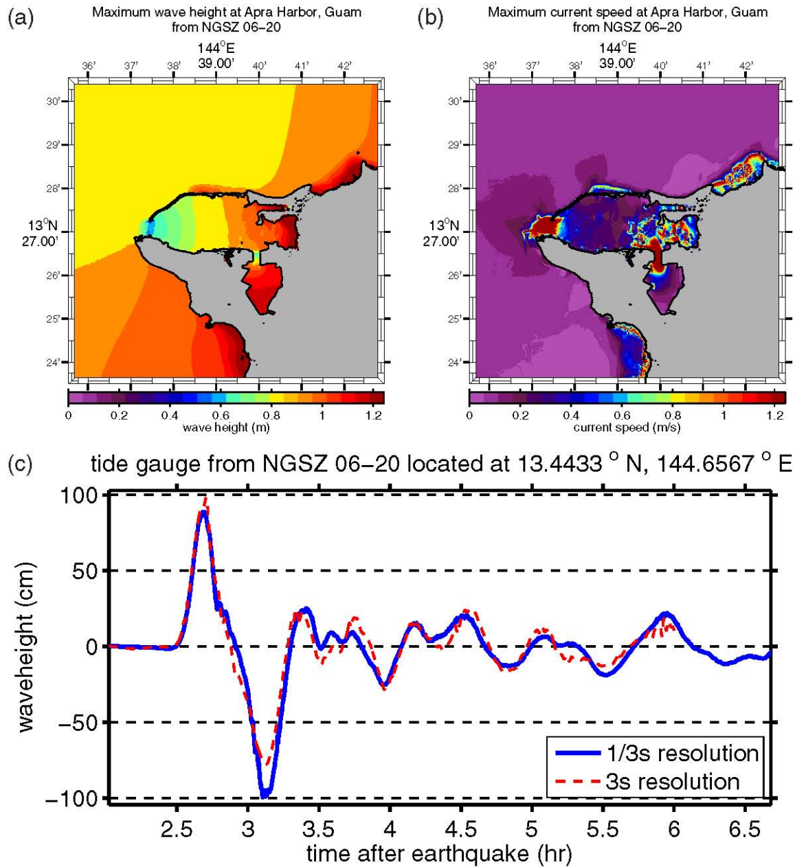
Figure D.17: (a) Maximum computed wave heights, (b) maximum computed currents, and (c) tsunami time history at the numerical tide gauge at Apra Harbor from a tsunami triggered by a Mw = 9.0 earthquake on NGSZ segments 06-20 by a 20-m slip.
