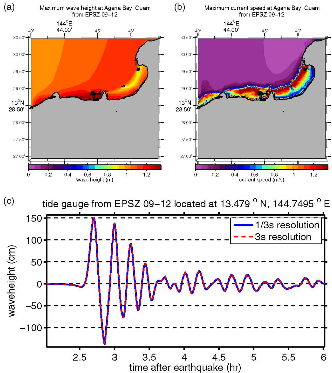
Figure F4: (a) Maximum computed wave heights, (b) maximum computed currents, and (c) tsunami time history at the numerical tide gauge at Agana Bay from a tsunami triggered by a M_w = 8.5 earthquake on EPSZ segments 09–12 by a 6-m slip.
