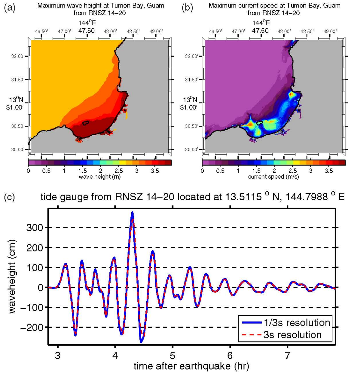
Figure C.18: (a) Maximum computed wave heights, (b) maximum computed currents, and (c) tsunami time history at the numerical tide gauge at Tumon Bay from a tsunami triggered by a M_w = 9.0 earthquake on RNSZ segments 14–20 by a 20-m slip.
