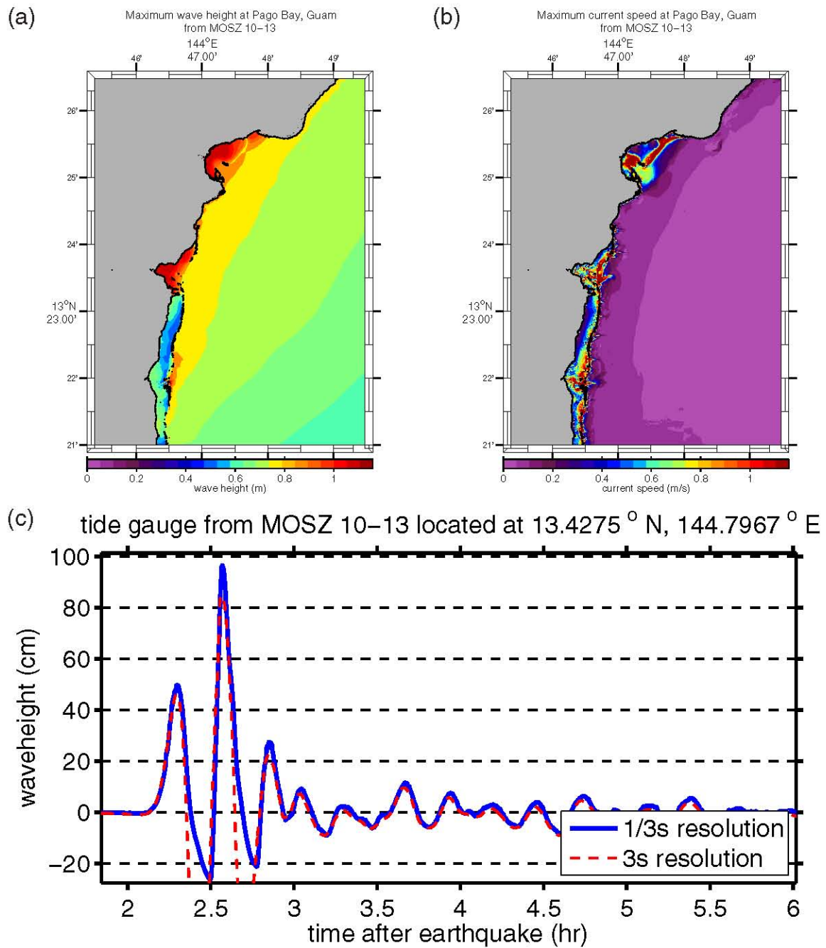
Figure E.7: (a) Maximum computed wave heights, (b) maximum computed currents, and (c) tsunami time history at the numerical tide gauge at Pago Bay from a tsunami triggered by a Mw = 8.5 earthquake on MOSZ segments 10–13 by a 6-m slip.
