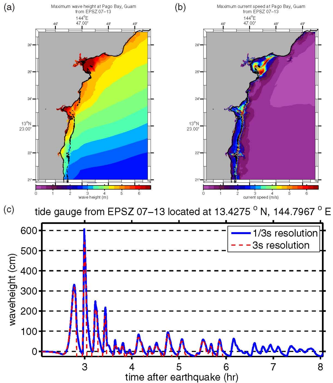
Figure E.12: (a) Maximum computed wave heights, (b) maximum computed currents, and (c) tsunami time history at the numerical tide gauge at Pago Bay from a tsunami triggered by a M_w = 9.0 earthquake on EPSZ segments 07–13 by a 20-m slip.
