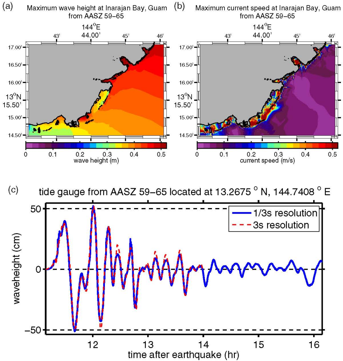
Figure G.11: (a) Maximum computed wave heights, (b) maximum computed currents, and (c) tsunami time history at the numerical tide gauge at Inarajan Bay from a tsunami triggered by a Mw = 9.0 earthquake on AASZ segments 59–65 by a 20-m slip.
