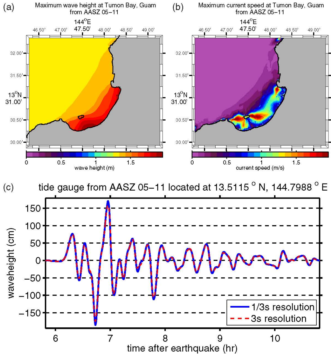
Figure C.11: (a) Maximum computed wave heights, (b) maximum computed currents, and (c) tsunami time history at the numerical tide gauge at Tumon Bay from a tsunami triggered by a Mw = 9.0 earthquake on AASZ segments 05–11 by a 20-m slip.
