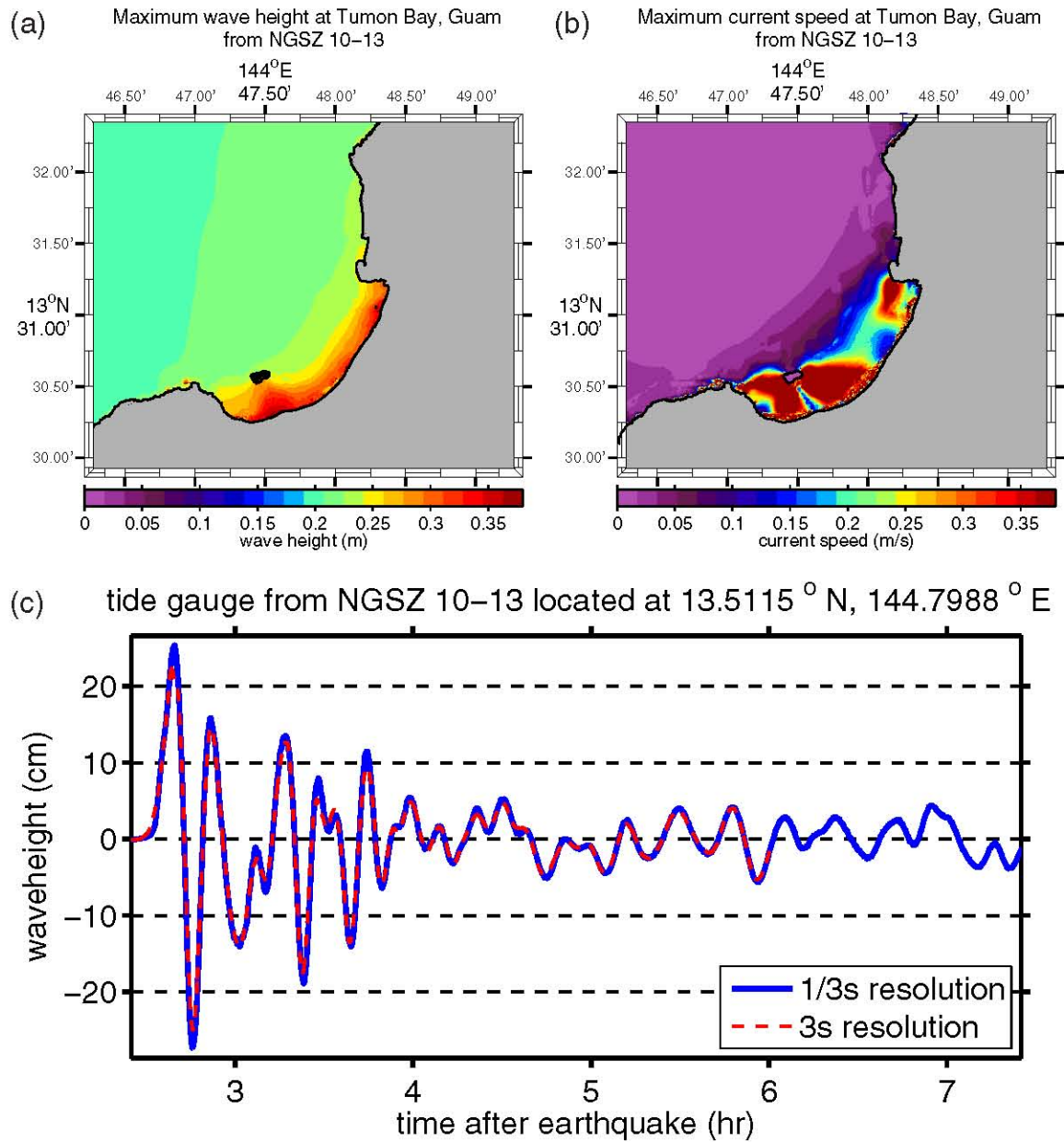
Figure C.9: (a) Maximum computed wave heights, (b) maximum computed currents, and (c) tsunami time history at the numerical tide gauge at Tumon Bay from a tsunami triggered by a Mw = 8.5 earthquake on NGSZ segments 10–13 by a 6-m slip.
