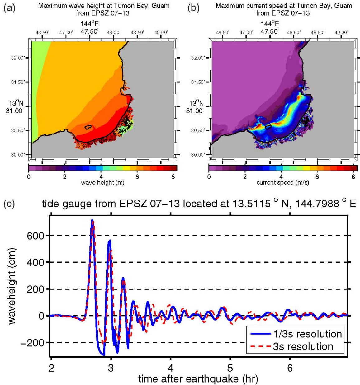
Figure C.13: (a) Maximum computed wave heights, (b) maximum computed currents, and (c) tsunami time history at the numerical tide gauge at Tumon Bay from a tsunami triggered by a Mw = 9.0 earthquake on EPSZ segments 07–13 by a 20-m slip.
