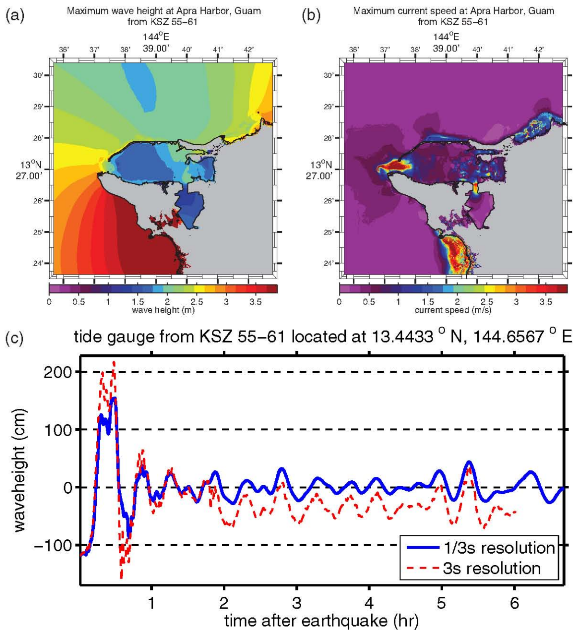
Figure D.14: (a) Maximum computed wave heights, (b) maximum computed currents, and (c) tsunami time history at the numerical tide gauge at Apra Harbor from a tsunami triggered by a M_w = 9.0 earthquake on KSZ segments 55–61 by a 20-m slip.
