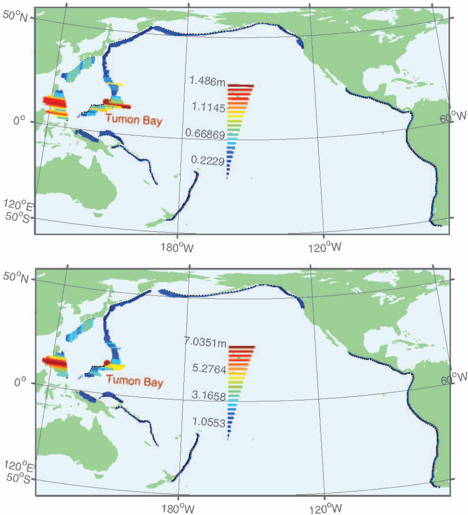
Figure 4.1: Tsunami wave height response at Tumon Bay from tsunamis triggered by (a) Mw = 8.5 and (b) Mw = 9.0 earthquakes.
