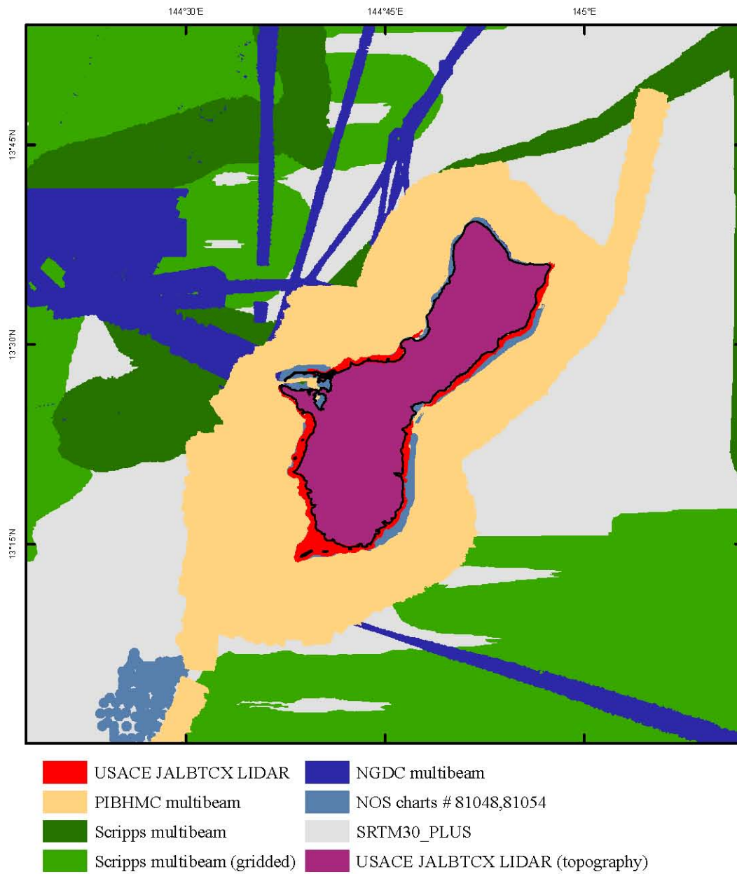
Figure 3.1: Data sources used for development of the Guam digital elevation model.
