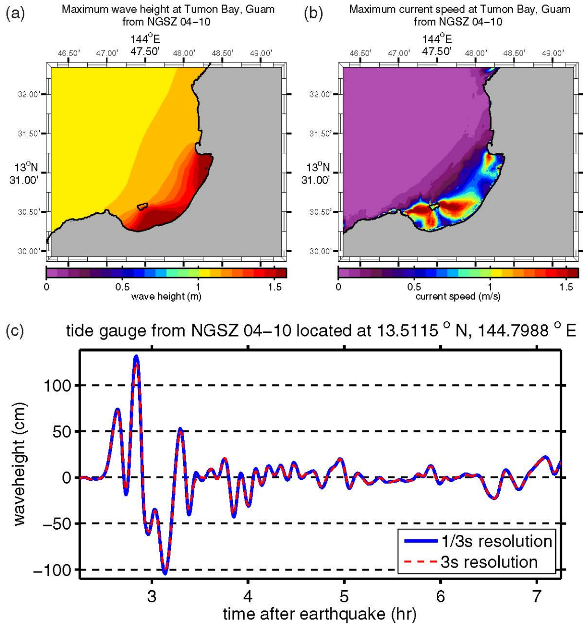
Figure C.17: (a) Maximum computed wave heights, (b) maximum computed currents, and (c) tsunami time history at the numerical tide gauge at Tumon Bay from a tsunami triggered by a Mw = 9.0 earthquake on NGSZ segments 04–10 by a 20-m slip.
