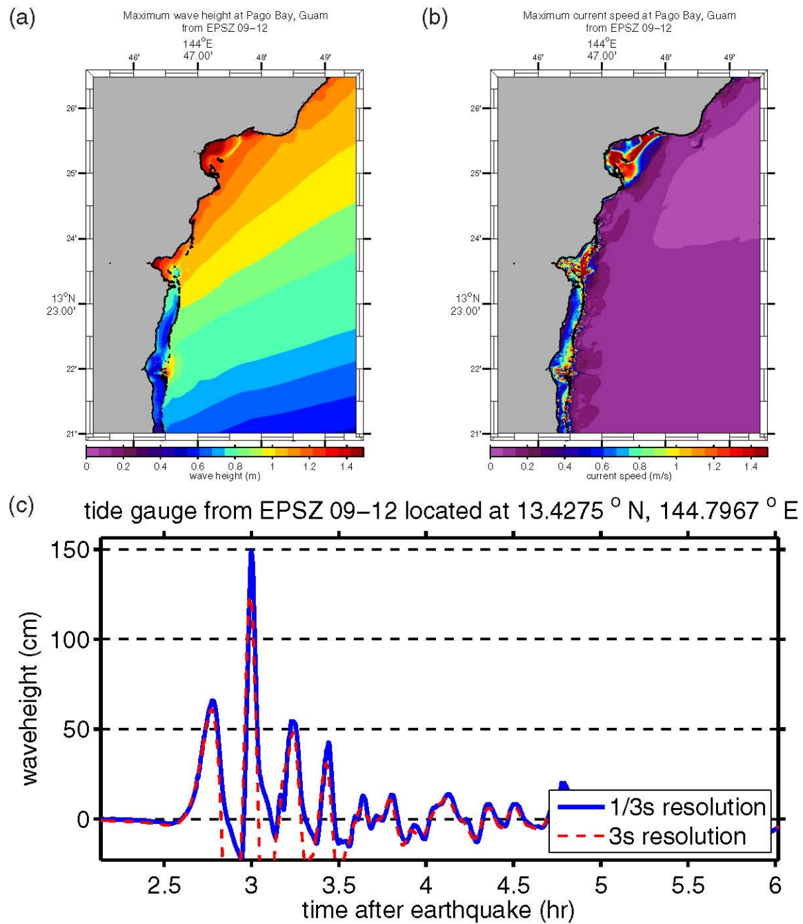
Figure E.4: (a) Maximum computed wave heights, (b) maximum computed currents, and (c) tsunami time history at the numerical tide gauge at Pago Bay from a tsunami triggered by a M_w = 8.5 earthquake on EPSZ segments 09–12 by a 6-m slip.
