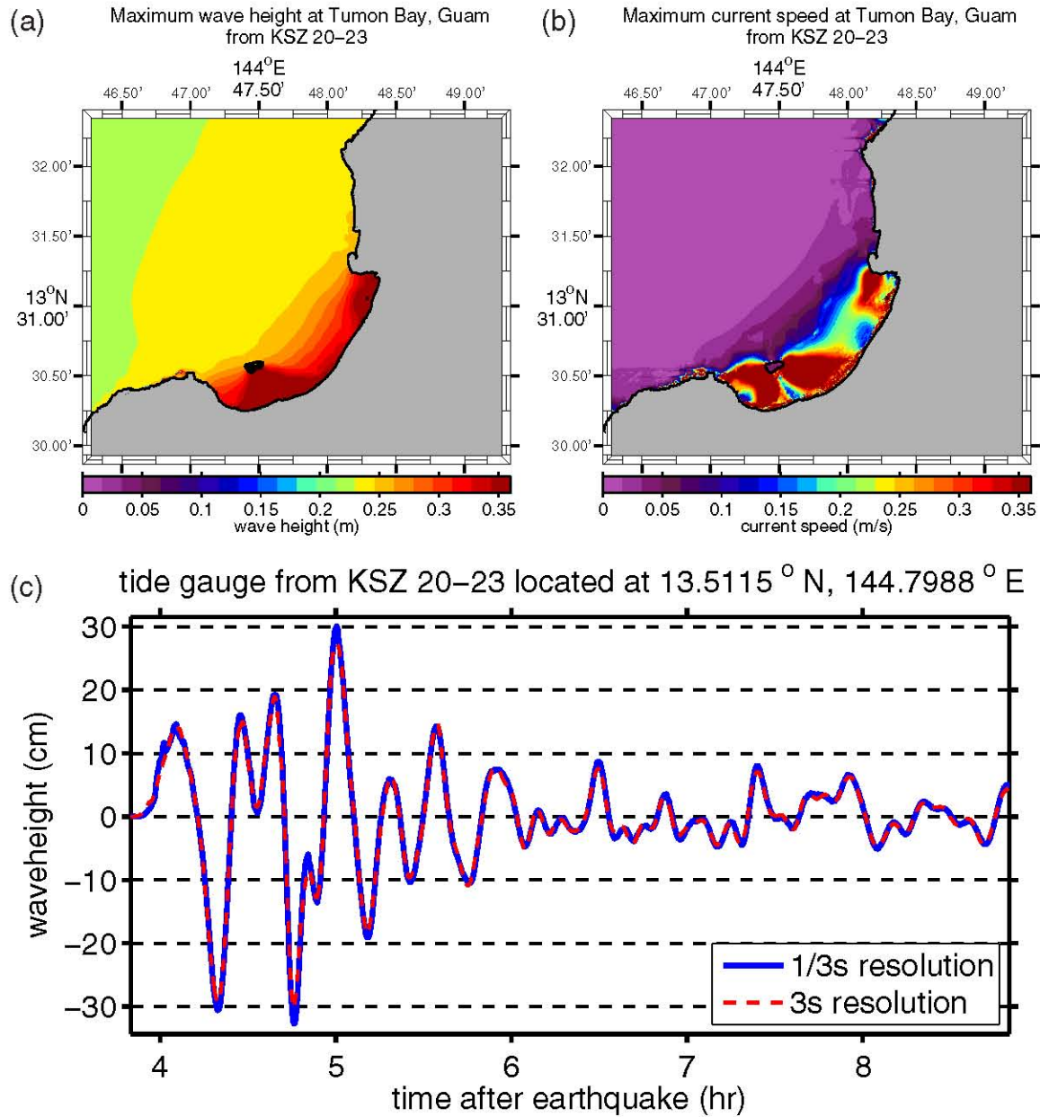
Figure C.5: (a) Maximum computed wave heights, (b) maximum computed currents, and (c) tsunami time history at the numerical tide gauge at Tumon Bay from a tsunami triggered by a Mw = 8.5 earthquake on KSZ segments 20–23 by a 6-m slip.
