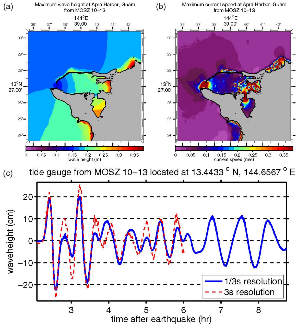
Figure D.8: (a) Maximum computed wave heights, (b) maximum computed currents, and (c) tsunami time history at the numerical tide gauge at Apra Harbor from a tsunami triggered by a M_w = 8.5 earthquake on MOSZ segments 10–13 by a 6-m slip.
