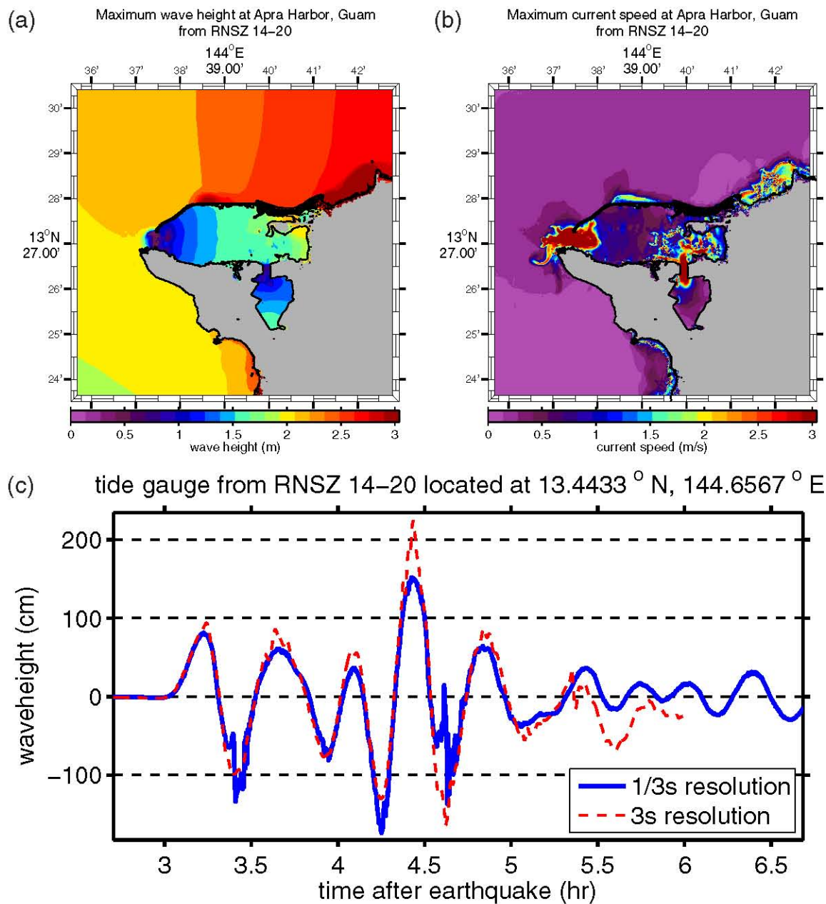
Figure D.18: (a) Maximum computed wave heights, (b) maximum computed currents, and (c) tsunami time history at the numerical tide gauge at Apra Harbor from a tsunami triggered by a M_w = 9.0 earthquake on RNSZ segments 14–20 by a 20-m slip.
