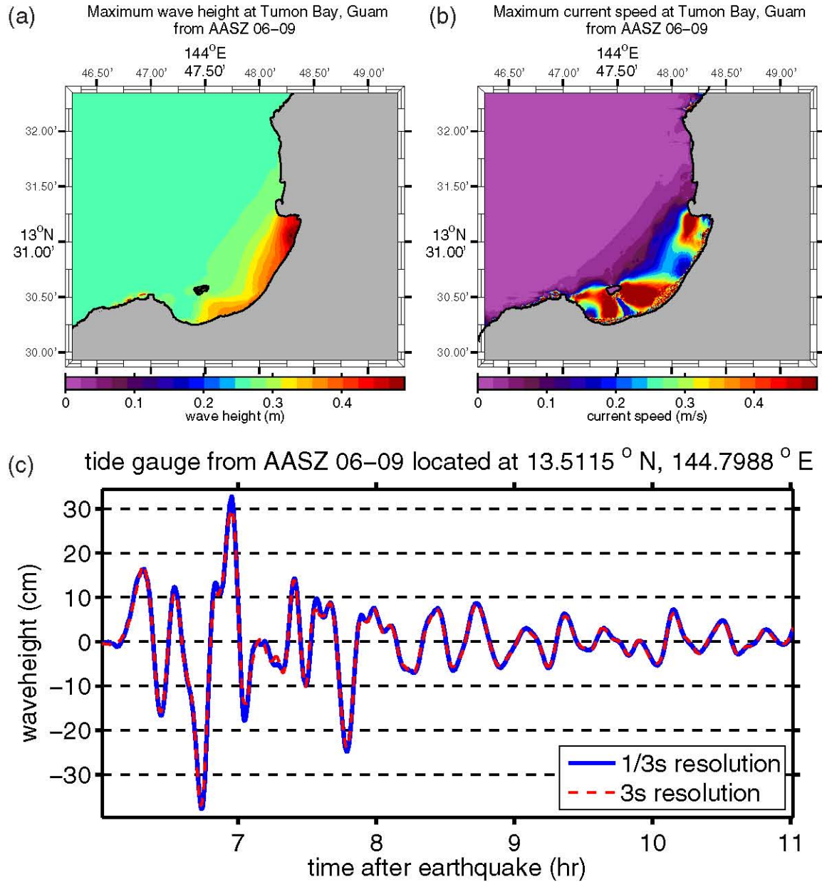
Figure C.2: (a) Maximum computed wave heights, (b) maximum computed currents, and (c) tsunami time history at the numerical tide gauge at Tumon Bay from a tsunami triggered by a M_w = 8.5 earthquake on AASZ segments 06–09 by a 6-m slip.
