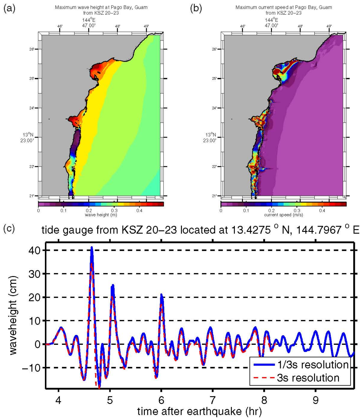
Figure E.5: (a) Maximum computed wave heights, (b) maximum computed currents, and (c) tsunami time history at the numerical tide gauge at Pago Bay from a tsunami triggered by a M_w = 8.5 earthquake on KSZ segments 20–23 by a 6-m slip.
