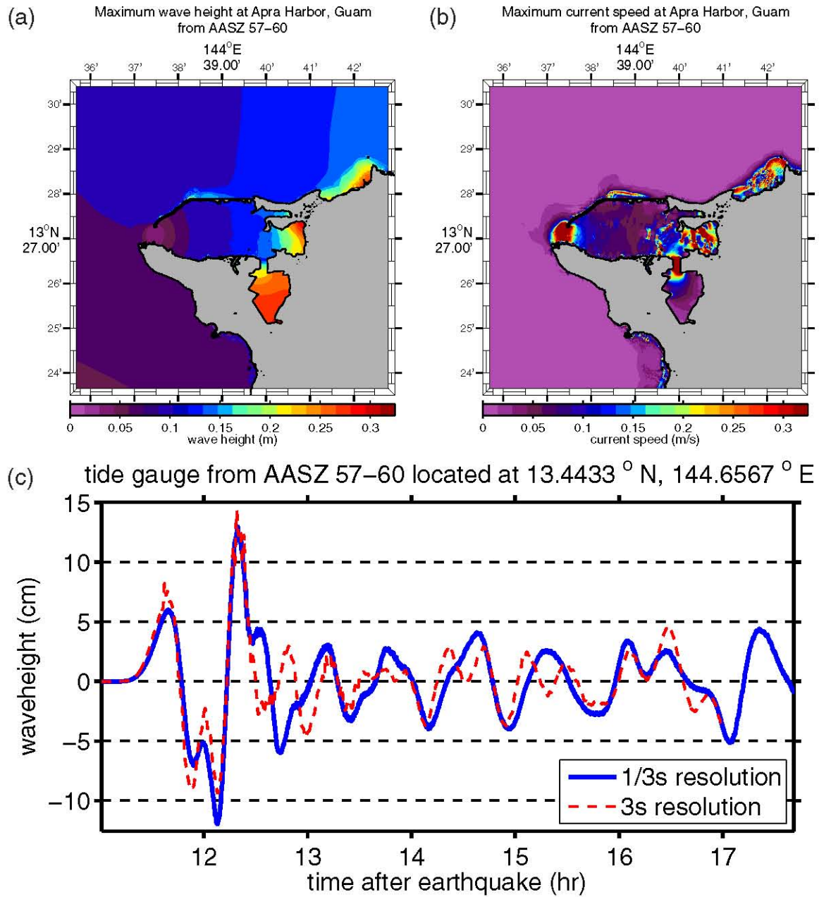
Figure D.3: (a) Maximum computed wave heights, (b) maximum computed currents, and (c) tsunami time history at the numerical tide gauge at Apra Harbor from a tsunami triggered by a Mw = 8.5 earthquake on AASZ segments 57–60 by a 6-m slip.
