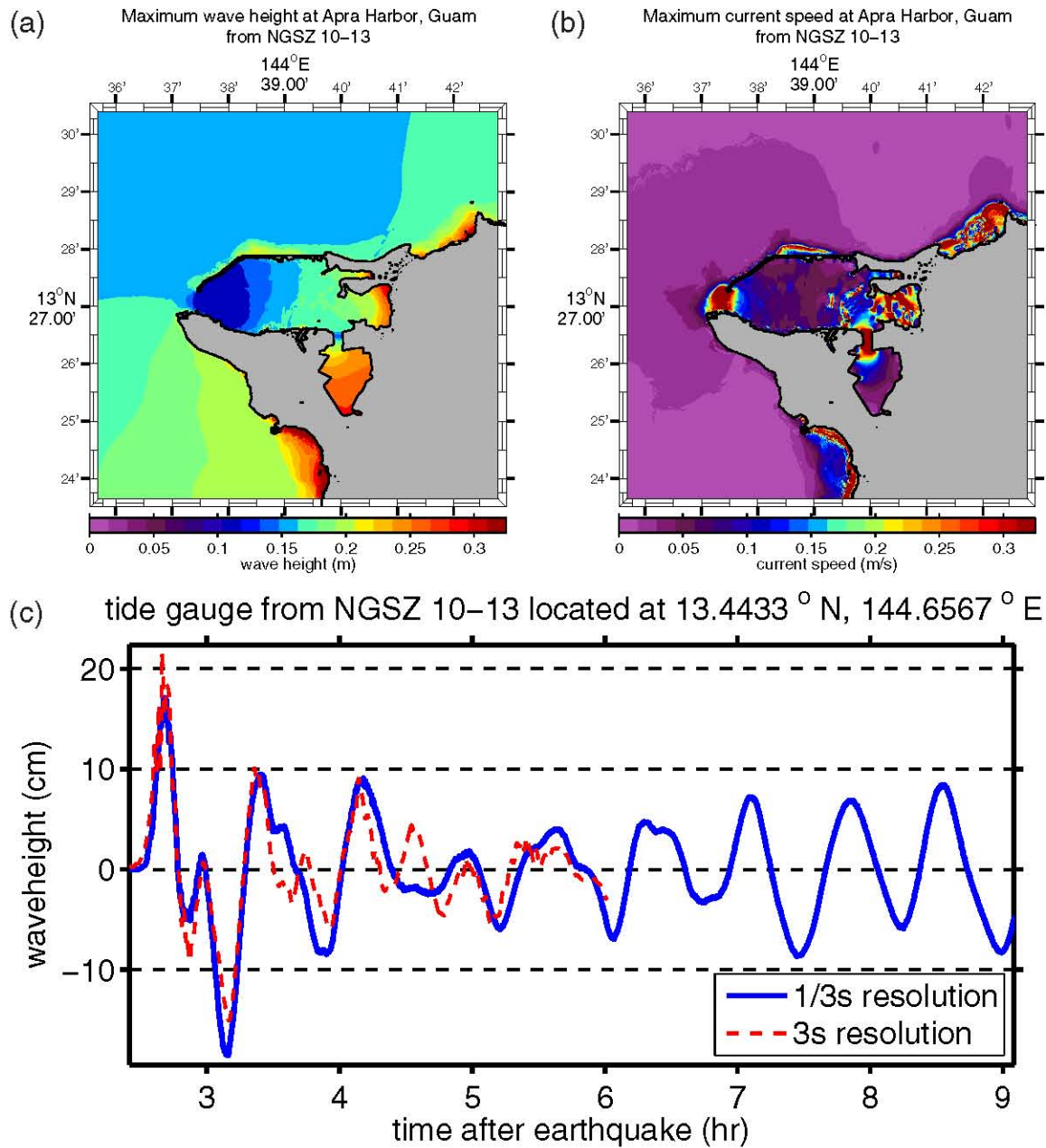
Figure D.9: (a) Maximum computed wave heights, (b) maximum computed currents, and (c) tsunami time history at the numerical tide gauge at Apra Harbor from a tsunami triggered by a Mw = 8.5 earthquake on NGSZ segments 10–13 by a 6-m slip.
