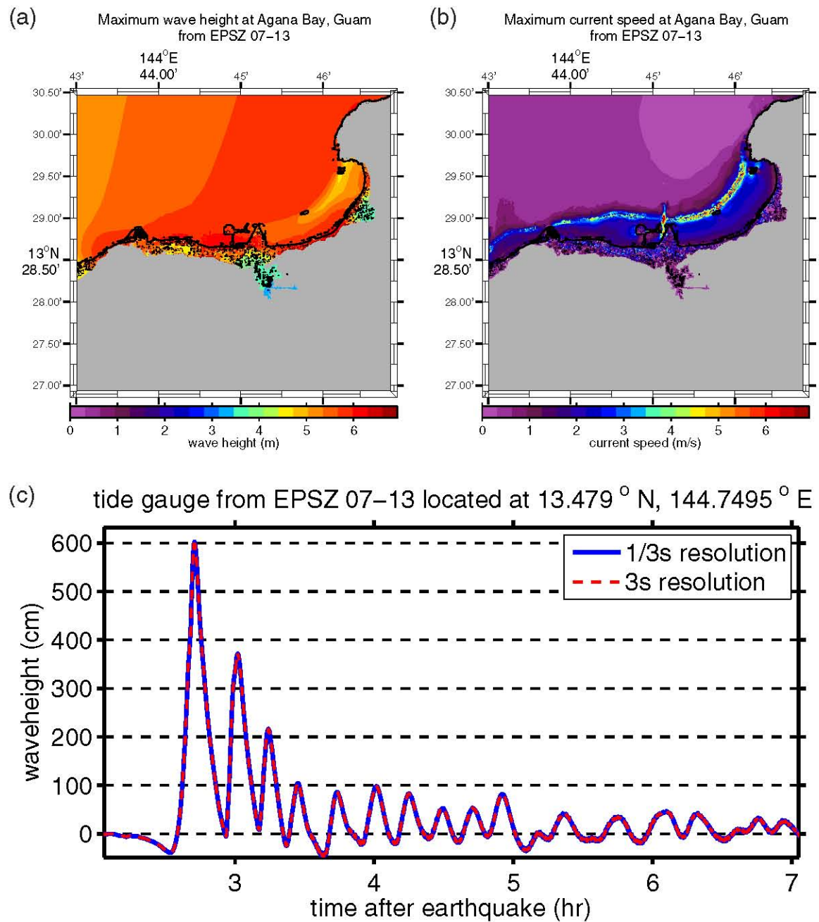
Figure E14: (a) Maximum computed wave heights, (b) maximum computed currents, and (c) tsunami time history at the numerical tide gauge at Agana Bay from a tsunami triggered by a M_w = 9.0 earthquake on EPSZ segments 07–13 by a 20-m slip.
