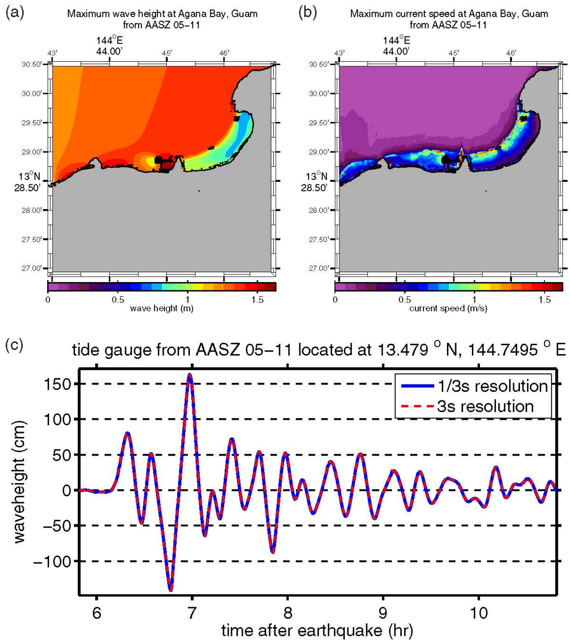
Figure E.11: (a) Maximum computed wave heights, (b) maximum computed currents, and (c) tsunami time history at the numerical tide gauge at Agana Bay from a tsunami triggered by a Mw = 9.0 earthquake on AASZ segments 05-11 by a 20-m slip.
