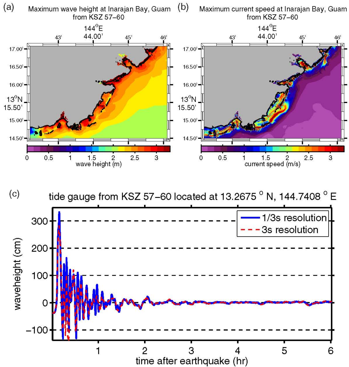
Figure G.6: (a) Maximum computed wave heights, (b) maximum computed currents, and (c) tsunami time history at the numerical tide gauge at Inarajan Bay from a tsunami triggered by a M_w = 8.5 earthquake on KSZ segments 57–60 by a 6-m slip.
