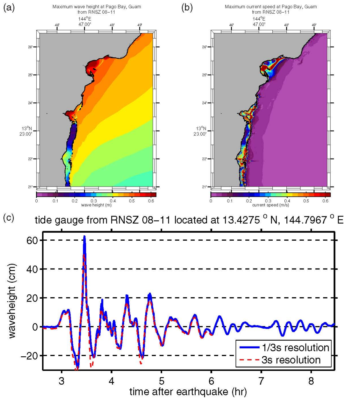
Figure E.9: (a) Maximum computed wave heights, (b) maximum computed currents, and (c) tsunami time history at the numerical tide gauge at Pago Bay from a tsunami triggered by a Mw = 8.5 earthquake on RNSZ segments 08–11 by a 6-m slip.
