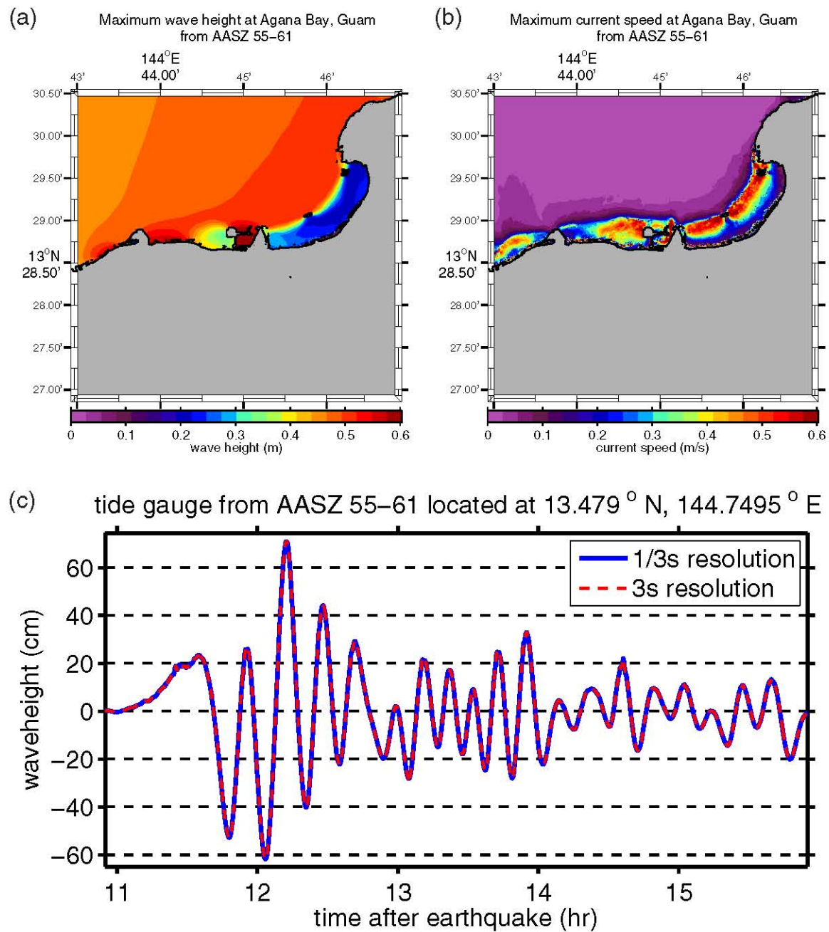
Figure F.12: (a) Maximum computed wave heights, (b) maximum computed currents, and (c) tsunami time history at the numerical tide gauge at Agana Bay from a tsunami triggered by a M_w = 9.0 earthquake on AASZ segments 55–61 by a 20-m slip.
