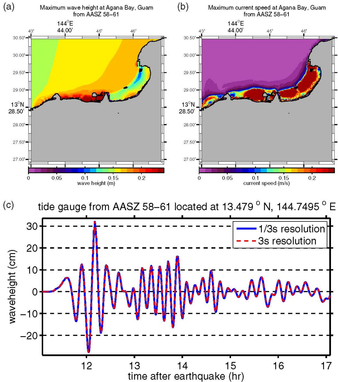
Figure E3: (a) Maximum computed wave heights, (b) maximum computed currents, and (c) tsunami time history at the numerical tide gauge at Agana Bay from a tsunami triggered by a M_w = 8.5 earthquake on AASZ segments 58–61 by a 6-m slip.
