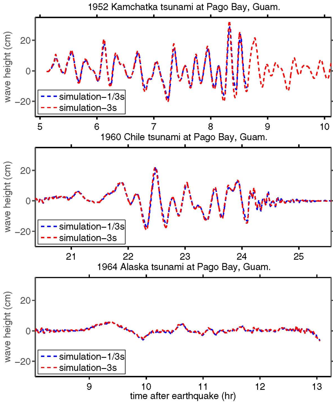
Figure B.3: The 1952 Kamchatka, the 1960 Chile and the 1964 Alaska Tsunamis at a numerical tide gauge in Pago Bay.
