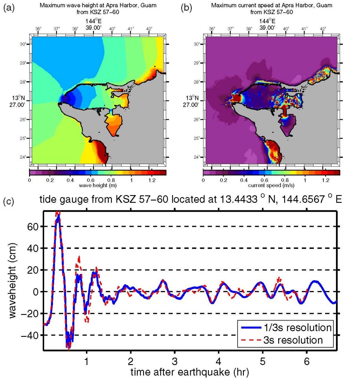
Figure D.6: (a) Maximum computed wave heights, (b) maximum computed currents, and (c) tsunami time history at the numerical tide gauge at Apra Harbor from a tsunami triggered by a Mw = 8.5 earthquake on KSZ segments 57–60 by a 6-m slip.
