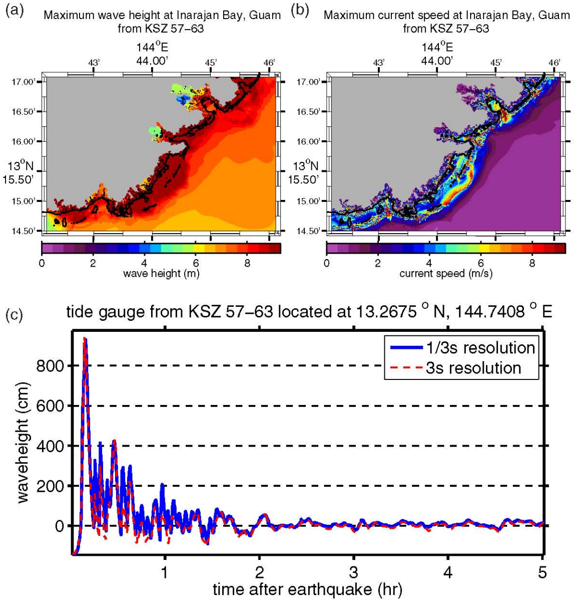
Figure 5.5: (a) Maximum computed wave heights, (b) maximum computed currents, and (c) tsunami time history at the numerical tide gauge at Inarajan Bay from a tsunami triggered by a M_w = 9.0 earthquake on KSZ segments 57–63 by a 20-m slip.
