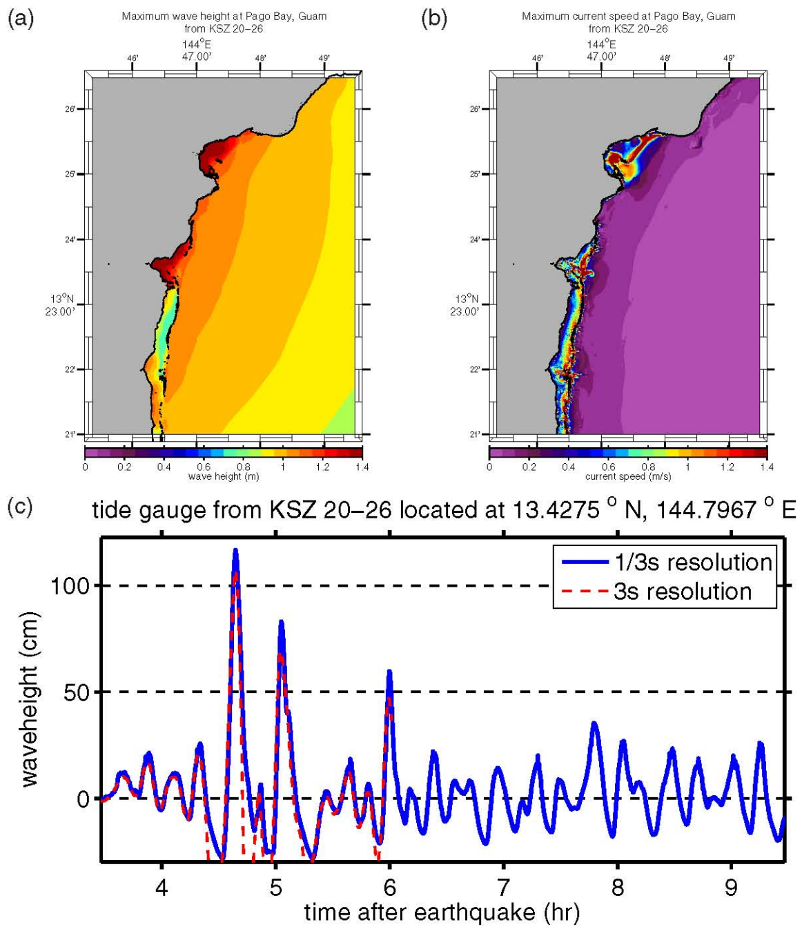
Figure E.13: (a) Maximum computed wave heights, (b) maximum computed currents, and (c) tsunami time history at the numerical tide gauge at Pago Bay from a tsunami triggered by a Mw = 9.0 earthquake on KSZ segments 20–26 by a 20-m slip.
