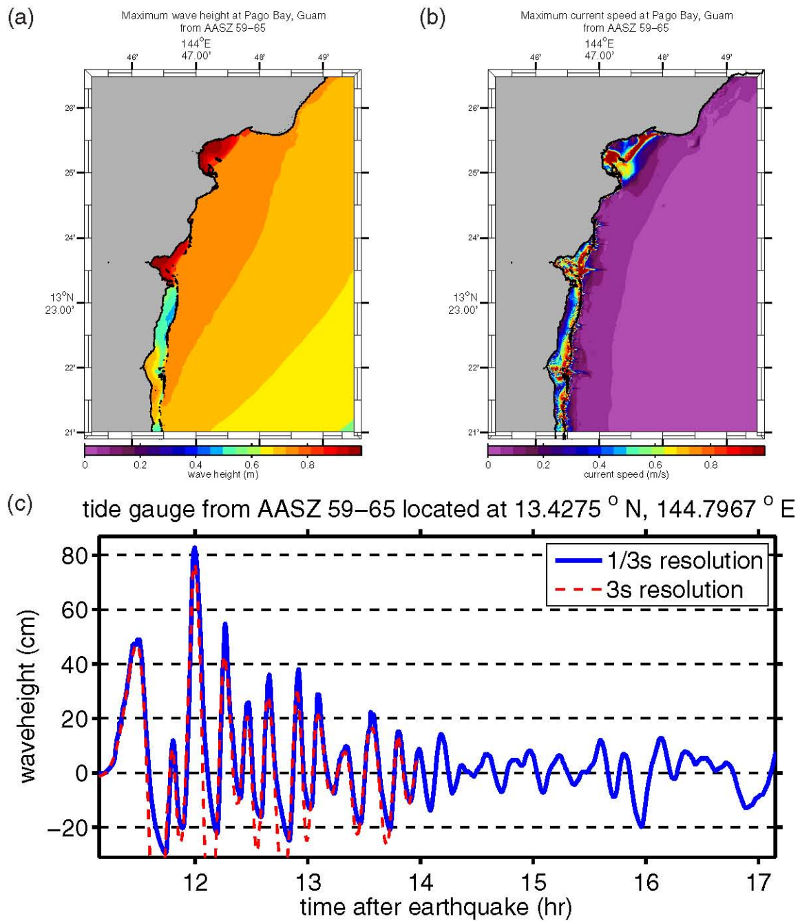
Figure E.11: (a) Maximum computed wave heights, (b) maximum computed currents, and (c) tsunami time history at the numerical tide gauge at Pago Bay from a tsunami triggered by a Mw = 9.0 earthquake on AASZ segments 59–65 by a 20-m slip.
