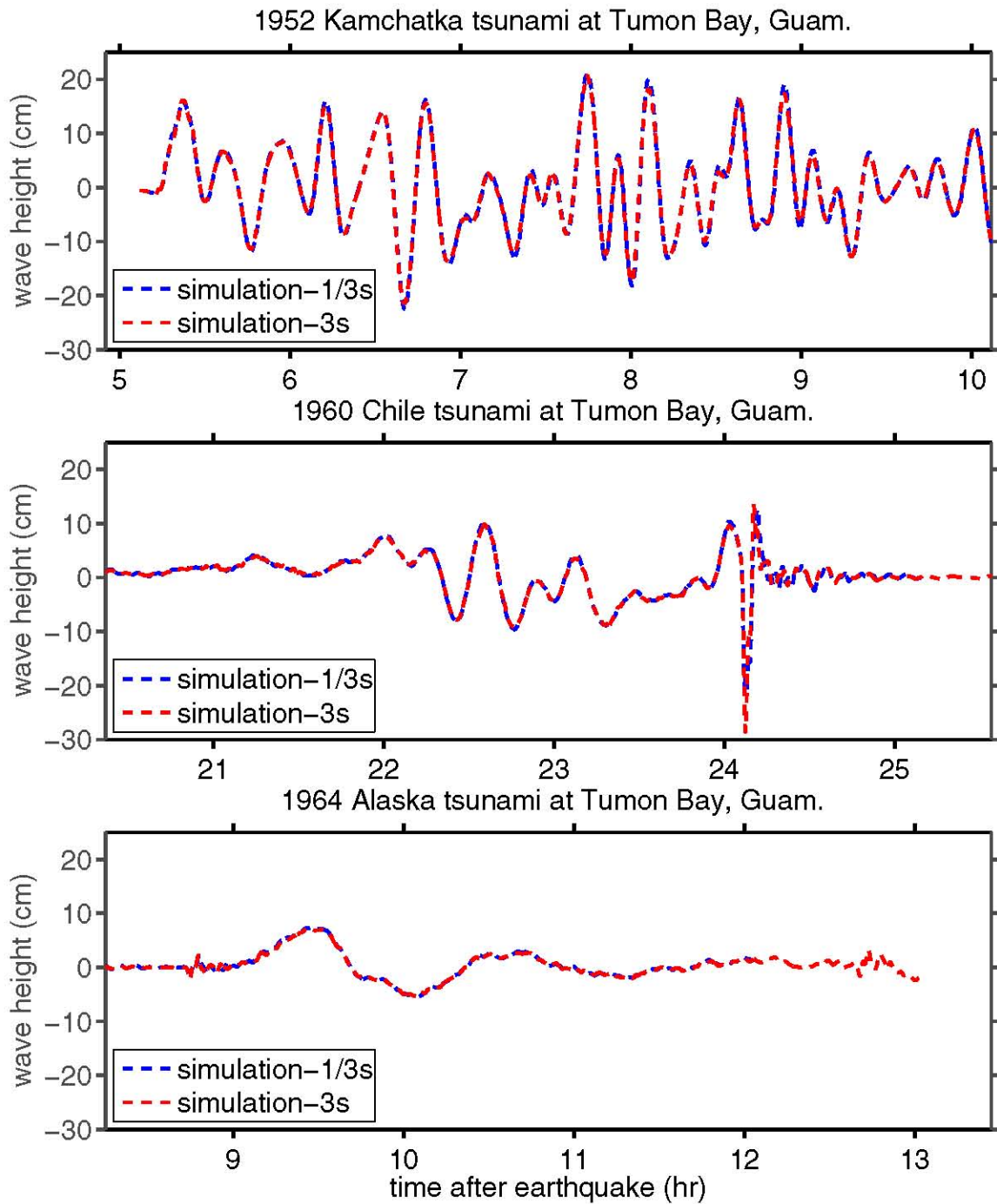
Figure B.1: The 1952 Kamchatka, the 1960 Chile and the 1964 Alaska Tsunamis at a numerical tide gauge in Tumon Bay.
