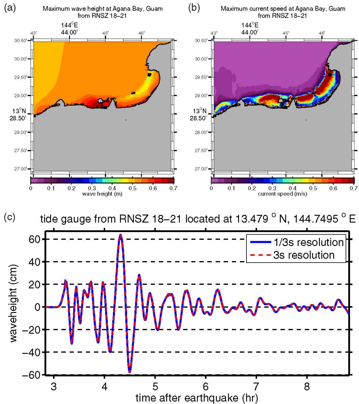
Figure E10: (a) Maximum computed wave heights, (b) maximum computed currents, and (c) tsunami time history at the numerical tide gauge at Agana Bay from a tsunami triggered by a M_w = 8.5 earthquake on RNSZ segments 18–21 by a 6-m slip.
