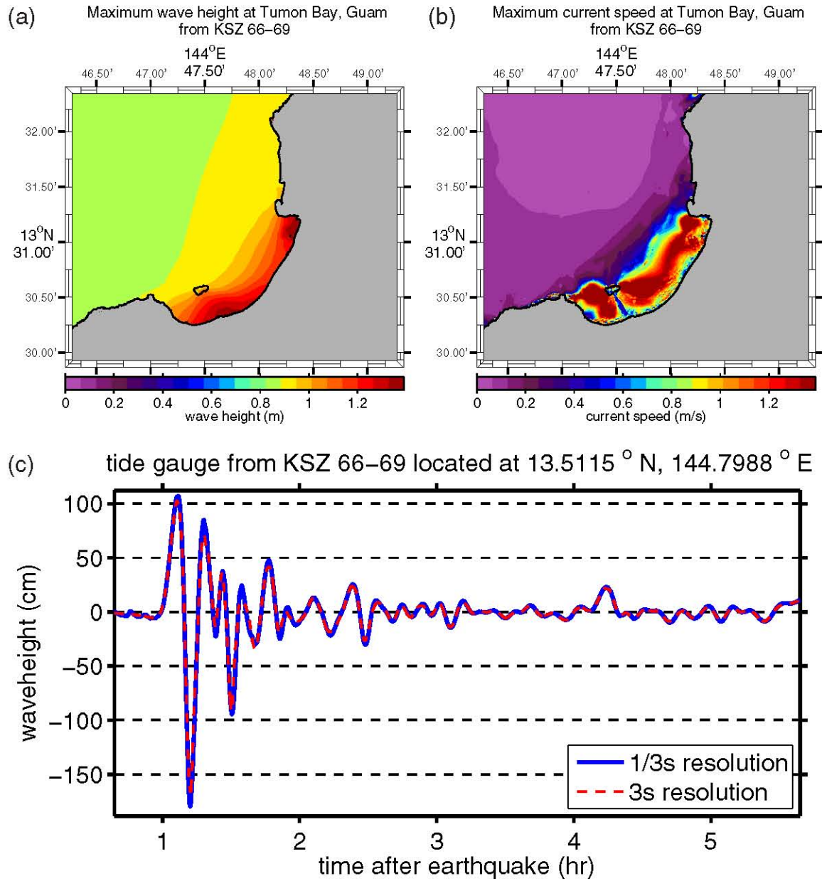
Figure C.7: (a) Maximum computed wave heights, (b) maximum computed currents, and (c) tsunami time history at the numerical tide gauge at Tumon Bay from a tsunami triggered by a Mw = 8.5 earthquake on KSZ segments 66–69 by a 6-m slip.
