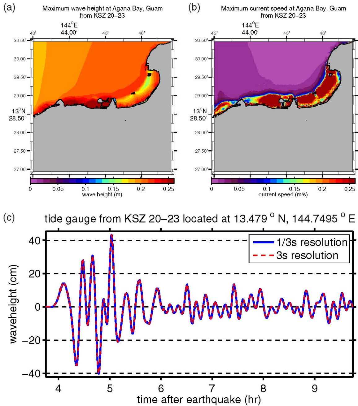
Figure E5: (a) Maximum computed wave heights, (b) maximum computed currents, and (c) tsunami time history at the numerical tide gauge at Agana Bay from a tsunami triggered by a Mw = 8.5 earthquake on KSZ segments 20–23 by a 6-m slip.
