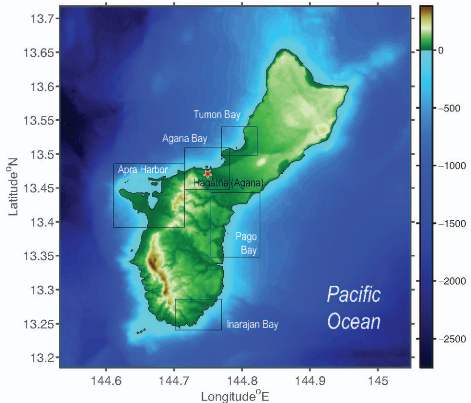
Figure 2.2: The five grids developed for tsunami hazard assessment at Apra Harbor, Agana, Tumon, Pago, and Inarajan bays.
