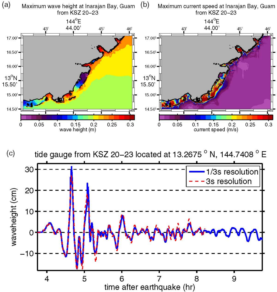
Figure G.5: (a) Maximum computed wave heights, (b) maximum computed currents, and (c) tsunami time history at the numerical tide gauge at Inarajan Bay from a tsunami triggered by a Mw = 8.5 earthquake on KSZ segments 20–23 by a 6-m slip.
