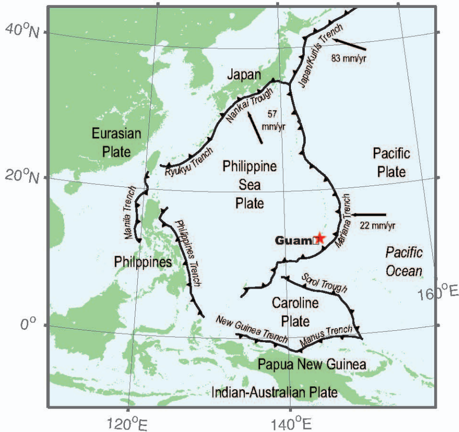
Figure 2.1: Regional setting showing the Island of Guam in relation to the Mariana Trench and surrounding tectonic plates and major specific subduction zones (Stein and Okal, 2007; Hall, 2002; 1997).
