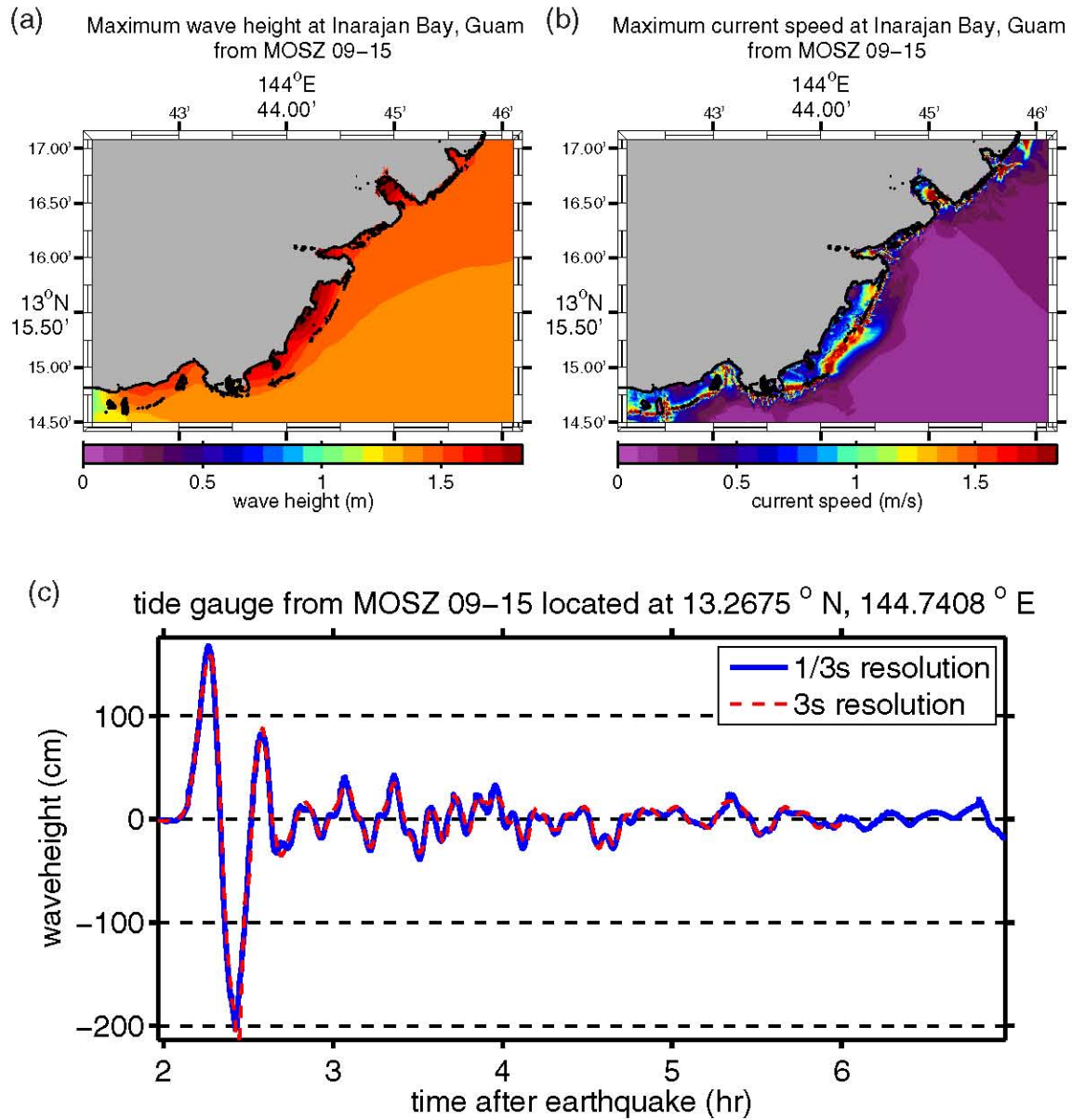
Figure G.16: (a) Maximum computed wave heights, (b) maximum computed currents, and (c) tsunami time history at the numerical tide gauge at Inarajan Bay from a tsunami triggered by a Mw = 9.0 earthquake on MOSZ segments 09–15 by a 20-m slip.
