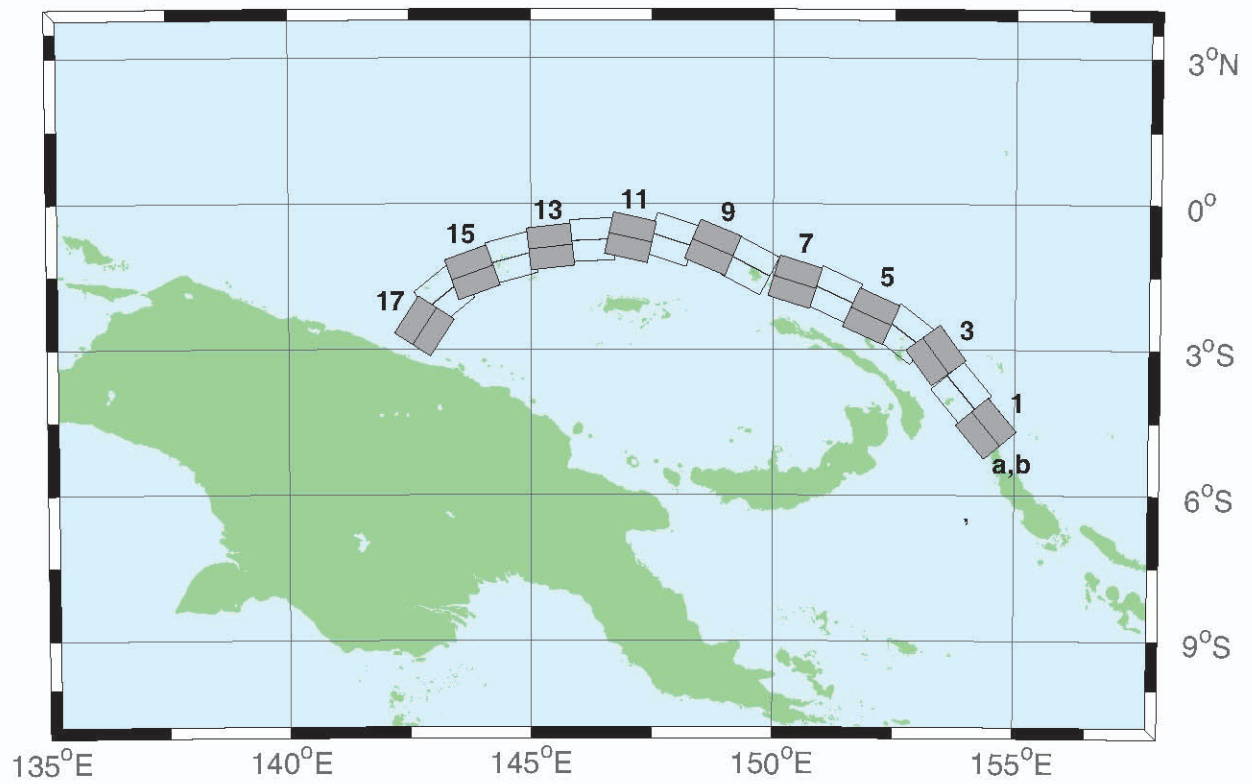
Figure H.5: Manus–Oceanic Convergent Boundary Subduction Zone unit sources.
