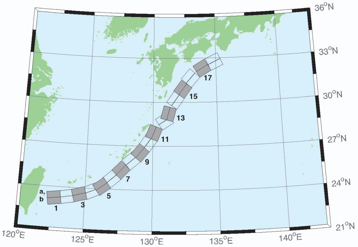
Figure H.9: Ryukyu-Kyushu-Nankai Zone unit sources.
