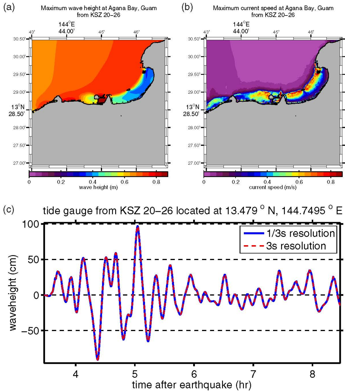
Figure E.15: (a) Maximum computed wave heights, (b) maximum computed currents, and (c) tsunami time history at the numerical tide gauge at Agana Bay from a tsunami triggered by a Mw =9.0 earthquake on KSZ segments 20–26 by a 20-m slip.
