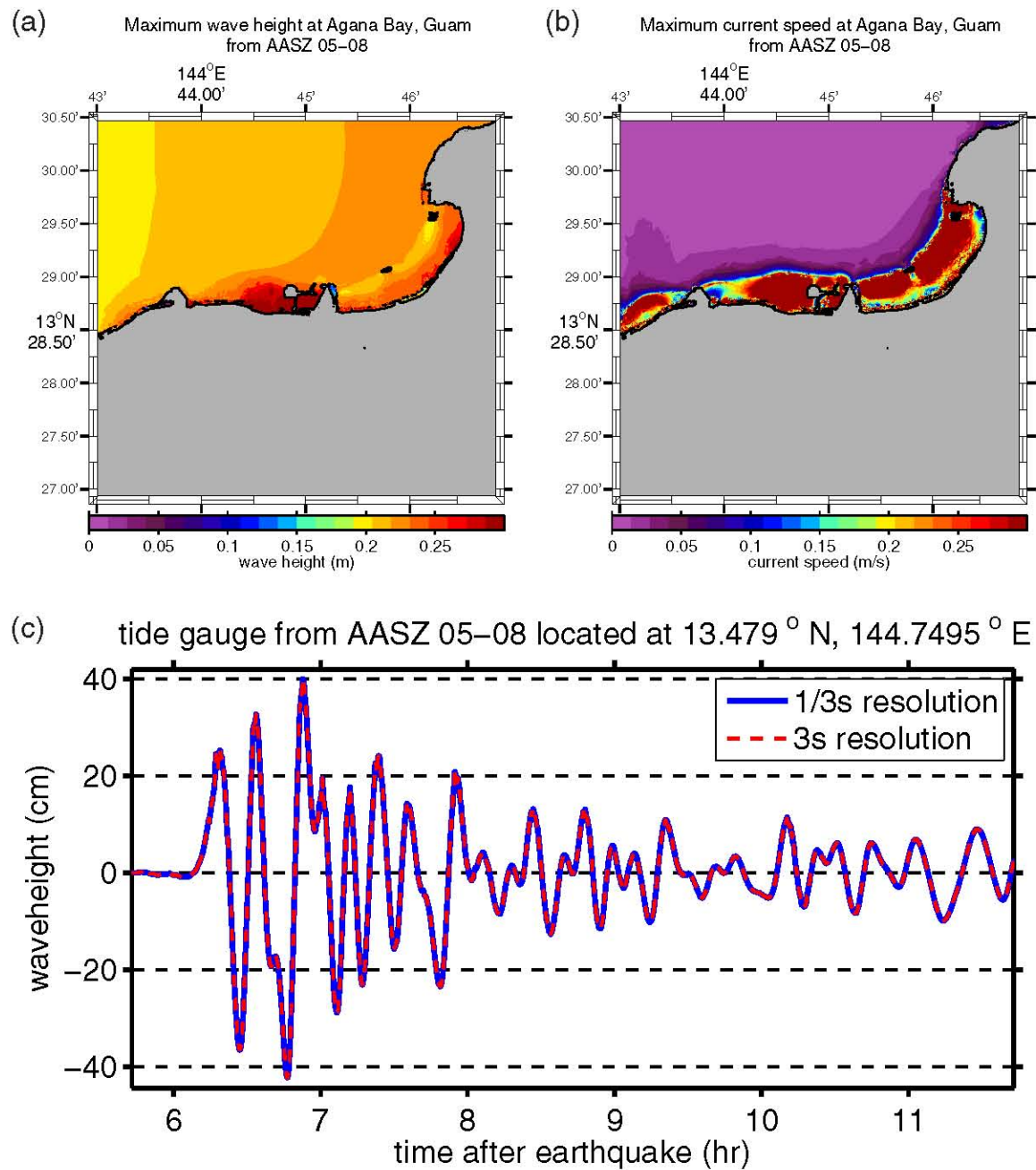
Figure F2: (a) Maximum computed wave heights, (b) maximum computed currents, and (c) tsunami time history at the numerical tide gauge at Agana Bay from a tsunami triggered by a M_w = 8.5 earthquake on AASZ segments 05–08 by a 6-m slip.
