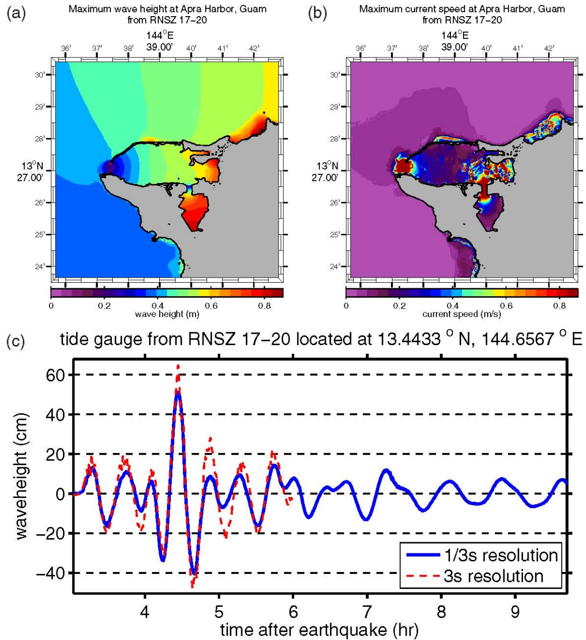
Figure D.10: (a) Maximum computed wave heights, (b) maximum computed currents, and (c) tsunami time history at the numerical tide gauge at Apra Harbor from a tsunami triggered by a M_w = 8.5 earthquake on RNSZ segments 17–20 by a 6-m slip.
