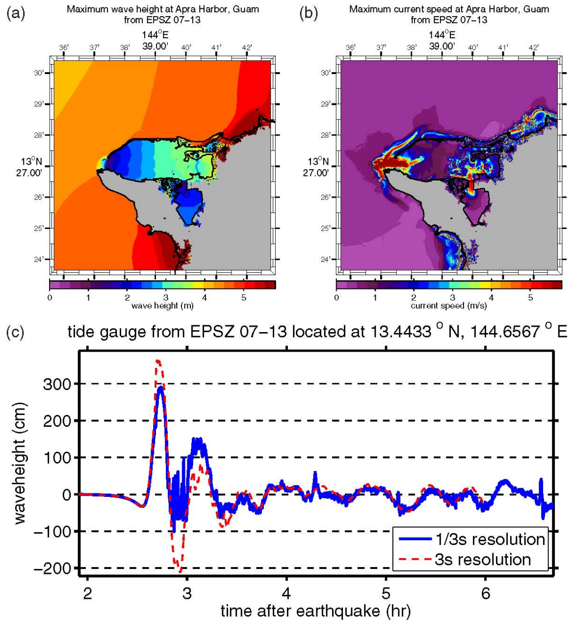
Figure D.12: (a) Maximum computed wave heights, (b) maximum computed currents, and (c) tsunami time history at the numerical tide gauge at Apra Harbor from a tsunami triggered by a M_w = 9.0 earthquake on EPSZ segments 07–13 by a 20-m slip.
