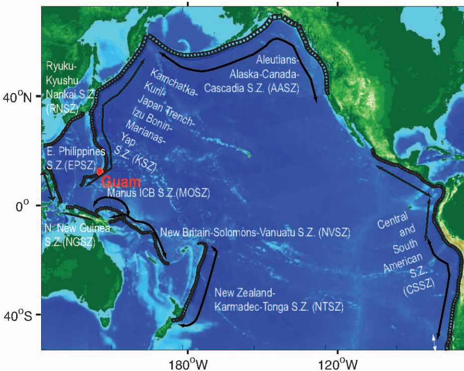
Figure 3.2: NOAA propagation database unit sources in the Pacific Ocean with respect to Guam.
