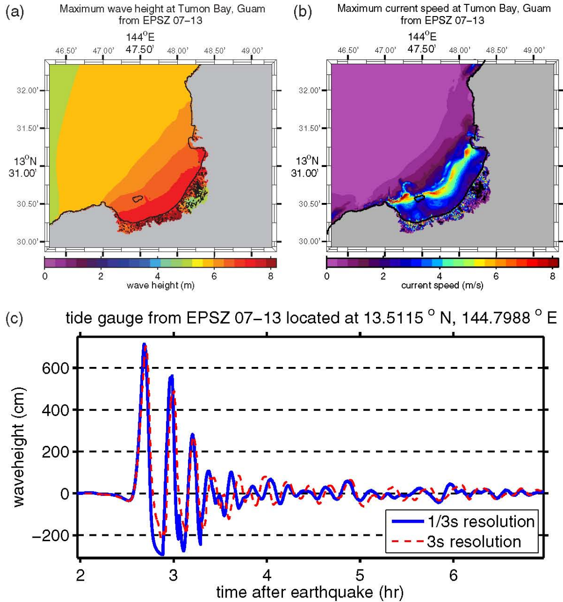
Figure 5.1: (a) Maximum computed wave heights, (b) maximum computed currents, and (c) tsunami time history at the numerical tide gauge at Tumon Bay from a tsunami triggered by a Mw = 9.0 earthquake on EPSZ segments 07–13 by a 20-m slip.
