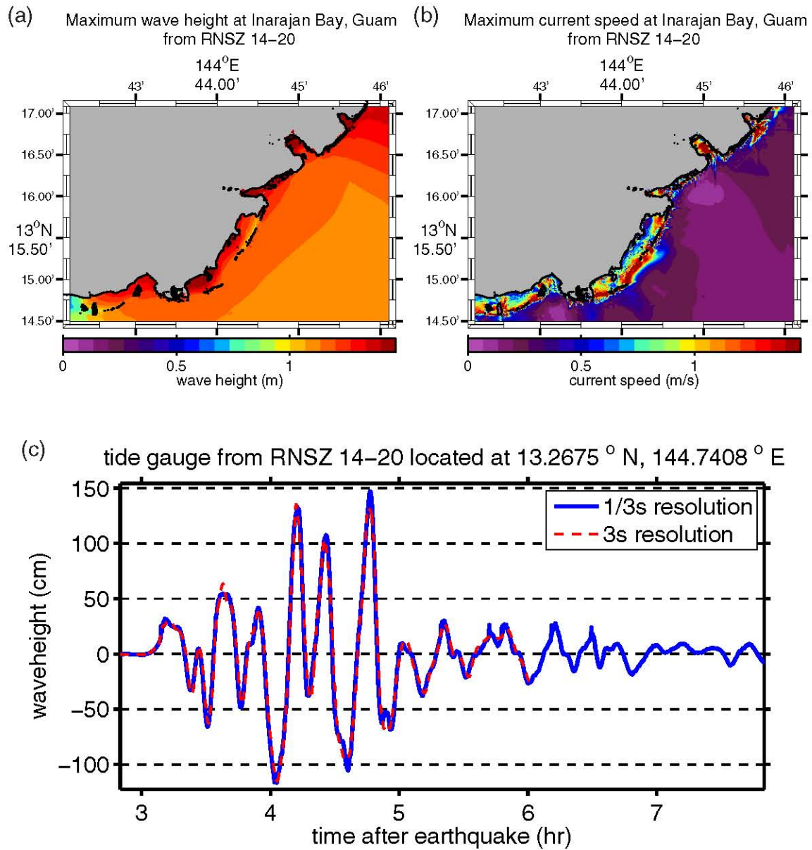
Figure G.18: (a) Maximum computed wave heights, (b) maximum computed currents, and (c) tsunami time history at the numerical tide gauge at Inarajan Bay from a tsunami triggered by a M_w = 9.0 earthquake on RNSZ segments 14–20 by a 20-m slip.
