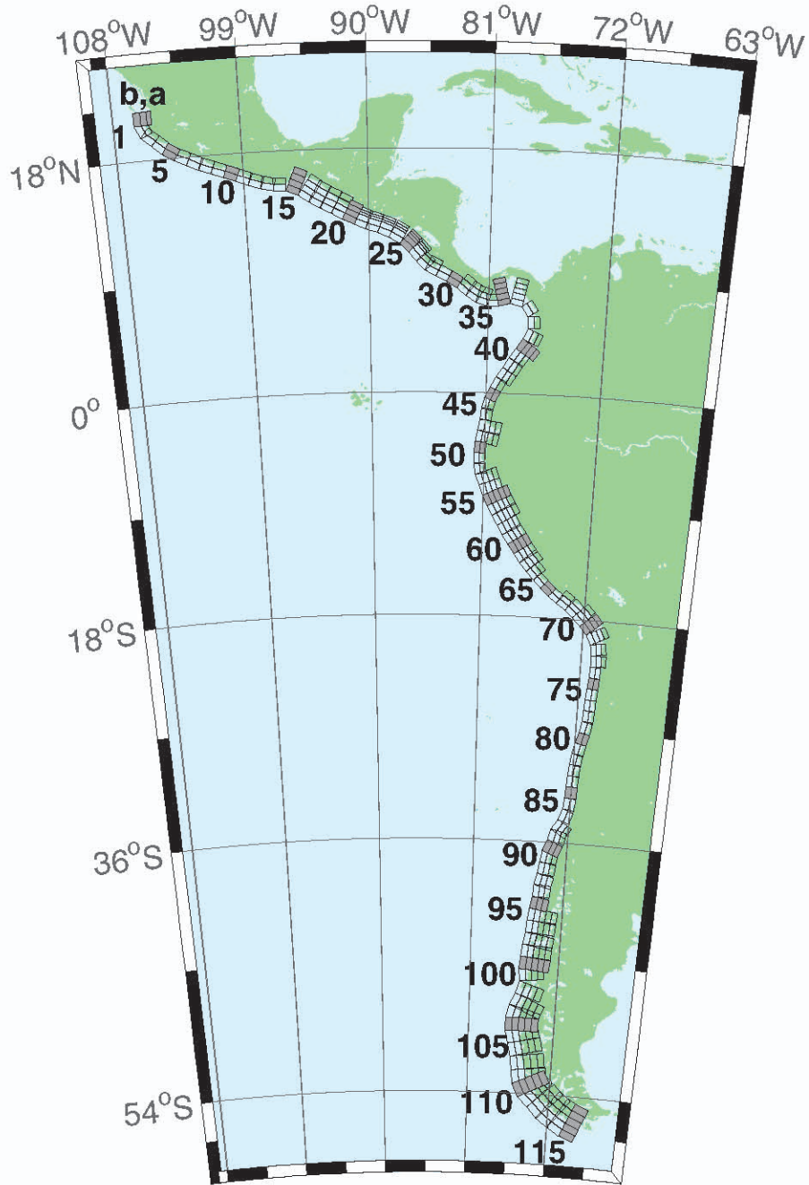
Figure H.2: Central and South America Subduction Zone unit sources.
