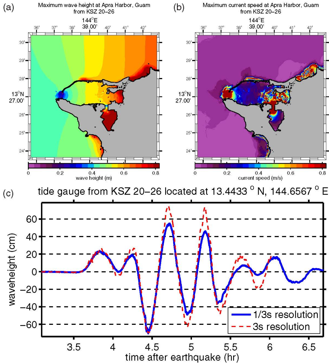
Figure D.13: (a) Maximum computed wave heights, (b) maximum computed currents, and (c) tsunami time history at the numerical tide gauge at Apra Harbor from a tsunami triggered by a Mw = 9.0 earthquake on KSZ segments 20–26 by a 20-m slip.
