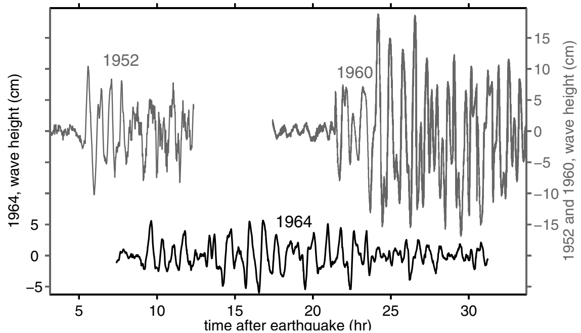
Figure 3.3: (a) Apra Harbor tide gauge observations of 1952, 1960, and 1964 tsunamis and (b) residual signal after detiding.
