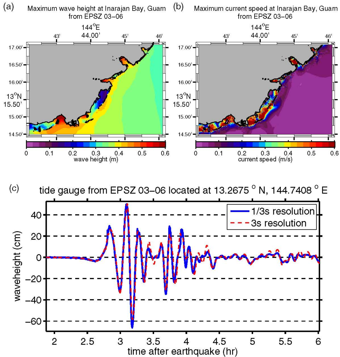
Figure G.4: (a) Maximum computed wave heights, (b) maximum computed currents, and (c) tsunami time history at the numerical tide gauge at Inarajan Bay from a tsunami triggered by a M_w = 8.5 earthquake on EPSZ segments 03–06 by a 6-m slip.
