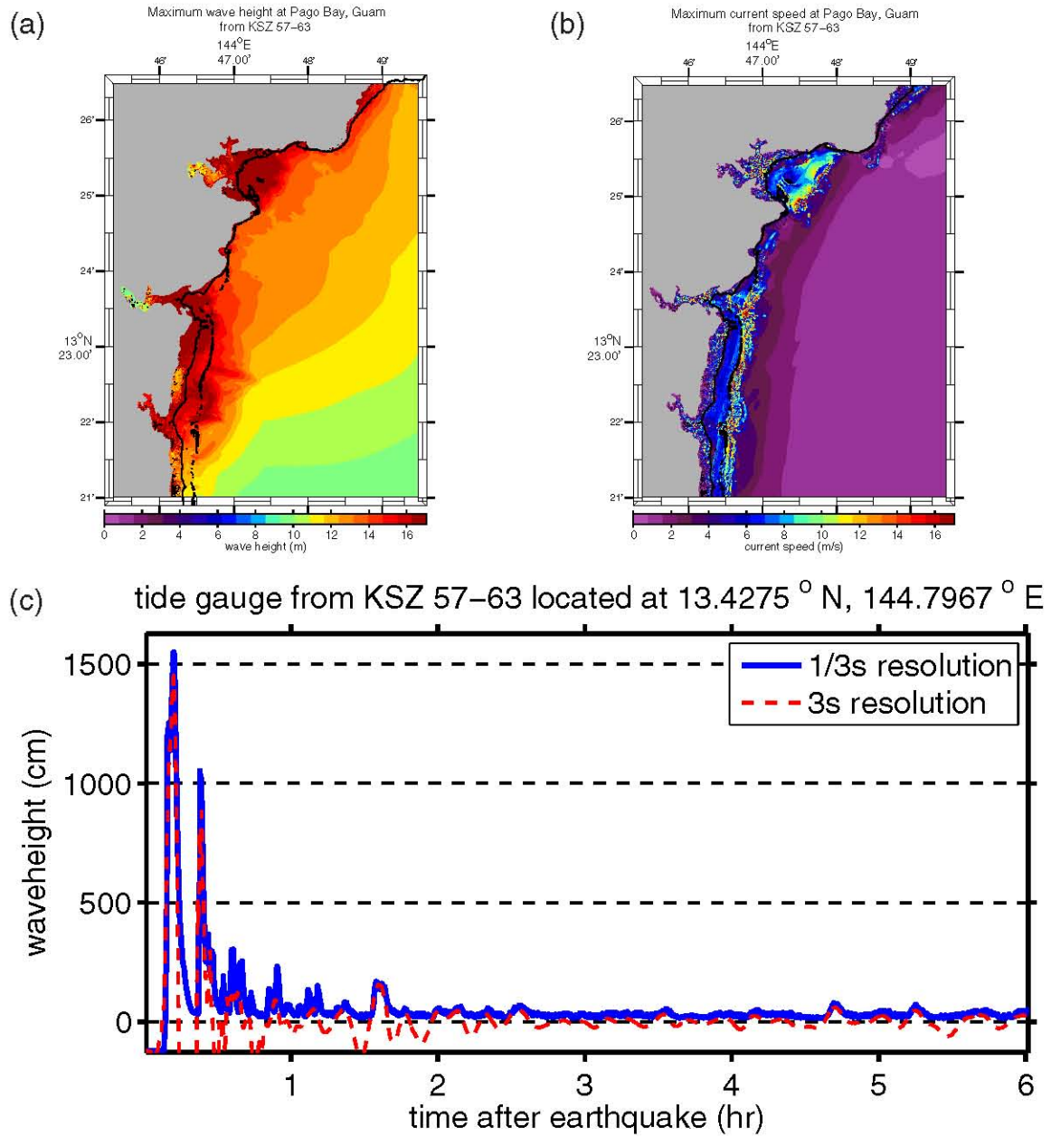
Figure 5.3: (a) Maximum computed wave heights, (b) maximum computed currents, and (c) tsunami time history at the numerical tide gauge at Pago Bay from a tsunami triggered by a Mw = 9.0 earthquake on KSZ segments 57–63 by a 20-m slip.
