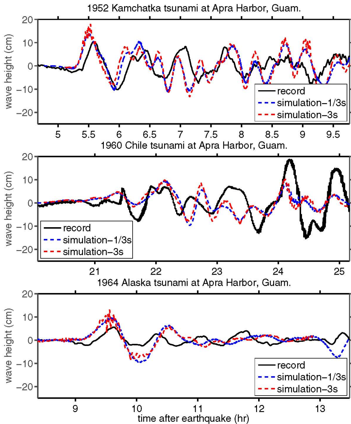
Figure 3.4: Comparison of numerical results with tide gauge records of 1952, 1960, and 1964 tsunamis at Apra Harbor.
