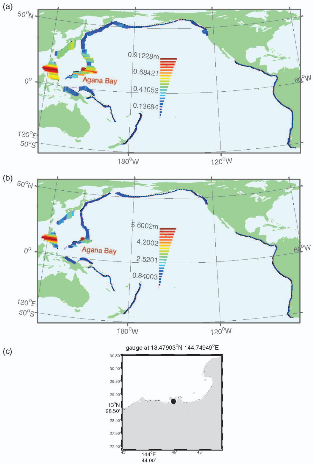
Figure E.1: Tsunami wave height response at Agana Bay from tsunamis triggered by (a) Mw = 8.5 and (b) Mw = 9.0 earthquakes.
