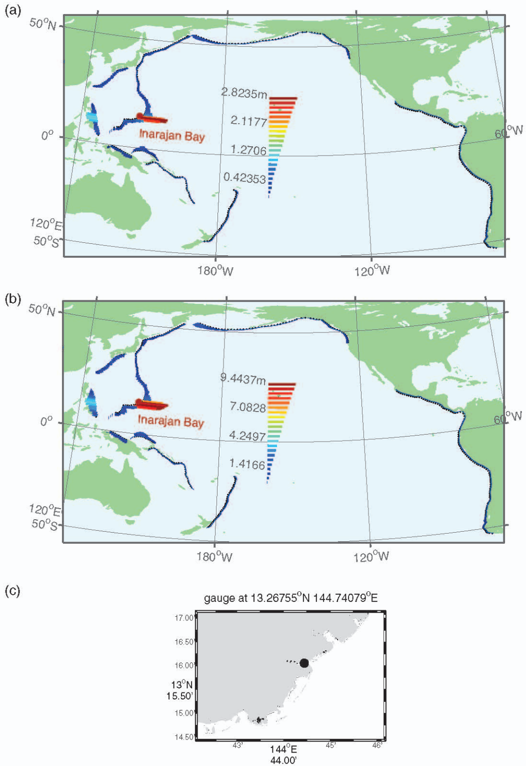
Figure G.1: Tsunami wave height response at Inarajan Bay from tsunamis triggered by (a) Mw = 8.5 and (b) Mw = 9.0 earthquakes.
