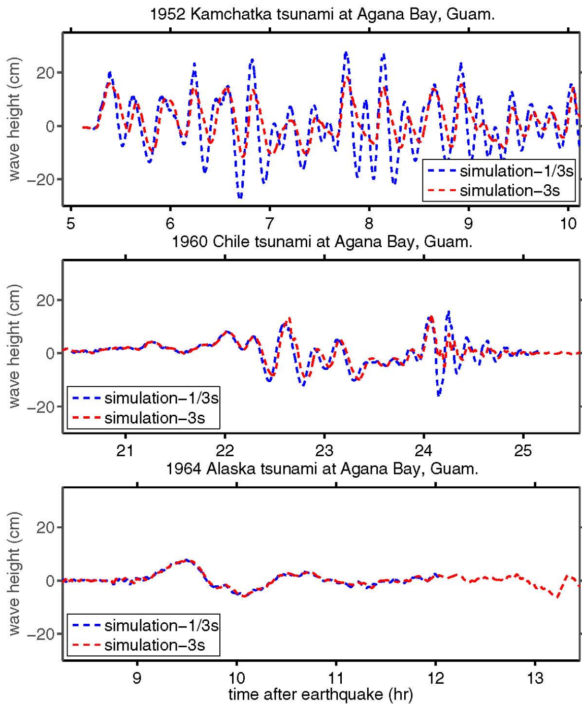
Figure B.4: The 1952 Kamchatka, the 1960 Chile and the 1964 Alaska Tsunamis at a numerical tide gauge in Agana Bay.
