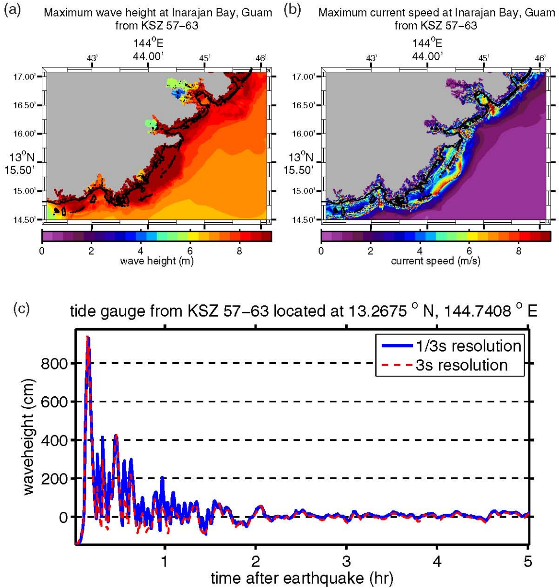
Figure G.15: (a) Maximum computed wave heights, (b) maximum computed currents, and (c) tsunami time history at the numerical tide gauge at Inarajan Bay from a tsunami triggered by a Mw = 9.0 earthquake on KSZ segments 57–63 by a 20-m slip.
