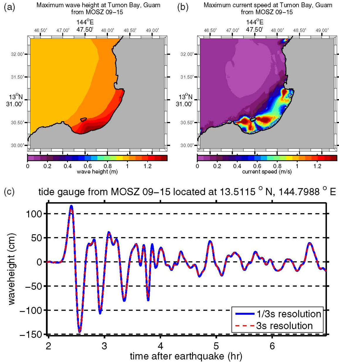
Figure C.16: (a) Maximum computed wave heights, (b) maximum computed currents, and (c) tsunami time history at the numerical tide gauge at Tumon Bay from a tsunami triggered by a M_w = 9.0 earthquake on MOSZ segments 09–15 by a 20-m slip.
