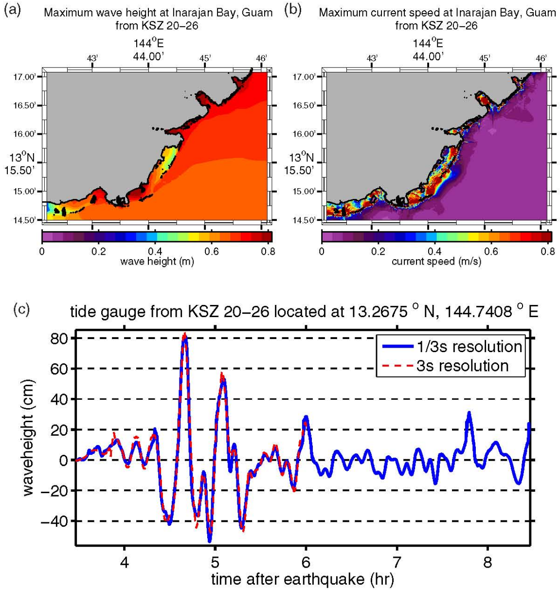
Figure G.13: (a) Maximum computed wave heights, (b) maximum computed currents, and (c) tsunami time history at the numerical tide gauge at Inarajan Bay from a tsunami triggered by a M_w = 9.0 earthquake on KSZ segments 20–26 by a 20-m slip.
