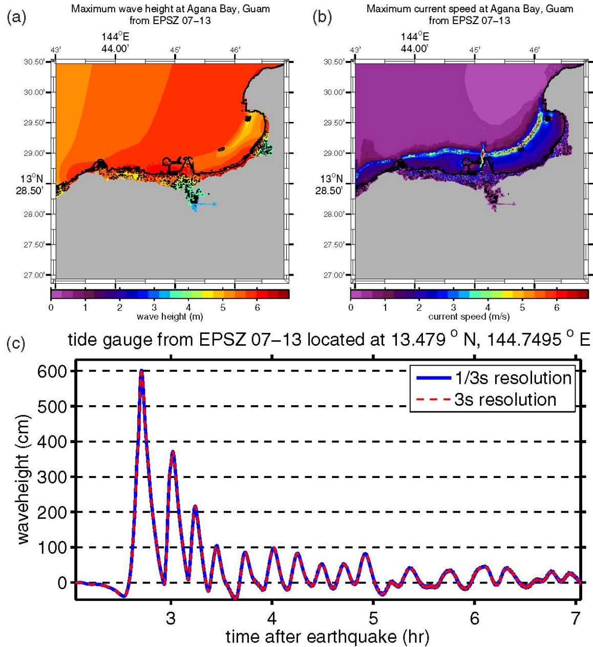
Figure 5.4: (a) Maximum computed wave heights, (b) maximum computed currents, and (c) tsunami time history at the numerical tide gauge at Agana Bay from a tsunami triggered by a Mw = 9.0 earthquake on EPSZ segments 07-13 by a 20-m slip.
