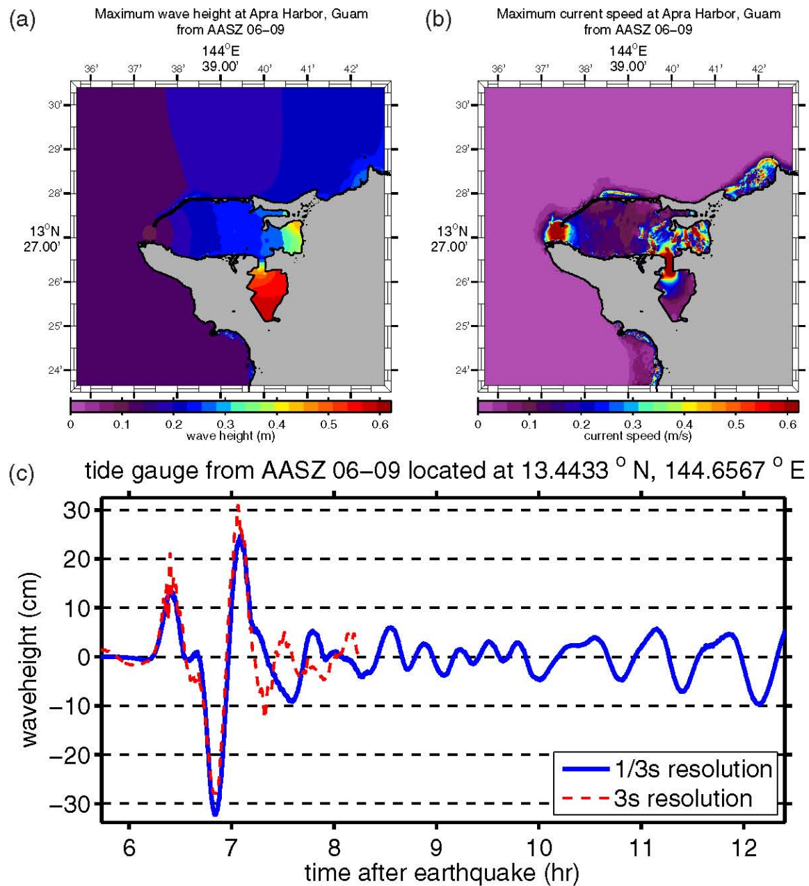
Figure D.2: (a) Maximum computed wave heights, (b) maximum computed currents, and (c) tsunami time history at the numerical tide gauge at Apra Harbor from a tsunami triggered by a M_w = 8.5 earthquake on AASZ segments 06–09 by a 6-m slip.
