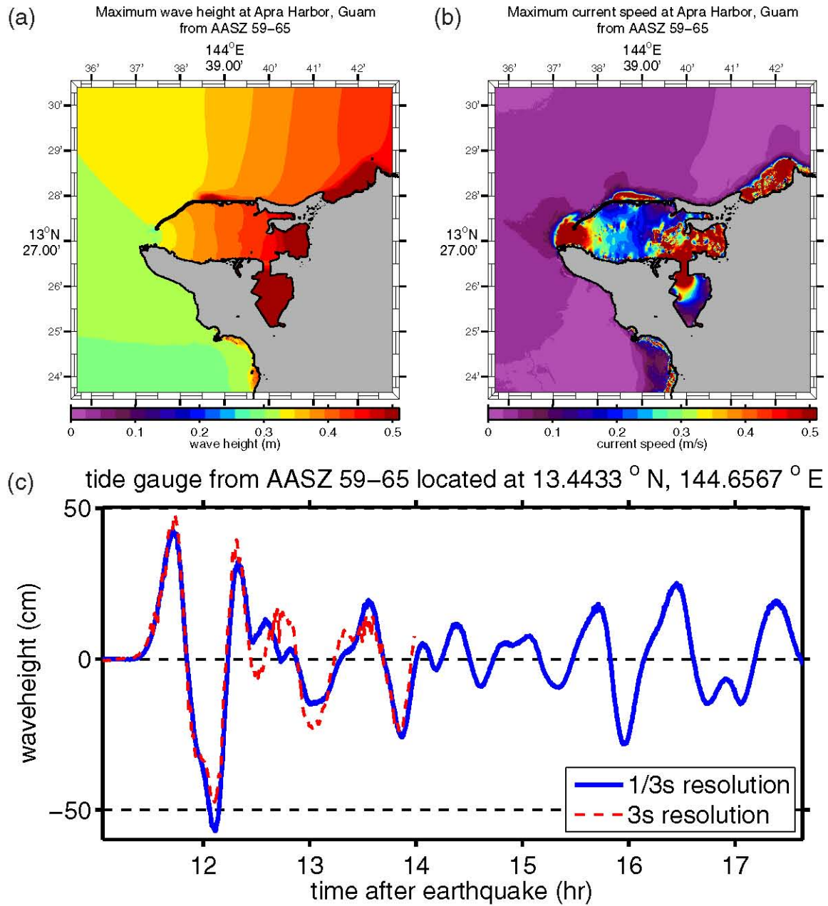
Figure D.11: (a) Maximum computed wave heights, (b) maximum computed currents, and (c) tsunami time history at the numerical tide gauge at Apra Harbor from a tsunami triggered by a Mw = 9.0 earthquake on AASZ segments 59–65 by a 20-m slip.
