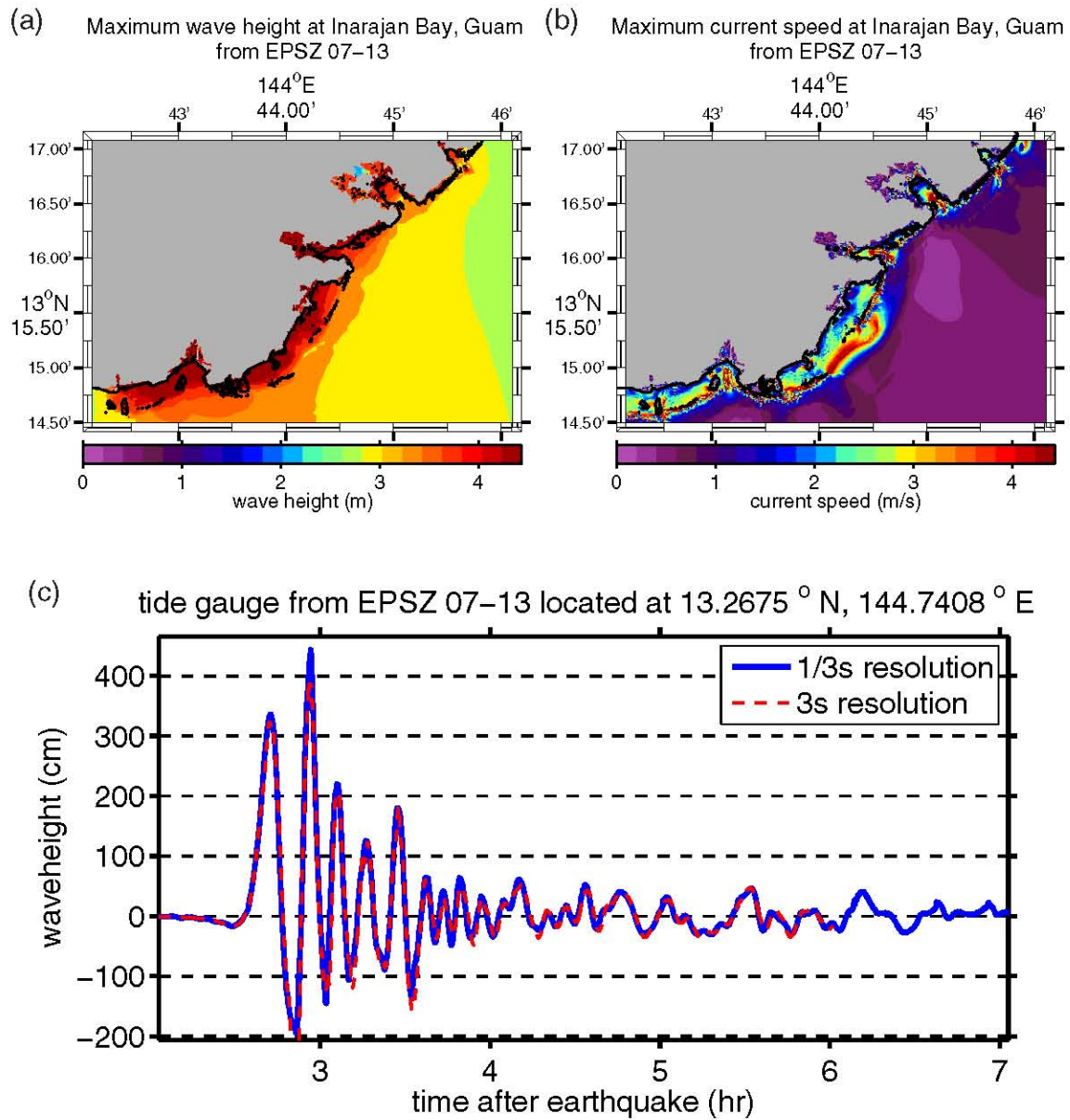
Figure G.12: (a) Maximum computed wave heights, (b) maximum computed currents, and (c) tsunami time history at the numerical tide gauge at Inarajan Bay from a tsunami triggered by a M_w = 9.0 earthquake on EPSZ segments 07–13 by a 20-m slip.
