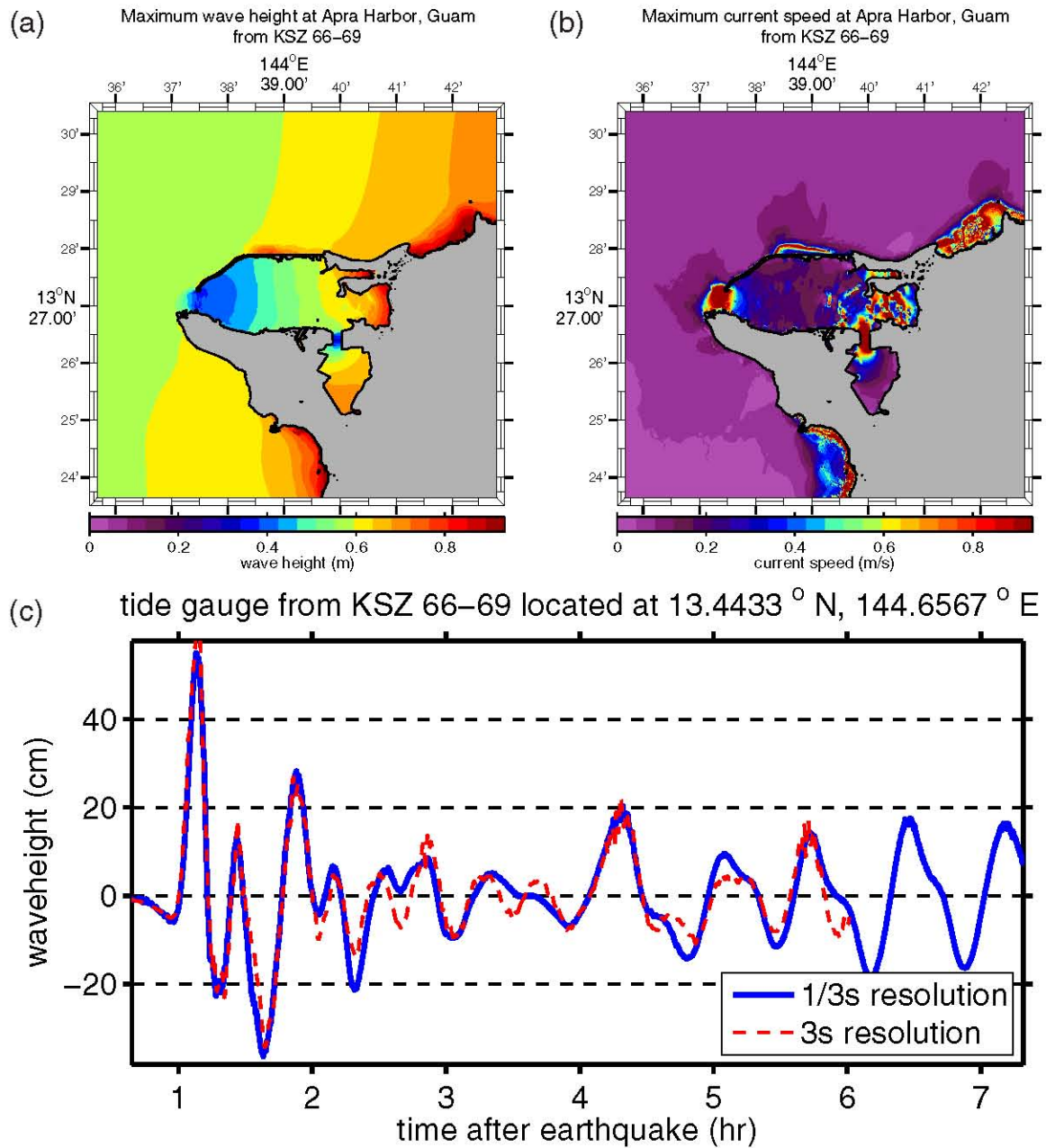
Figure D.7: (a) Maximum computed wave heights, (b) maximum computed currents, and (c) tsunami time history at the numerical tide gauge at Apra Harbor from a tsunami triggered by a Mw = 8.5 earthquake on KSZ segments 66–69 by a 6-m slip.
