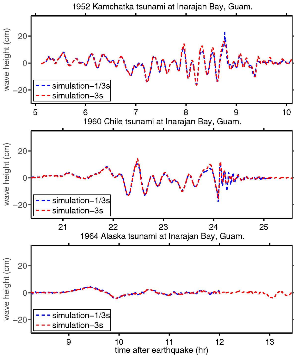
Figure B.5: The 1952 Kamchatka, the 1960 Chile and the 1964 Alaska Tsunamis at a numerical tide gauge in Inarajan Bay.
