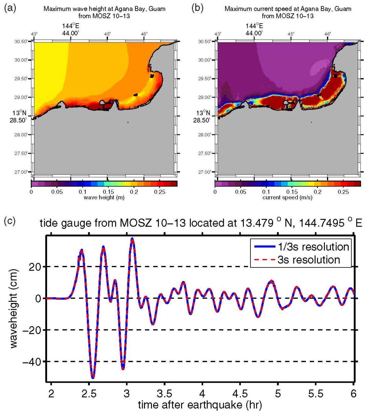
Figure F8: (a) Maximum computed wave heights, (b) maximum computed currents, and (c) tsunami time history at the numerical tide gauge at Agana Bay from a tsunami triggered by a M_w = 8.5 earthquake on MOSZ segments 10–13 by a 6-m slip.
