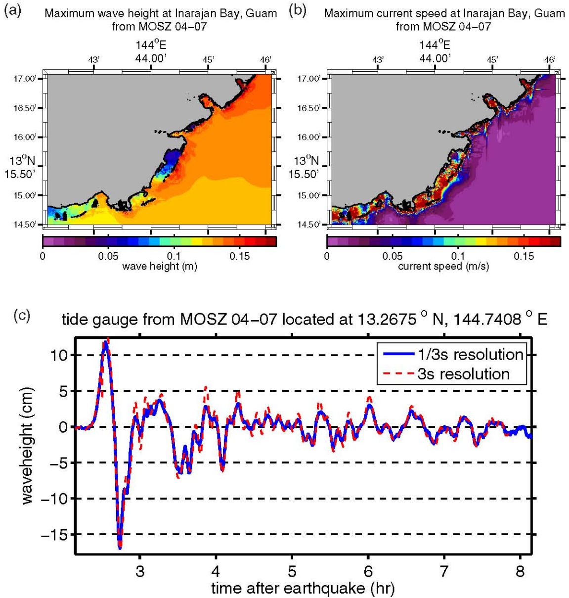
Figure G.7: (a) Maximum computed wave heights, (b) maximum computed currents, and (c) tsunami time history at the numerical tide gauge at Inarajan Bay from a tsunami triggered by a Mw = 8.5 earthquake on MOSZ segments 04–07 by a 6-m slip.
