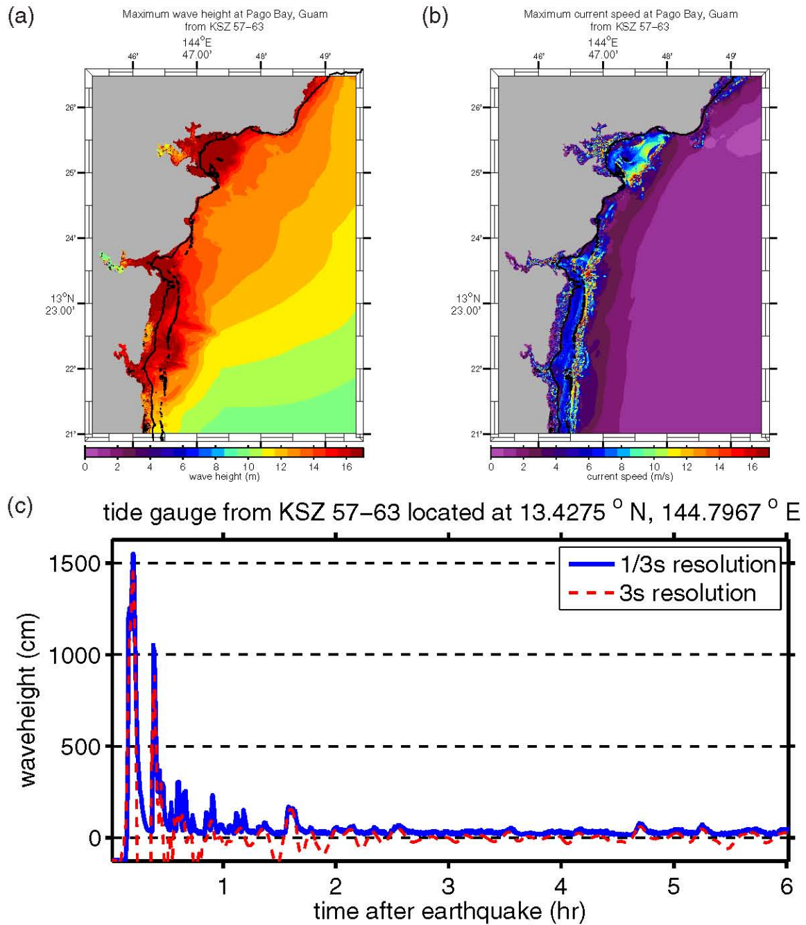
Figure E.15: (a) Maximum computed wave heights, (b) maximum computed currents, and (c) tsunami time history at the numerical tide gauge at Pago Bay from a tsunami triggered by a Mw = 9.0 earthquake on KSZ segments 57–63 by a 20-m slip.
