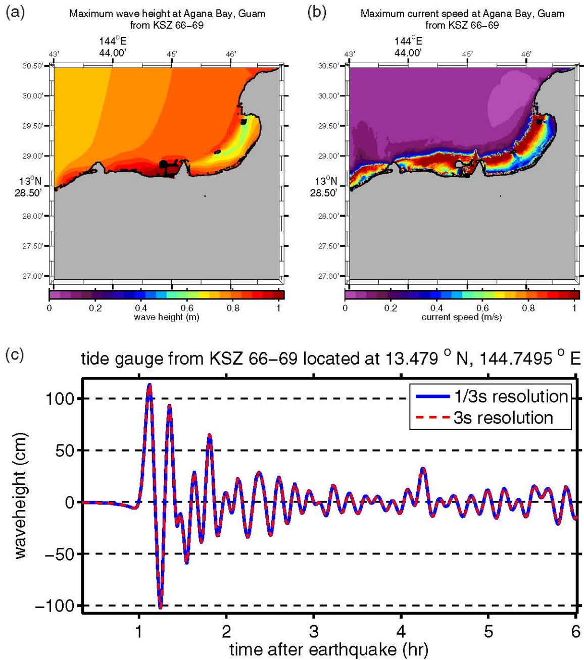
Figure F7: (a) Maximum computed wave heights, (b) maximum computed currents, and (c) tsunami time history at the numerical tide gauge at Agana Bay from a tsunami triggered by a Mw = 8.5 earthquake on KSZ segments 66–69 by a 6-m slip.
