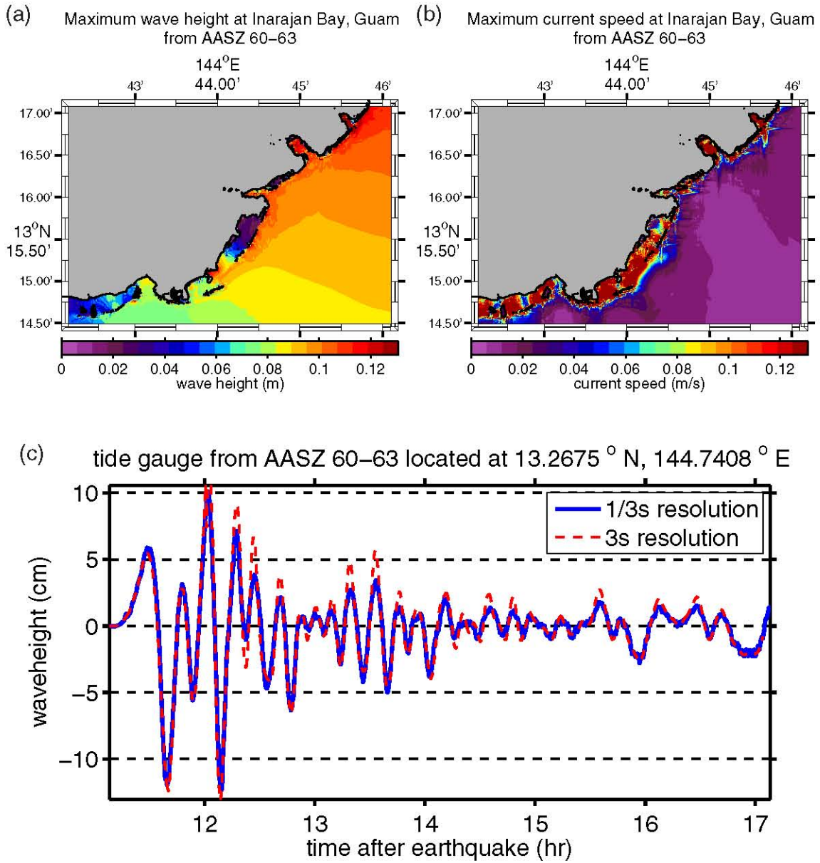
Figure G.3: (a) Maximum computed wave heights, (b) maximum computed currents, and (c) tsunami time history at the numerical tide gauge at Inarajan Bay from a tsunami triggered by a Mw = 8.5 earthquake on AASZ segments 60–63 by a 6-m slip.
