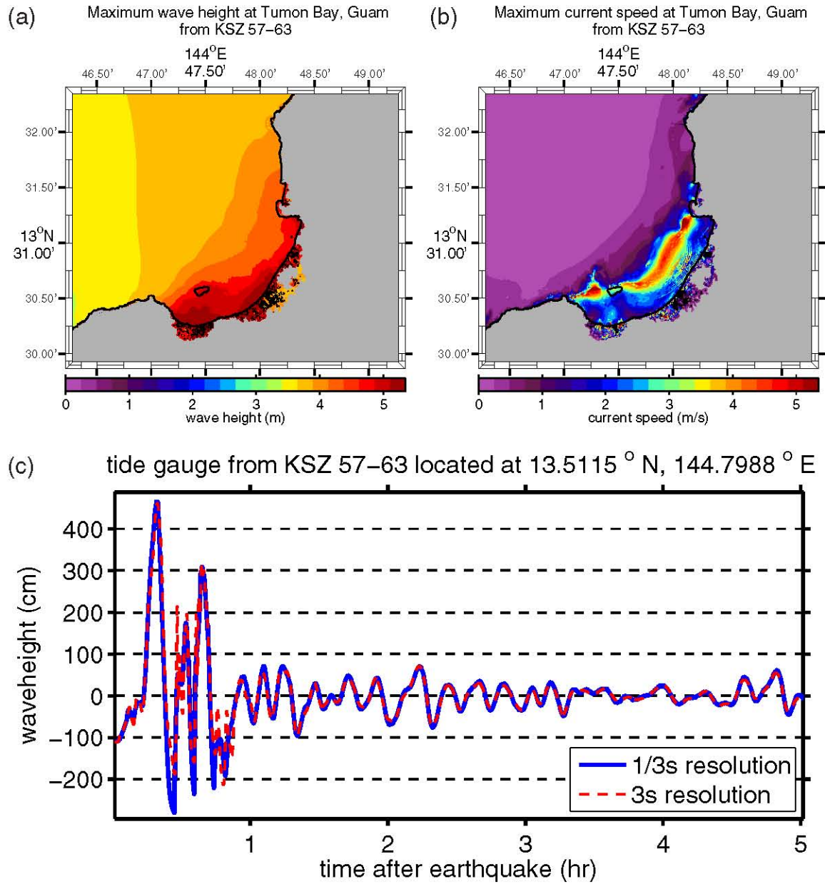
Figure C.15: (a) Maximum computed wave heights, (b) maximum computed currents, and (c) tsunami time history at the numerical tide gauge at Tumon Bay from a tsunami triggered by a Mw = 9.0 earthquake on KSZ segments 57-63 by a 20-m slip.
