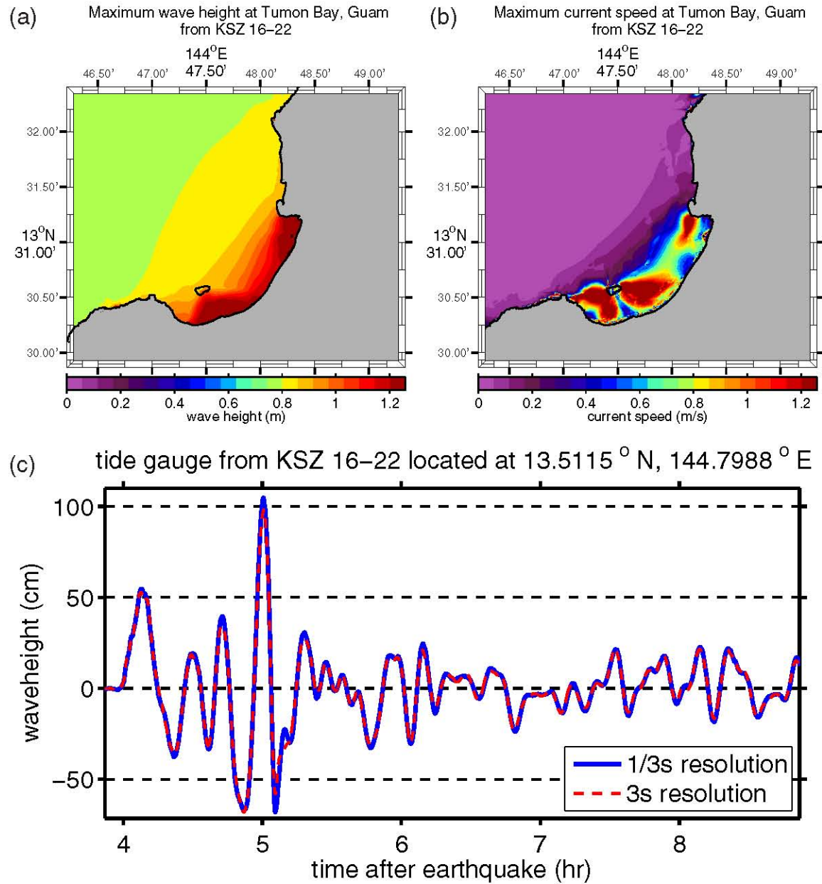
Figure C.14: (a) Maximum computed wave heights, (b) maximum computed currents, and (c) tsunami time history at the numerical tide gauge at Tumon Bay from a tsunami triggered by a M_w = 9.0 earthquake on KSZ segments 16–22 by a 20-m slip.
