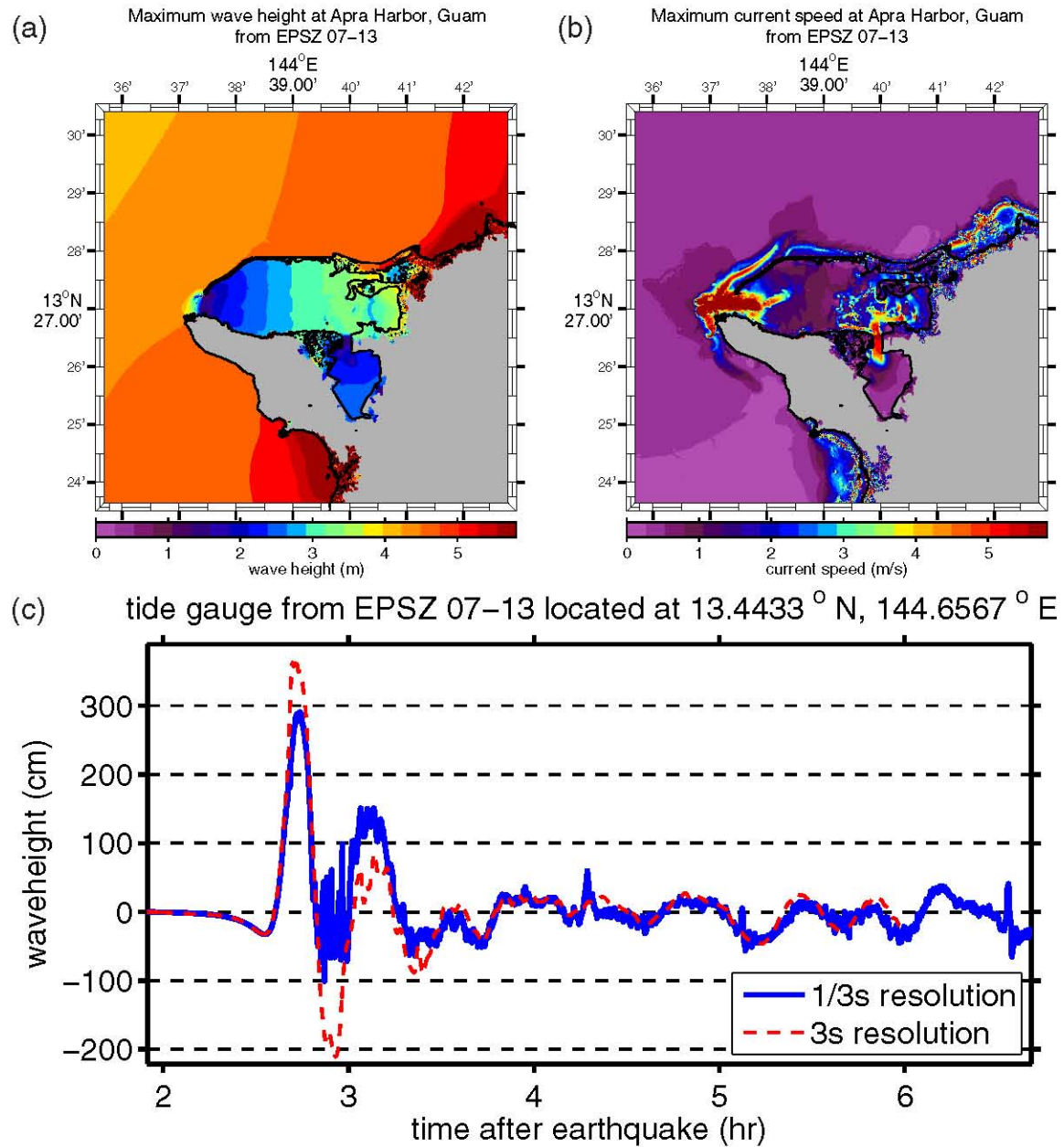
Figure 5.2: (a) Maximum computed wave heights, (b) maximum computed currents, and (c) tsunami time history at the numerical tide gauge at Apra Harbor from a tsunami triggered by a Mw = 9.0 earthquake on EPSZ segments 07–13 by a 20-m slip.
