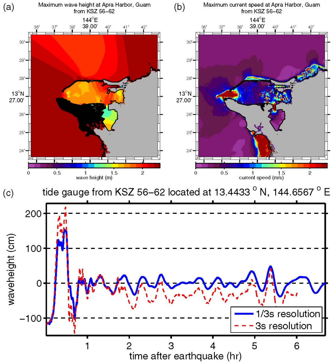
Figure D.15: (a) Maximum computed wave heights, (b) maximum computed currents, and (c) tsunami time history at the numerical tide gauge at Apra Harbor from a tsunami triggered by a Mw = 9.0 earthquake on KSZ segments 56–62 by a 20-m slip.
