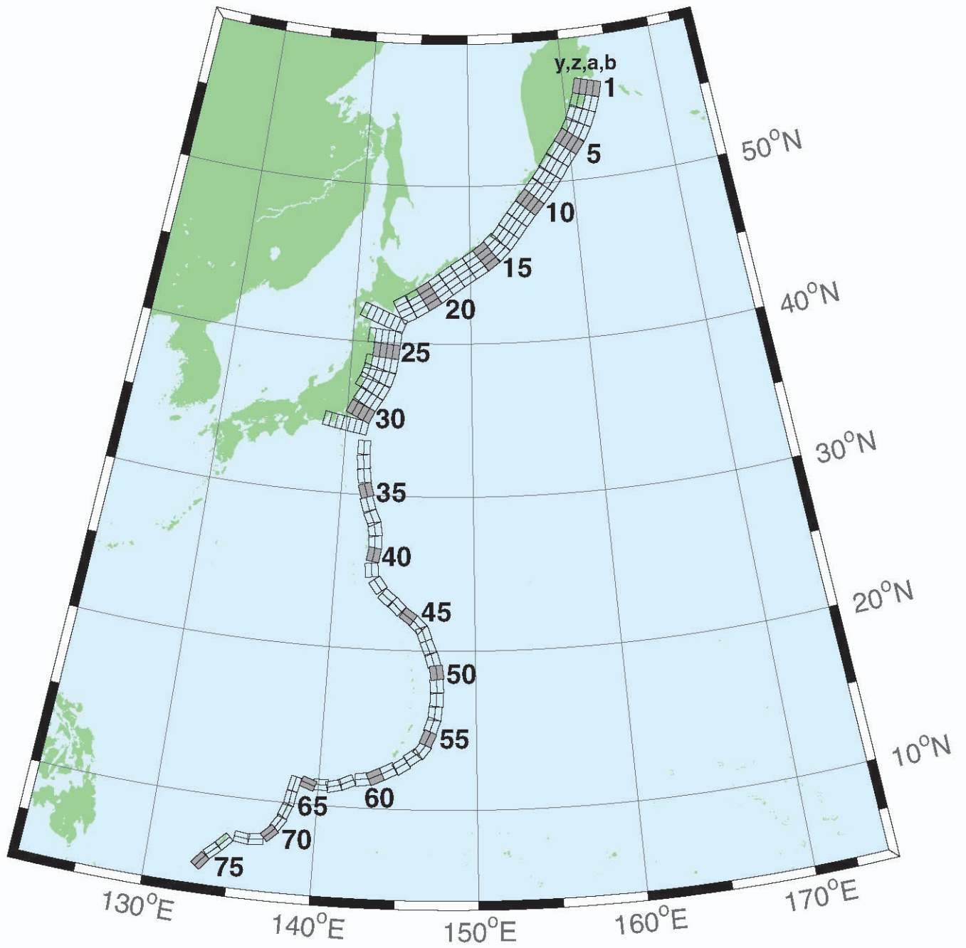
Figure H.4: Kamchatka-Kuril-Japan-Izu-Mariana-Yap Subduction Zone unit sources.
