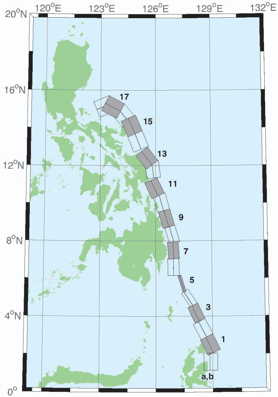
Figure H.3: Eastern Philippines Subduction Zone unit sources.
