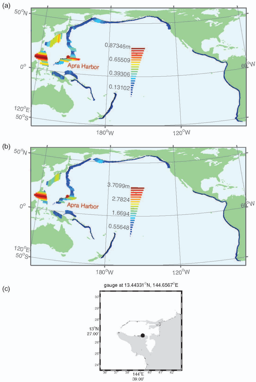
Figure D.1: Tsunami wave height response at Apra Harbor from tsunamis triggered by (a) Mw = 8.5 and (b) Mw = 9.0 earthquakes.
