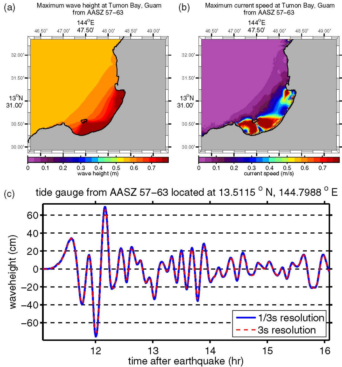
Figure C.12: (a) Maximum computed wave heights, (b) maximum computed currents, and (c) tsunami time history at the numerical tide gauge at Tumon Bay from a tsunami triggered by a M_w = 9.0 earthquake on AASZ segments 57–63 by a 20-m slip.
