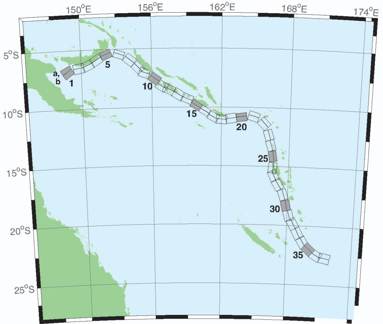
Figure H.8: New Britain-Solomons-Vanuatu Zone unit sources.
