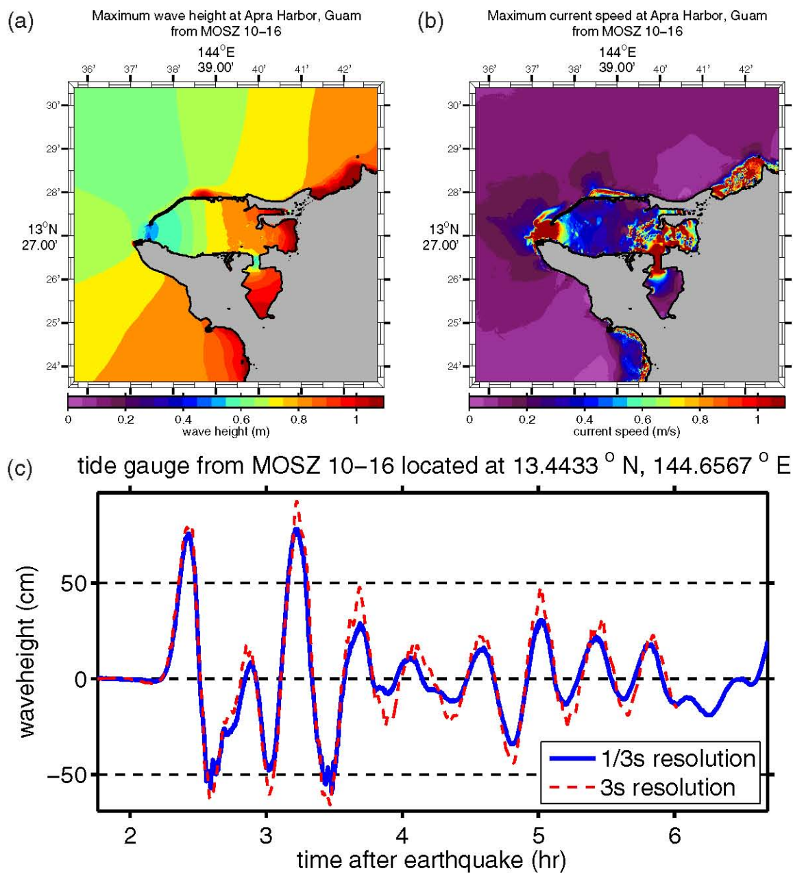
Figure D.16: (a) Maximum computed wave heights, (b) maximum computed currents, and (c) tsunami time history at the numerical tide gauge at Apra Harbor from a tsunami triggered by a Mw = 9.0 earthquake on MOSZ segments 10–16 by a 20-m slip.
