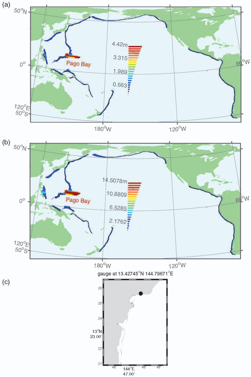
Figure E.1: Tsunami wave height response at Pago Bay from tsunamis triggered by (a) Mw = 8.5 and (b) Mw = 9.0 earthquakes.
