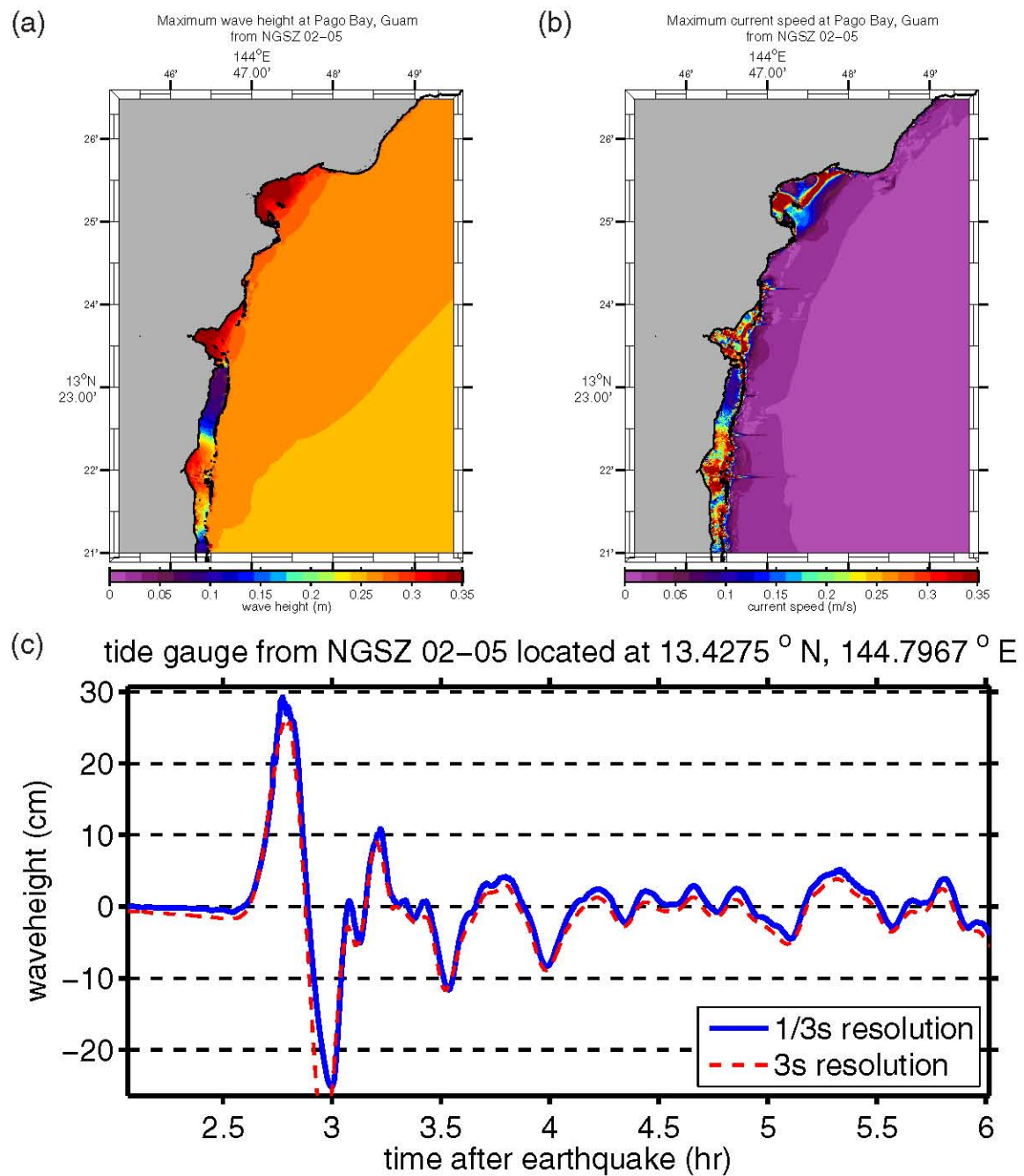
Figure E.8: (a) Maximum computed wave heights, (b) maximum computed currents, and (c) tsunami time history at the numerical tide gauge at Pago Bay from a tsunami triggered by a M_w = 8.5 earthquake on NGSZ segments 02–05 by a 6-m slip.
