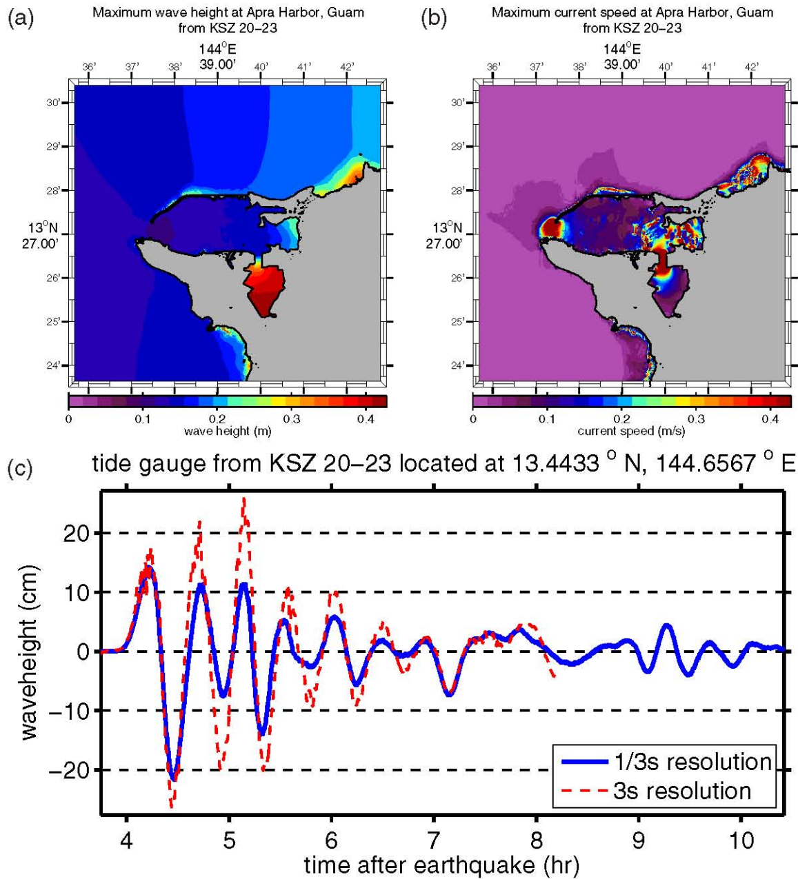
Figure D.5: (a) Maximum computed wave heights, (b) maximum computed currents, and (c) tsunami time history at the numerical tide gauge at Apra Harbor from a tsunami triggered by a Mw = 8.5 earthquake on KSZ segments 20–23 by a 6-m slip.
