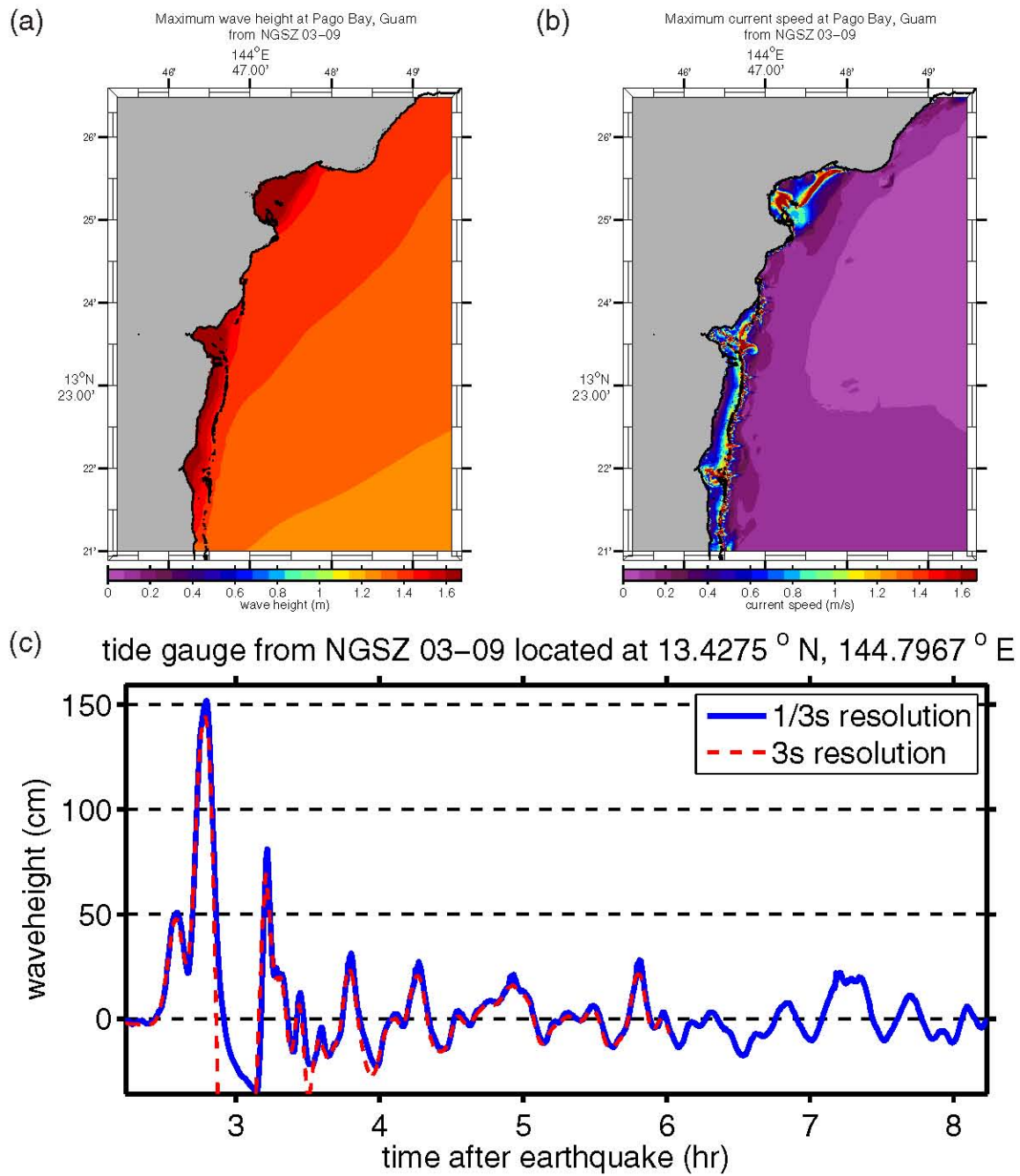
Figure E.17: (a) Maximum computed wave heights, (b) maximum computed currents, and (c) tsunami time history at the numerical tide gauge at Pago Bay from a tsunami triggered by a Mw = 9.0 earthquake on NGSZ segments 03–09 by a 20-m slip.
