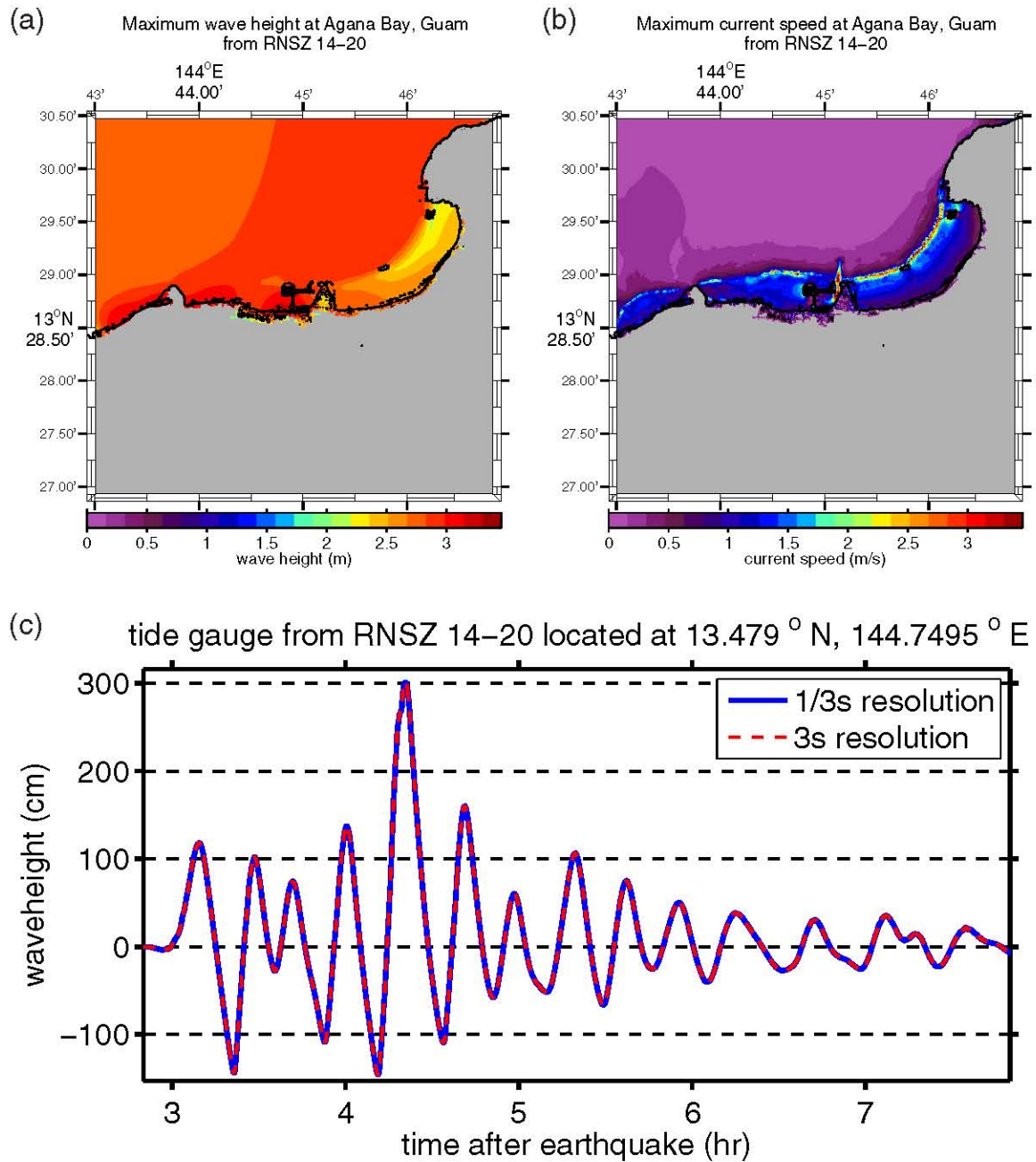
Figure E.19: (a) Maximum computed wave heights, (b) maximum computed currents, and (c) tsunami time history at the numerical tide gauge at Agana Bay from a tsunami triggered by a Mw = 9.0 earthquake on RNSZ segments 14-20 by a 20-m slip.
