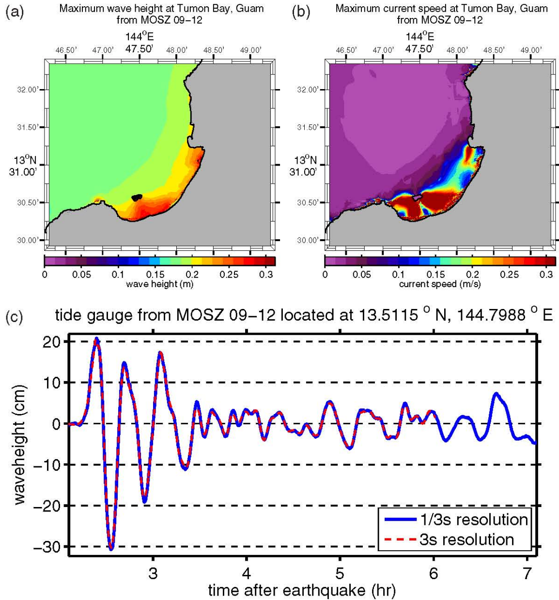
Figure C.8: (a) Maximum computed wave heights, (b) maximum computed currents, and (c) tsunami time history at the numerical tide gauge at Tumon Bay from a tsunami triggered by a M_w = 8.5 earthquake on MOSZ segments 09–12 by a 6-m slip.
