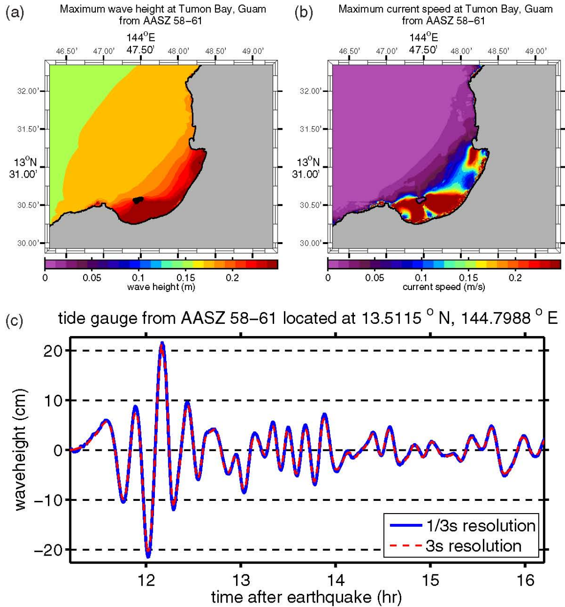
Figure C.3: (a) Maximum computed wave heights, (b) maximum computed currents, and (c) tsunami time history at the numerical tide gauge at Tumon Bay from a tsunami triggered by a Mw = 8.5 earthquake on AASZ segments 58–61 by a 6-m slip.
