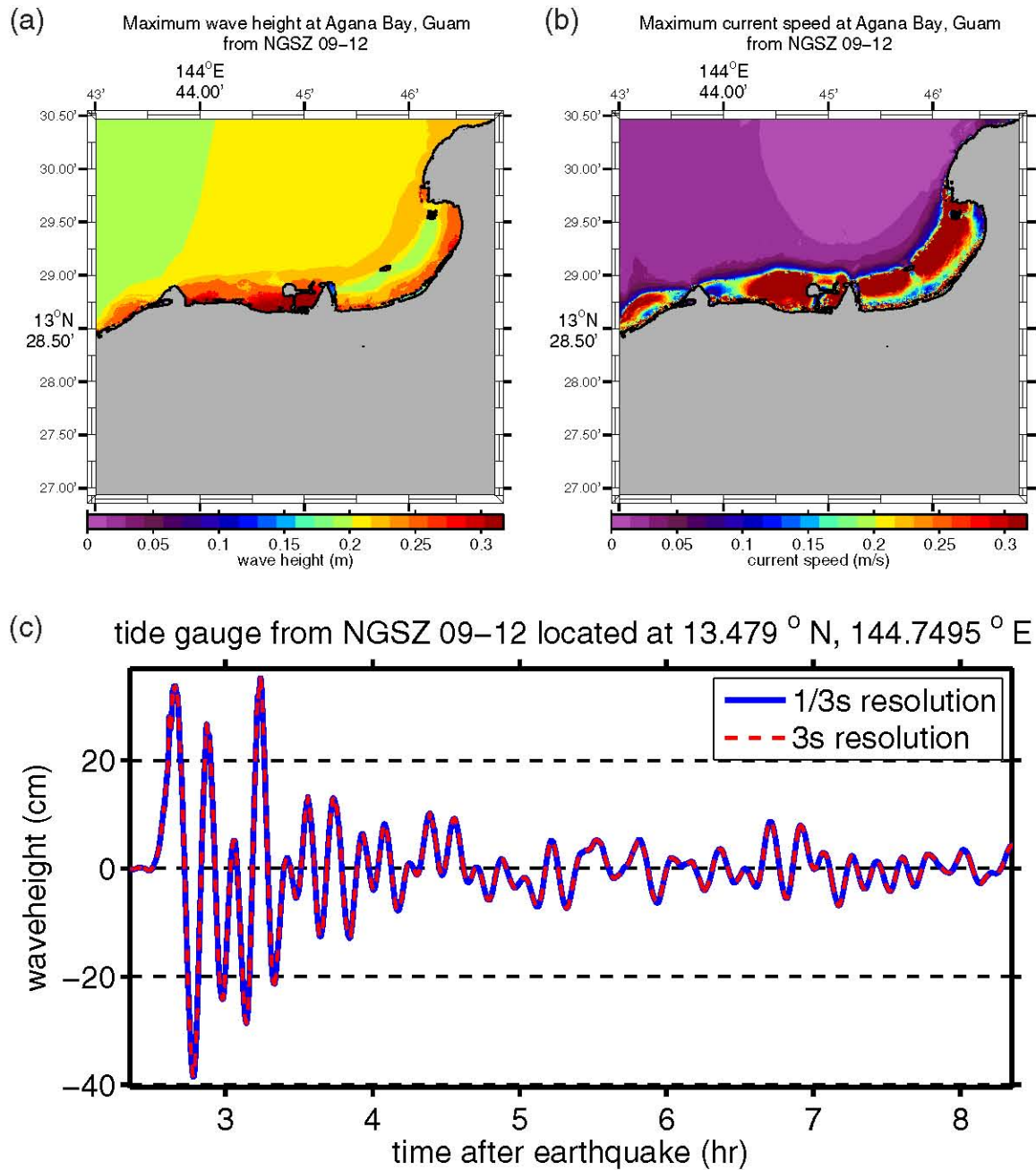
Figure F.9: (a) Maximum computed wave heights, (b) maximum computed currents, and (c) tsunami time history at the numerical tide gauge at Agana Bay from a tsunami triggered by a Mw = 8.5 earthquake on NGSZ segments 09–12 by a 6-m slip.
