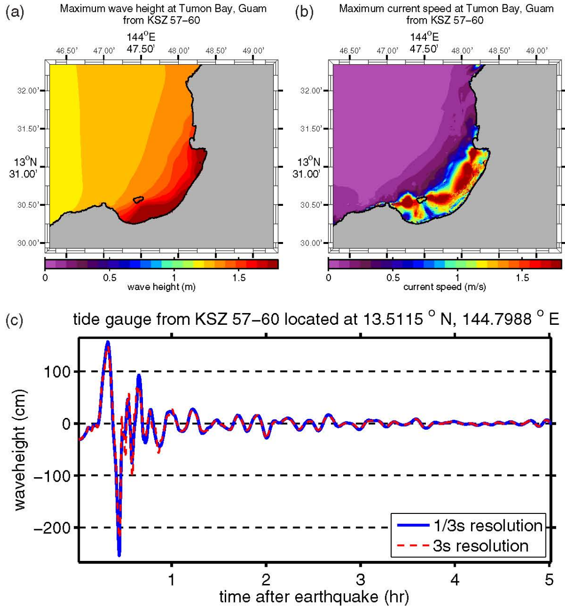
Figure C.6: (a) Maximum computed wave heights, (b) maximum computed currents, and (c) tsunami time history at the numerical tide gauge at Tumon Bay from a tsunami triggered by a M_w = 8.5 earthquake on KSZ segments 57–60 by a 6-m slip.
