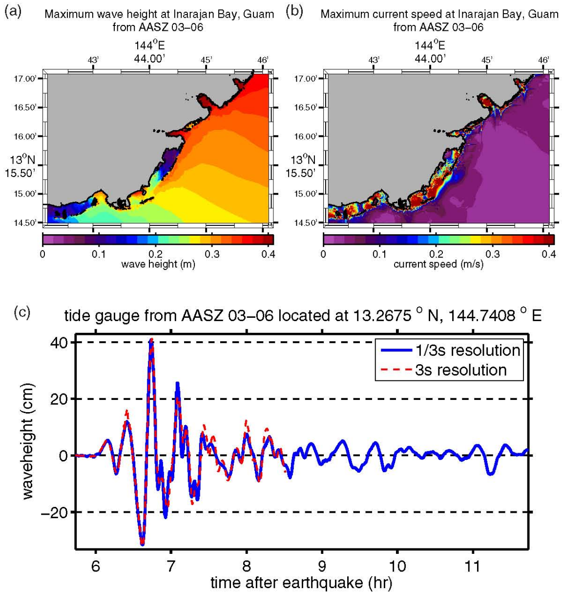
Figure G.2: (a) Maximum computed wave heights, (b) maximum computed currents, and (c) tsunami time history at the numerical tide gauge at Inarajan Bay from a tsunami triggered by a M_w = 8.5 earthquake on AASZ segments 03–06 by a 6-m slip.
