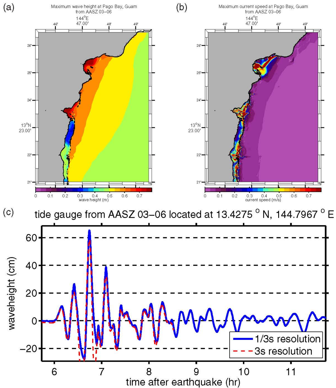
Figure E.2: (a) Maximum computed wave heights, (b) maximum computed currents, and (c) tsunami time history at the numerical tide gauge at Pago Bay from a tsunami triggered by a M_w = 8.5 earthquake on AASZ segments 03–06 by a 6-m slip.
