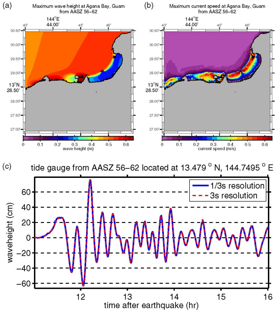
Figure E.13: (a) Maximum computed wave heights, (b) maximum computed currents, and (c) tsunami time history at the numerical tide gauge at Agana Bay from a tsunami triggered by a Mw = 9.0 earthquake on AASZ segments 56–62 by a 20-m slip.
