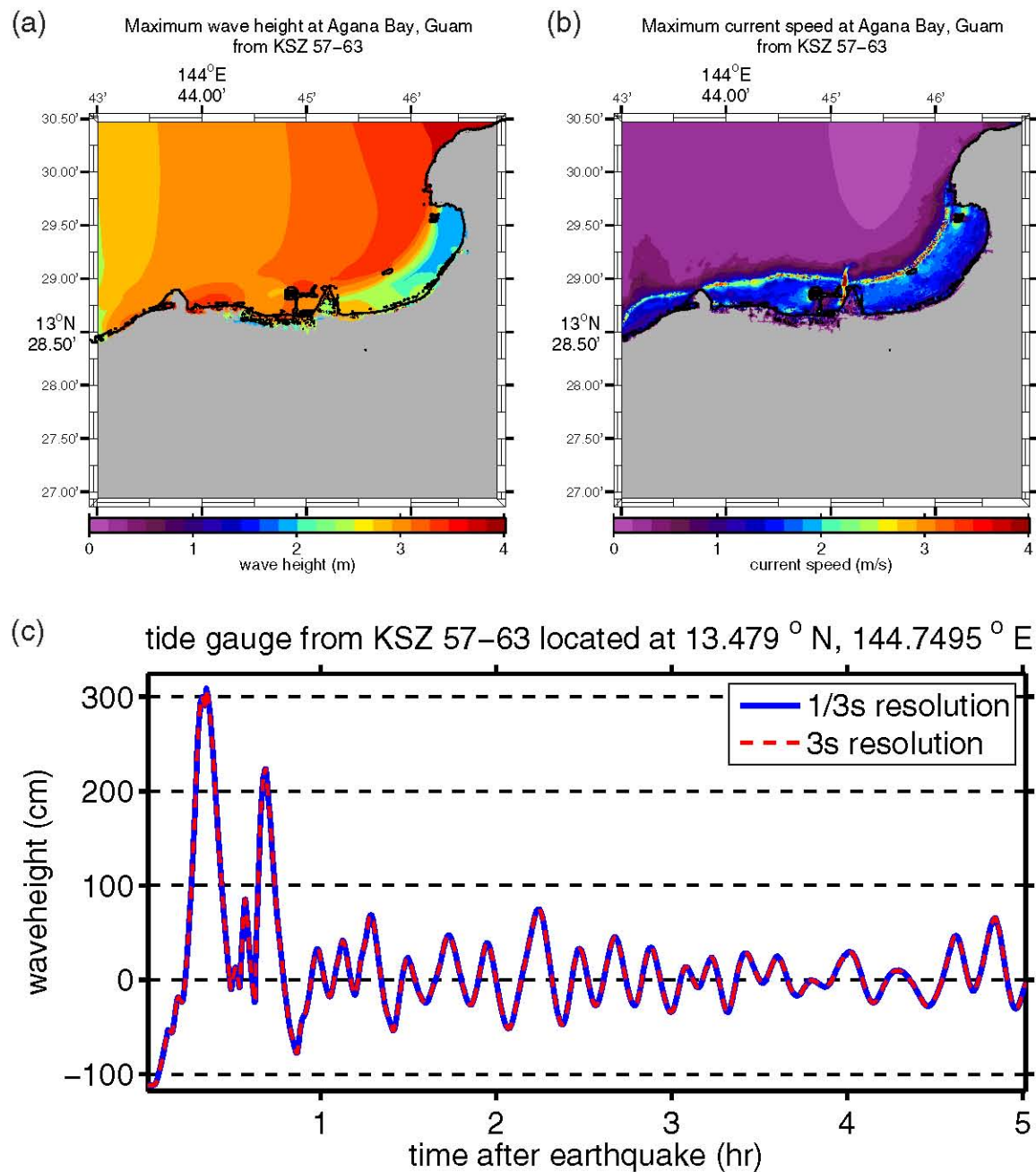
Figure E.16: (a) Maximum computed wave heights, (b) maximum computed currents, and (c) tsunami time history at the numerical tide gauge at Agana Bay from a tsunami triggered by a M_w = 9.0 earthquake on KSZ segments 57–63 by a 20-m slip.
