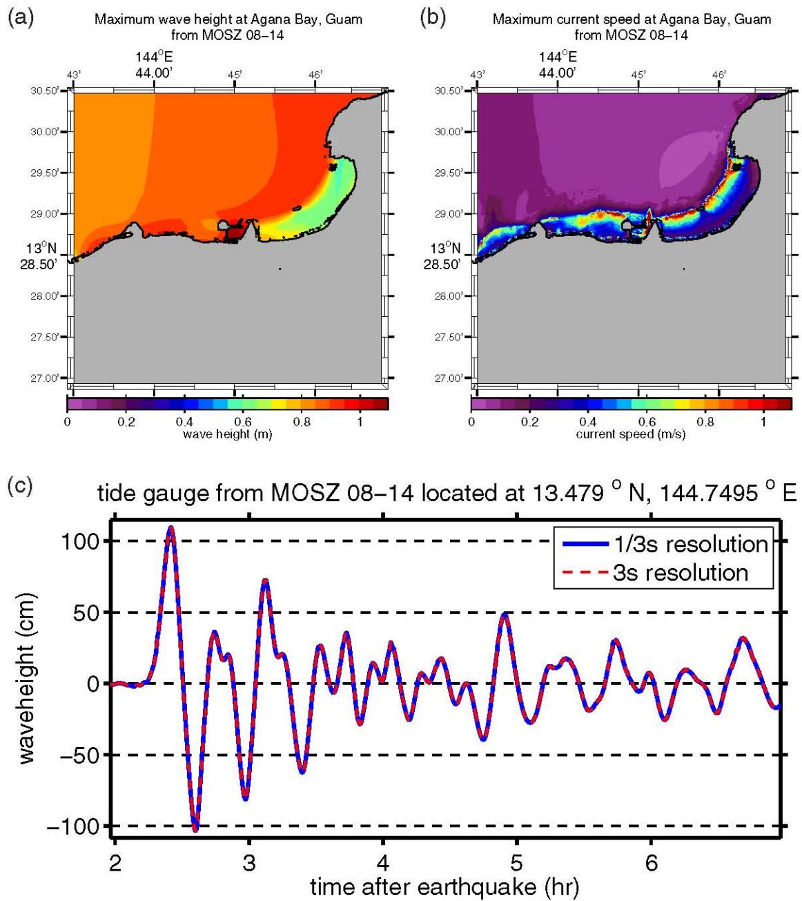
Figure E.17: (a) Maximum computed wave heights, (b) maximum computed currents, and (c) tsunami time history at the numerical tide gauge at Agana Bay from a tsunami triggered by a Mw = 9.0 earthquake on MOSZ segments 08–14 by a 20-m slip.
