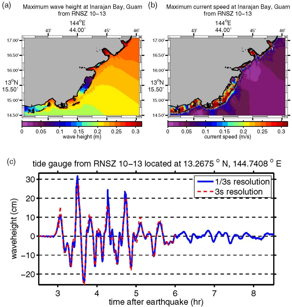
Figure G.9: (a) Maximum computed wave heights, (b) maximum computed currents, and (c) tsunami time history at the numerical tide gauge at Inarajan Bay from a tsunami triggered by a Mw = 8.5 earthquake on RNSZ segments 10–13 by a 6-m slip.
