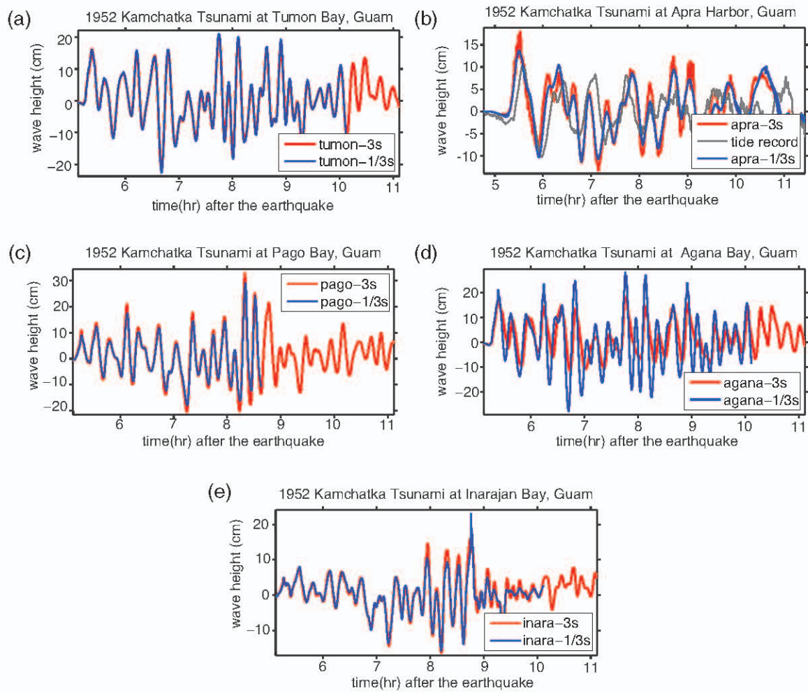
Figure 3.5: Comparison of computed 1952 tsunami with 1/3 arc sec to 3 arc sec at (a) Tumon Bay, (b) Apra Harbor, (c) Pago Bay, (d) Agana Bay, and (e) Inarajan Bay.
