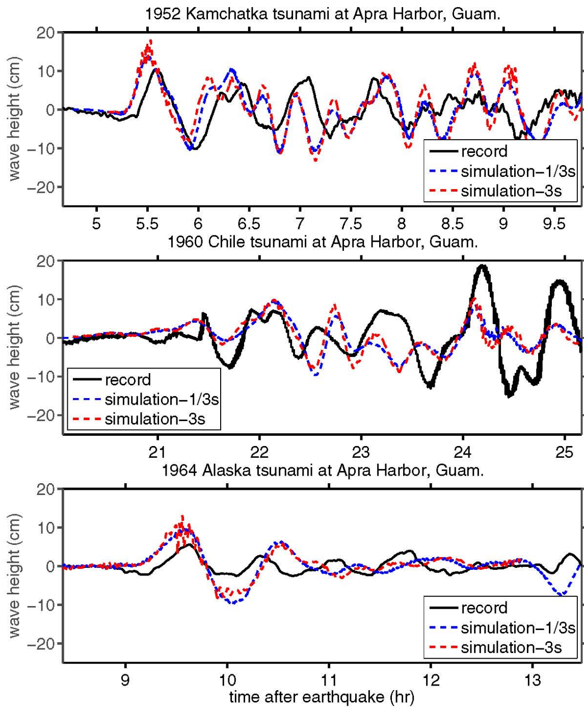
Figure B.2: The 1952 Kamchatka, the 1960 Chile and the 1964 Alaska Tsunamis at Apra Harbor tide gauge.
