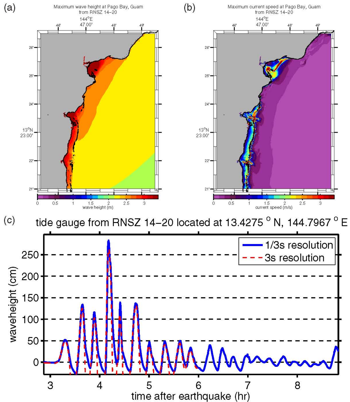
Figure E.18: (a) Maximum computed wave heights, (b) maximum computed currents, and (c) tsunami time history at the numerical tide gauge at Pago Bay from a tsunami triggered by a Mw = 9.0 earthquake on RNSZ segments 14–20 by a 20-m slip.
