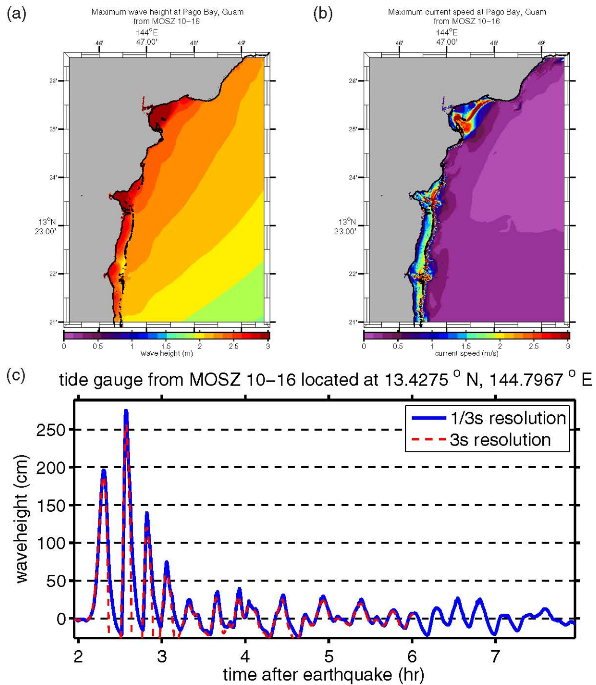
Figure E.16: (a) Maximum computed wave heights, (b) maximum computed currents, and (c) tsunami time history at the numerical tide gauge at Pago Bay from a tsunami triggered by a Mw = 9.0 earthquake on MOSZ segments 10–16 by a 20-m slip.
