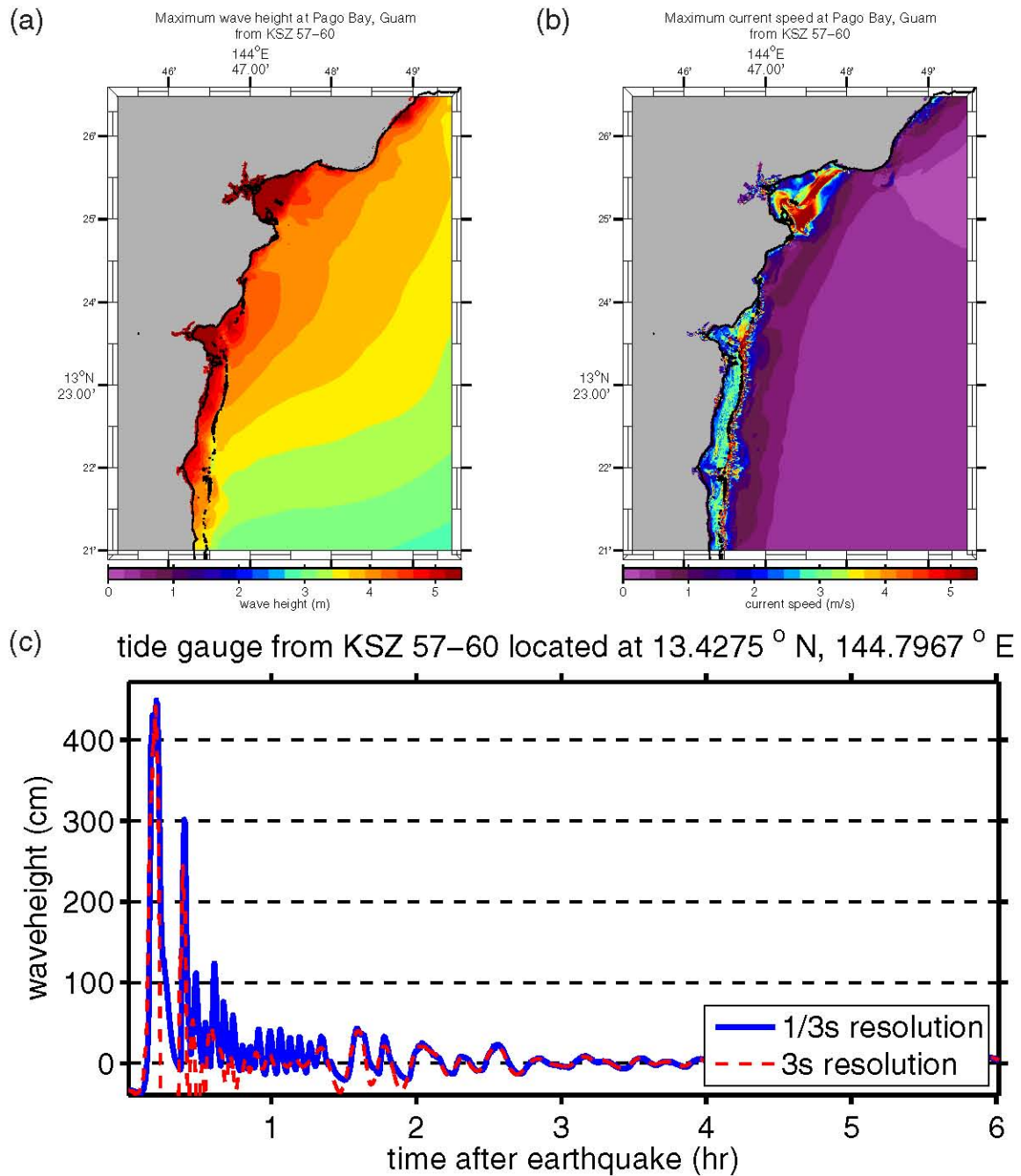
Figure E.6: (a) Maximum computed wave heights, (b) maximum computed currents, and (c) tsunami time history at the numerical tide gauge at Pago Bay from a tsunami triggered by a M_w = 8.5 earthquake on KSZ segments 57-60 by a 6-m slip.
