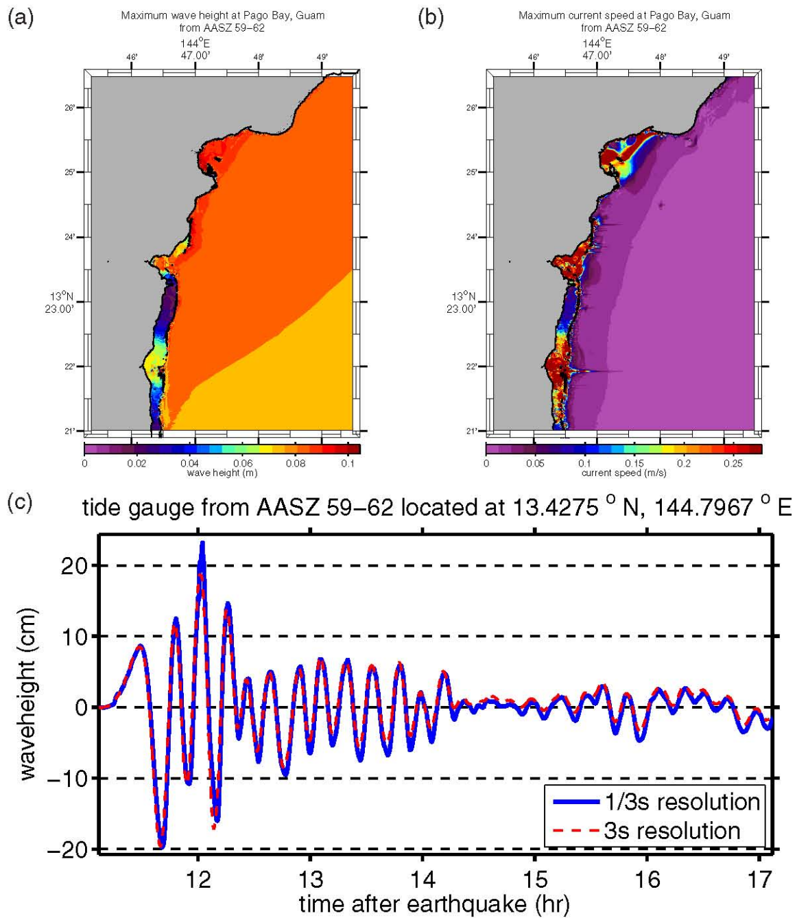
Figure E.3: (a) Maximum computed wave heights, (b) maximum computed currents, and (c) tsunami time history at the numerical tide gauge at Pago Bay from a tsunami triggered by a Mw = 8.5 earthquake on AASZ segments 59–62 by a 6-m slip.
