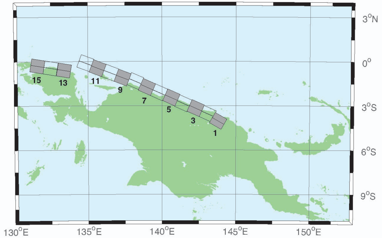
Figure H.6: New Guinea Subduction Zone unit sources.
