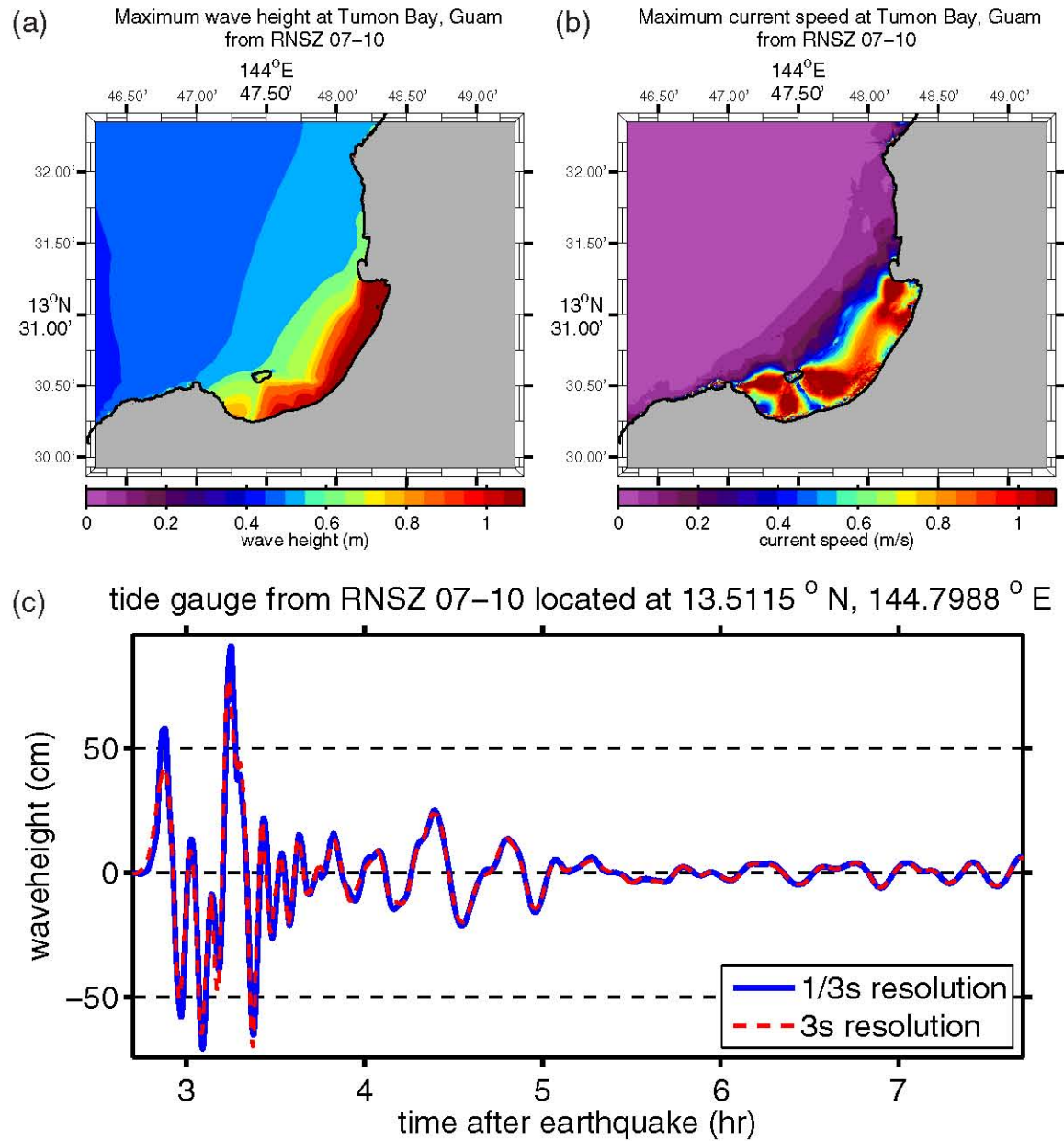
Figure C.10: (a) Maximum computed wave heights, (b) maximum computed currents, and (c) tsunami time history at the numerical tide gauge at Tumon Bay from a tsunami triggered by a M_w = 8.5 earthquake on RNSZ segments 07–10 by a 6-m slip.
