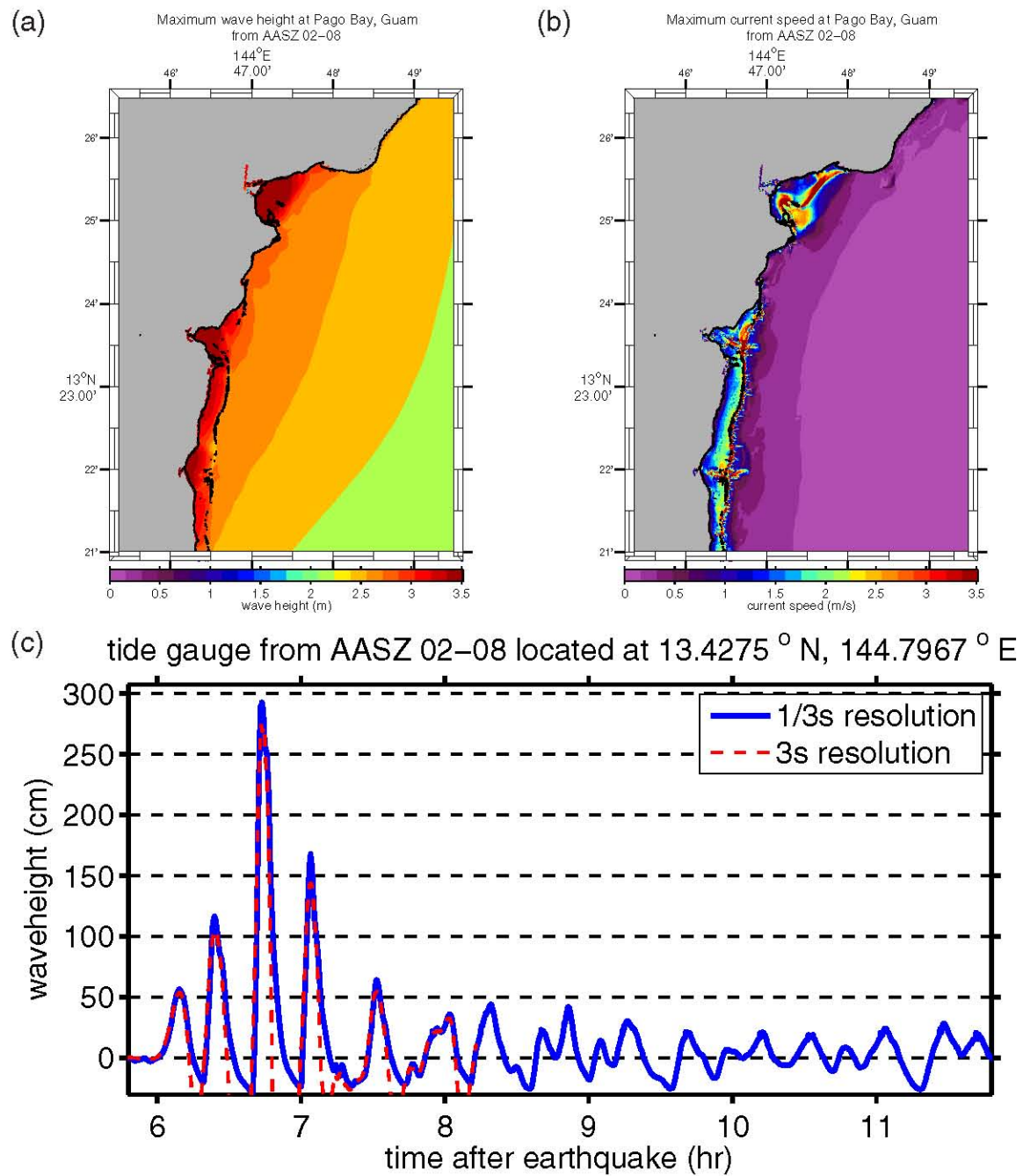
Figure E.10: (a) Maximum computed wave heights, (b) maximum computed currents, and (c) tsunami time history at the numerical tide gauge at Pago Bay from a tsunami triggered by a M_w = 9.0 earthquake on AASZ segments 02–08 by a 20-m slip.
