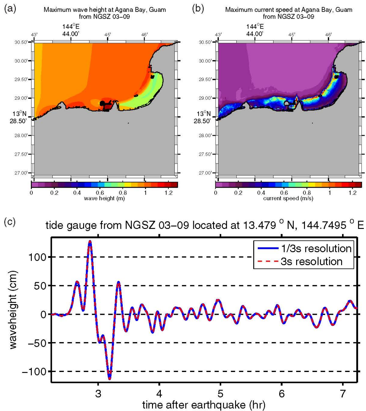
Figure E18: (a) Maximum computed wave heights, (b) maximum computed currents, and (c) tsunami time history at the numerical tide gauge at Agana Bay from a tsunami triggered by a M_w = 9.0 earthquake on NGSZ segments 03–09 by a 20-m slip.
