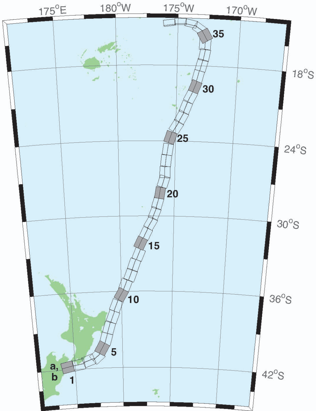
Figure H.7: New Zealand-Keradec-Tonga Subduction Zone unit sources.
