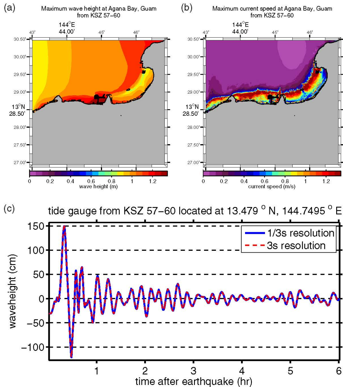
Figure F6: (a) Maximum computed wave heights, (b) maximum computed currents, and (c) tsunami time history at the numerical tide gauge at Agana Bay from a tsunami triggered by a Mw = 8.5 earthquake on K SZ segments 57–60 by a 6-m slip.
