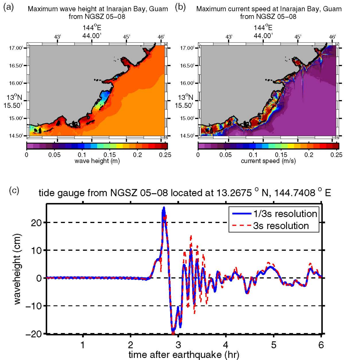
Figure G.8: (a) Maximum computed wave heights, (b) maximum computed currents, and (c) tsunami time history at the numerical tide gauge at Inarajan Bay from a tsunami triggered by a M_w = 8.5 earthquake on NGSZ segments 05–08 by a 6-m slip.
