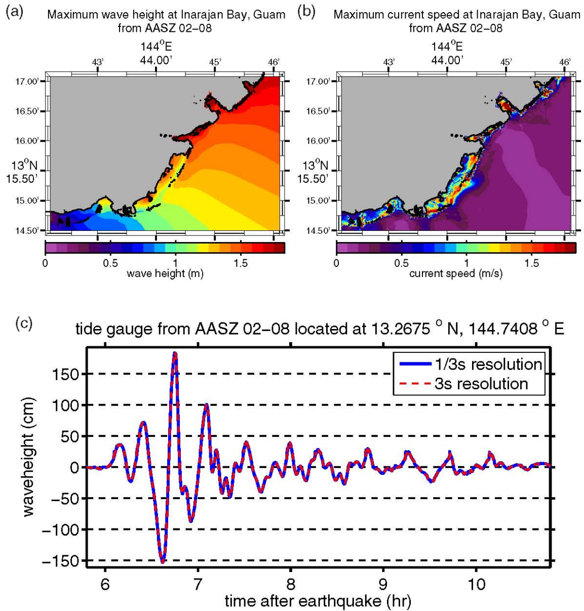
Figure G.10: (a) Maximum computed wave heights, (b) maximum computed currents, and (c) tsunami time history at the numerical tide gauge at Inarajan Bay from a tsunami triggered by a M_w = 9.0 earthquake on AASZ segments 02–08 by a 20-m slip.
