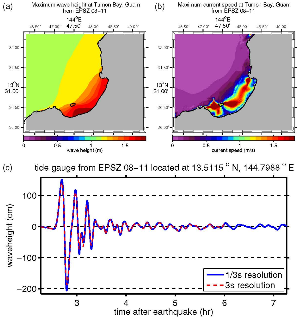
Figure C.4: (a) Maximum computed wave heights, (b) maximum computed currents, and (c) tsunami time history at the numerical tide gauge at Tumon Bay from a tsunami triggered by a M_w = 8.5 earthquake on EPSZ segments 08–11 by a 6-m slip.
