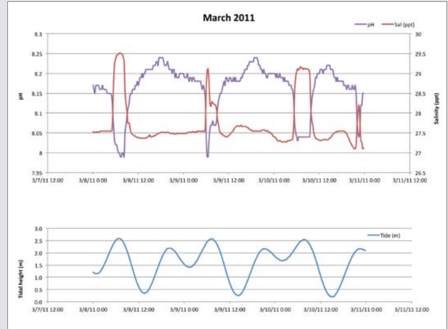
Figure 33. Salinity (ppt), tide (m), and pH NBS at the Lummi tide gate in March 2011.
