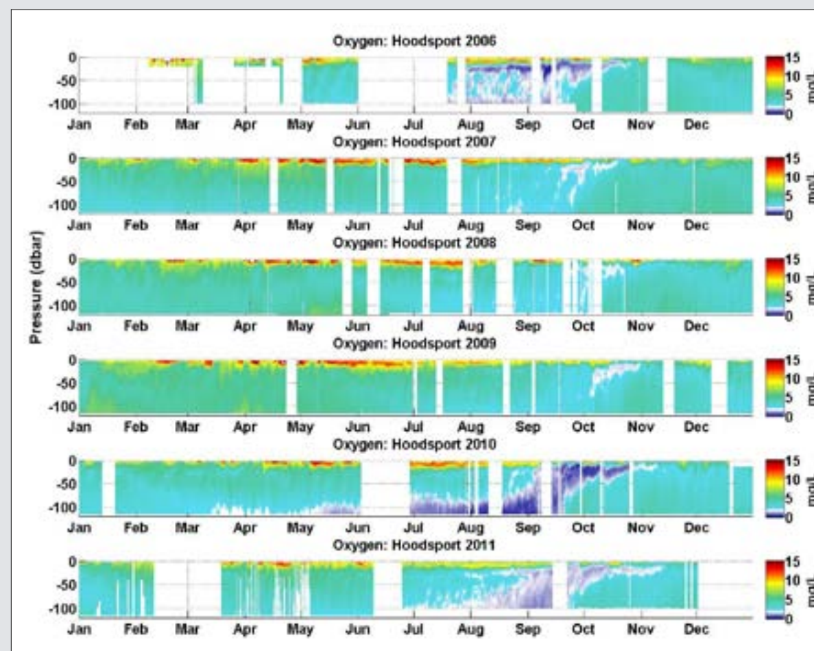
Figure 24. Oxygen profiles from the Hoodsport mooring in southern Hood Canal from 2006 to 2011. Pressure in dbar is roughly equivalent to depth in meters.
