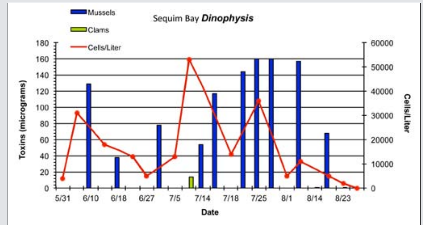
Figure 35. DSP toxins in mussels and clams and Dinophysis spp. cells counts in Sequim Bay from May through August 2011. Note that oysters were also sampled on August 14 and August 23, 2011, but DSP levels were low (0 and 0.4 micrograms, respectively).
