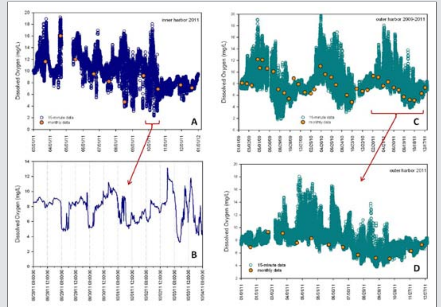
Figure 29. Dissolved oxygen (mg/L) in Quartermaster Harbor compiled from two dockside moorings at Dockton (7-m depth) in the outer harbor and the Yacht Club (1-m depth) in the inner harbor.
