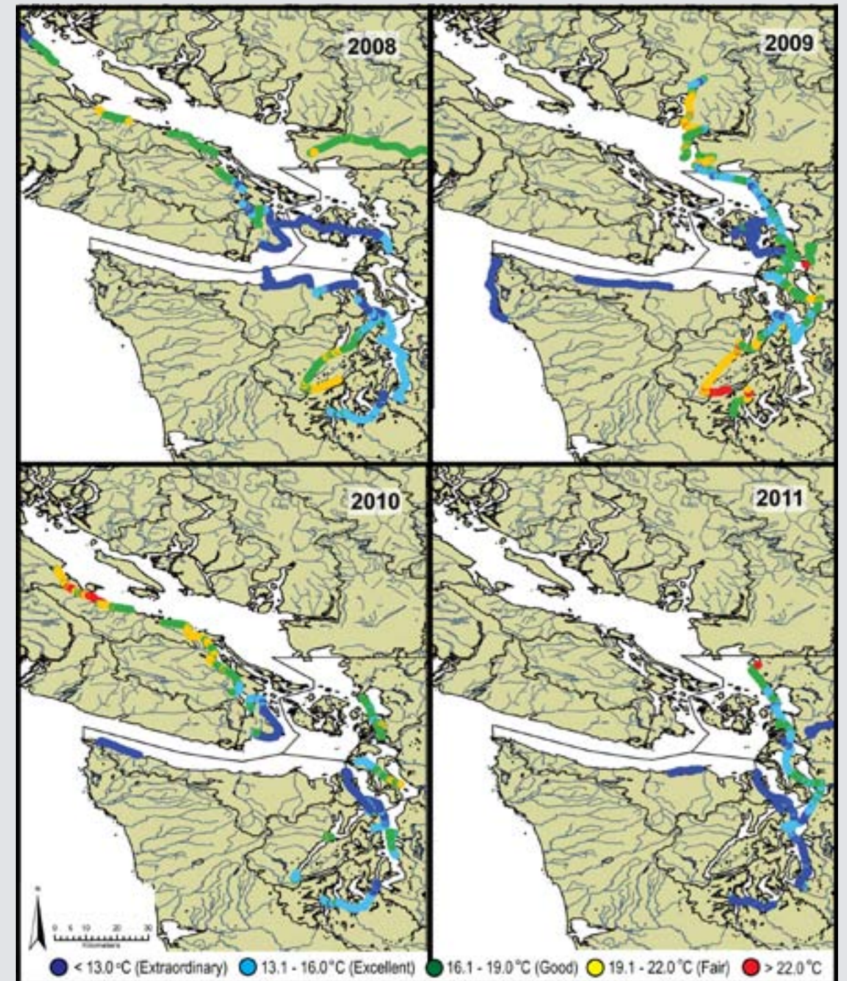
Figure 14. Map showing the results of surface temperature measurements during the 2008 to 2011 TJWQP mapped by Washington State Marine Water Quality Standard classifications.
