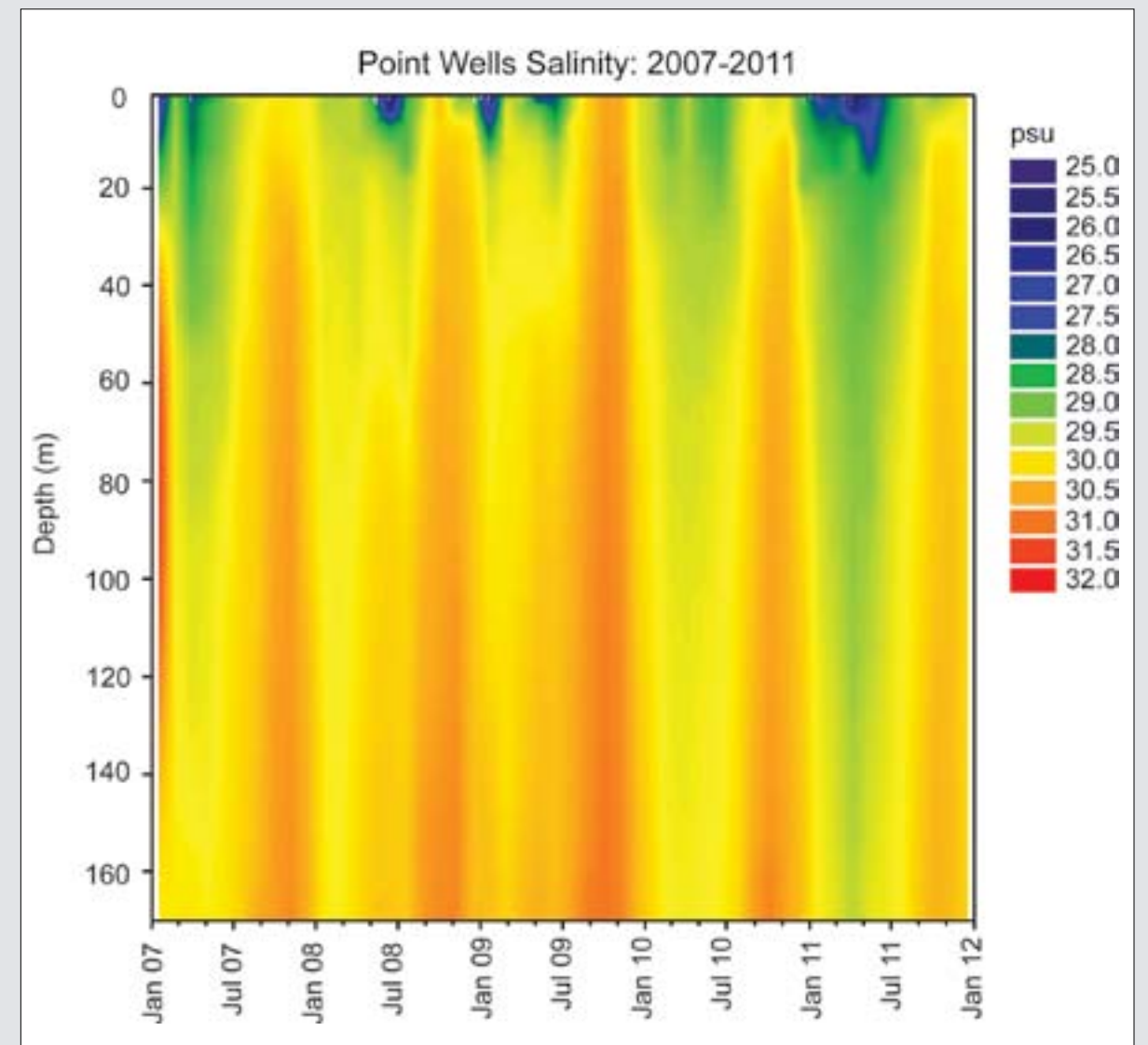
Figure 13. Contours of monthly water column salinity profile data for a northern Central Basin site (Point Wells) showing the increased freshwater input during the wet spring months for the last five years.
