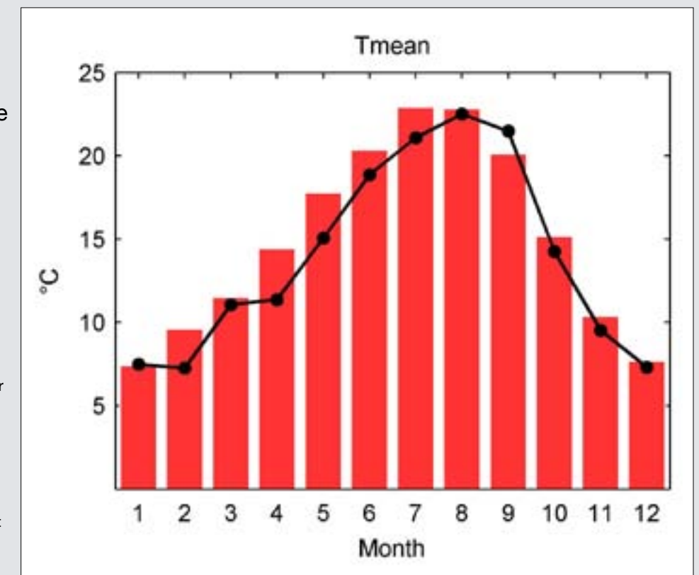
Figure 4. Monthly climatology and 2011 weather conditions for the Puget Sound region. Bars show the monthly mean values; dotted lines indicate 2011 values. Opposite page: Snow water equivalent, Stevens Pass, WA SNOTEL site. This page, top: Monthly precipitation averaged over six long-term Puget Sound stations from the US Historical Climate Network (Bellingham, Blaine, Everett, Olga, Port Townsend, and Seattle). This page, bottom: Monthly mean temperature averages from the same six long-term Puget Sound stations.
