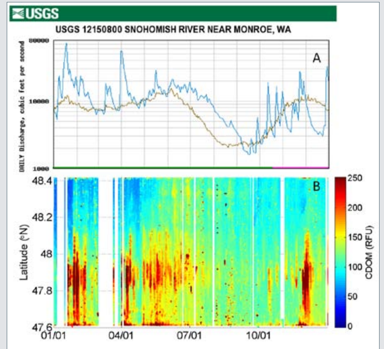
Figure 20. (A) 2011 Snohomish River discharge (blue) and historical average (brown). (B) CDOM (Colored Dissolved Organic Matter) fluorescence along Clipper transect from Elliott Bay to Victoria, B.C.
