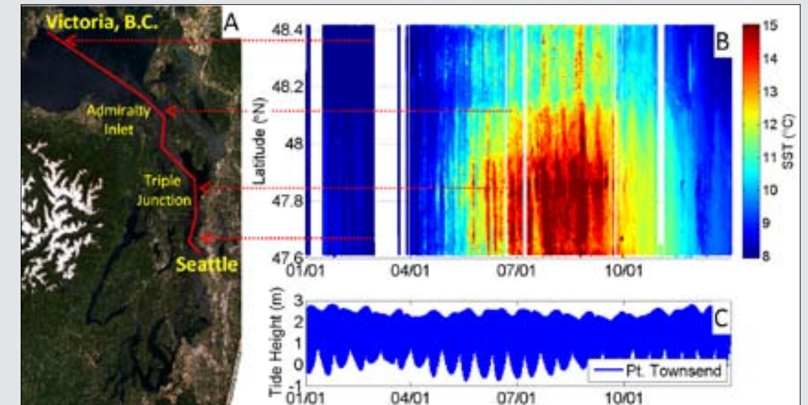
Figure 11. (A) Orientation of the Victoria Clipper transect. (B) SST gradient from Elliott Bay to Strait of Juan de Fuca. (C) Spring/neap tide variability
