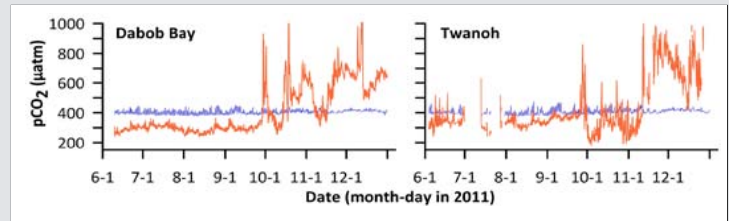
Figure 31. Moored time series measurements of pCO 2 in air (blue, ~1 m above water surface) and water (orange, ~1 m below water surface) at Dabob Bay and Twanoh ORCA buoy sites in Hood Canal.
