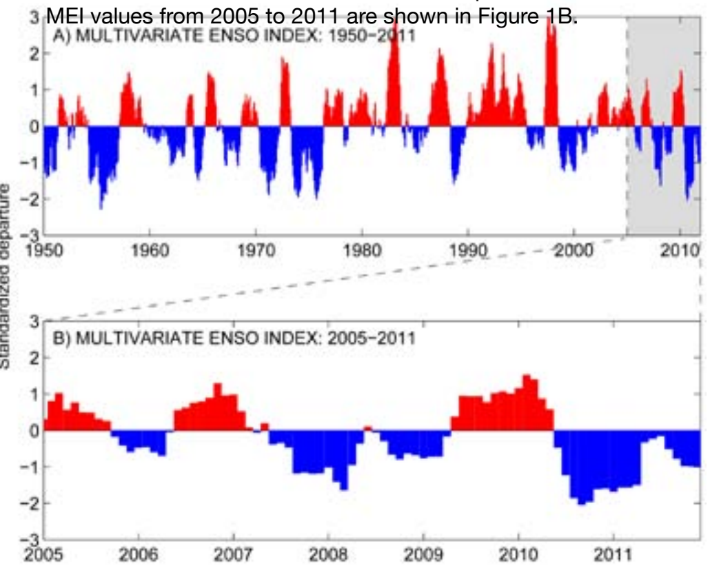
Figure 1. NOAA Physical Sciences Division attempts to monitor ENSO by basing the Multivariate ENSO Index (MEI) on the six main observed variables over the Pacific. These six variables are: sea-level pressure, zonal and meridional components of the surface wind, sea surface temperature, surface air temperature, and total cloudiness fraction of the sky. Monthly values of the MEI are shown from (A) 1950 to
