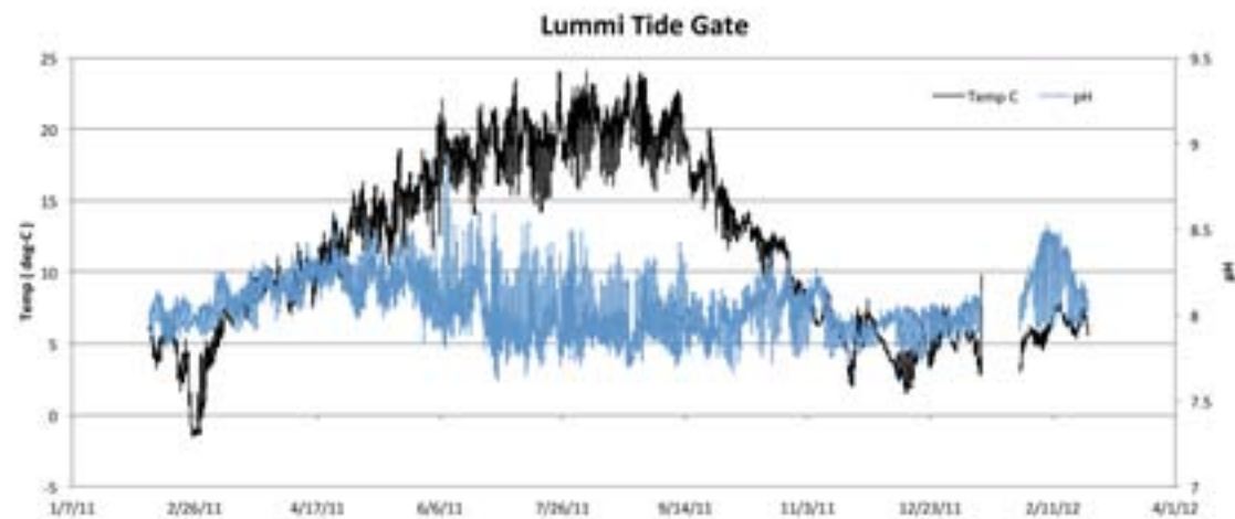
Figure 32. Temperature and pH NBS at the Lummi tide gate in 2011.
