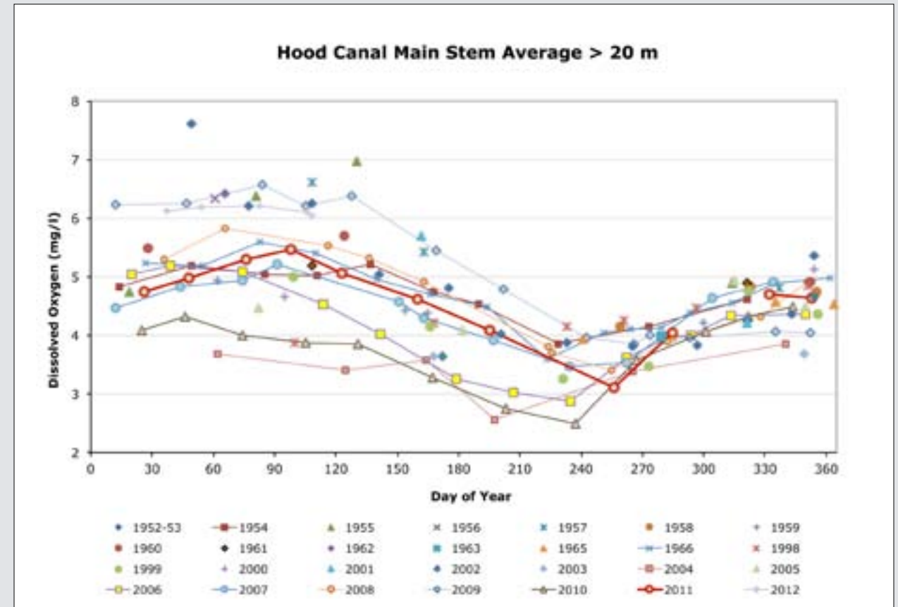
Figure 27. The average dissolved oxygen concentration in the water below 20 meters depth in the region between Dabob Bay and the Great Bend (PRISM Station 11) plotted versus the day of the year. There are two important aspects of this figure to note: the annual cycle in the dissolved oxygen concentrations and the interannual variability.
