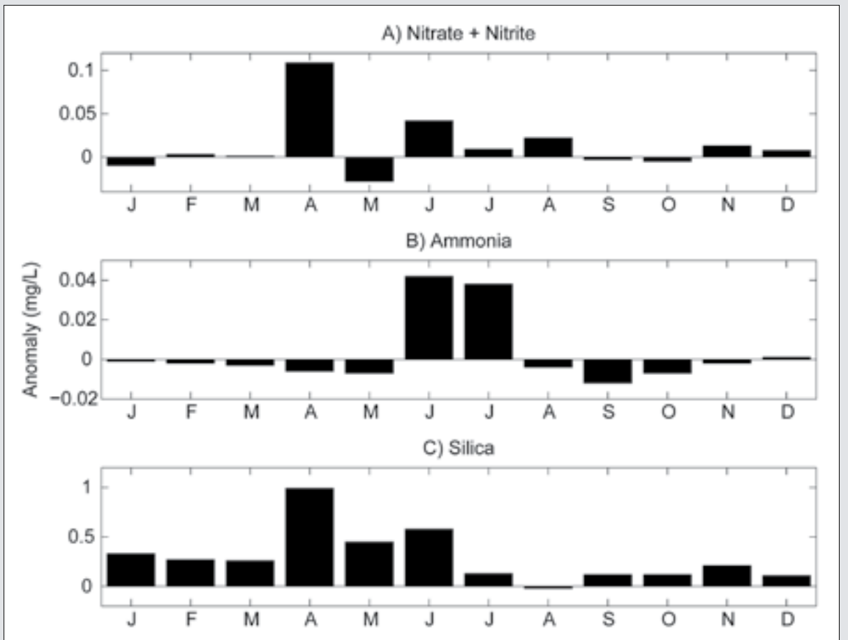
Figure 22. These figures show 2011 anomalies for 12 open water sites for (A) nitrate and nitrite, (B) ammonia, and (C) silica. Anomalies were calculated using a 12-year dataset for surface waters <2 m. The positive nitrate+nitrite and silica anomalies in April are due to the lack of phytoplankton uptake. The silica figure also reflects the increased riverine input in 2011. Positive ammonia anomalies in June and July are due to the prior months phytoplankton blooms degradation.
