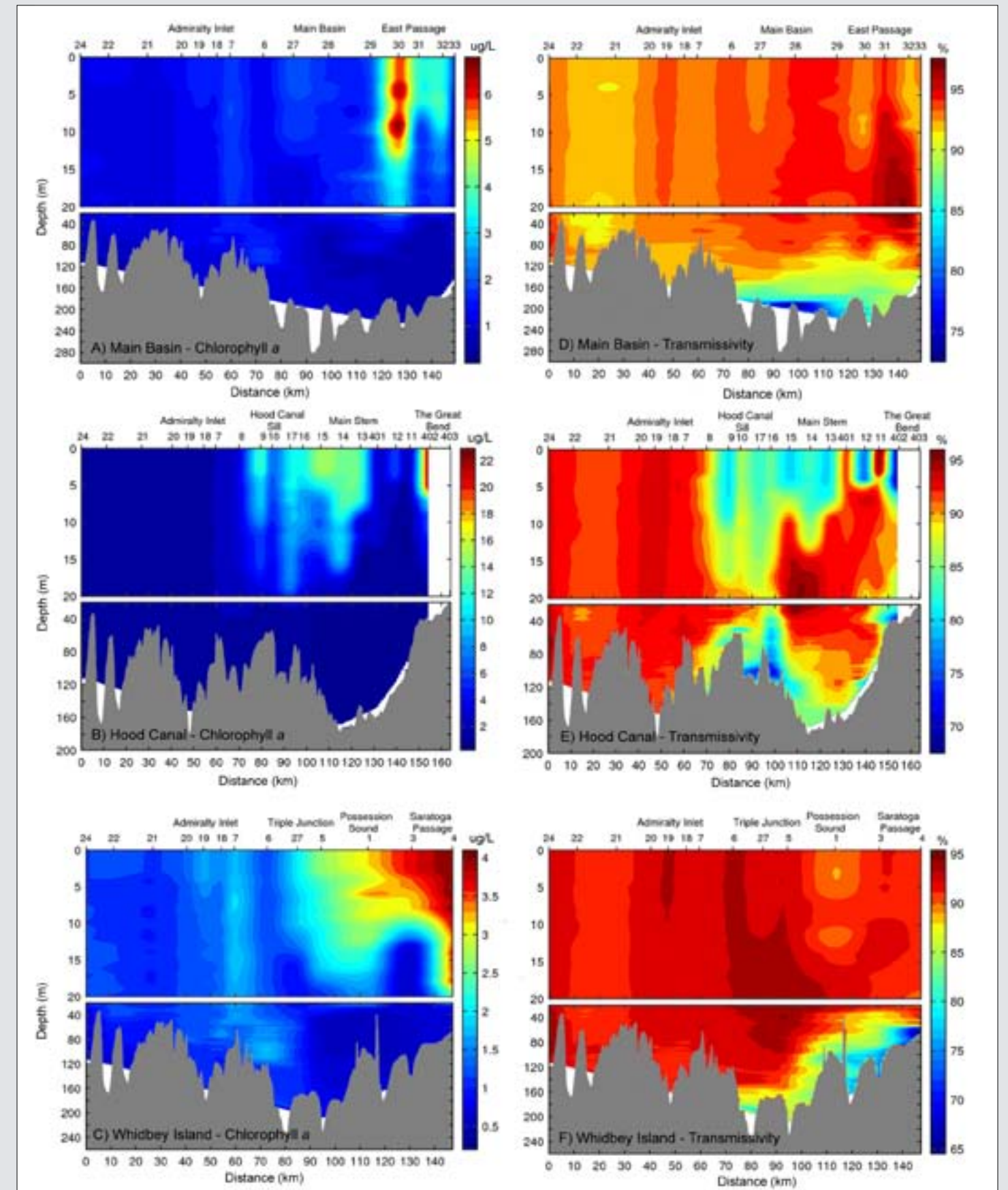
Figure 23. Sections from the UW October 2011 PRISM-NANOOS cruise showing chlorophyll in (A) Main Basin, (B) Hood Canal, and (C) Whidbey Basin, and transmissivity in (D) Main Basin, (E) Hood Canal, and (F) Whidbey Basin.
