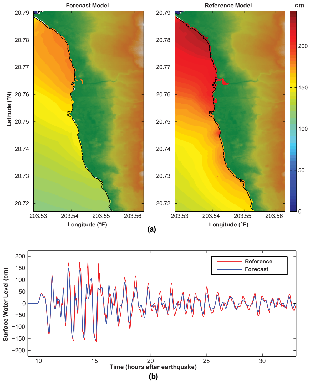
Figure 21: Representative plot of minimal or no inundation. Forecast and reference model comparison for synthetic case NGSZ 6–15: (a) maximum tsunami wave amplitude distribution and (b) tsunami time series at the warning point.
