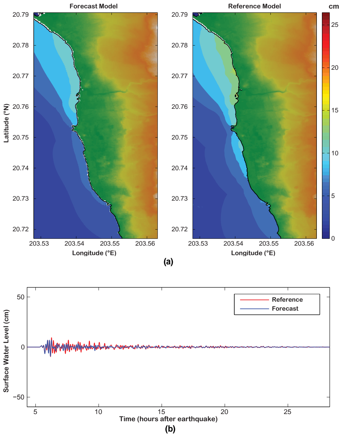
Figure 10: Forecast and reference model comparison of 2003 Rat Island tsunami: (a) maximum tsunami wave amplitude distribution and (b) tsunami time series at the warning point.
