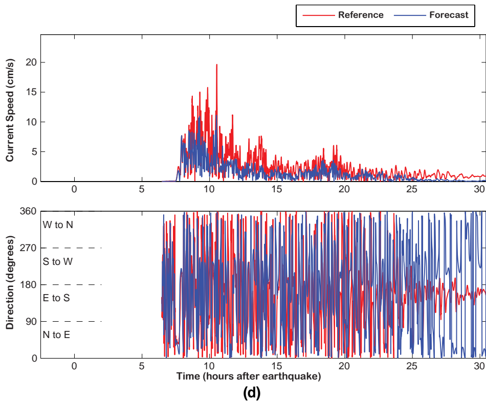
Figure 9, continued: Forecast and reference model comparison of 1994 East Kuril tsunami: (c) maximum current speed distribution and (d) current speed and directionality at the warning point.
