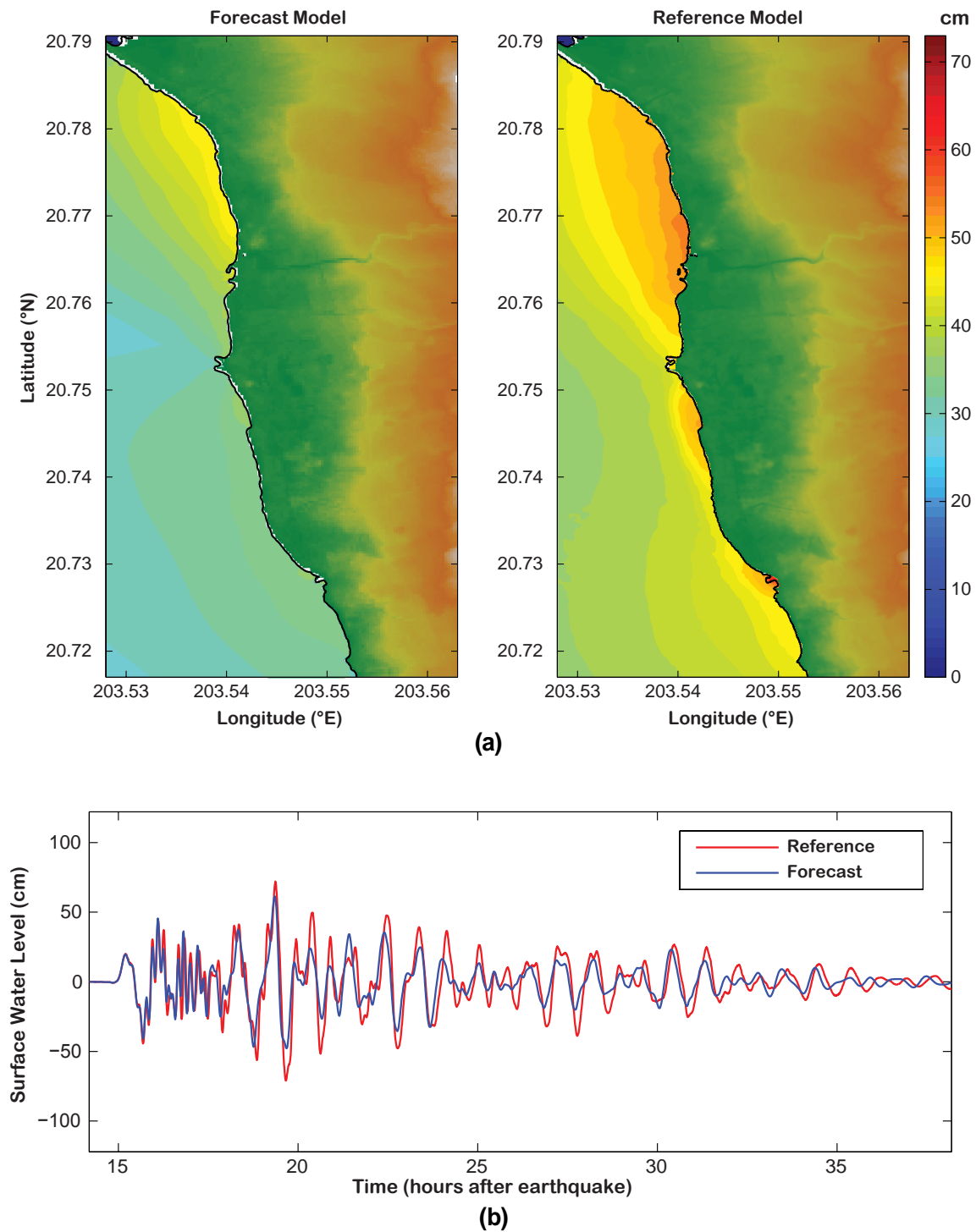
Figure 17: Forecast and reference model comparison of 2010 Chile tsunami: (a) maximum tsunami wave amplitude distribution and (b) tsunami time series at the warning point.
