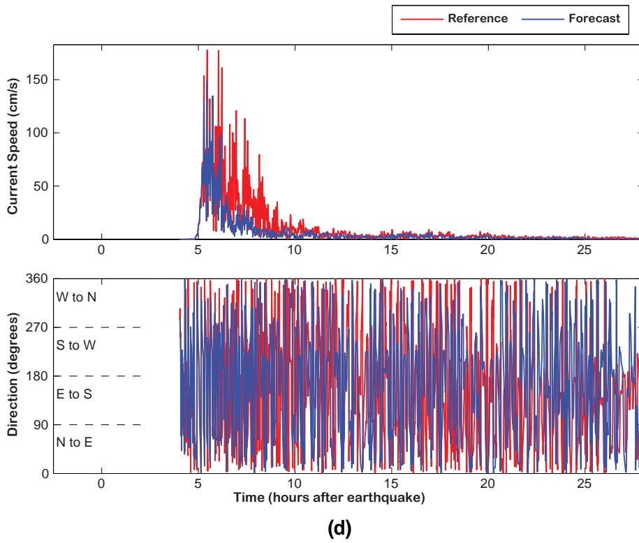
Figure 6, continued: Forecast and reference model comparison of 1946 Unimak tsunami: (c) maximum current speed distribution and (d) current speed and directionality at the warning point.
