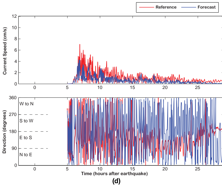
Figure 16, continued: Forecast and reference model comparison of 2009 Samoa tsunami: (c) maximum current speed distribution and (d) current speed and directionality at the warning point.
