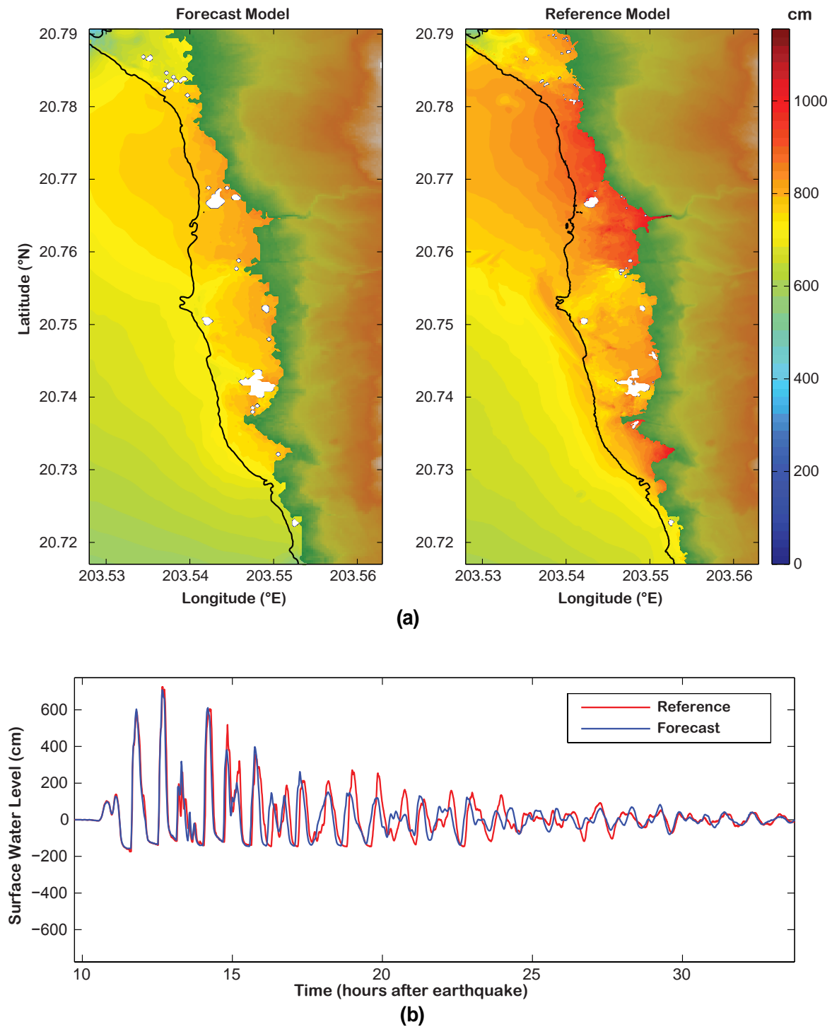
Figure 19: Representative plot of extreme inundation. White spots on land indicate non-inundated areas. Forecast and reference model comparison for synthetic case EPSZ 9–18: (a) maximum tsunami wave amplitude distribution and (b) tsunami time series at the warning point.
