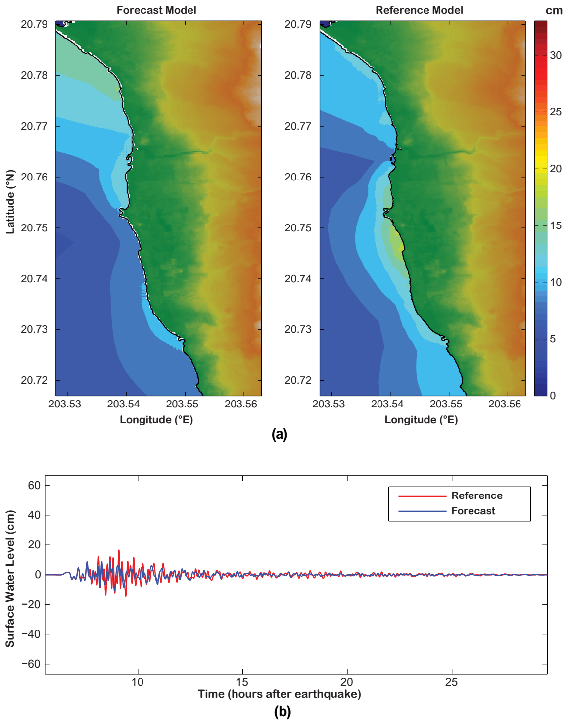
Figure 11: Forecast and reference model comparison of 2006 Tonga tsunami: (a) maximum tsunami wave amplitude distribution and (b) tsunami time series at the warning point.
