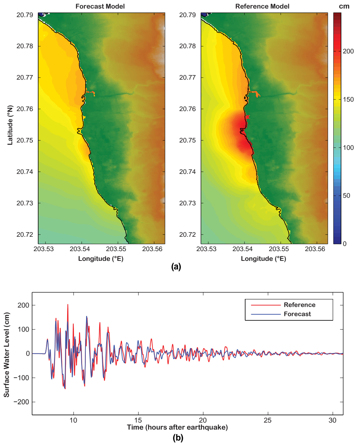
Figure 18: Forecast and reference model comparison of 2011 Tohoku tsunami: (a) maximum tsunami wave amplitude distribution and (b) tsunami time series at the warning point.
