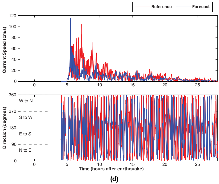
Figure 7, continued: Forecast and reference model comparison of 1957 Andreanof tsunami: (c) maximum current speed distribution and (d) current speed and directionality at the warning point.
