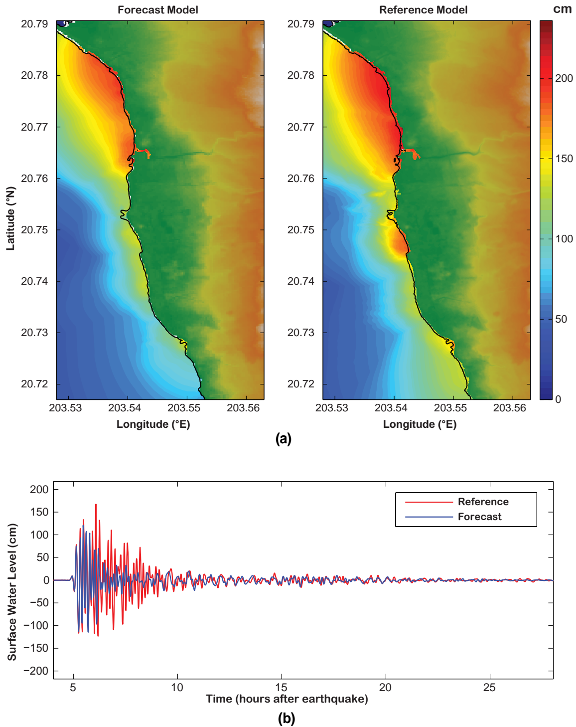
Figure 6: Forecast and reference model comparison of 1946 Unimak tsunami: (a) maximum tsunami wave amplitude distribution and (b) tsunami time series at the warning point.
