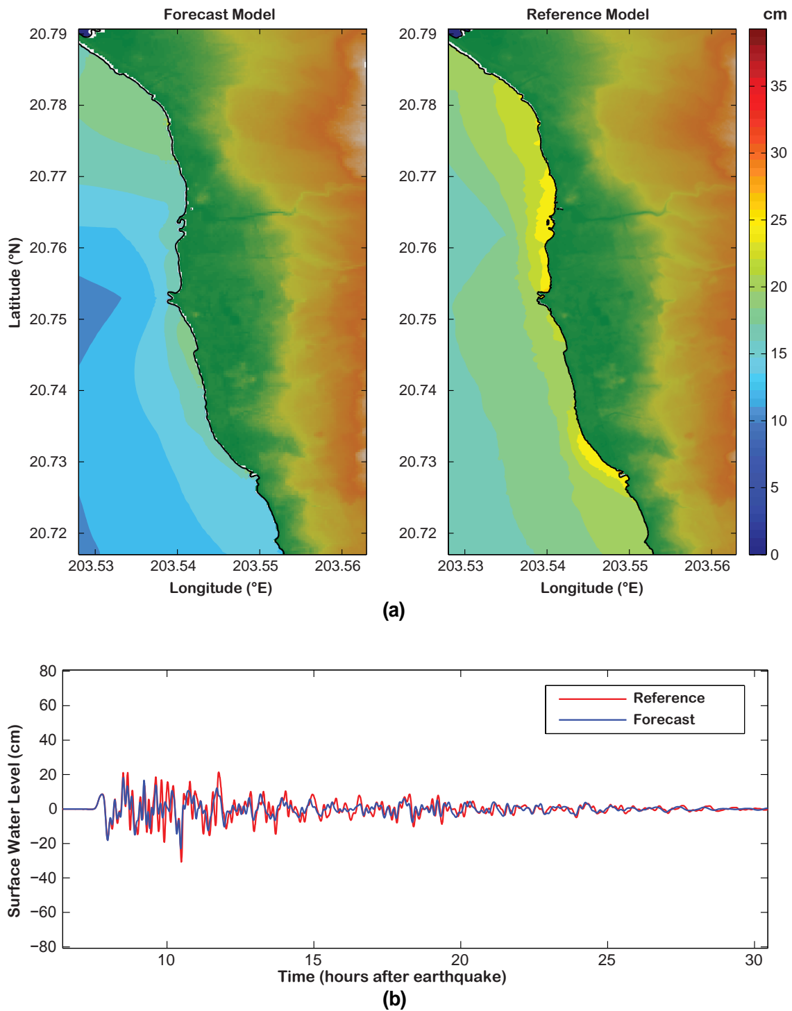
Figure 9: Forecast and reference model comparison of 1994 East Kuril tsunami: (a) maximum tsunami wave amplitude distribution and (b) tsunami time series at the warning point.
