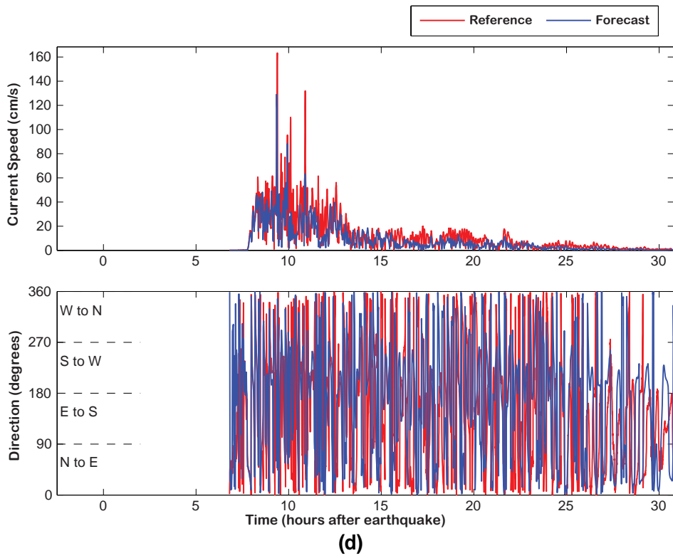
Figure 18, continued: Forecast and reference model comparison of 2011 Tohoku tsunami: (c) maximum current speed distribution and (d) current speed and directionality at the warning point.
