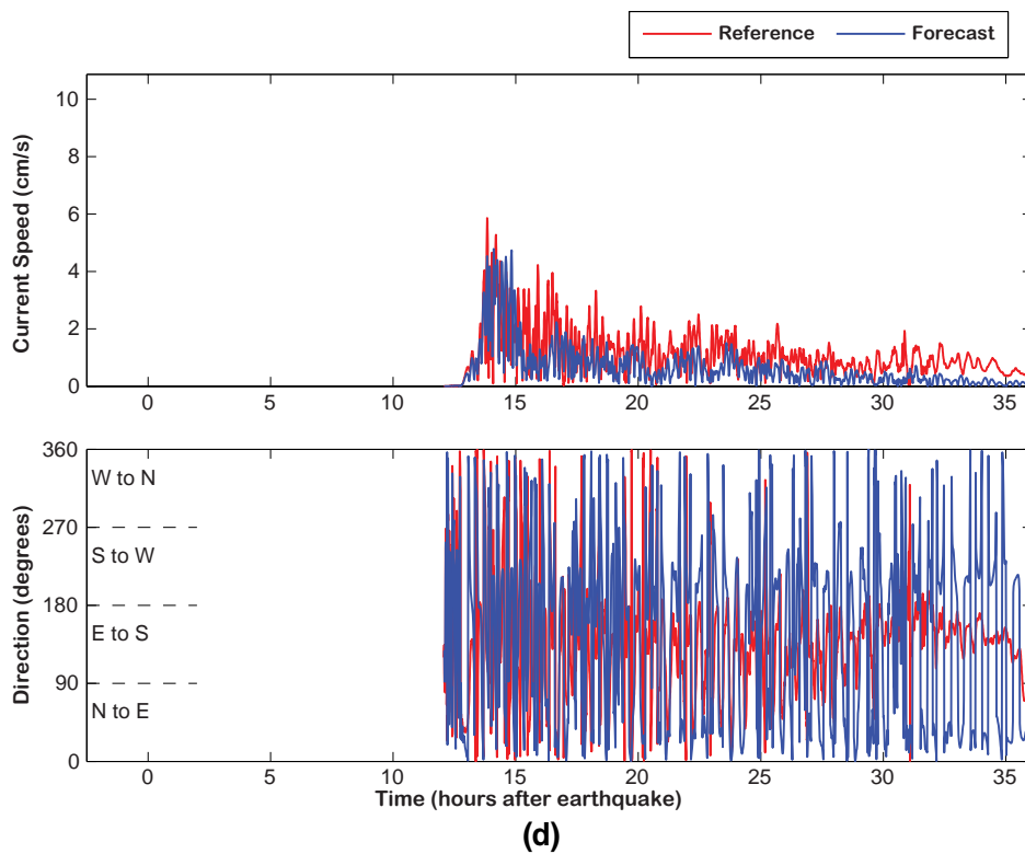
Figure 15, continued: Forecast and reference model comparison of 2007 Peru tsunami: (c) maximum current speed distribution and (d) current speed and directionality at the warning point.
