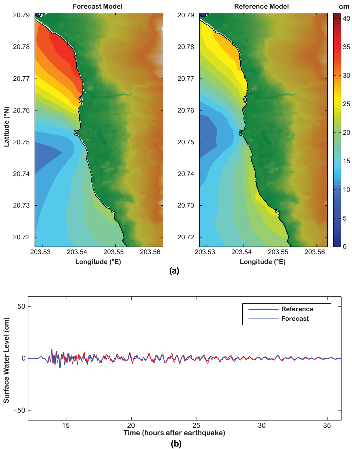
Figure 15: Forecast and reference model comparison of 2007 Peru tsunami: (a) maximum tsunami wave amplitude distribution and (b) tsunami time series at the warning point.
