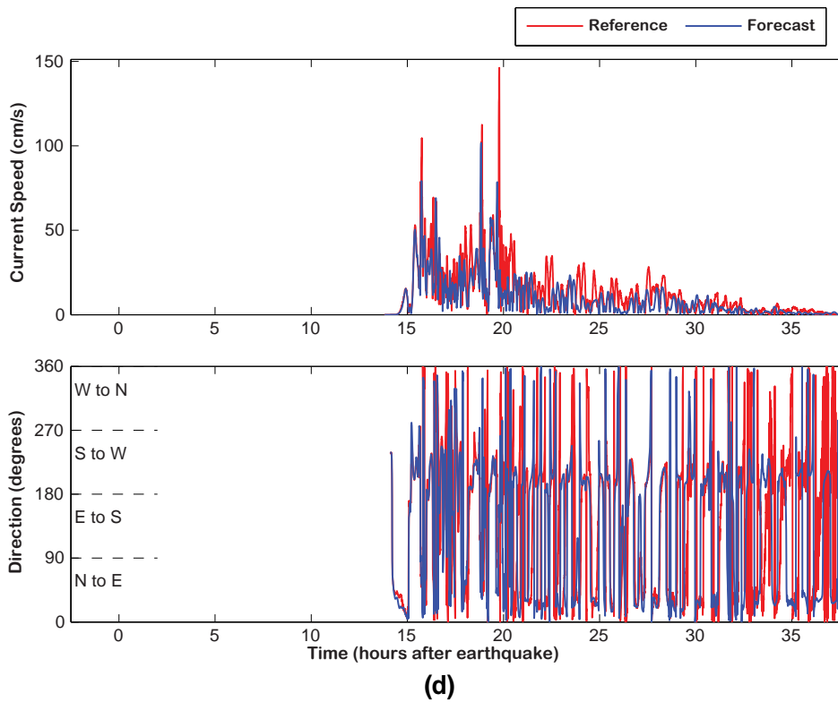
Figure 8, continued: Forecast and reference model comparison of 1960 Chile tsunami: (c) maximum current speed distribution and (d) current speed and directionality at the warning point.
