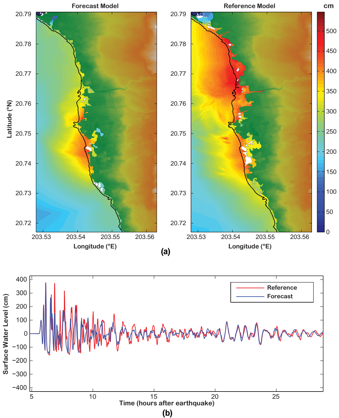
Figure 20: Representative plot of non-extreme but significant inundation. White spots on land indicate non-inundated areas. Forecast and reference model comparison for synthetic case ACSZ 46–55: (a) maximum tsunami wave amplitude distribution and (b) tsunami time series at the warning point.
