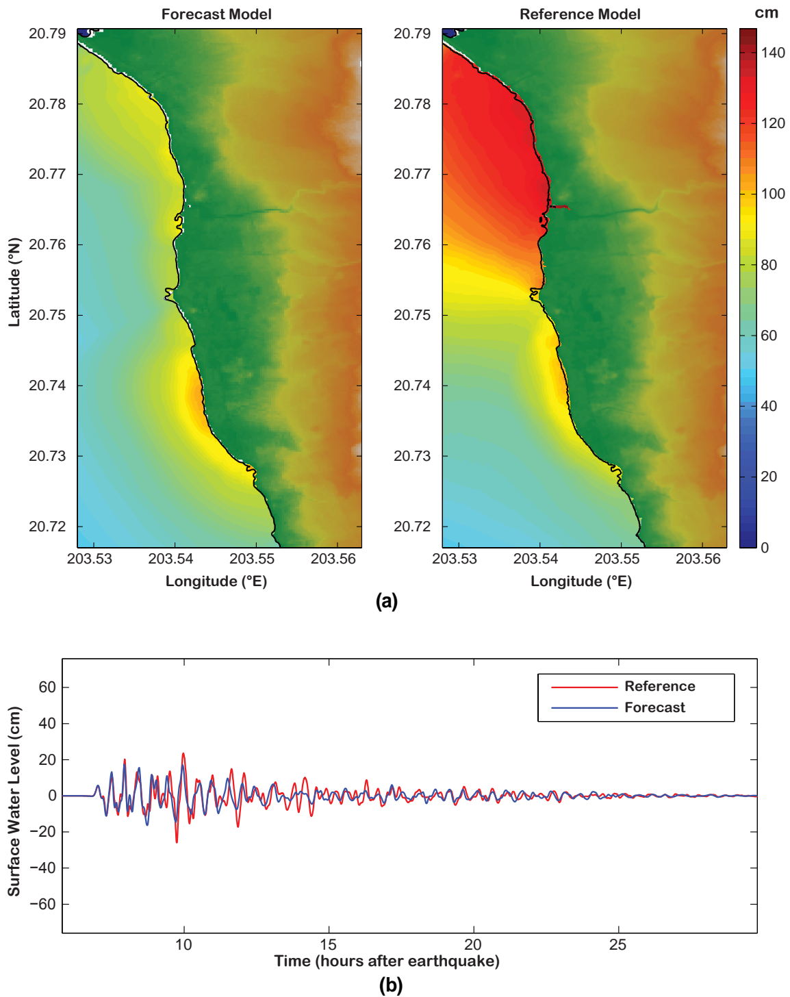
Figure 12: Forecast and reference model comparison of 2006 Kuril tsunami: (a) maximum tsunami wave amplitude distribution and (b) tsunami time series at the warning point.
