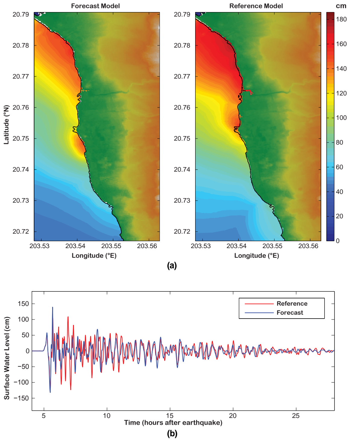
Figure 7: Forecast and reference model comparison of 1957 Andreanof tsunami: (a) maximum tsunami wave amplitude distribution and (b) tsunami time series at the warning point.
