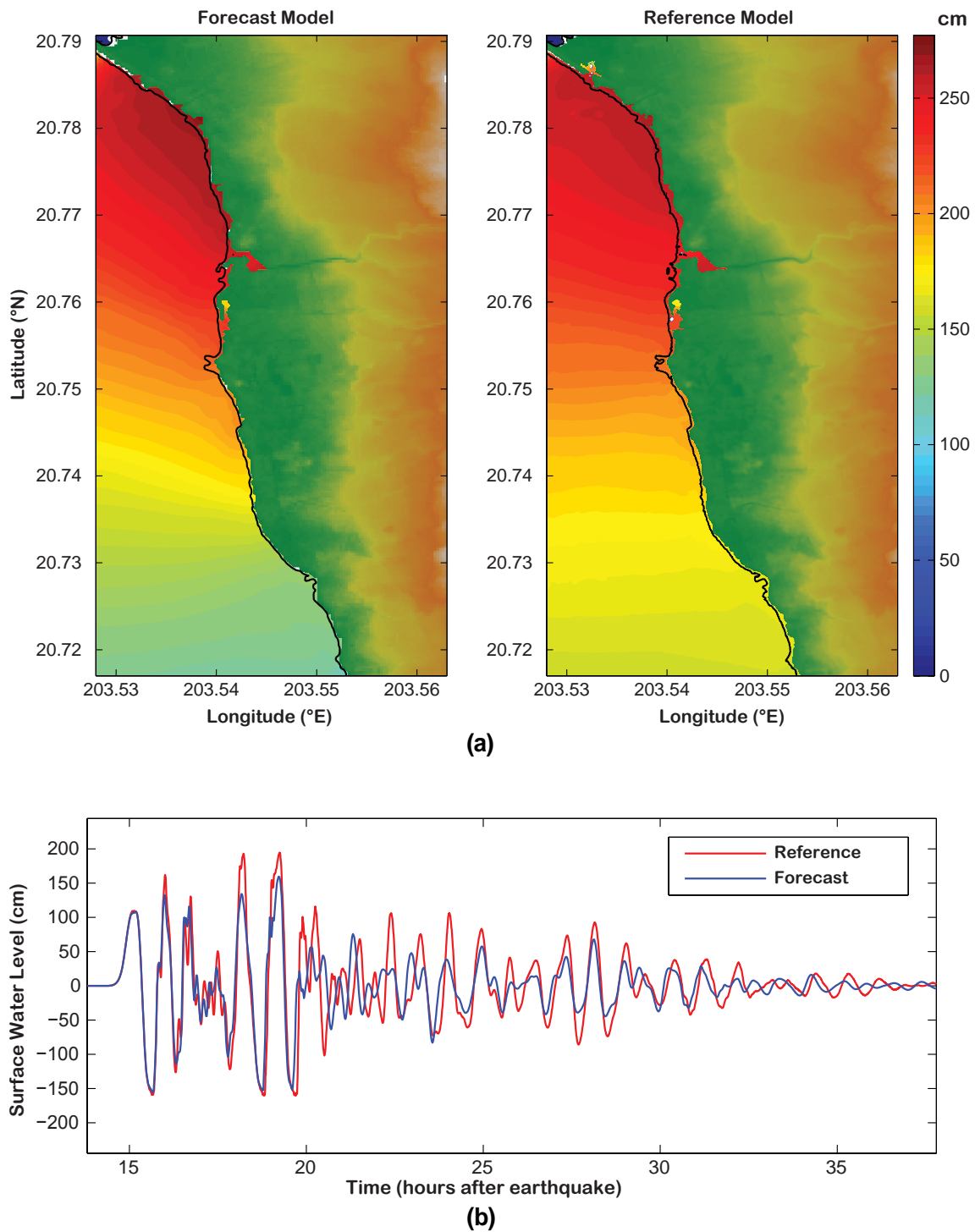
Figure 8: Forecast and reference model comparison of 1960 Chile tsunami: (a) maximum tsunami wave amplitude distribution and (b) tsunami time series at the warning point.
