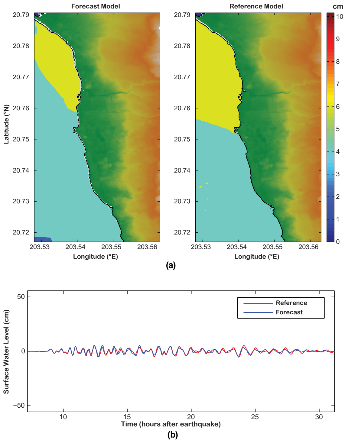
Figure 14: Forecast and reference model comparison of 2007 Solomon tsunami: (a) maximum tsunami wave amplitude distribution and (b) tsunami time series at the warning point.
