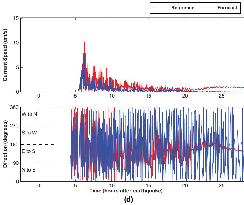
Figure 10, continued: Forecast and reference model comparison of 2003 Rat Island tsunami: (c) maximum current speed distribution and (d) current speed and directionality at the warning point.
