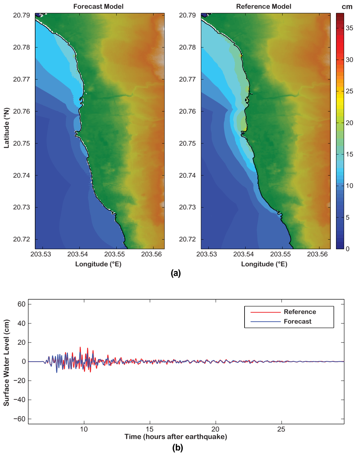
Figure 13: Forecast and reference model comparison of 2007 Kuril tsunami: (a) maximum tsunami wave amplitude distribution and (b) tsunami time series at the warning point.
