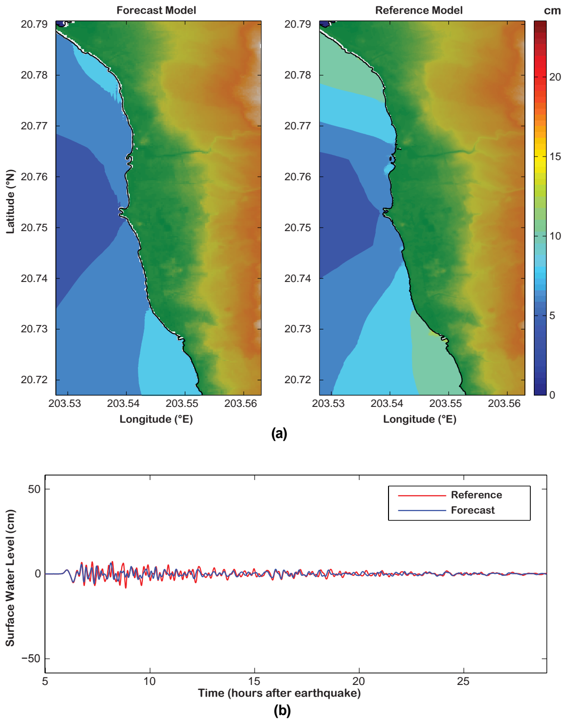
Figure 16: Forecast and reference model comparison of 2009 Samoa tsunami: (a) maximum tsunami wave amplitude distribution and (b) tsunami time series at the warning point.
