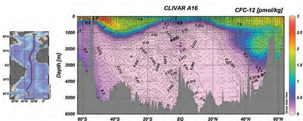
Chlorofluorocarbon-12 (CFC-12) concentrations, used as ocean tracers of circulation and mixing processes, measured along the meridional section A16 in the Atlantic Ocean basin
